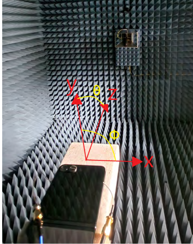
Figure 1: Geometry for A3LSMF731JPN for Radiation patterns.
