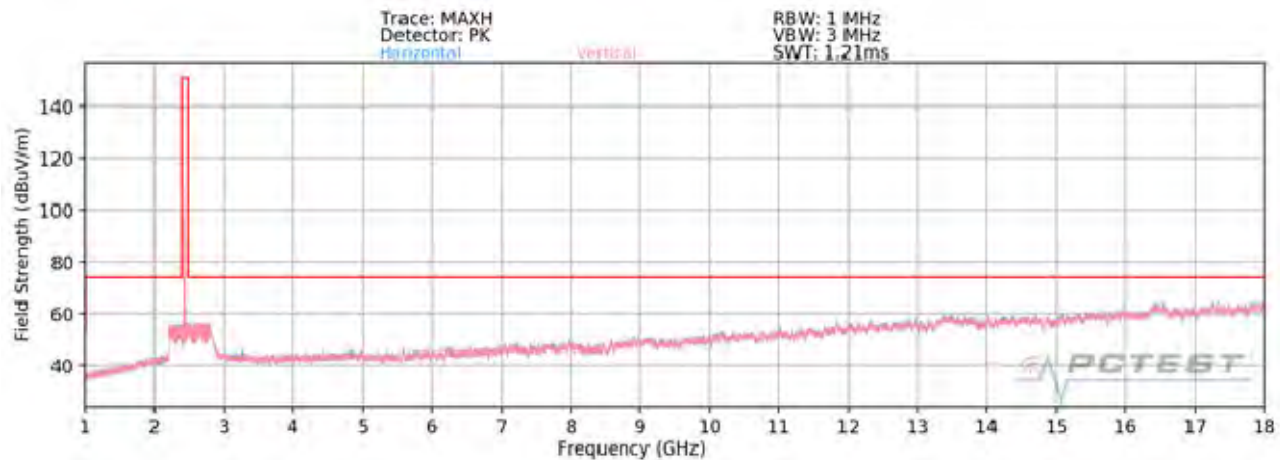
Plot 7-94. Radiated Spurious Plot above 1GHz SISO ANT1 (802.11b – Ch. 6)
