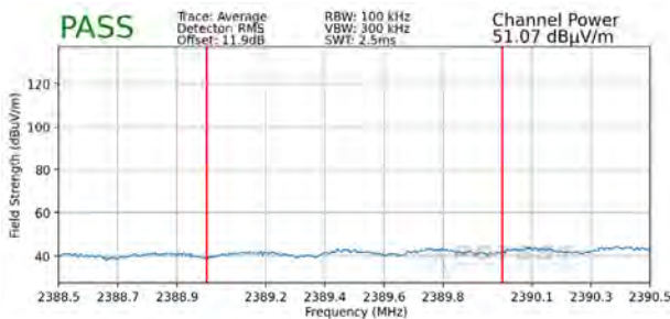
Plot 7-121. Radiated Restricted Lower Band Edge Measurement MIMO (Average)
