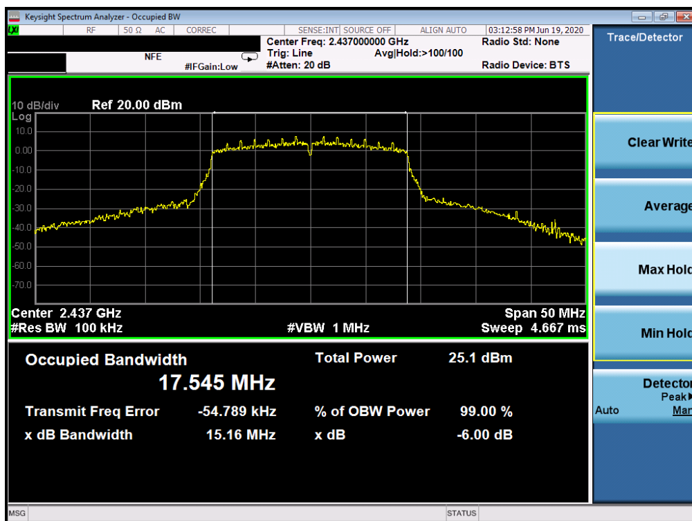
Plot 7-20. 6dB Bandwidth Plot SISO ANT1 (802.11n (2.4GHz) – Ch. 6)
