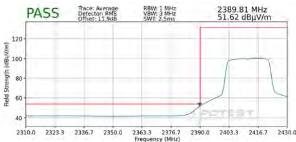
Plot 7-113. Radiated Restricted Lower Band Edge Measurement SISO ANT2 (Average)
