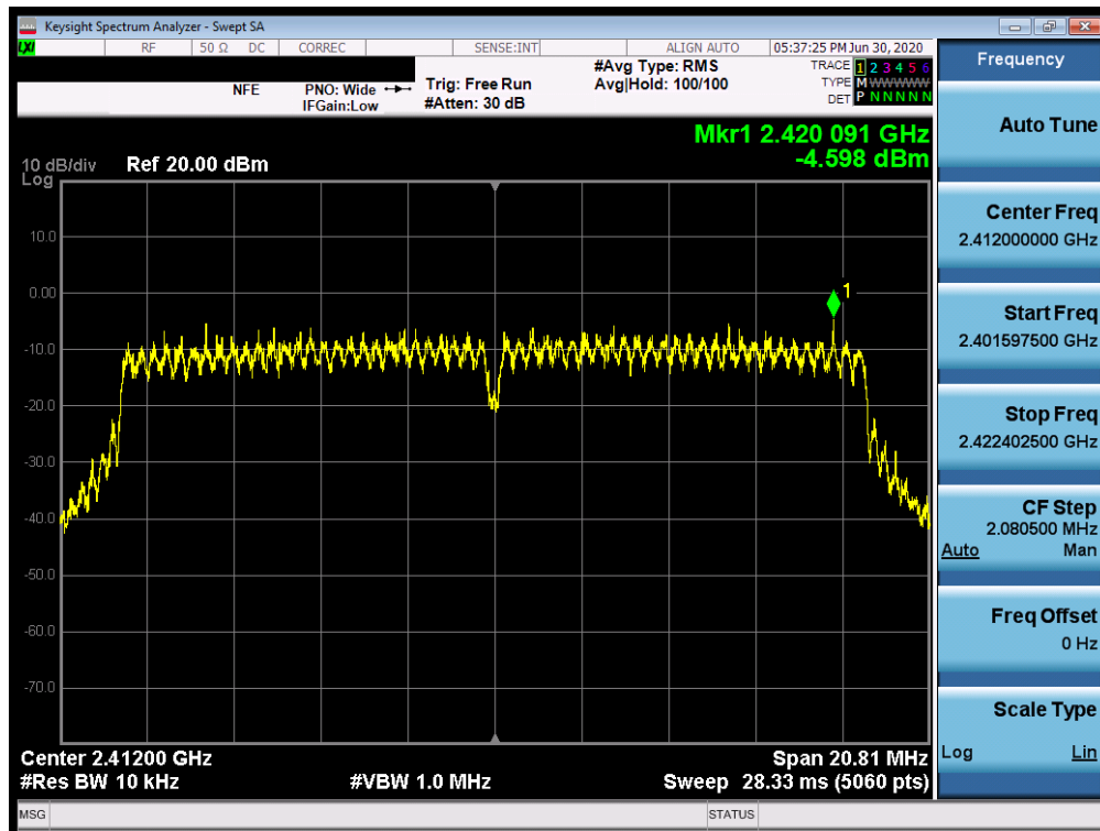
Plot 7-31. Power Spectral Density Plot SISO ANT1 (802.11n (2.4GHz) – Ch. 1)
