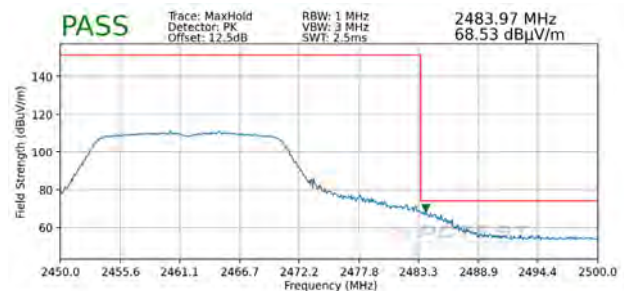
Plot 7-116. Radiated Restricted Upper Band Edge Measurement SISO ANT2 (Peak)
