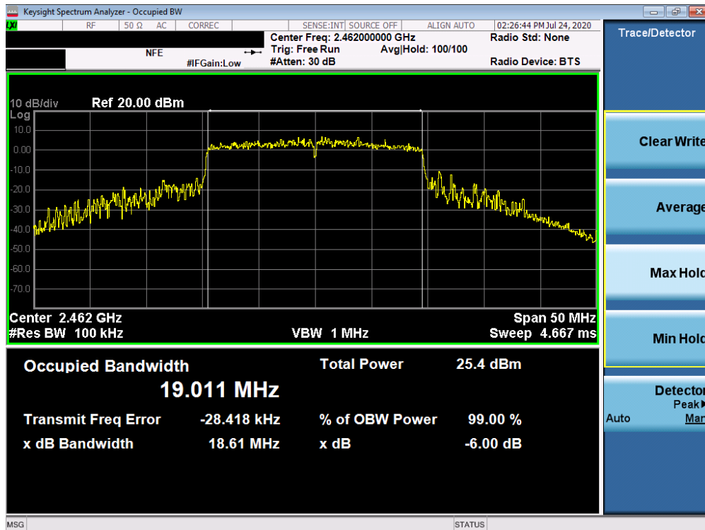
Plot 7-24. 6dB Bandwidth Plot SISO ANT1 (802.11ax (2.4GHz) - Ch. 11)
