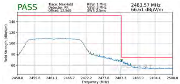
Plot 7-108. Radiated Restricted Upper Band Edge Measurement SISO ANT1 (Peak)
