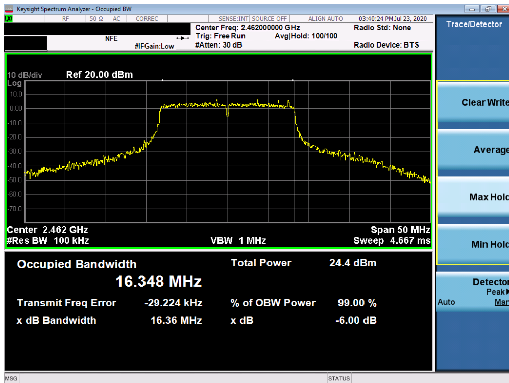
Plot 7-18. 6dB Bandwidth Plot SISO ANT1 (802.11g – Ch. 11)
