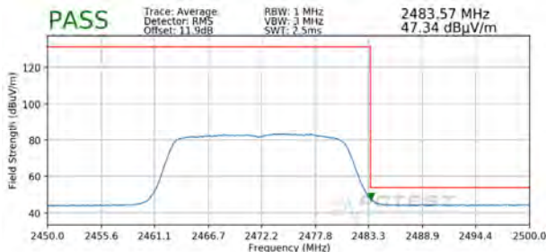
Plot 7-131. Radiated Restricted Upper Band Edge Measurement MIMO (Average)
