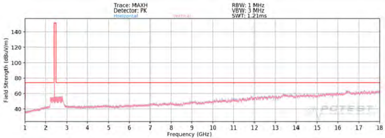
Plot 7-93. Radiated Spurious Plot above 1GHz SISO ANT1 (802.11b – Ch. 1)
