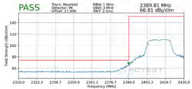
Plot 7-106. Radiated Restricted Lower Band Edge Measurement SISO ANT1 (Peak)
