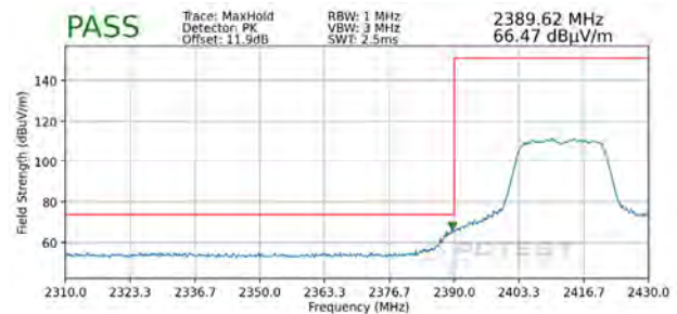
Plot 7-122. Radiated Restricted Lower Band Edge Measurement MIMO (Peak)
