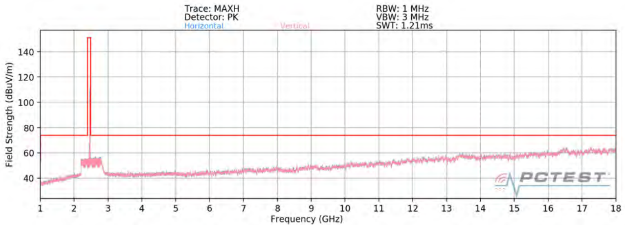
Plot 7-99. Radiated Spurious Plot above 1GHz SISO ANT2 (802.11b – Ch. 11)
