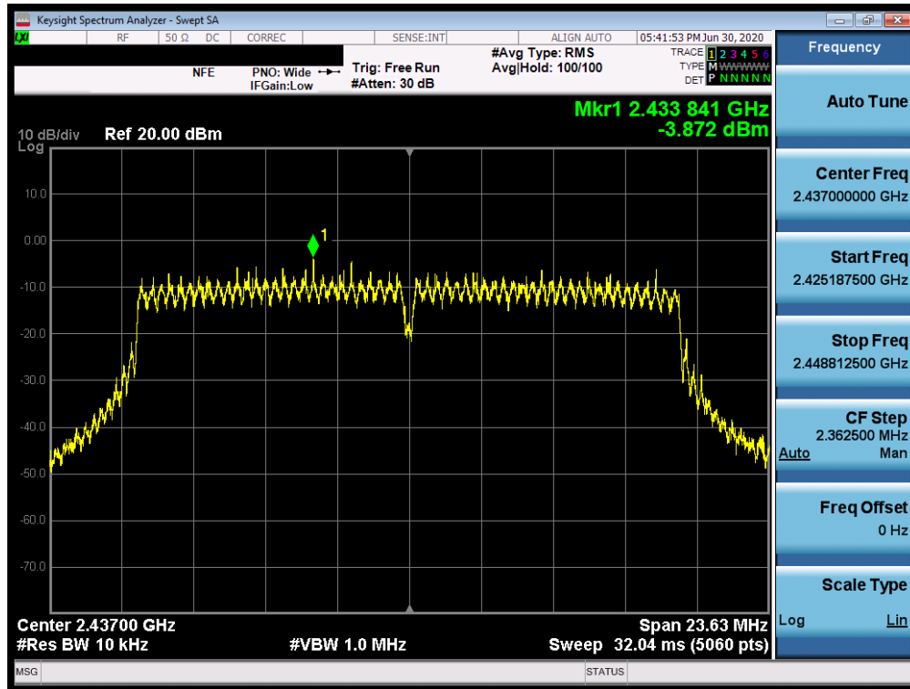
Plot 7-32. Power Spectral Density Plot SISO ANT1 (802.11n (2.4GHz) – Ch. 6)
