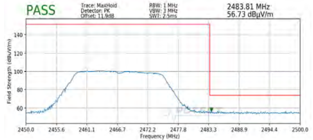
Plot 7-110. Radiated Restricted Upper Band Edge Measurement SISO ANT1 (Peak)
