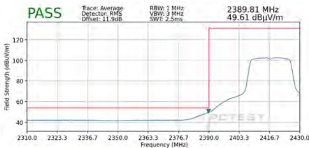
Plot 7-123. Radiated Restricted Lower Band Edge Measurement MIMO (Average)
