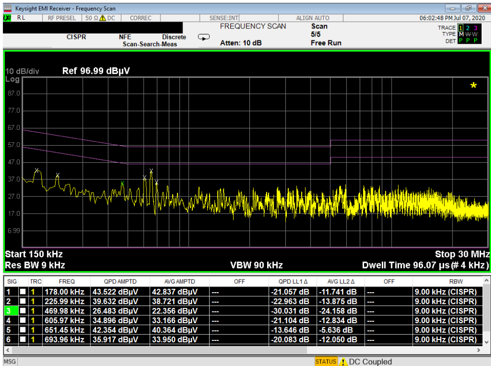
Plot 7-137. Line Conducted Plot with 802.11b (N)
