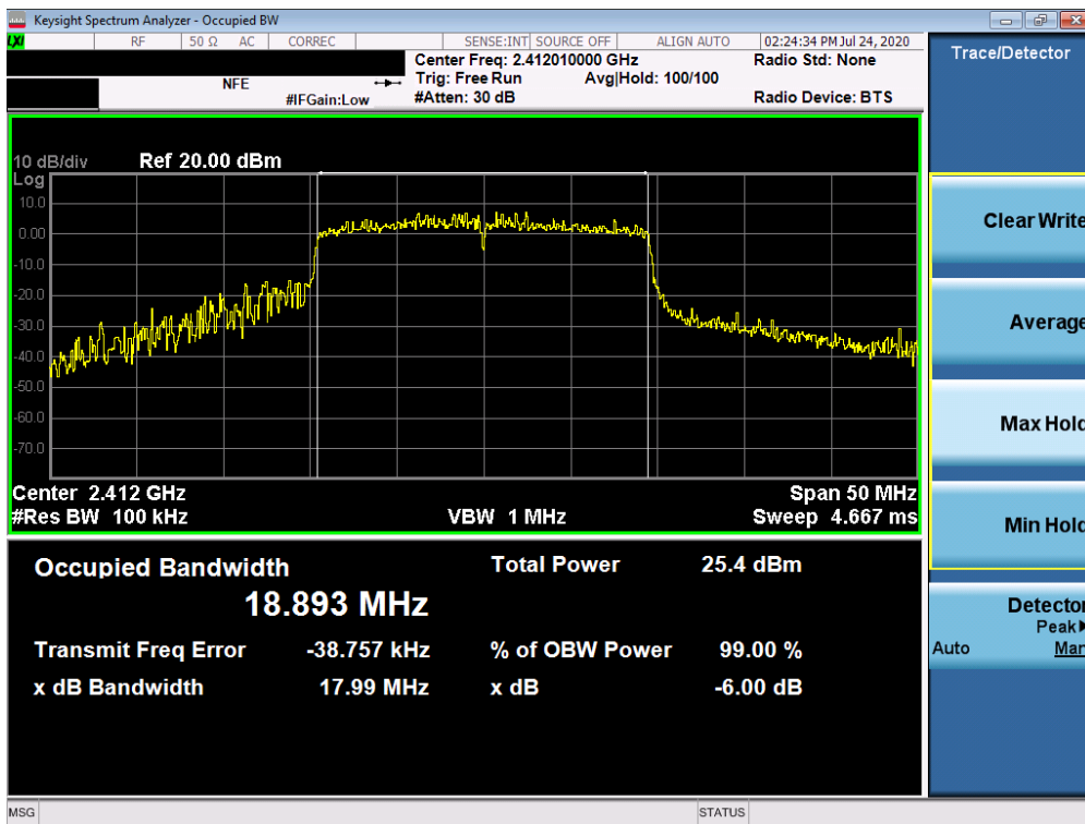
Plot 7-22. 6dB Bandwidth Plot SISO ANT1 (802.11ax (2.4GHz) – Ch. 1)
