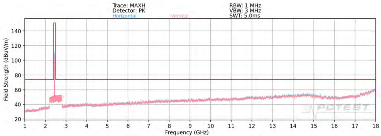
Plot 7-102. Radiated Spurious Plot above 1GHz MIMO/CDD (802.11g – Ch. 6)
