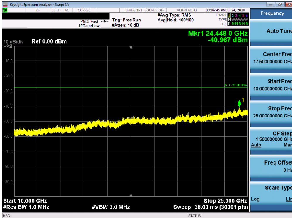
Plot 7-90. Conducted Spurious Plot SISO ANT2 (802.11b – Ch. 6)
