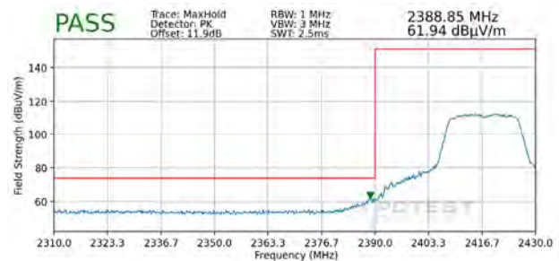
Plot 7-124. Radiated Restricted Lower Band Edge Measurement MIMO (Peak)
