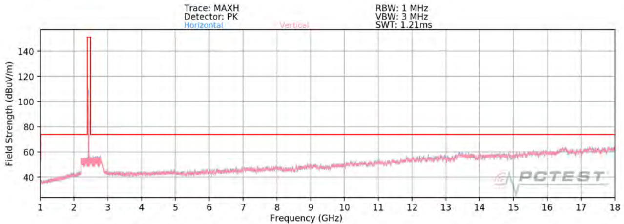
Plot 7-98. Radiated Spurious Plot above 1GHz SISO ANT2 (802.11b – Ch. 6)
