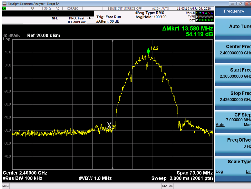
Plot 7-65. Band Edge Plot SISO ANT2 (802.11b - Ch. 1)
