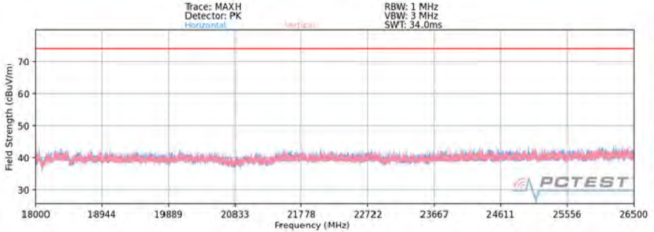
Plot 7-96. Radiated Spurious Plot above 18GHz SISO ANT1
