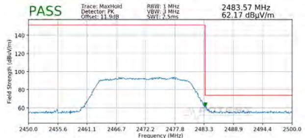
Plot 7-132. Radiated Restricted Upper Band Edge Measurement MIMO (Peak)
