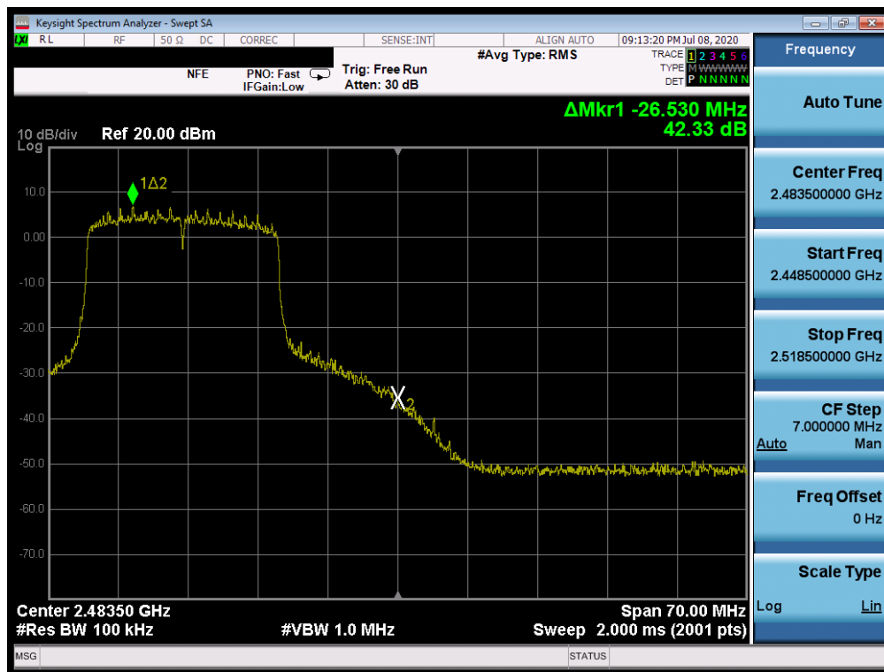
Plot 7-62. Band Edge Plot SISO ANT1 (802.11ax (2.4GHz) – Ch. 11)
