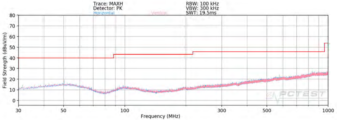
Plot 7-135. Radiated Spurious Plot below 1GHz
