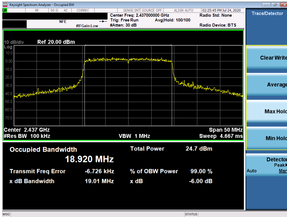
Plot 7-23. 6dB Bandwidth Plot SISO ANT1 (802.11ax (2.4GHz) - Ch. 6)
