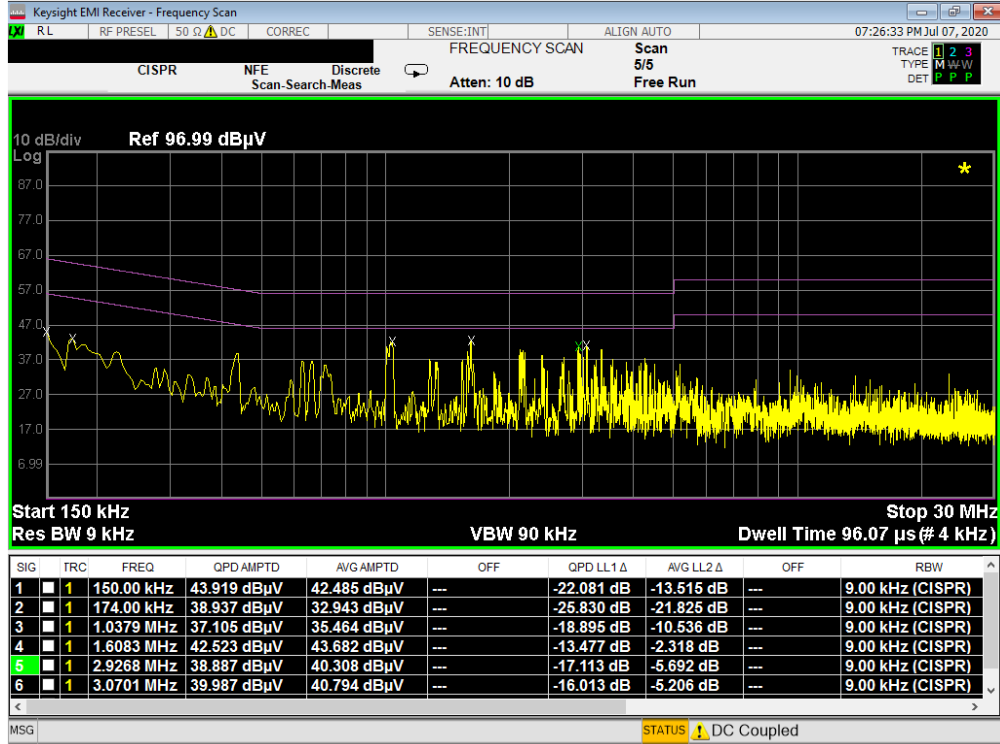
Plot 7-138. Line Conducted Plot with 802.11b (L1) with WCP
