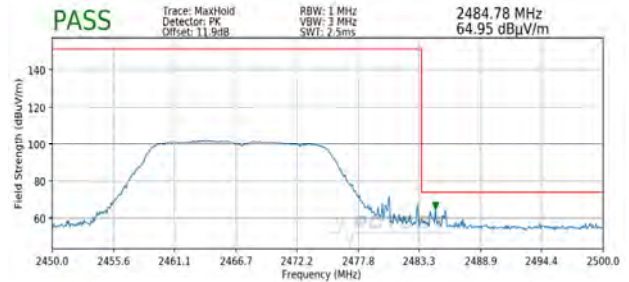
Plot 7-118. Radiated Restricted Upper Band Edge Measurement SISO ANT2 (Peak)
