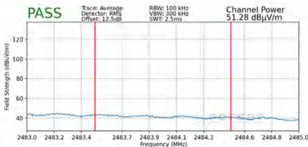
Plot 7-115. Radiated Restricted Upper Band Edge Measurement SISO ANT2 (Average)
