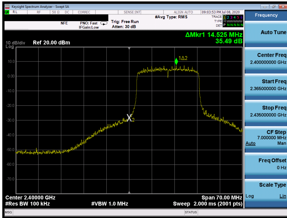
Plot 7-61. Band Edge Plot SISO ANT1 (802.11ax (2.4GHz) – Ch. 1)
