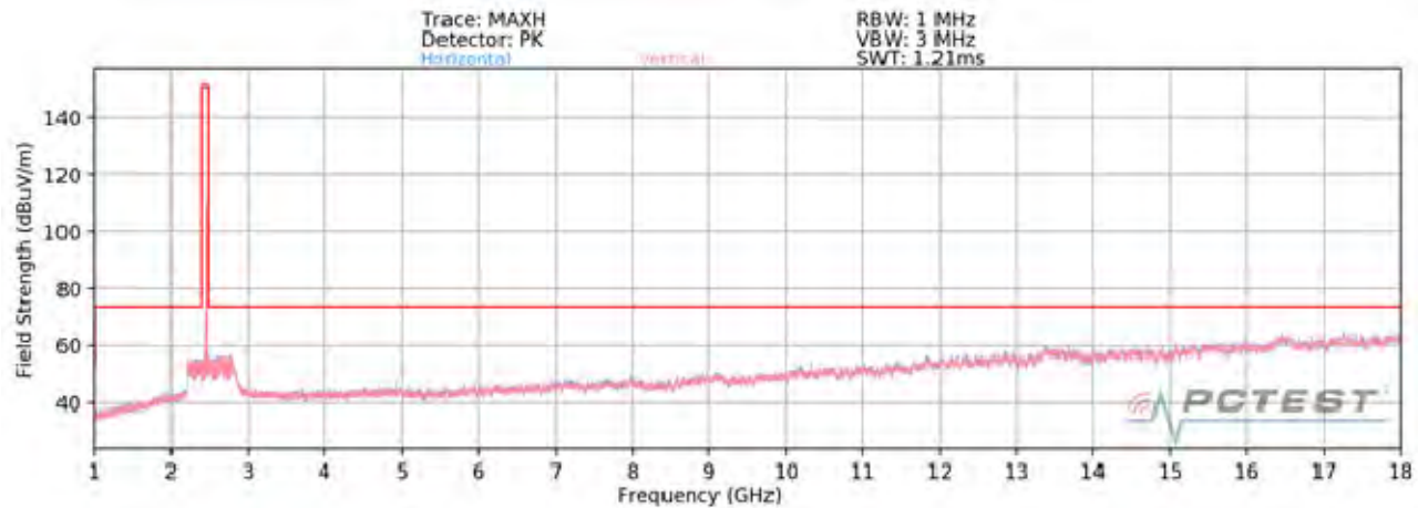
Plot 7-95. Radiated Spurious Plot above 1GHz SISO ANT1 (802.11b – Ch. 11)
