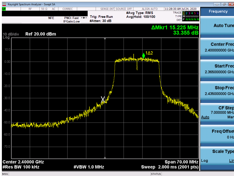
Plot 7-69. Band Edge Plot SISO ANT2 (802.11g- Ch. 1)
