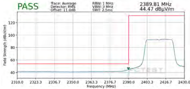
Plot 7-133. Radiated Restricted Band Edge Measurement MIMO with WCP (Average)
