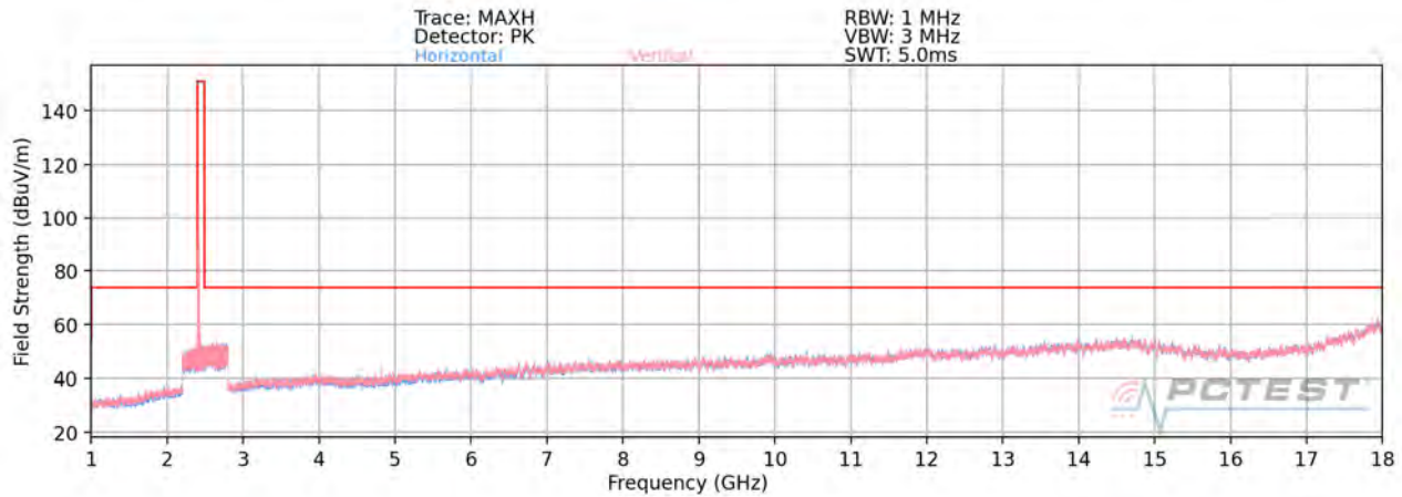
Plot 7-101. Radiated Spurious Plot above 1GHz MIMO/CDD (802.11g – Ch. 1)
