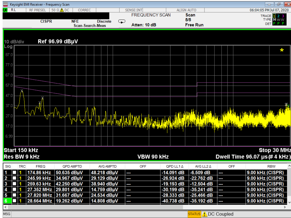
Plot 7-136. Line Conducted Plot with 802.11b (L1)
