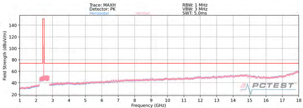
Plot 7-103. Radiated Spurious Plot above 1GHz MIMO/CDD (802.11g – Ch. 11)
