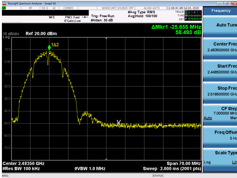
Plot 7-66. Band Edge Plot SISO ANT2 (802.11b - Ch. 11)
