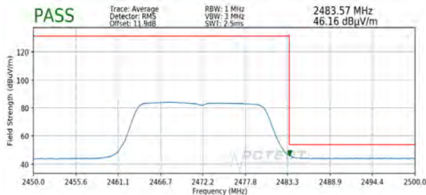
Plot 7-111. Radiated Restricted Upper Band Edge Measurement SISO ANT1 (Average)
