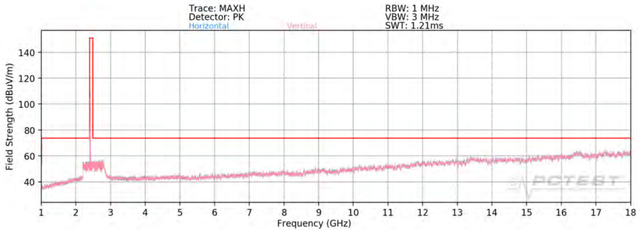
Plot 7-97. Radiated Spurious Plot above 1GHz SISO ANT2 (802.11b – Ch. 1)
