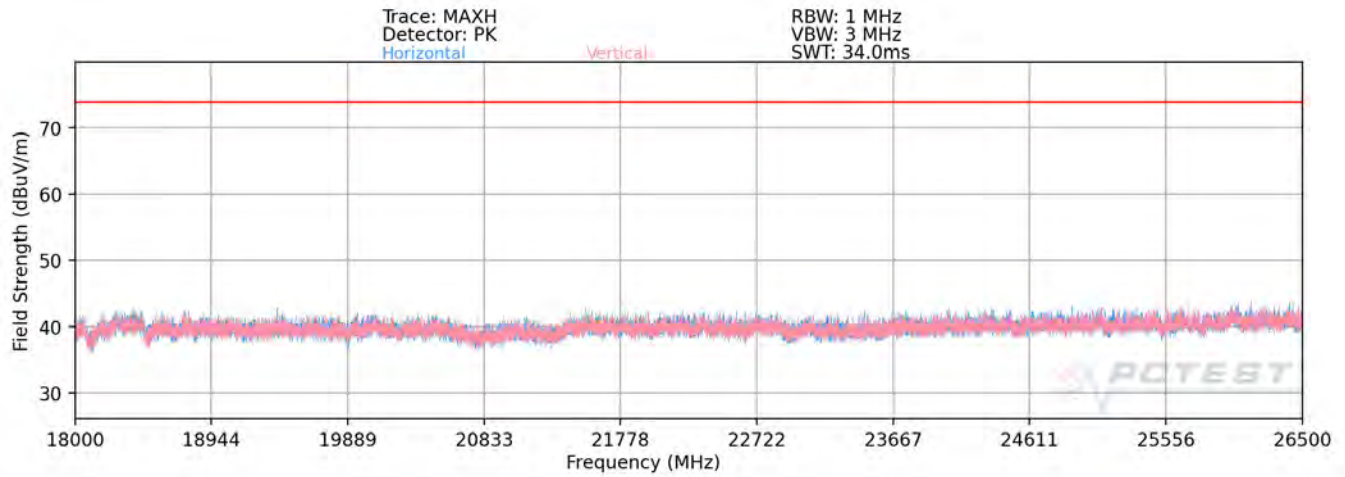
Plot 7-104. Radiated Spurious Plot above 18GHz MIMO/CDD
