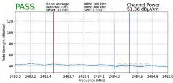
Plot 7-127. Radiated Restricted Upper Band Edge Measurement MIMO (Average)
