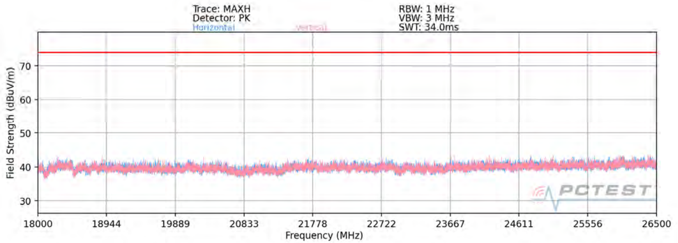
Plot 7-100. Radiated Spurious Plot above 18GHz SISO ANT2
