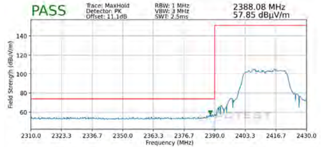
Plot 7-134. Radiated Restricted Band Edge Measurement MIMO with WCP (Peak)
