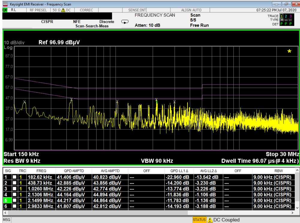
Plot 7-139. Line Conducted Plot with 802.11b (N) with WCP
