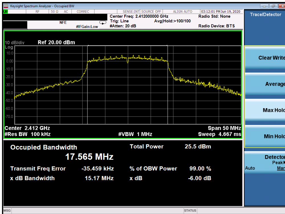
Plot 7-19. 6dB Bandwidth Plot SISO ANT1 (802.11n (2.4GHz) – Ch. 1)
