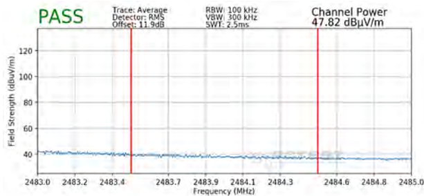
Plot 7-95. Radiated Restricted Upper Band Edge Measurement SISO ANT1 (Average – 106 Tones)
