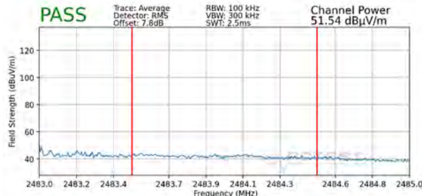
Plot 7-131. Radiated Restricted Upper Band Edge Measurement MIMO (Average - 242 Tones)
