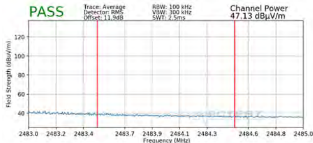
Plot 7-103. Radiated Restricted Upper Band Edge Measurement SISO ANT1 (Average – 242 Tones)
