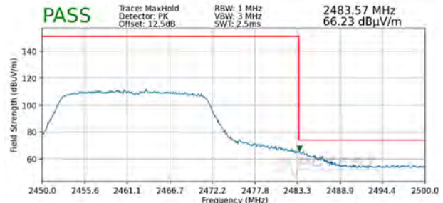
Plot 7-132. Radiated Restricted Upper Band Edge Measurement MIMO (Peak - 242 Tones)
