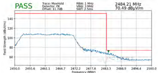
Plot 7-116. Radiated Restricted Upper Band Edge Measurement SISO ANT2 (Peak - 242 Tones)
