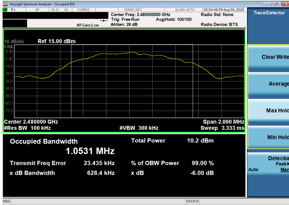
Plot 7-9. 6dB Bandwidth Plot (Bluetooth (LE), 1Mbps – Ch. 39)
