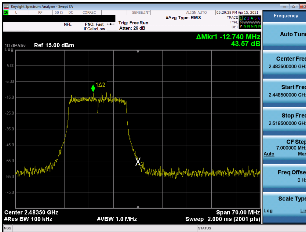
Plot 7-98. Band Edge Plot MIMO ANT1 (802.11g – Ch. 13)
