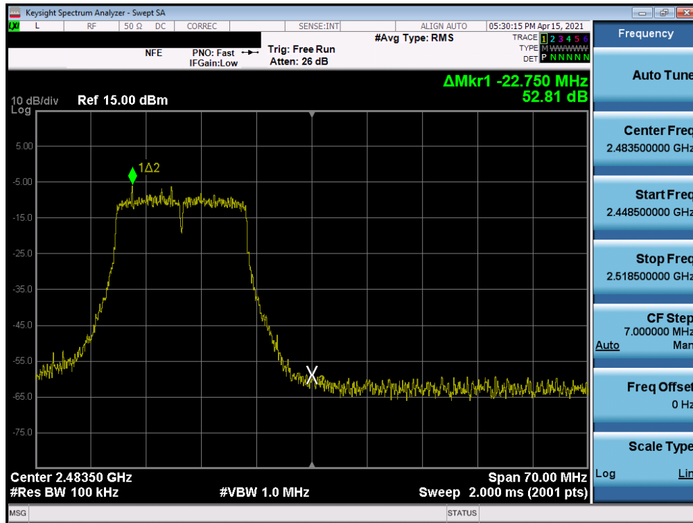
Plot 7-97. Band Edge Plot MIMO ANT1 (802.11g – Ch. 12)
