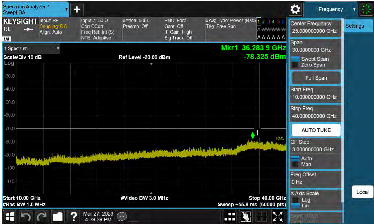
Sub6 n77. Conducted Spurious Plot_2 (662000ch_100 MHz_BPSK)
