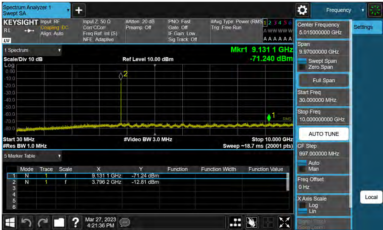
Sub6 n77. Conducted Spurious Plot_1 (656000ch_90 MHz_BPSK)
