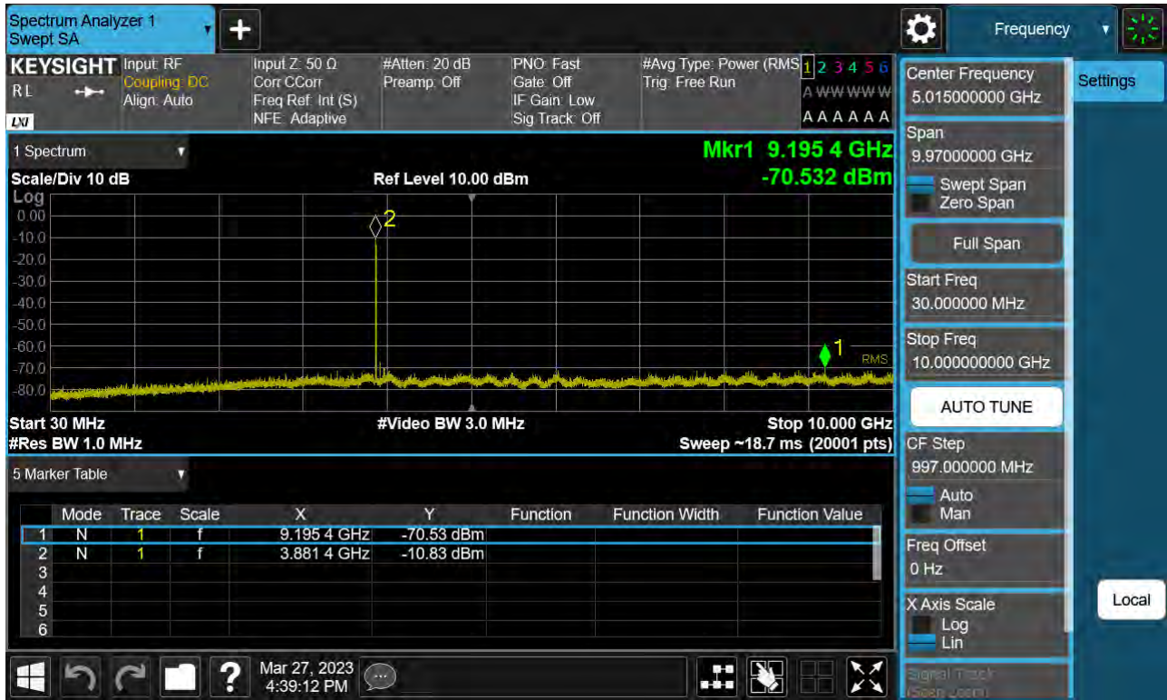
Sub6 n77. Conducted Spurious Plot_1 (662000ch_100 MHz_BPSK)
