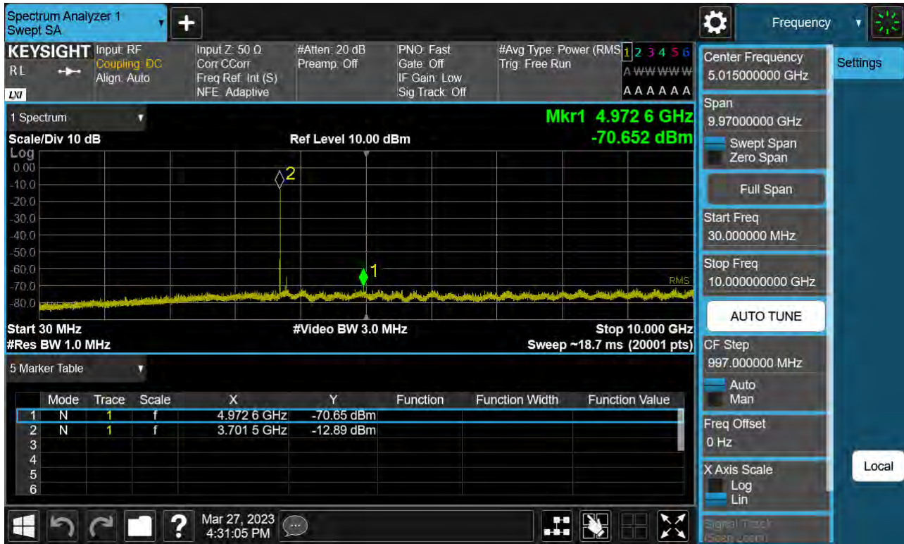
Sub6 n77. Conducted Spurious Plot_1 (650000ch_100 MHz_BPSK)
