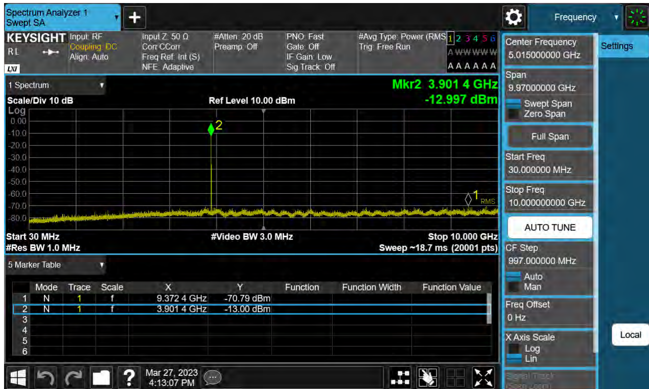
Sub6 n77. Conducted Spurious Plot_1 (662666ch_80 MHz_BPSK)
