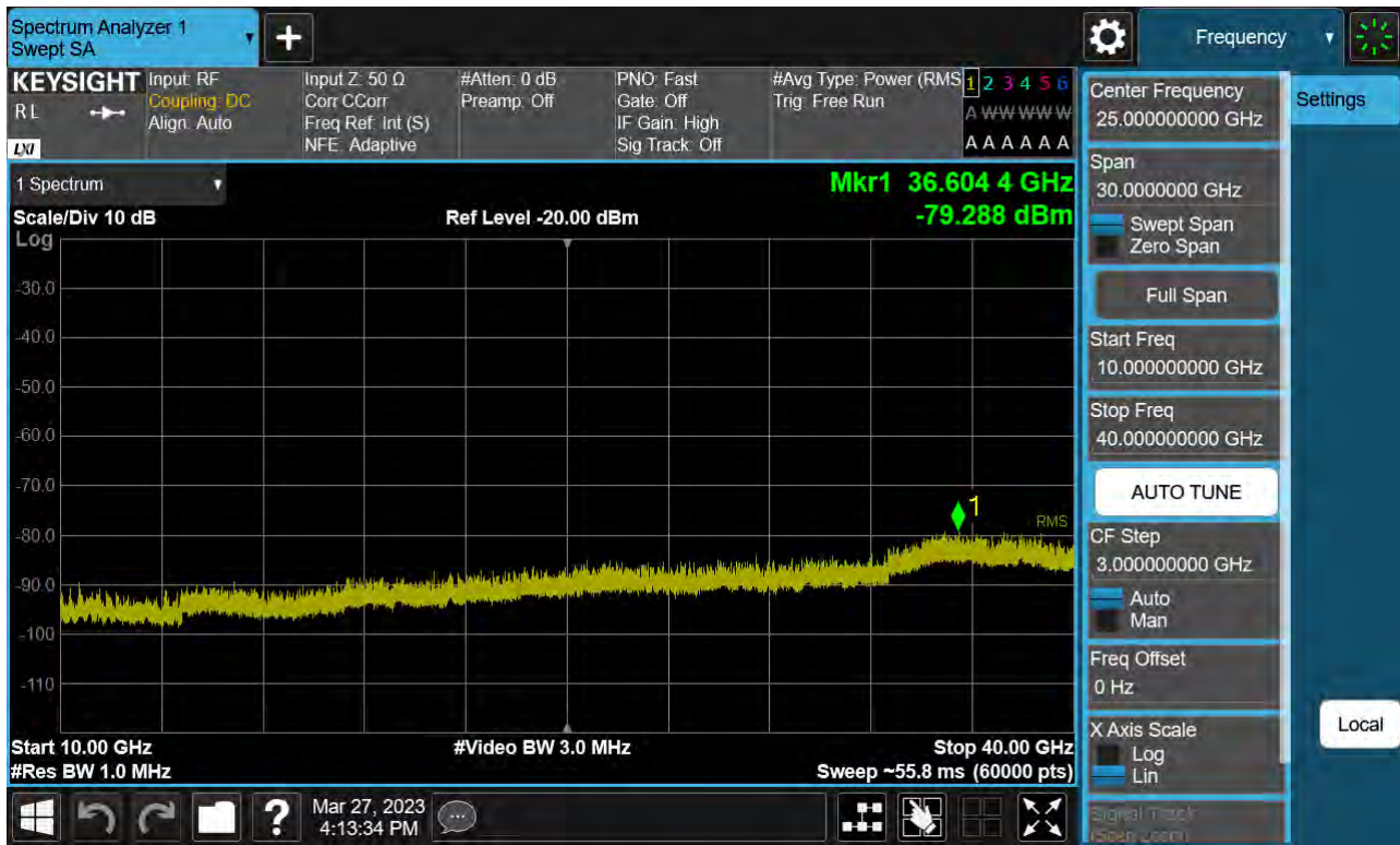
Sub6 n77. Conducted Spurious Plot_2 (662666ch_80 MHz_BPSK)
