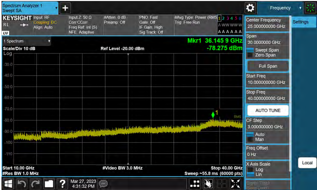
Sub6 n77. Conducted Spurious Plot_2 (650000ch_100 MHz_BPSK)
