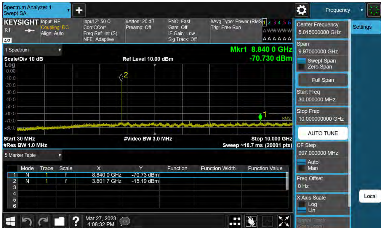
Sub6 n77. Conducted Spurious Plot_1 (656000ch_80 MHz_BPSK)
