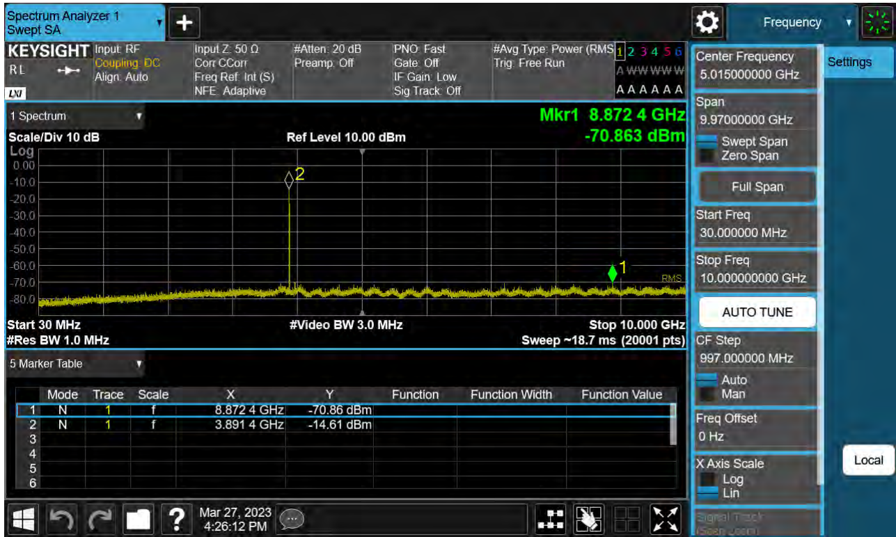
Sub6 n77. Conducted Spurious Plot_1 (662332ch_90 MHz_BPSK)
