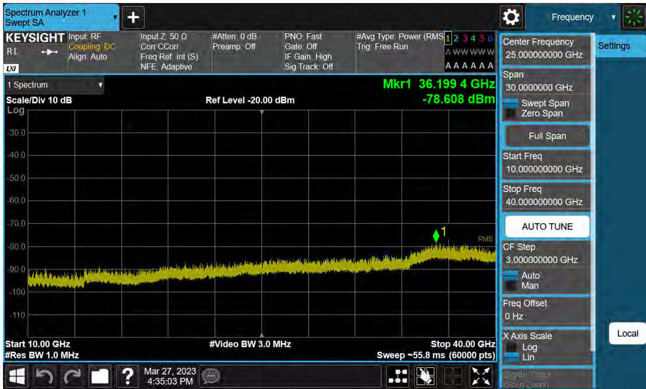
Sub6 n77. Conducted Spurious Plot_2 (656000ch_100 MHz_BPSK)
