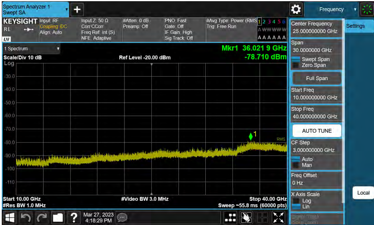
Sub6 n77. Conducted Spurious Plot_2 (649668ch_90 MHz_BPSK)
