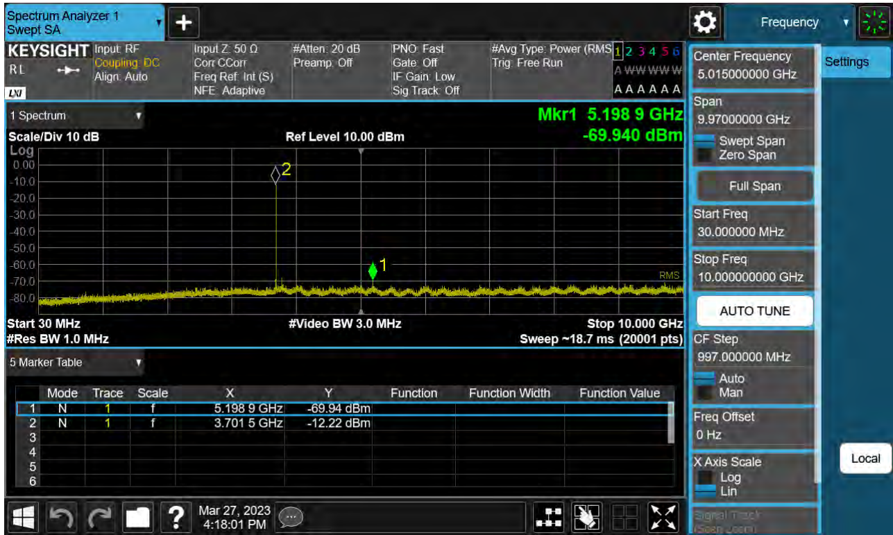
Sub6 n77. Conducted Spurious Plot_1 (649668ch_90 MHz_BPSK)
