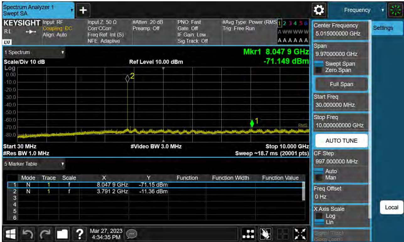
Sub6 n77. Conducted Spurious Plot_1 (656000ch_100 MHz_BPSK)
