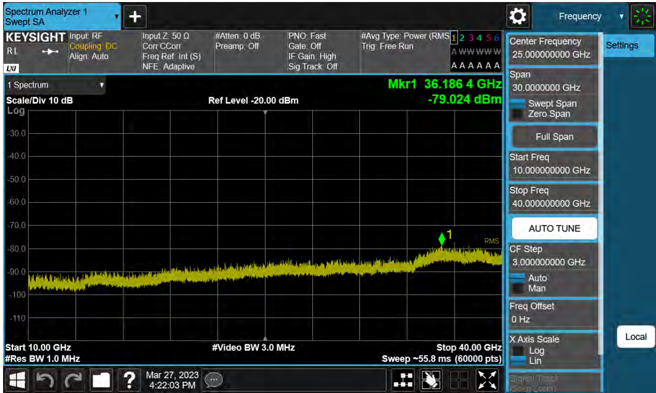
Sub6 n77. Conducted Spurious Plot_2 (656000ch_90 MHz_BPSK)
