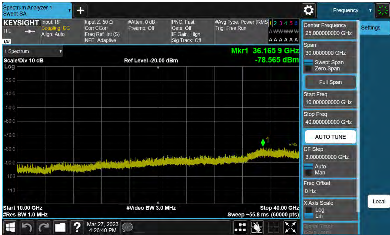
Sub6 n77. Conducted Spurious Plot_2 (662332ch_90 MHz_BPSK)
