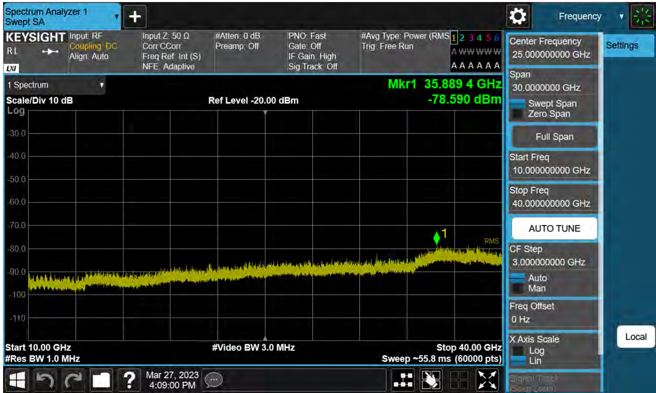
Sub6 n77. Conducted Spurious Plot_2 (656000ch_80 MHz_BPSK)
