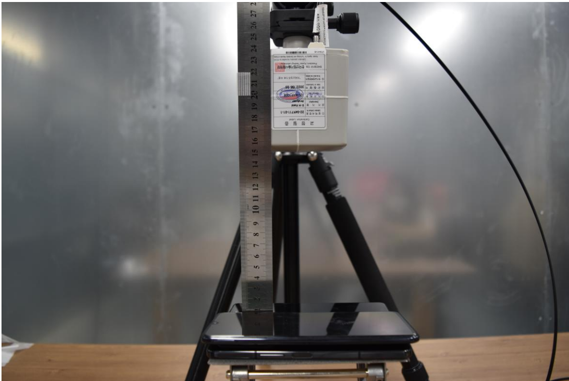
Configuration.7 : Top -Charger below client
