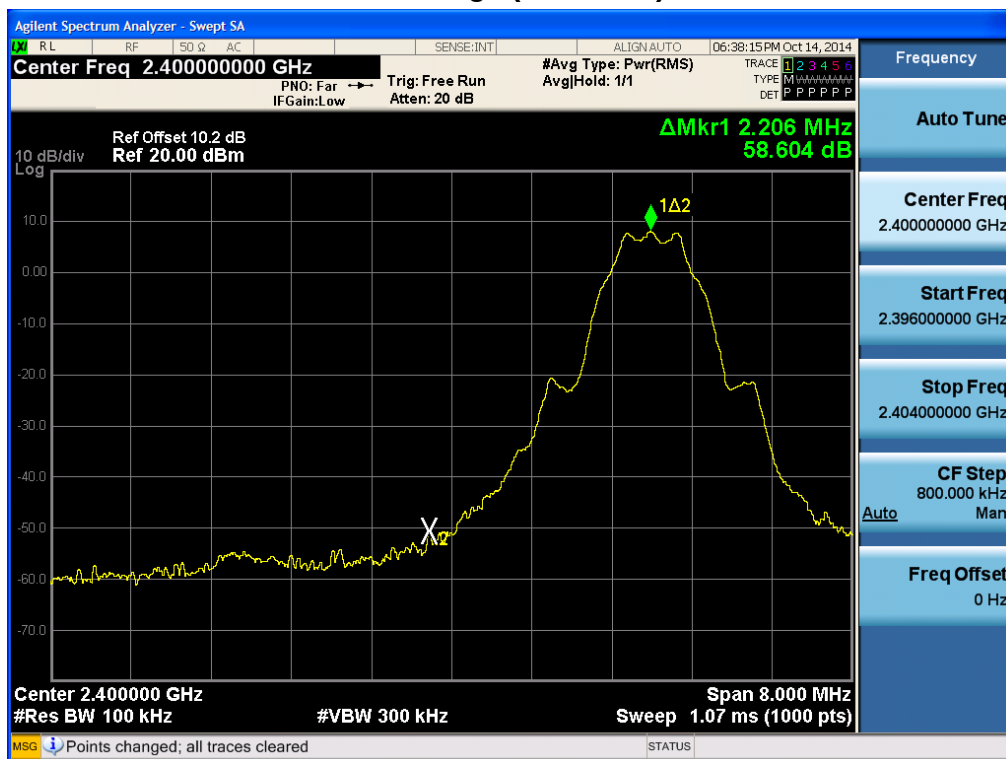
BandEdge (Low-CH 0)
