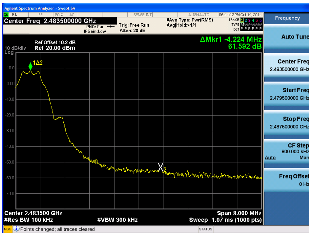
BandEdge (High-CH 39)
