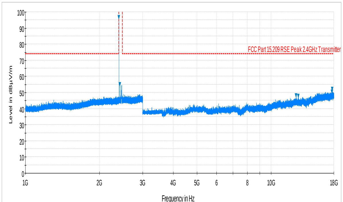
Plot 6-43. Radiated Spurious Plot above 1GHz (Bluetooth – Ch. 0, Ant. Pol. V)
