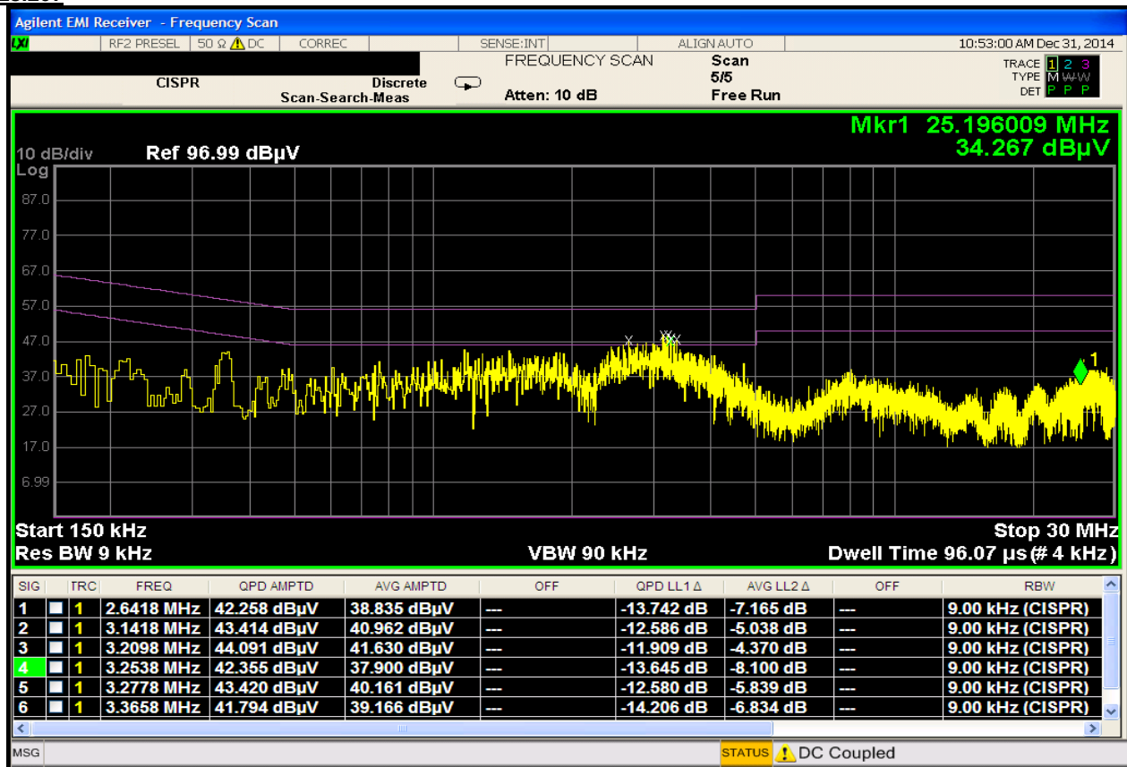
Plot 6-52. Line-Conducted Test Plot (L1)
