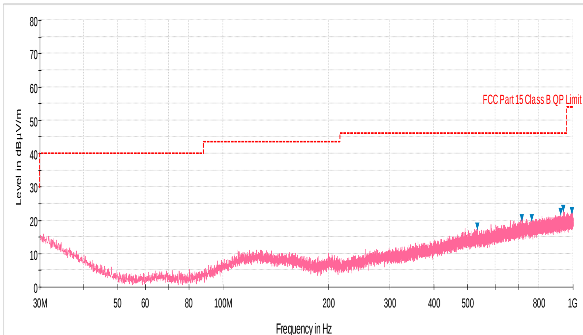
Plot 6-48. Radiated Spurious Plot below 1GHz (Pol. H)
