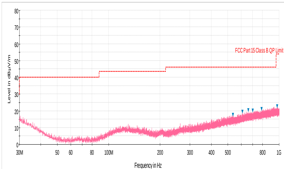
Plot 6-49. Radiated Spurious Plot below 1GHz (Pol. V)
