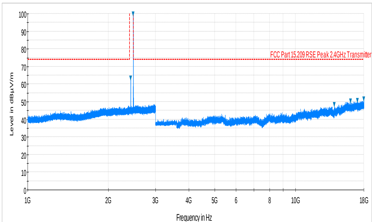
Plot 6-47. Radiated Spurious Plot above 1GHz (Bluetooth – Ch. 78, Ant. Pol. V)
