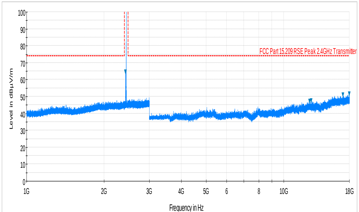
Plot 6-45. Radiated Spurious Plot above 1GHz (Bluetooth – Ch. 39, Ant. Pol. V)
