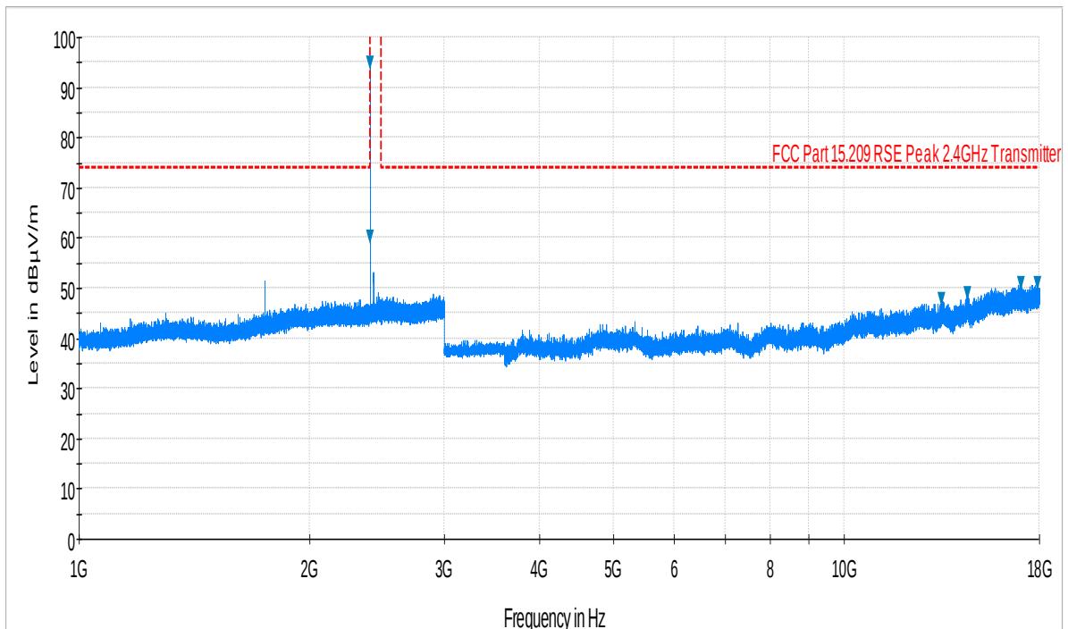
Plot 6-42. Radiated Spurious Plot above 1GHz (Bluetooth – Ch. 0, Ant. Pol. H)
