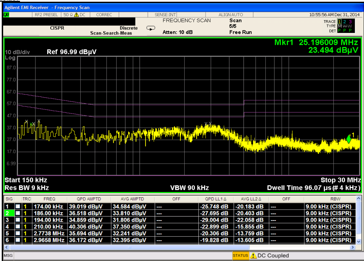
Plot 6-53. Line-Conducted Test Plot (N)
