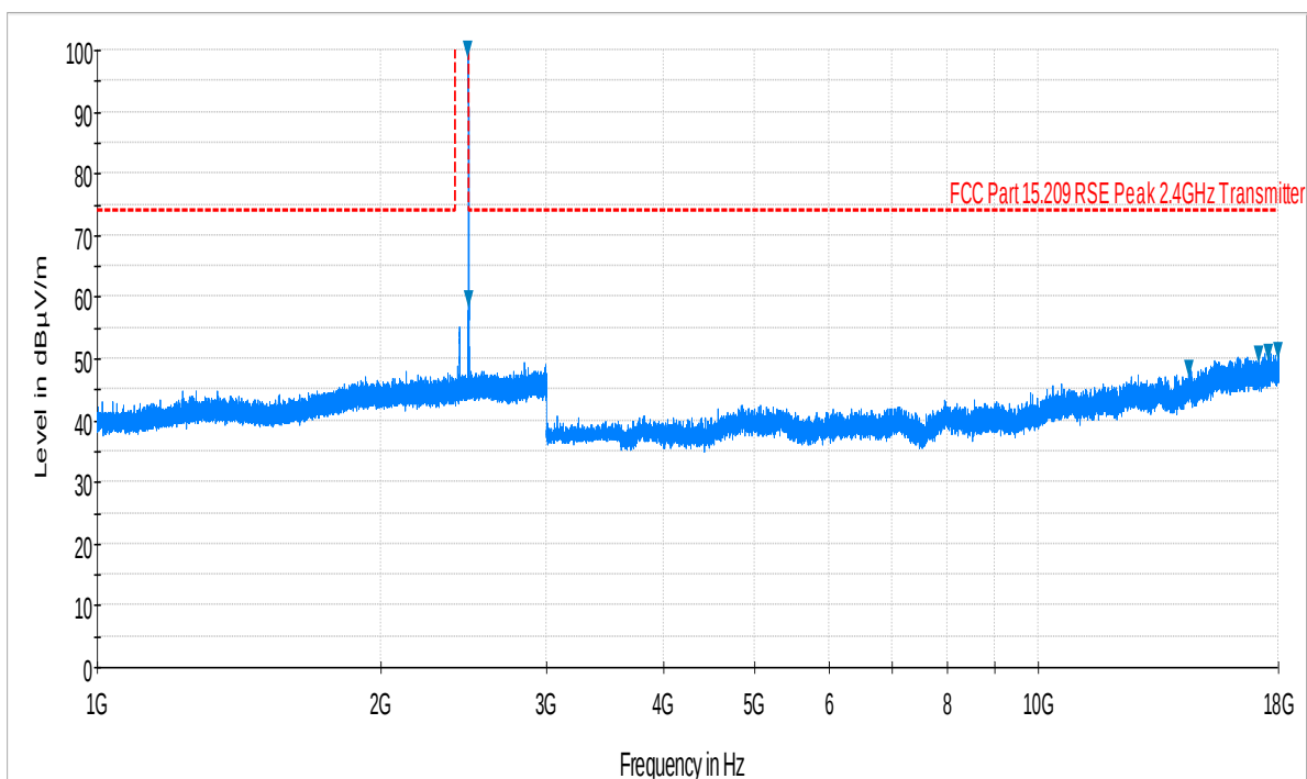
Plot 6-46. Radiated Spurious Plot above 1GHz (Bluetooth – Ch. 78, Ant. Pol. H)
