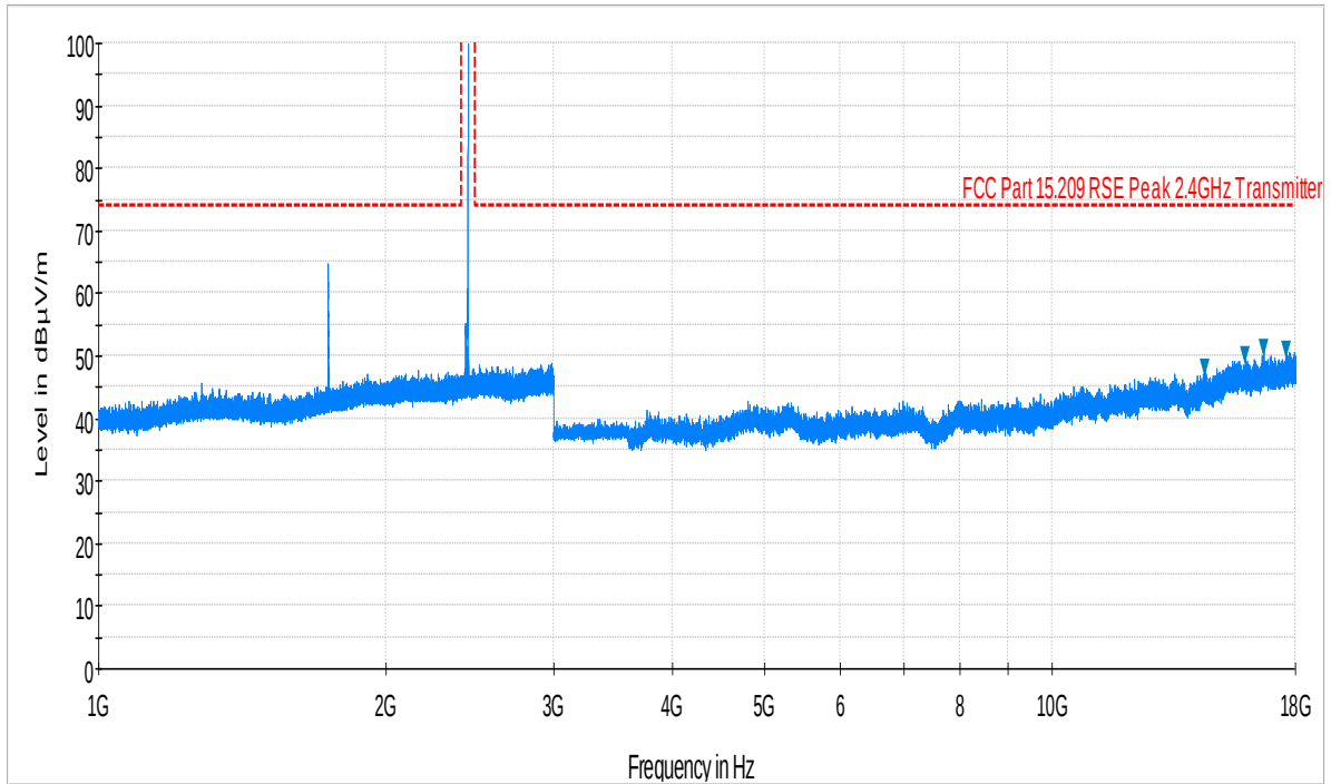
Plot 6-44. Radiated Spurious Plot above 1GHz (Bluetooth – Ch. 39, Ant. Pol. H)
