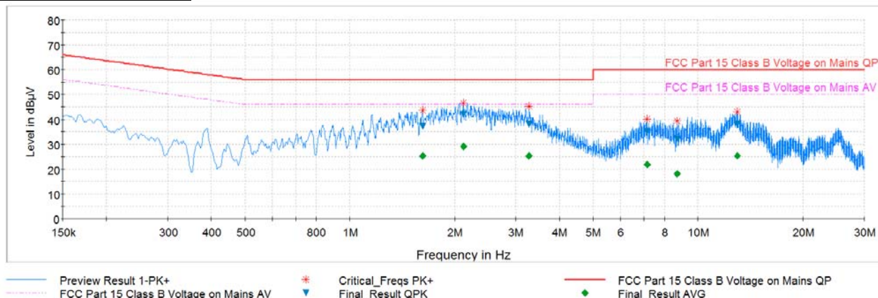
Plot 6-21. Line Conducted Plot with Bluetooth LE (N)
