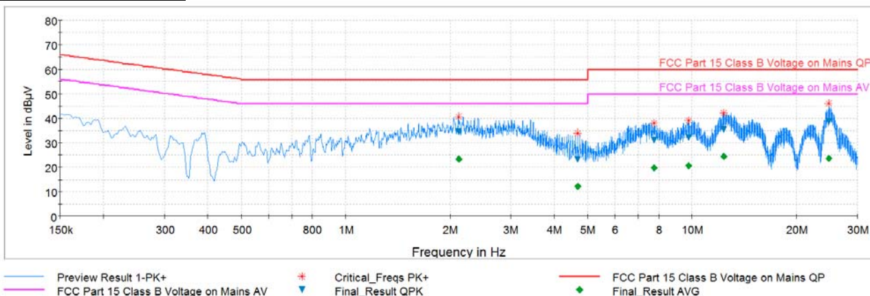
Plot 6-20. Line Conducted Plot with Bluetooth LE (L1)
