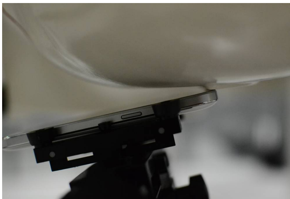
SAR Test Setup Photo 4: Left Tilt
