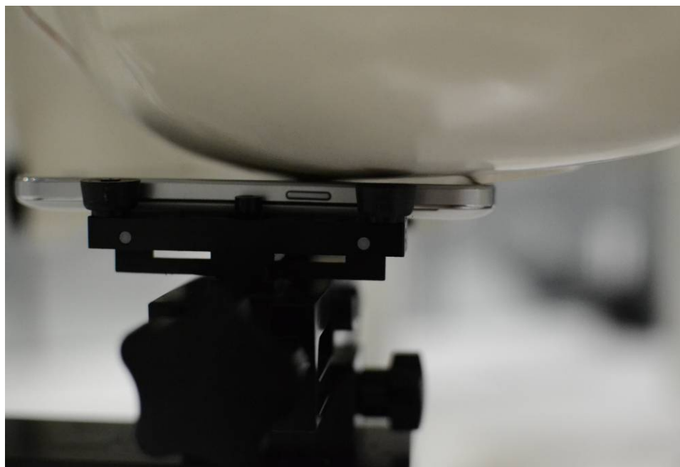
SAR Test Setup Photo 3: Left Cheek
