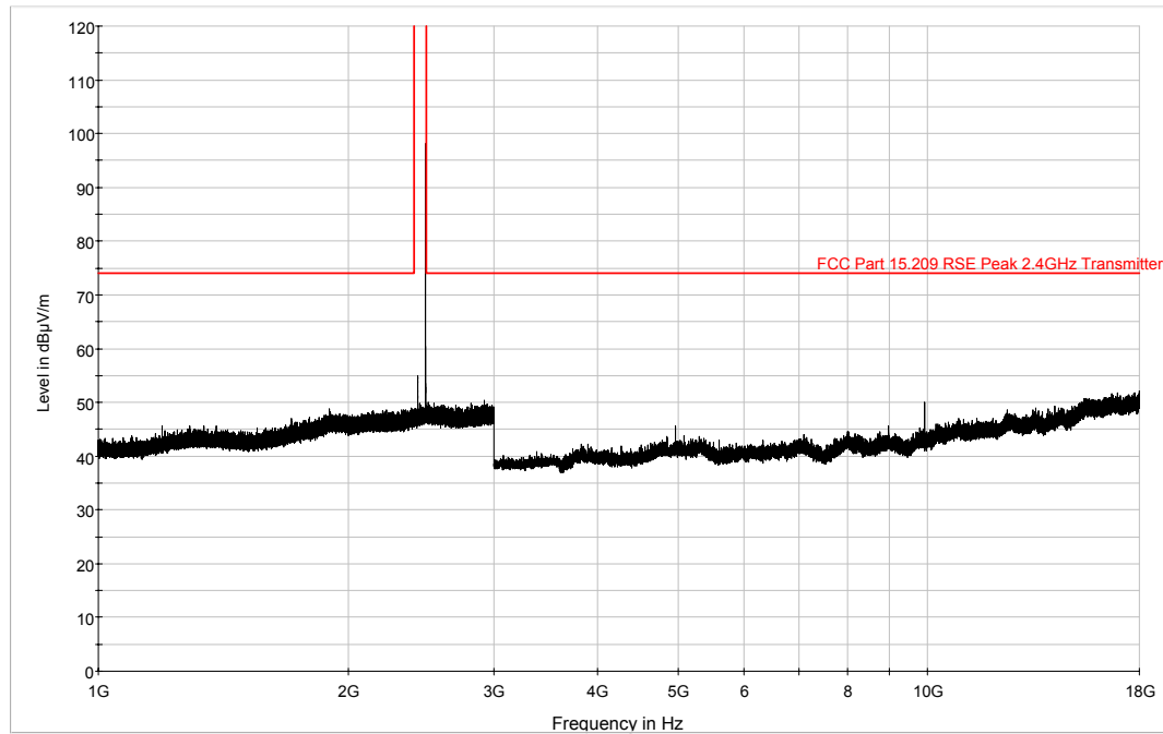
Plot 6-46. 1GHz – 18GHz Horizontal Pre-Scan Plot (Bluetooth, 1Mbps – Ch. 78)
