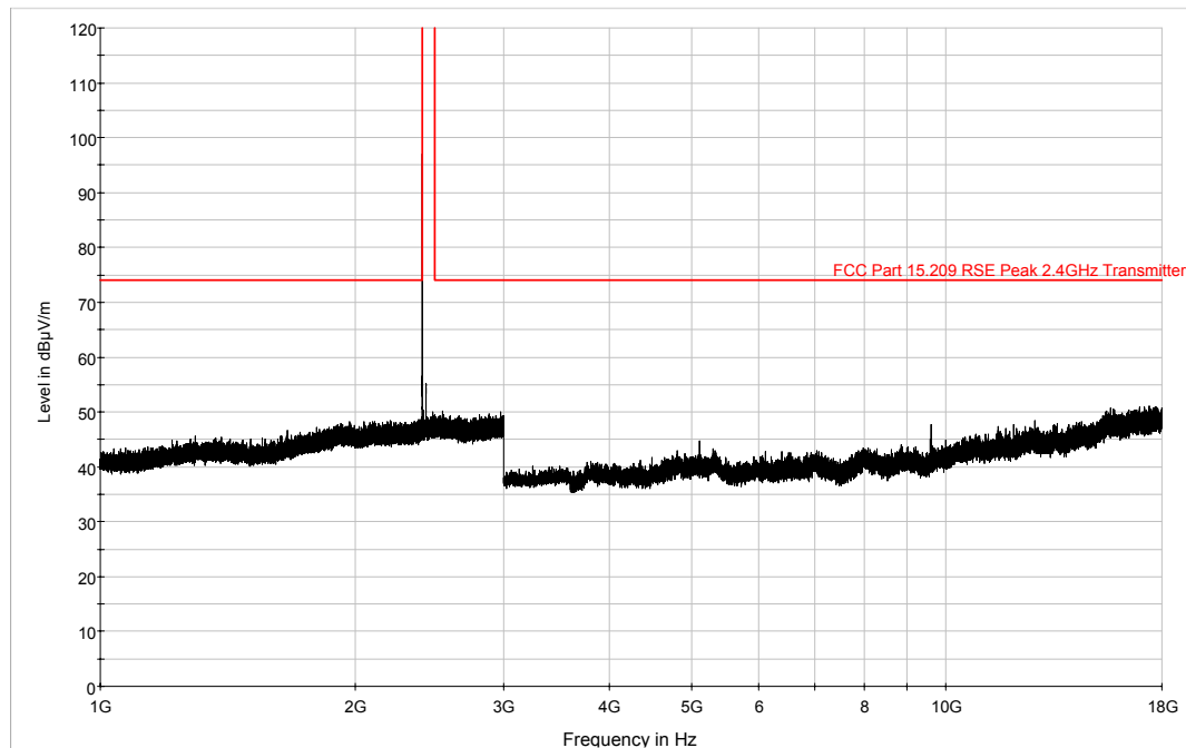
Plot 6-43. 1GHz – 18GHz Vertical Pre-Scan Plot (Bluetooth, 1Mbps – Ch. 0)
