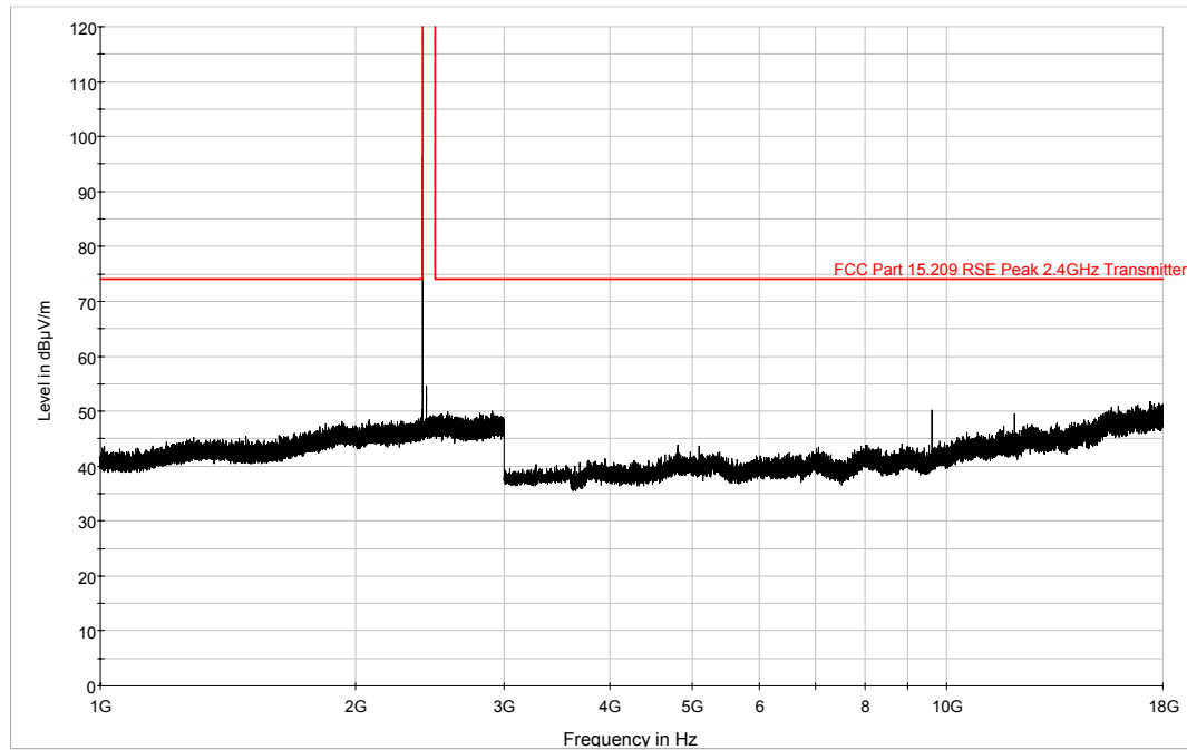
Plot 6-42. 1GHz – 18GHz Horizontal Pre-Scan Plot (Bluetooth, 1Mbps – Ch. 0)
