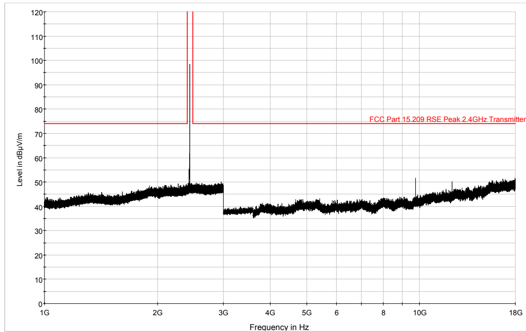
Plot 6-44. 1GHz – 18GHz Horizontal Pre-Scan Plot (Bluetooth, 1Mbps – Ch. 39)
