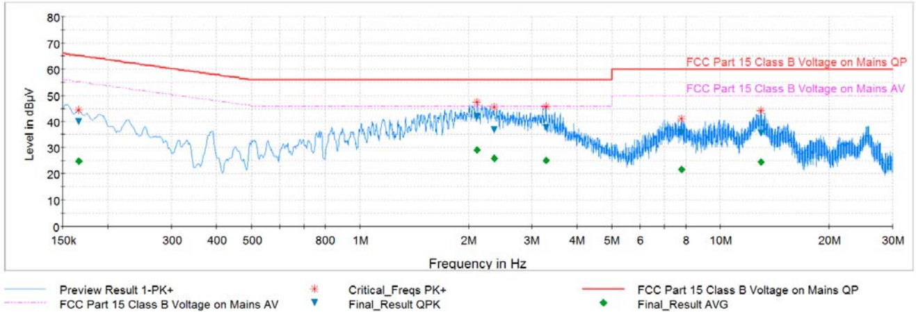
Plot 6-53. Line-Conducted Test Plot (N)
