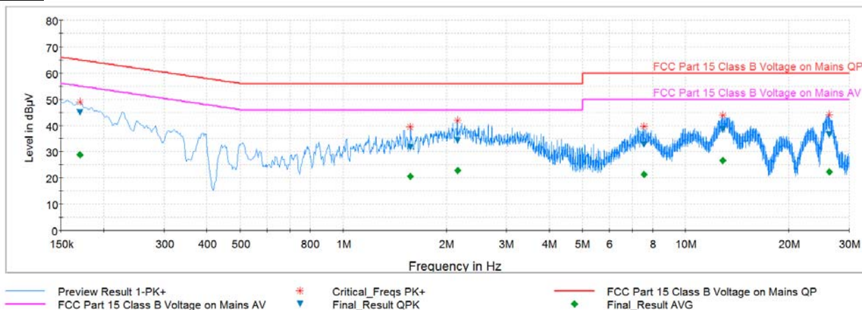
Plot 6-52. Line-Conducted Test Plot (L1)
