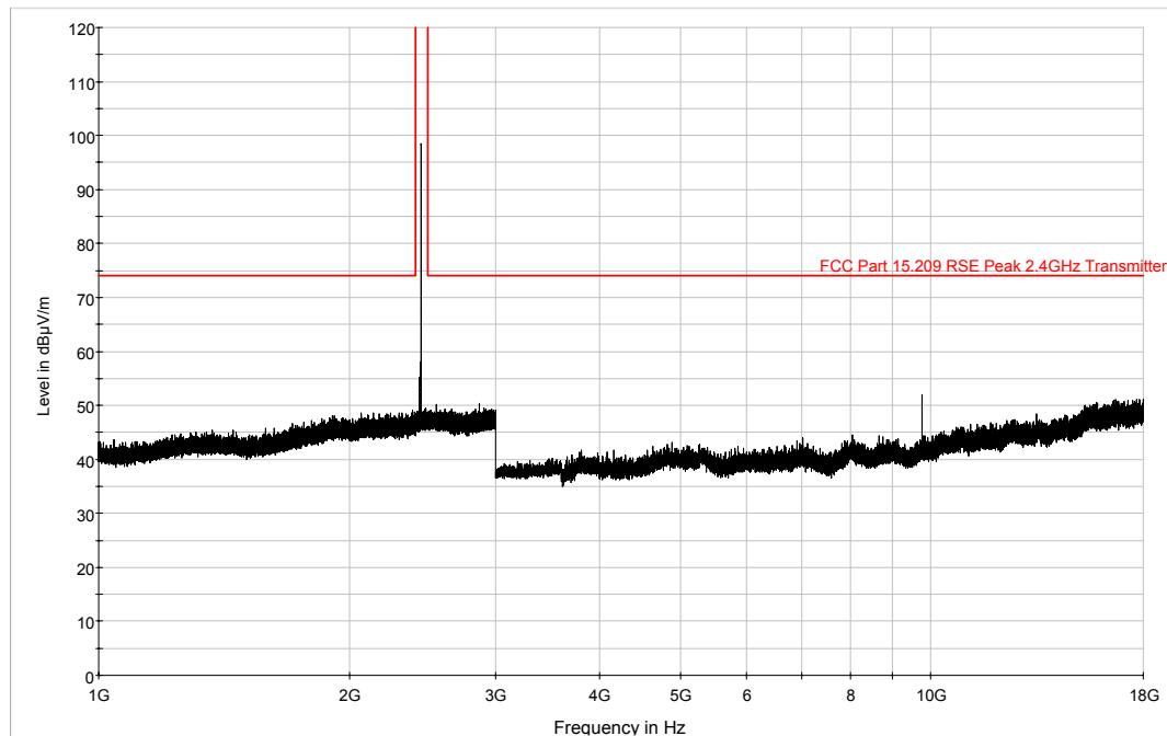
Plot 6-45. 1GHz – 18GHz Vertical Pre-Scan Plot (Bluetooth, 1Mbps – Ch. 39)
