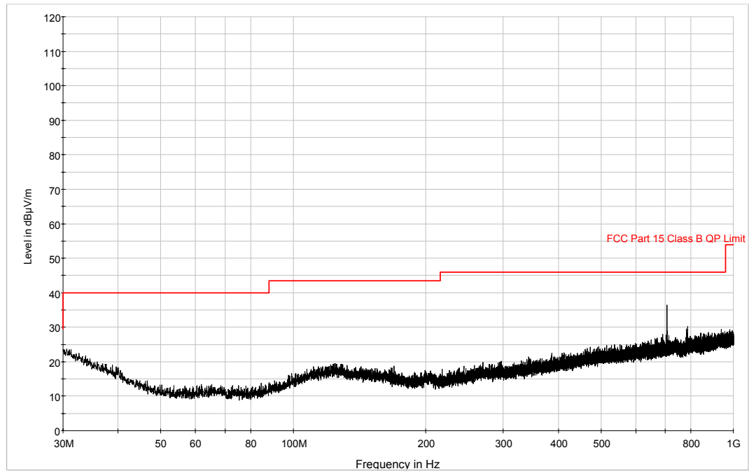
Plot 6-48. 30MHz – 1GHz Horizontal Pre-Scan Plot (Bluetooth, 1Mbps – Ch. 39)
