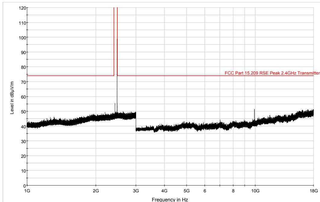
Plot 6-47. 1GHz – 18GHz Vertical Pre-Scan Plot (Bluetooth, 1Mbps – Ch. 78)
