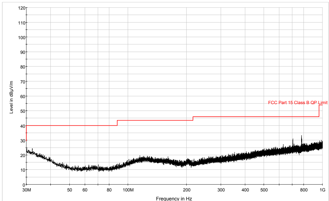
Plot 6-49. 30MHz – 1GHz Vertical Pre-Scan Plot (Bluetooth, 1Mbps – Ch. 39)
