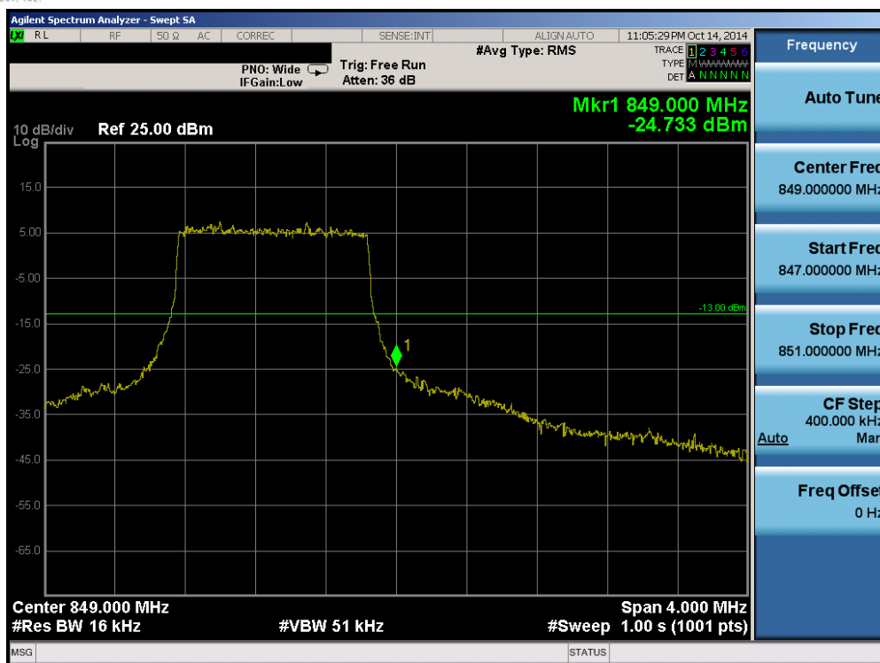
Plot 6-52. Upper Band Edge Plot (Band 26 – 1.4MHz QPSK – RB Size 6)
