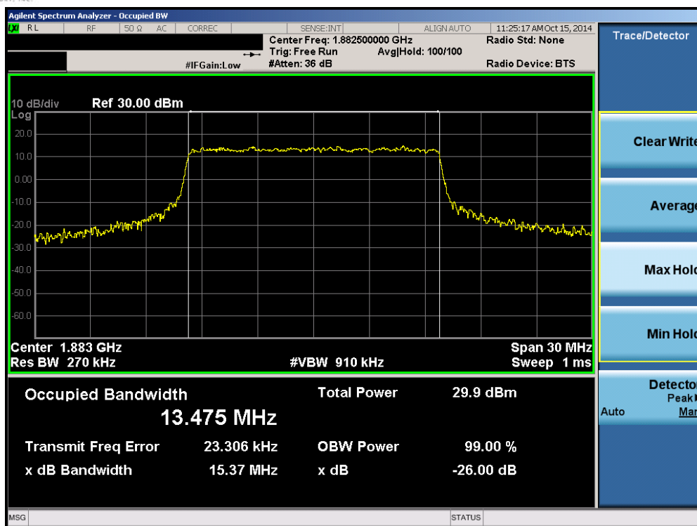
Plot 6-17. Occupied Bandwidth Plot (Band 25 – 15.0MHz QPSK – RB Size 75)
