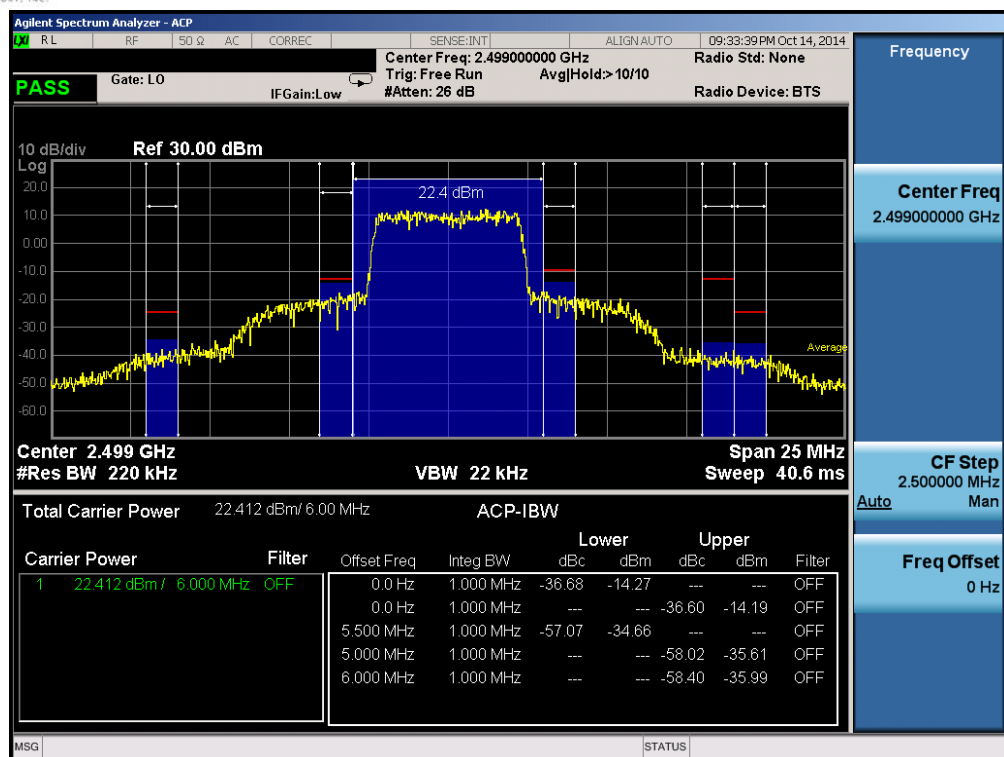
Plot 6-90. Lower ACP Plot (Band 41 – 5.0MHz QPSK – RB Size 25)
