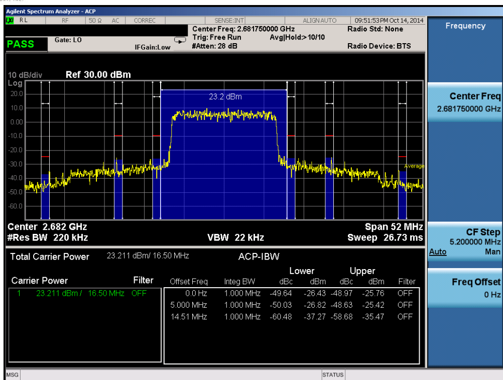
Plot 6-98. Upper ACP Plot (Band 41 – 15.0MHz QPSK – RB Size 75)
