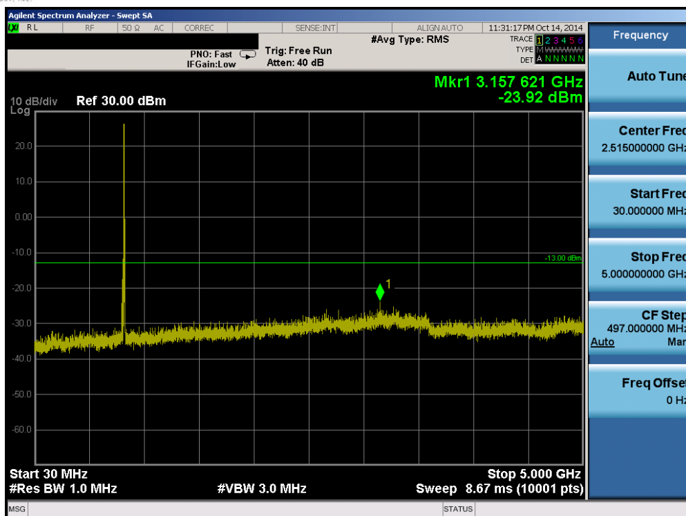
Plot 6-33. Conducted Spurious Plot (Band 26 – 10.0MHz QPSK – RB Size 1, RB Offset 0 – High Channel)
