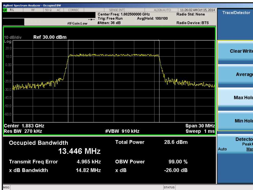
Plot 6-18. Occupied Bandwidth Plot (Band 25 – 15.0MHz 16-QAM – RB Size 75)
