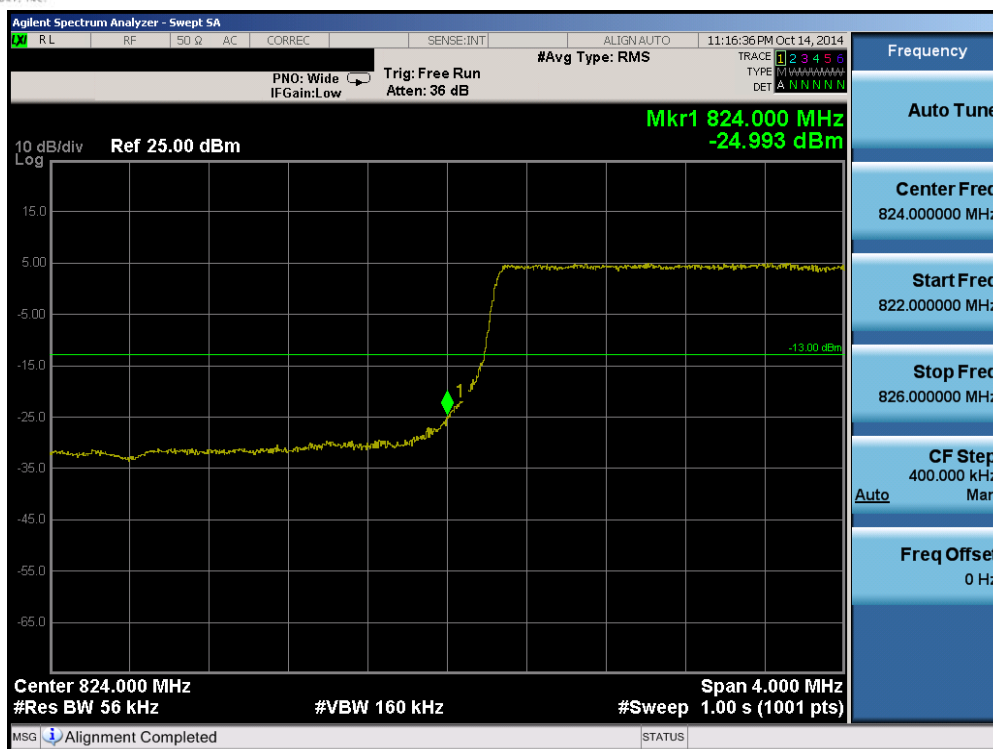
Plot 6-58. Lower Band Edge Plot (Band 26 – 5.0MHz QPSK – RB Size 25)
