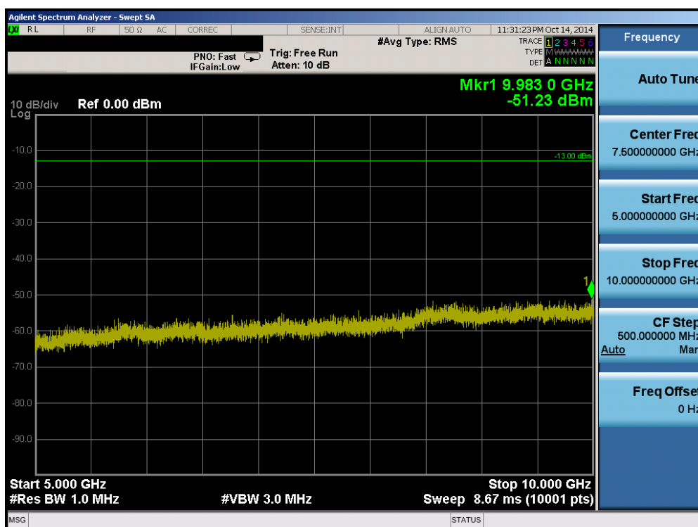
Plot 6-34. Conducted Spurious Plot (Band 26 – 10.0MHz QPSK – RB Size 1, RB Offset 0 – High Channel)
