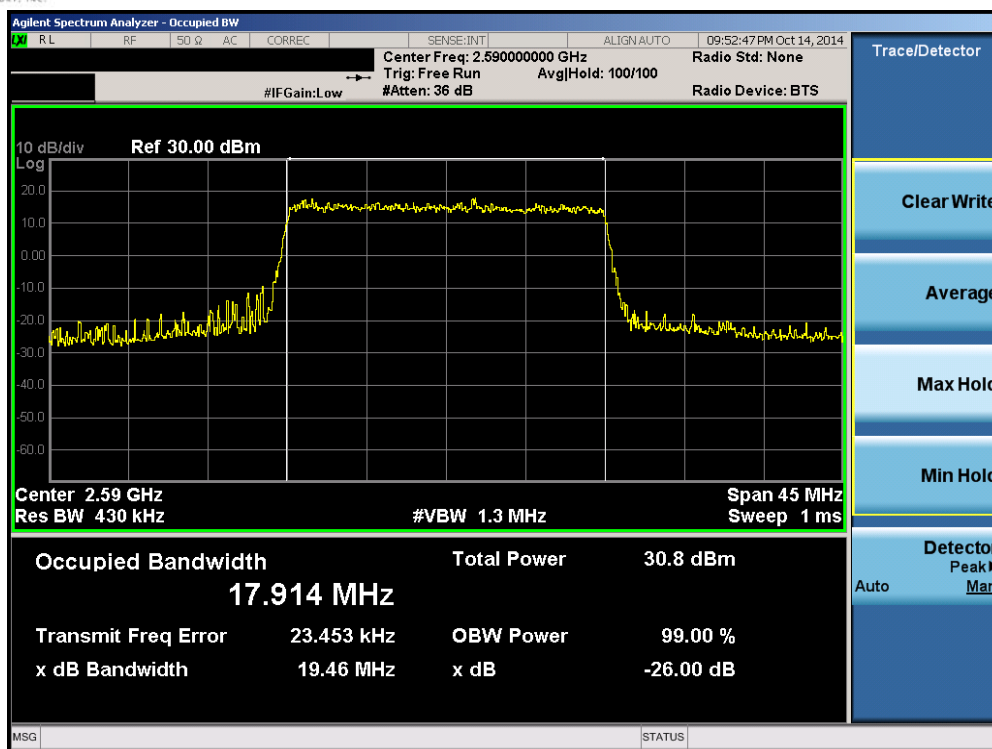
Plot 6-27. Occupied Bandwidth Plot (Band 41 – 20.0MHz QPSK – RB Size 100)
