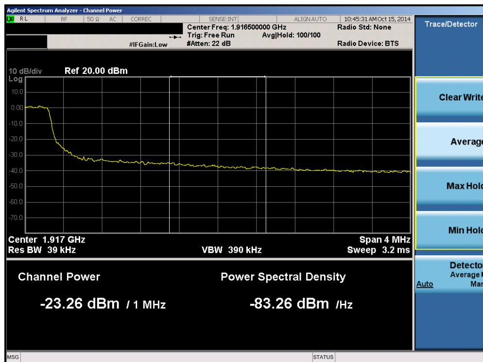
Plot 6-77. Upper Extended Band Edge Plot (Band 25 – 5.0MHz QPSK – RB Size 25)
