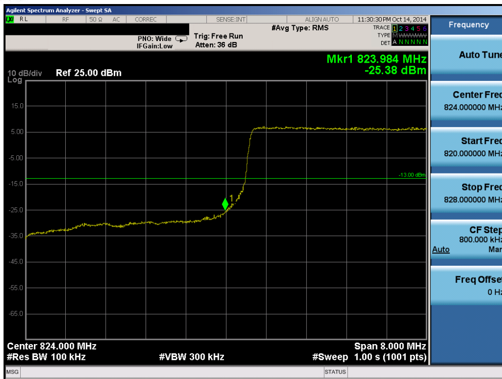
Plot 6-62. Lower Band Edge Plot (Band 26 – 10.0MHz QPSK – RB Size 50)
