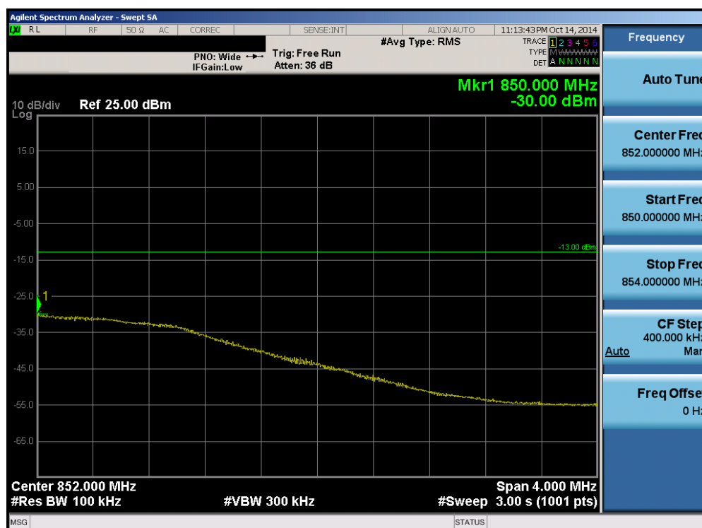
Plot 6-57. Upper Extended Band Edge Plot (Band 26 - Band 5 - 3.0MHz QPSK - RB Size 15)
