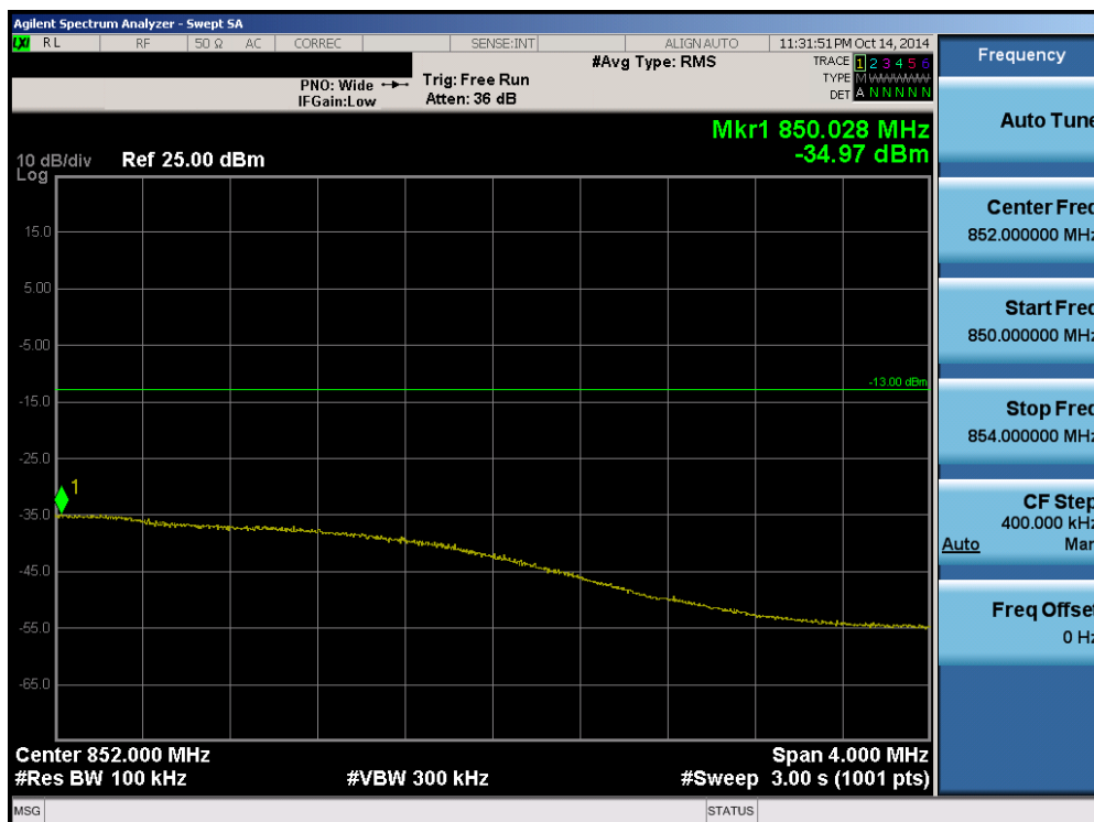
Plot 6-65. Upper Extended Band Edge Plot (Band 26 – 10.0MHz QPSK – RB Size 50)
