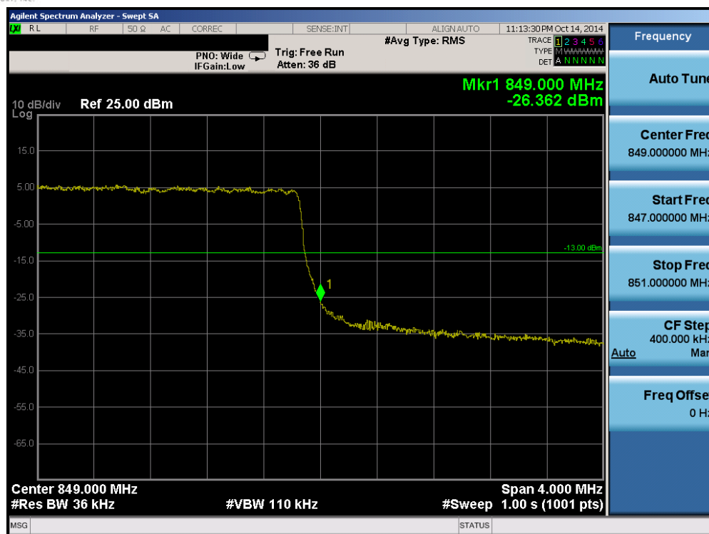
Plot 6-56. Upper Band Edge Plot (Band 26 - 3.0MHz QPSK - RB Size 15)
