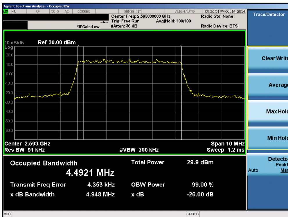
Plot 6-22. Occupied Bandwidth Plot (Band 41 – 5.0MHz 16-QAM – RB Size 25)
