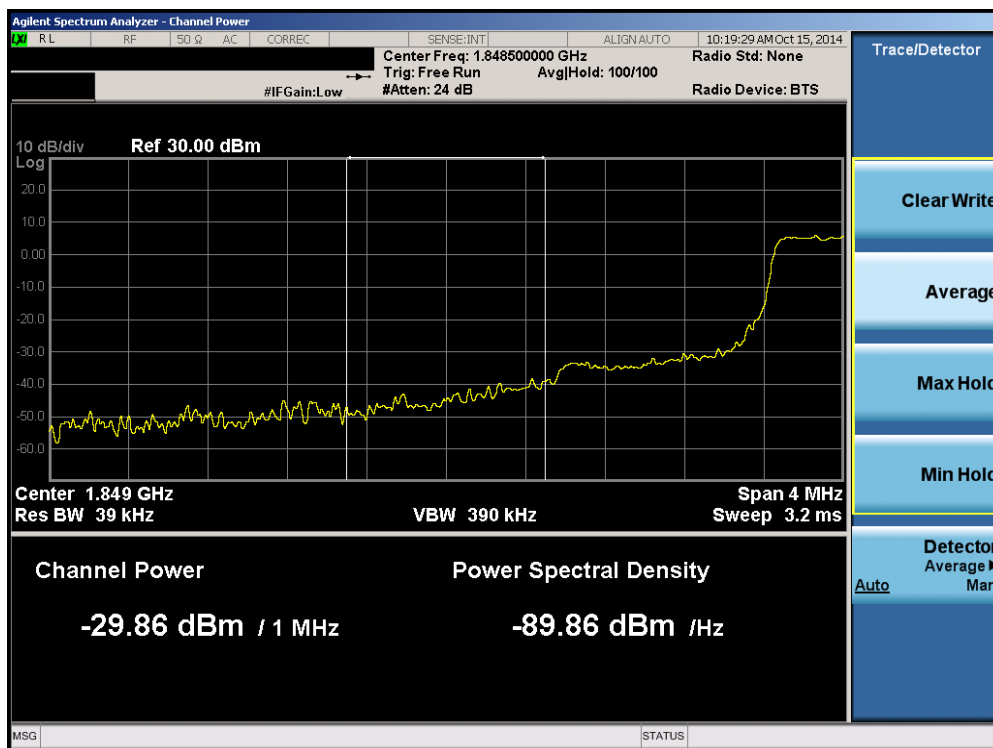
Plot 6-67. Lower Extended Band Edge Plot (Band 25 – 1.4MHz QPSK – RB Size 6)
