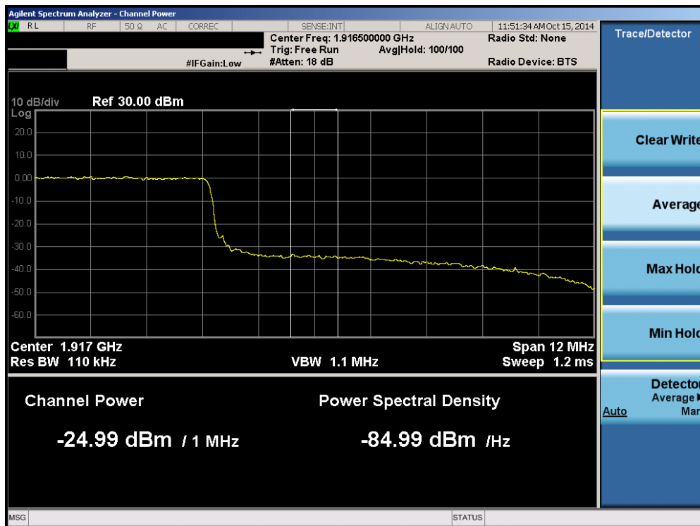
Plot 6-85. Upper Extended Band Edge Plot (Band 25 - 15.0MHz QPSK - RB Size 75)
