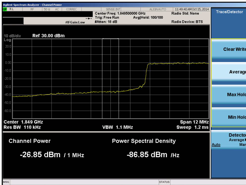
Plot 6-83. Lower Extended Band Edge Plot (Band 25 – 15.0MHz QPSK – RB Size 75)
