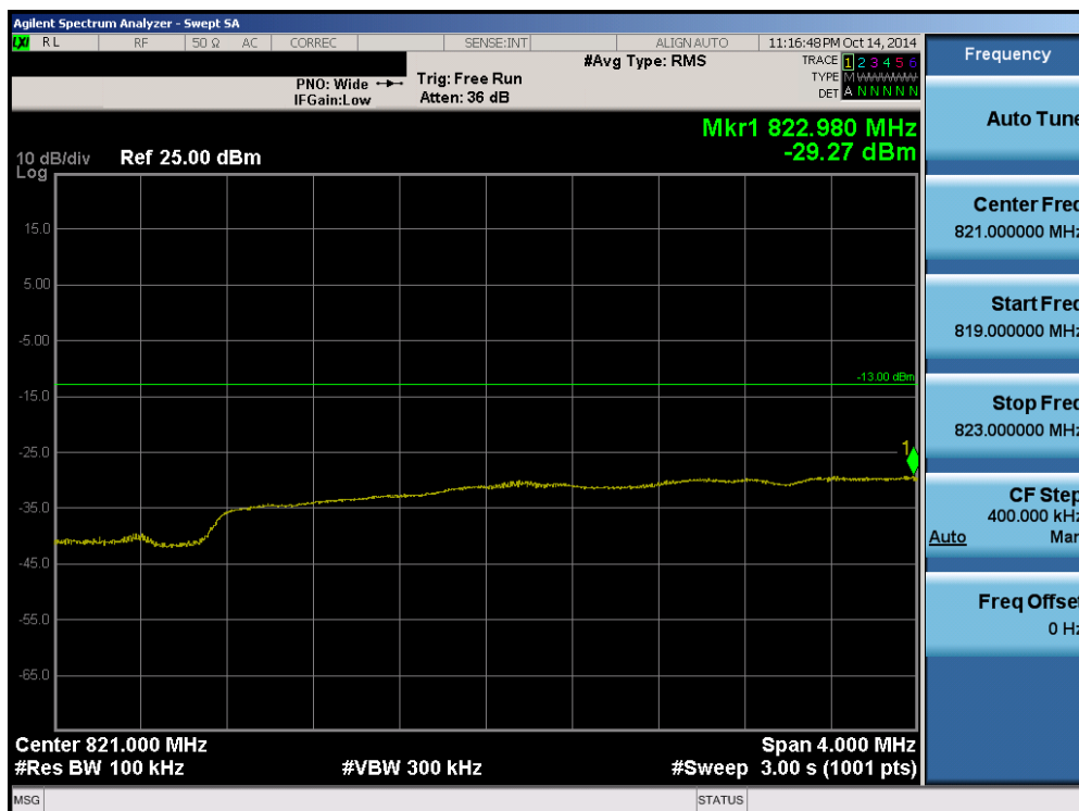
Plot 6-59. Lower Extended Band Edge Plot (Band 26 – 5.0MHz QPSK – RB Size 25)
