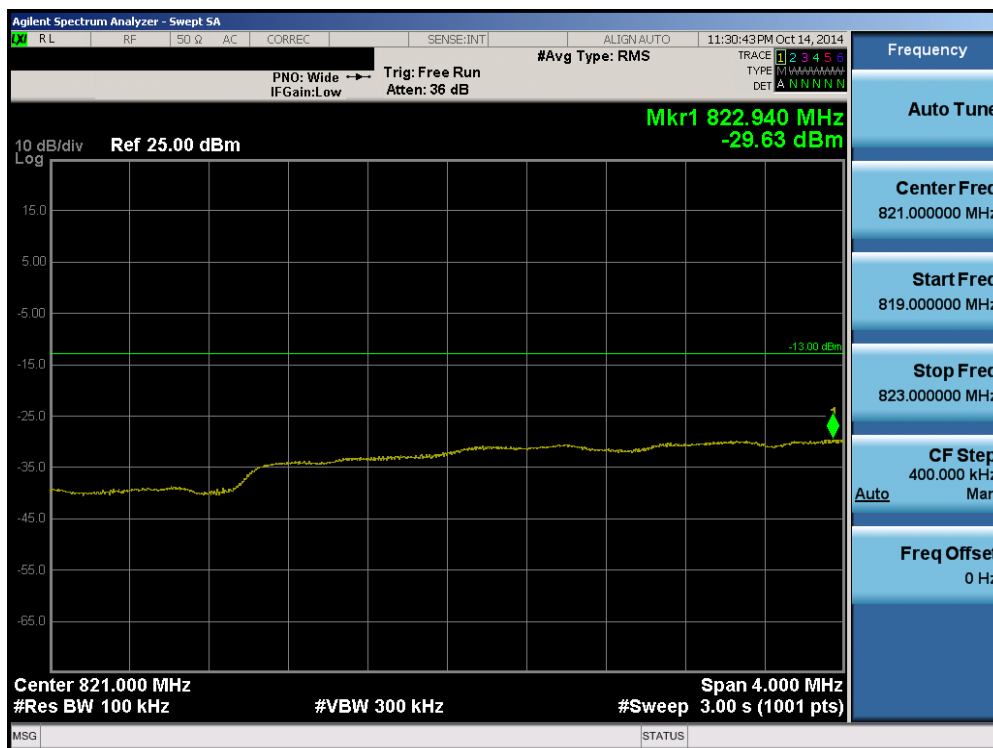
Plot 6-63. Lower Extended Band Edge Plot (Band 26 – 10.0MHz QPSK – RB Size 50)
