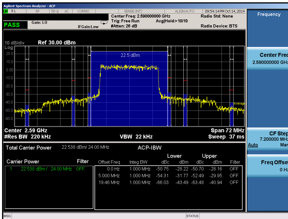
Plot 6-100. Mid ACP Plot (Band 41 – 20.0MHz QPSK – RB Size 100)
