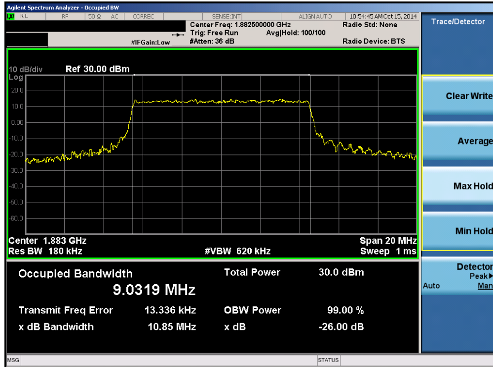
Plot 6-15. Occupied Bandwidth Plot (Band 25 – 10.0MHz QPSK – RB Size 50)
