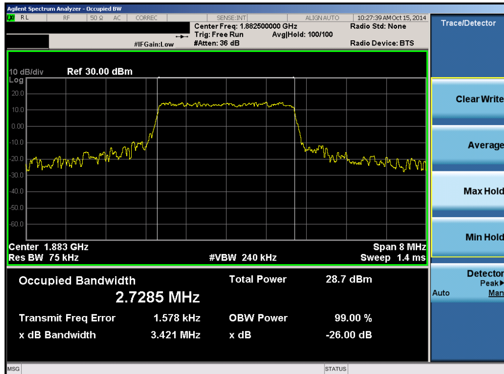
Plot 6-12. Occupied Bandwidth Plot (Band 25 – 3.0MHz 16-QAM – RB Size 15)
