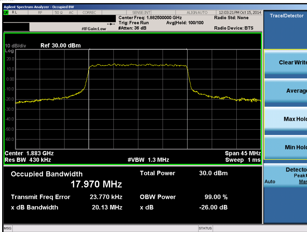
Plot 6-19. Occupied Bandwidth Plot (Band 25 – 20.0MHz QPSK – RB Size 100)
