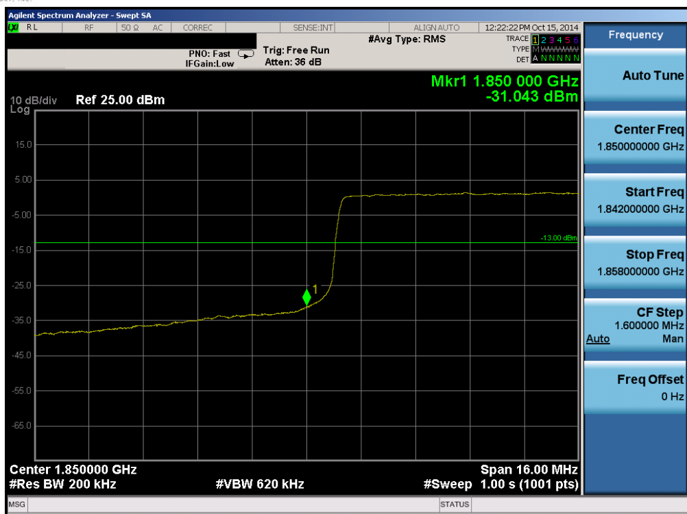
Plot 6-86. Lower Band Edge Plot (Band 25 – 20.0MHz QPSK – RB Size 100)
