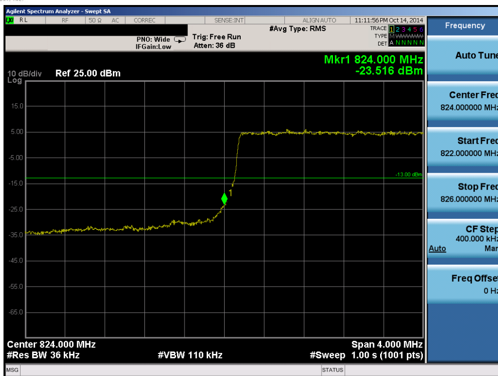
Plot 6-54. Lower Band Edge Plot (Band 26 – 3.0MHz QPSK – RB Size 15)
