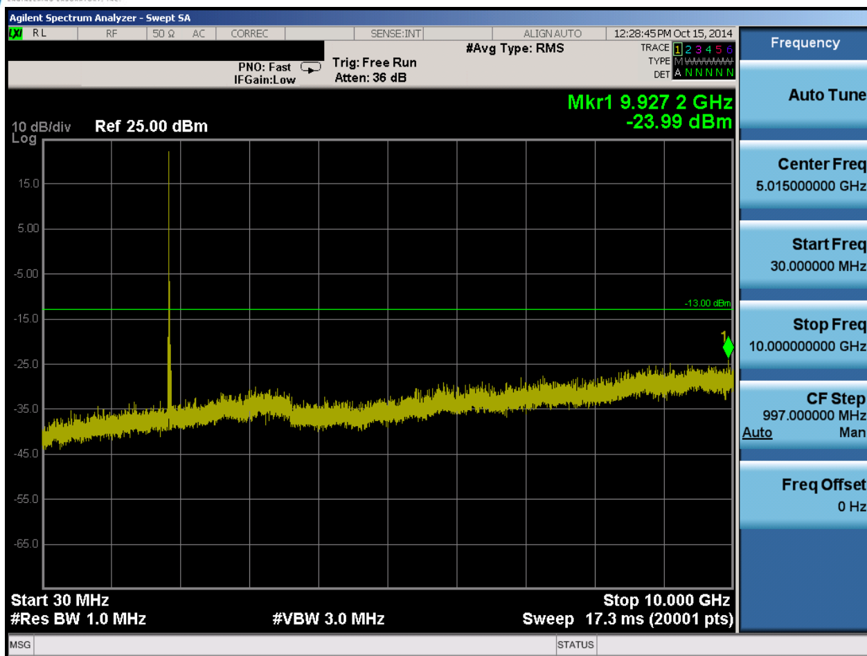
Plot 6-35. Conducted Spurious Plot (Band 25 – 10.0MHz QPSK – RB Size 1, RB Offset 0– Low Channel)
