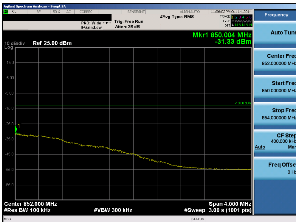
Plot 6-53. Upper Extended Band Edge Plot (Band 26 – 1.4MHz QPSK – RB Size 6)
