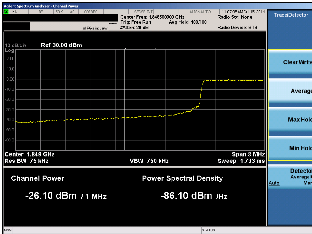
Plot 6-79. Lower Extended Band Edge Plot (Band 25 – 10.0MHz QPSK – RB Size 50)
