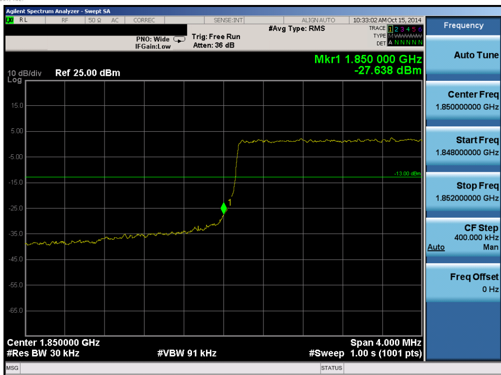
Plot 6-70. Lower Band Edge Plot (Band 25 – 3.0MHz QPSK – RB Size 15)
