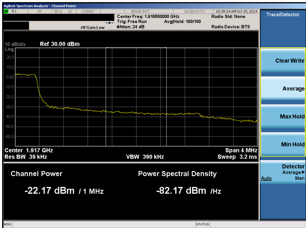
Plot 6-73. Upper Extended Band Edge Plot (Band 25 – 3.0MHz QPSK – RB Size 15)
