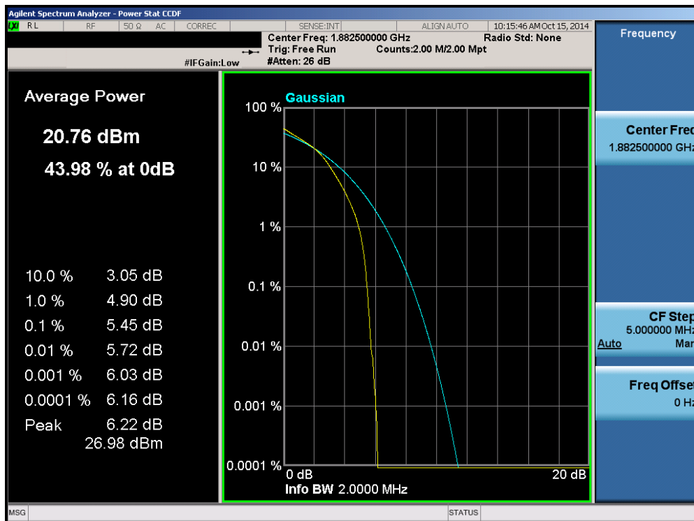
Plot 6-103. PAR Plot (Band 25 – 1.4MHz 16-QAM – RB Size 6)
