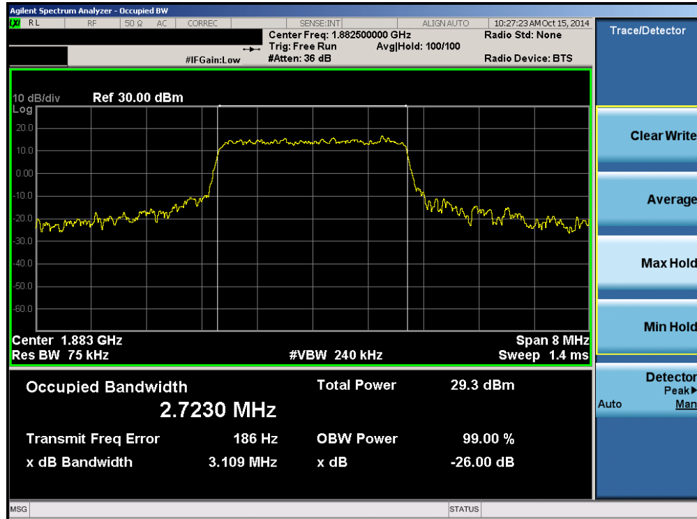
Plot 6-11. Occupied Bandwidth Plot (Band 25 – 3.0MHz QPSK – RB Size 15)
