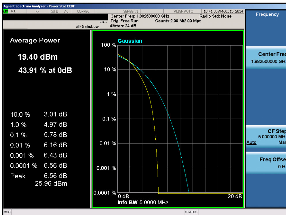
Plot 6-107. PAR Plot (Band 25 – 5.0MHz 16-QAM – RB Size 25)
