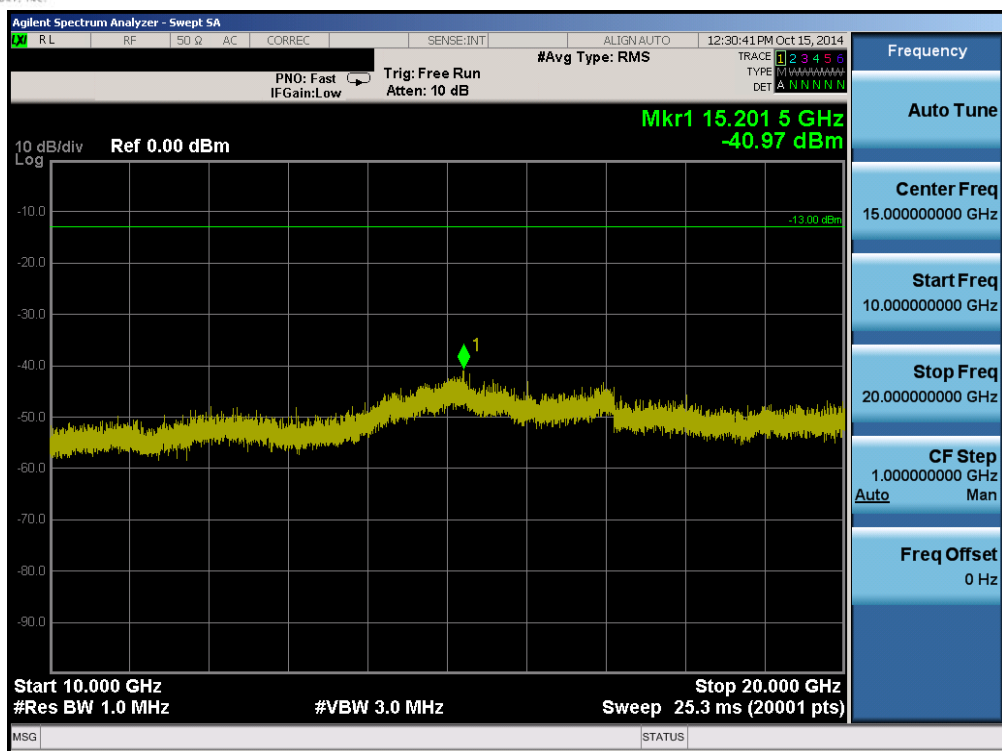
Plot 6-40. Conducted Spurious Plot (Band 25 – 10.0MHz QPSK – RB Size 1, RB Offset 0 – High Channel)
