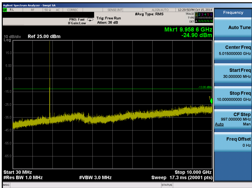
Plot 6-37. Conducted Spurious Plot (Band 25 – 10.0MHz QPSK – RB Size 1, RB Offset 0 – Mid Channel)
