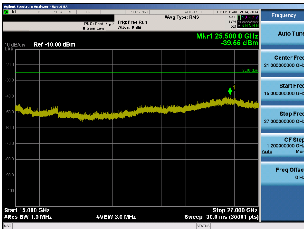
Plot 6-49. Conducted Spurious Plot (Band 41 – 20.0MHz QPSK – RB Size 1, RB Offset 0 – High Channel)
