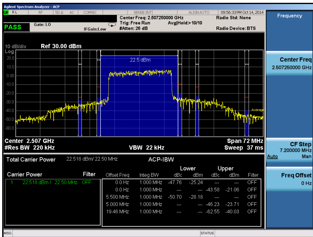
Plot 6-99. Lower ACP Plot (Band 41 – 20.0MHz QPSK – RB Size 100)
