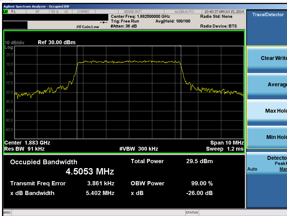
Plot 6-13. Occupied Bandwidth Plot (Band 25 – 5.0MHz QPSK – RB Size 25)
