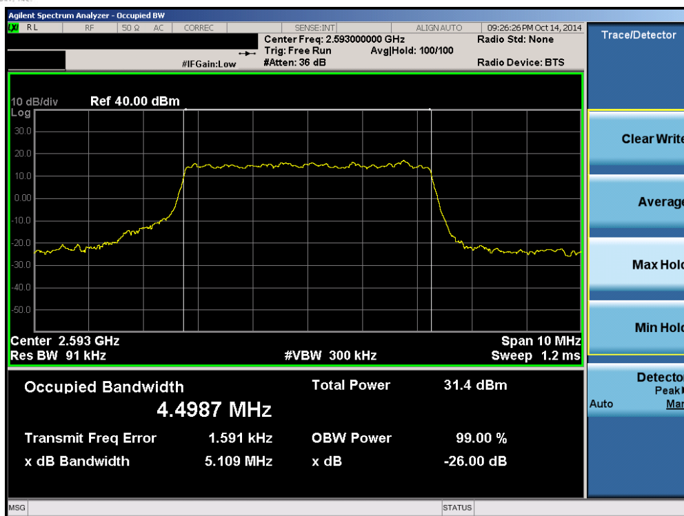
Plot 6-21. Occupied Bandwidth Plot (Band 41 – 5.0MHz QPSK – RB Size 25)
