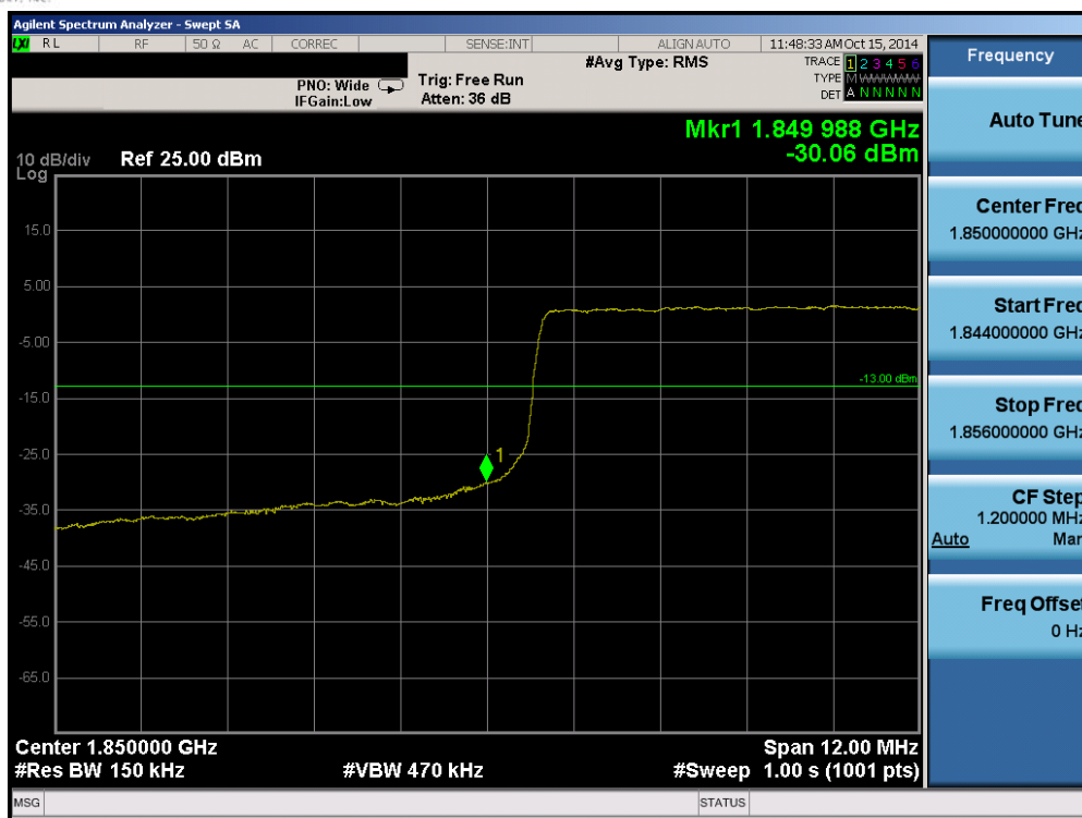
Plot 6-82. Lower Band Edge Plot (Band 25 – 15.0MHz QPSK – RB Size 75)
