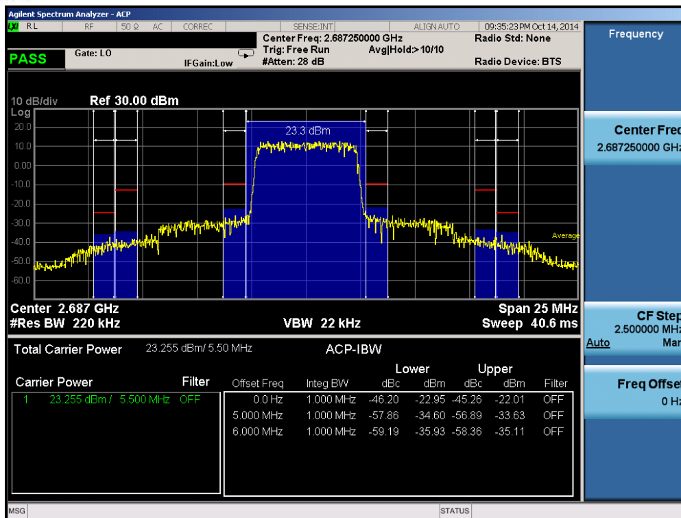
Plot 6-92. Upper ACP Plot (Band 41 – 5.0MHz QPSK – RB Size 25)
