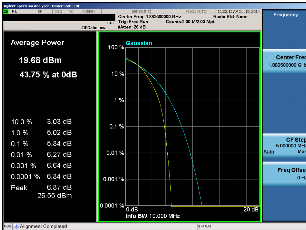
Plot 6-109. PAR Plot (Band 25 – 10.0MHz 16-QAM – RB Size 50)
