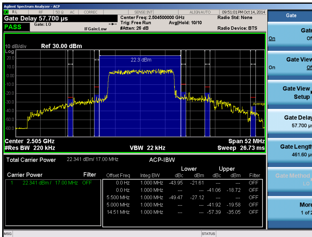
Plot 6-96. Lower ACP Plot (Band 41 – 15.0MHz QPSK – RB Size 75)
