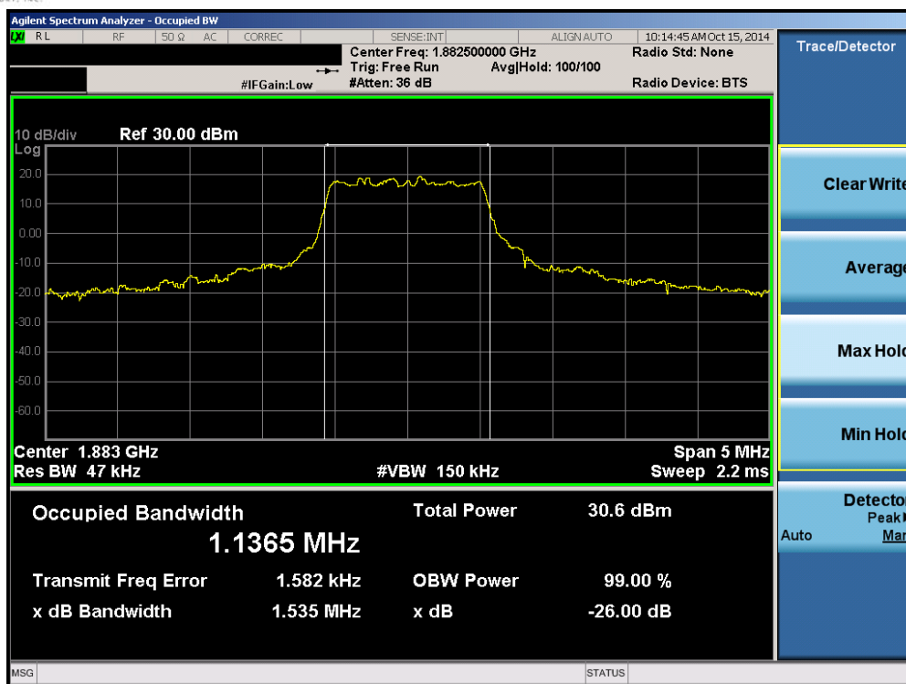
Plot 6-9. Occupied Bandwidth Plot (Band 25 – 1.4MHz QPSK – RB Size 6)
