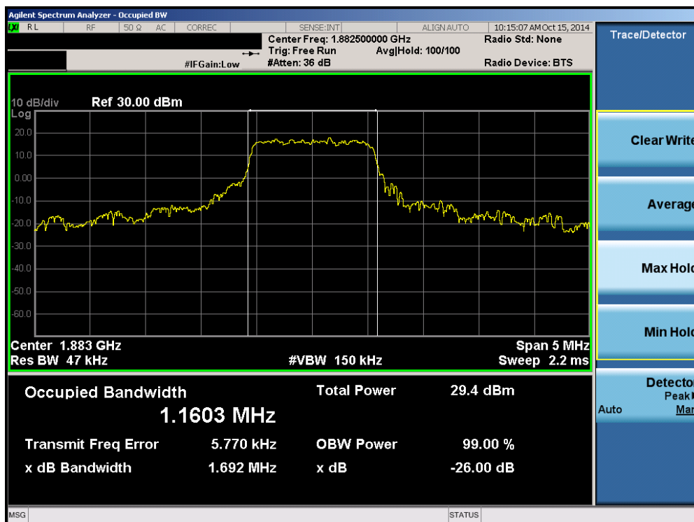
Plot 6-10. Occupied Bandwidth Plot (Band 25 – 1.4MHz 16-QAM – RB Size 6)
