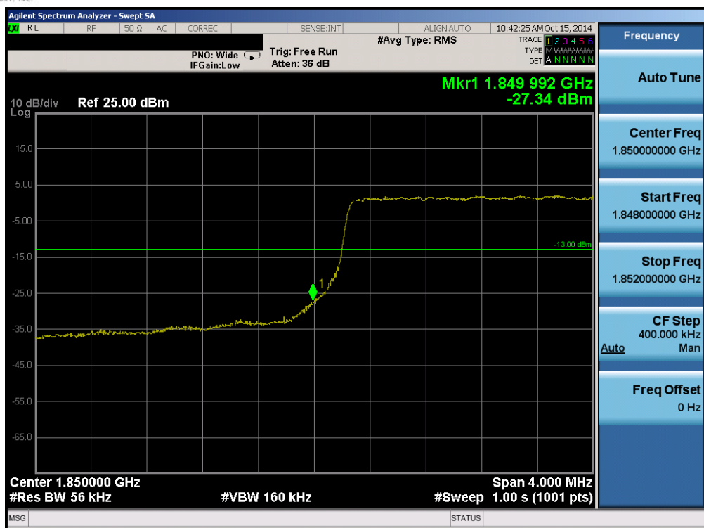
Plot 6-74. Lower Band Edge Plot (Band 25 – 5.0MHz QPSK – RB Size 25)
