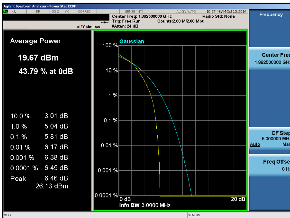
Plot 6-105. PAR Plot (Band 25 – 3.0MHz 16-QAM – RB Size 15)
