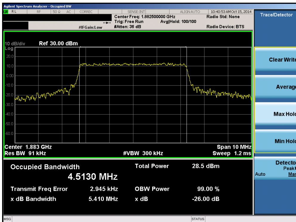
Plot 6-14. Occupied Bandwidth Plot (Band 25 – 5.0MHz 16-QAM – RB Size 25)
