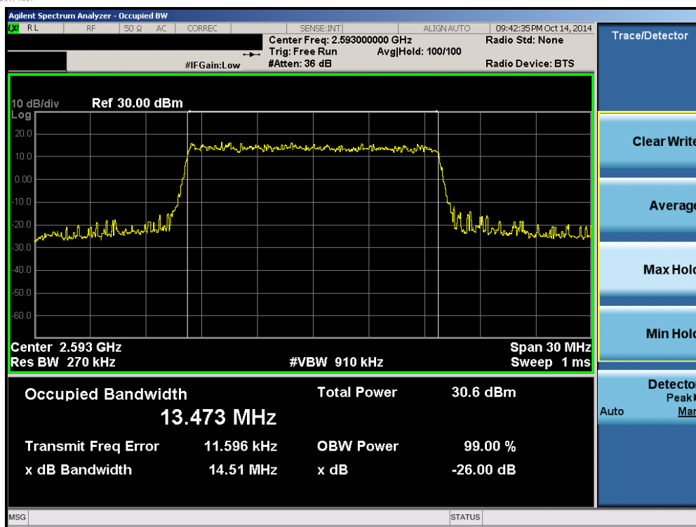
Plot 6-25. Occupied Bandwidth Plot (Band 41 – 15.0MHz QPSK – RB Size 75)
