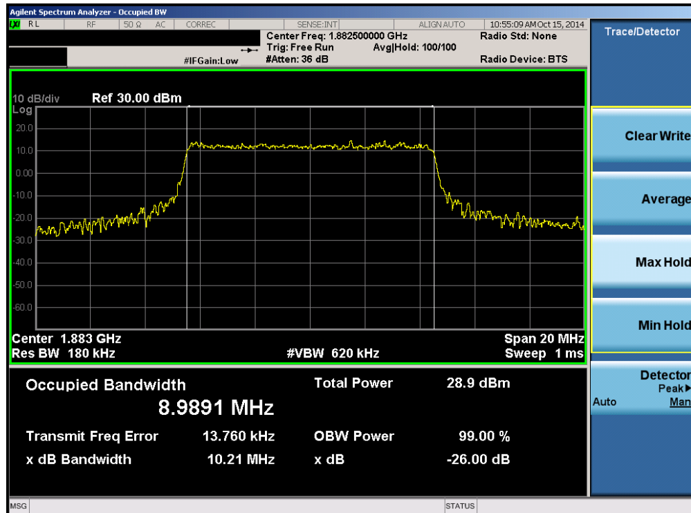
Plot 6-16. Occupied Bandwidth Plot (Band 25 – 10.0MHz 16-QAM – RB Size 50)
