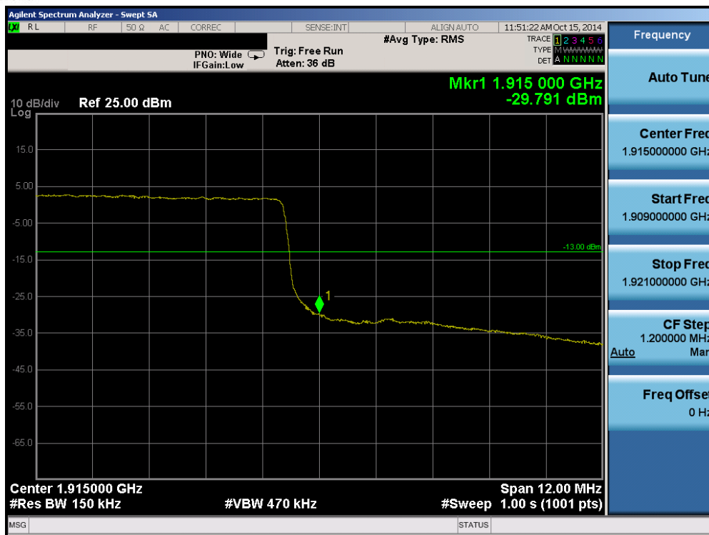
Plot 6-84. Upper Band Edge Plot (Band 25 - 15.0MHz QPSK - RB Size 75)
