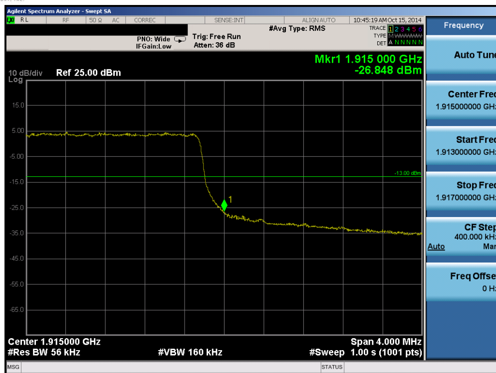
Plot 6-76. Upper Band Edge Plot (Band 25 – 5.0MHz QPSK – RB Size 25)
