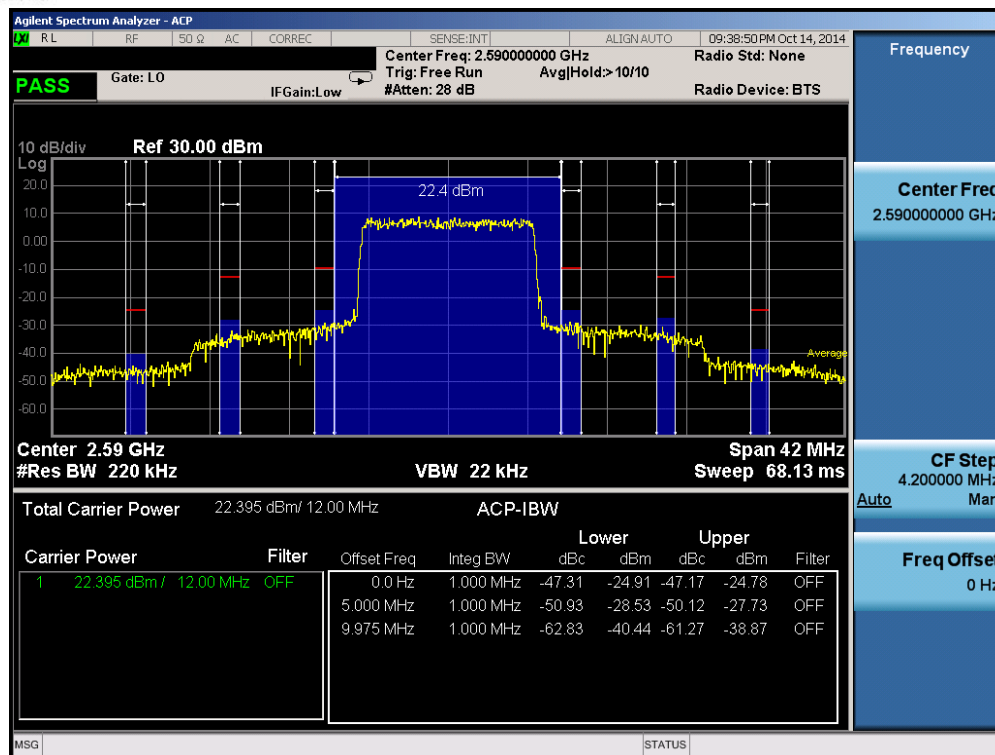
Plot 6-94. Mid ACP Plot (Band 41 – 10.0MHz QPSK – RB Size 50)
