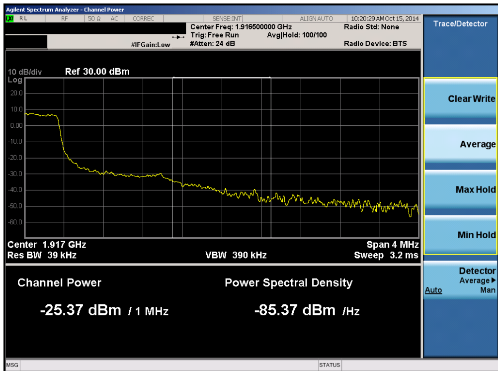
Plot 6-69. Upper Extended Band Edge Plot (Band 25 – 1.4MHz QPSK – RB Size 6)
