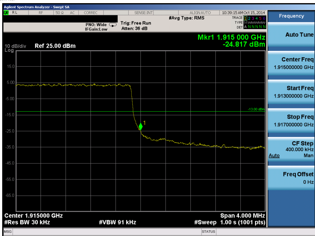
Plot 6-72. Upper Band Edge Plot (Band 25 – 3.0MHz QPSK – RB Size 15)
