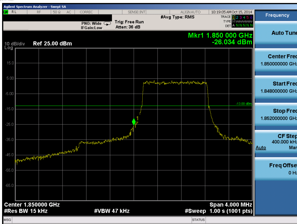
Plot 6-66. Lower Band Edge Plot (Band 25 – 1.4MHz QPSK – RB Size 6)
