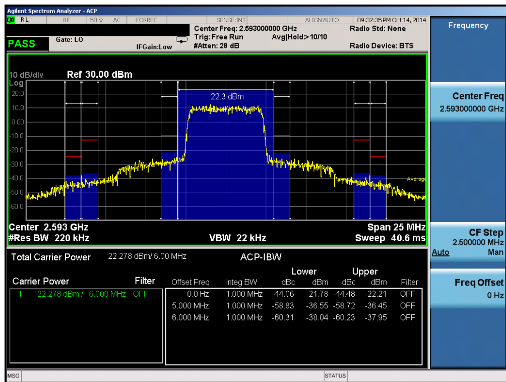
Plot 6-91. Mid ACP Plot (Band 41 – 5.0MHz QPSK – RB Size 25)
