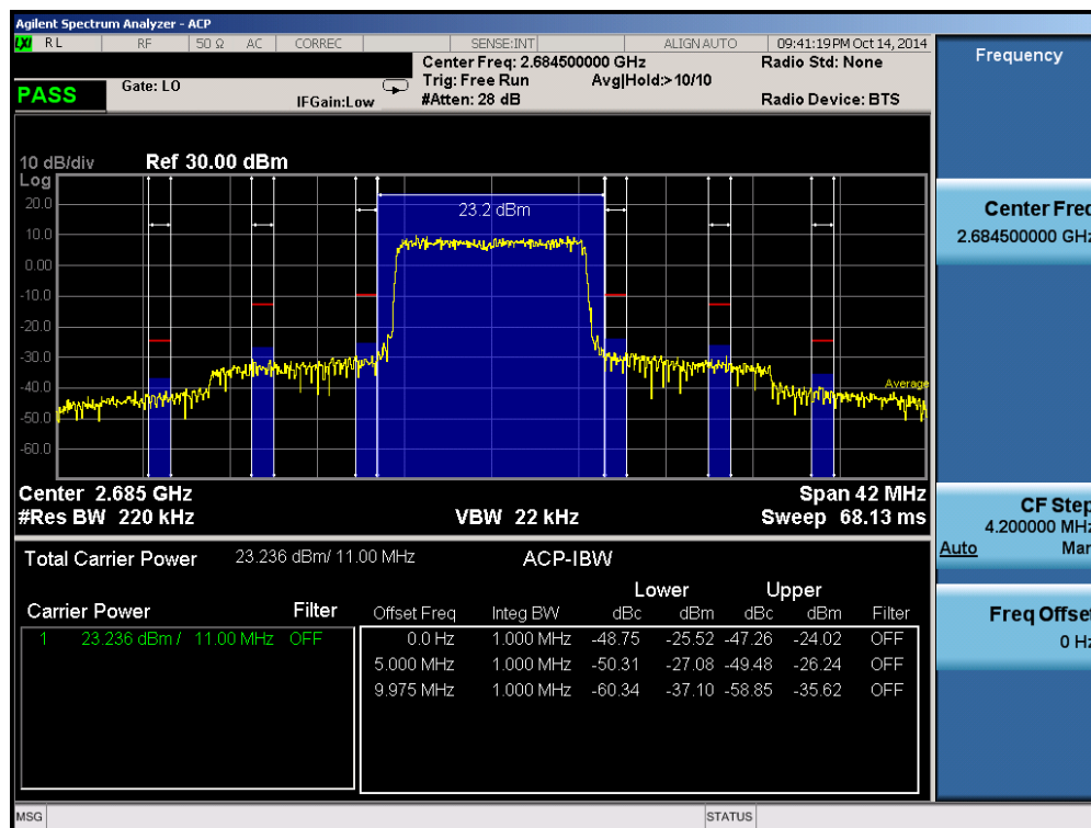
Plot 6-95. Upper ACP Plot (Band 41 – 10.0MHz QPSK – RB Size 50)
