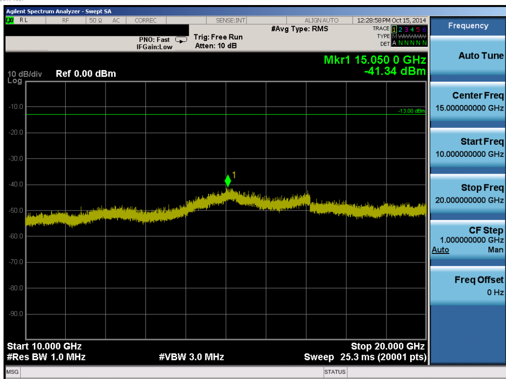
Plot 6-36. Conducted Spurious Plot (Band 25 – 10.0MHz QPSK – RB Size 1, RB Offset 0 – Low Channel)
