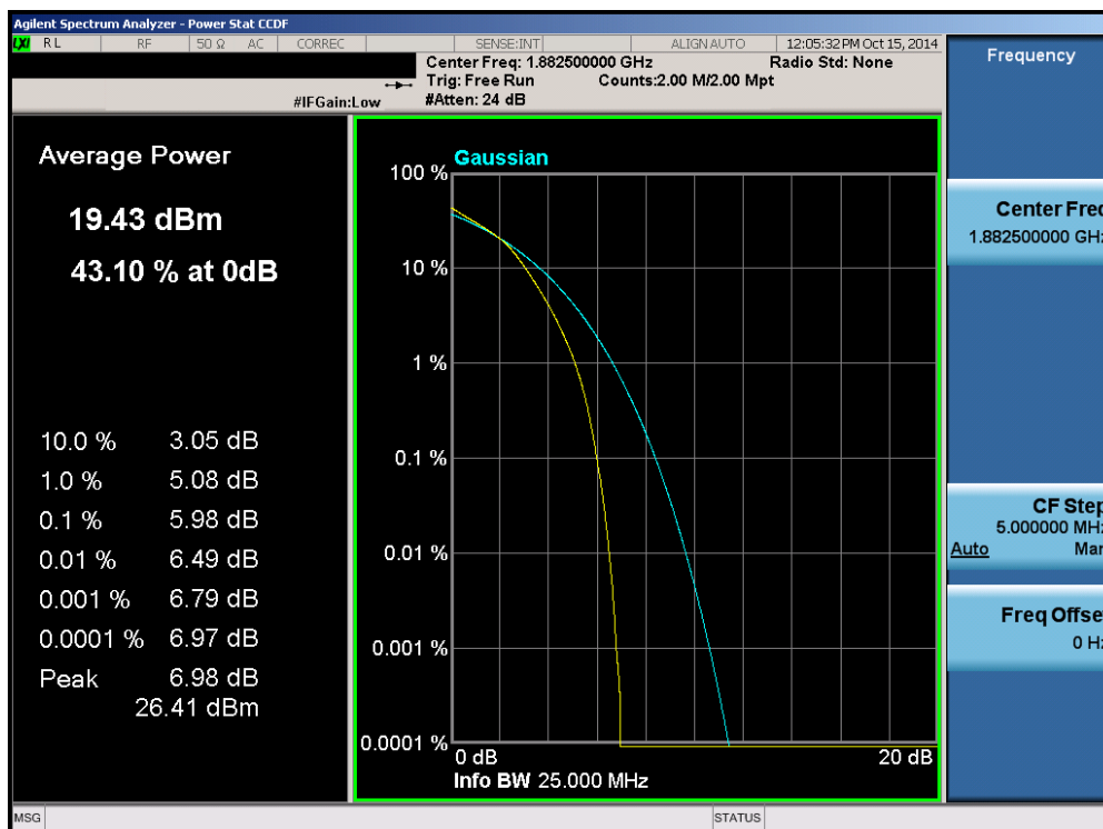
Plot 6-113. PAR Plot (Band 25 – 20.0MHz 16-QAM – RB Size 100)
