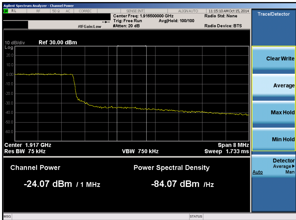
Plot 6-81. Upper Extended Band Edge Plot (Band 25 – 10.0MHz QPSK – RB Size 50)
