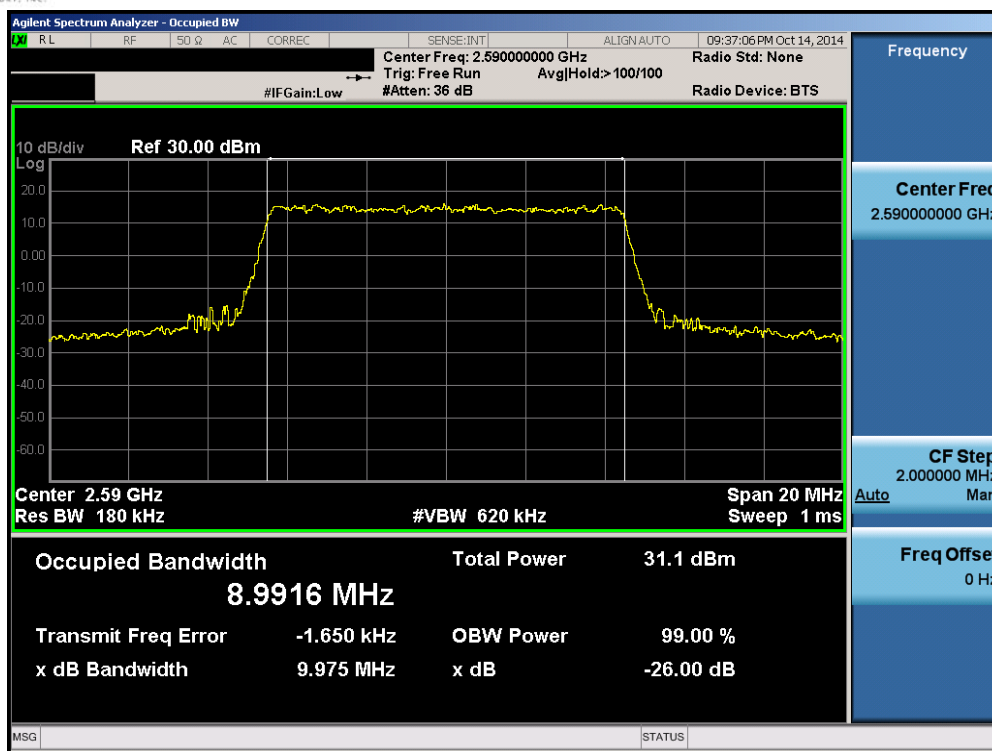
Plot 6-23. Occupied Bandwidth Plot (Band 41 – 10.0MHz QPSK – RB Size 50)
