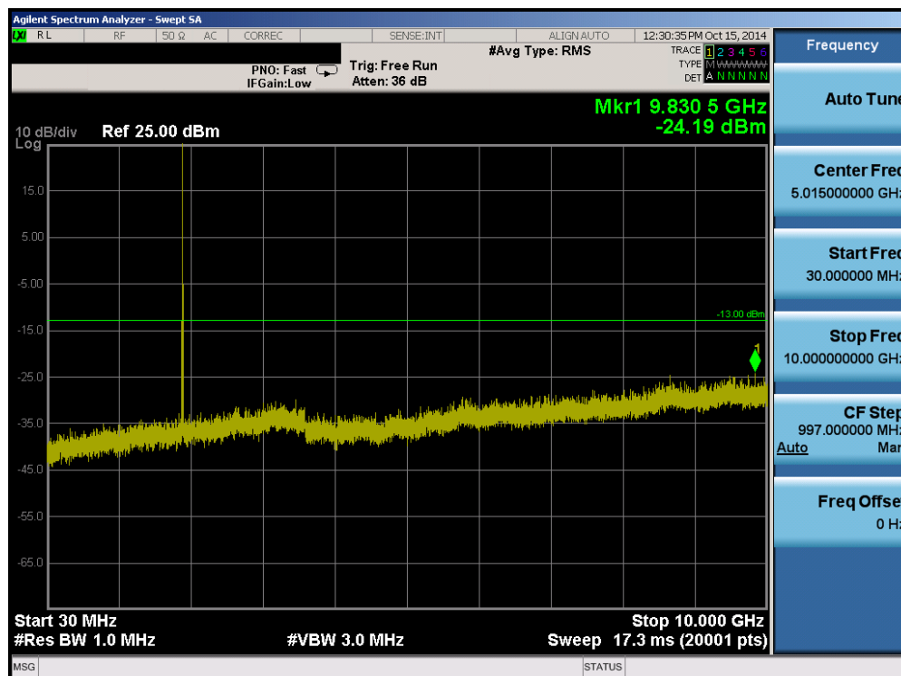
Plot 6-39. Conducted Spurious Plot (Band 25 – 10.0MHz QPSK – RB Size 1, RB Offset 0 – High Channel)
