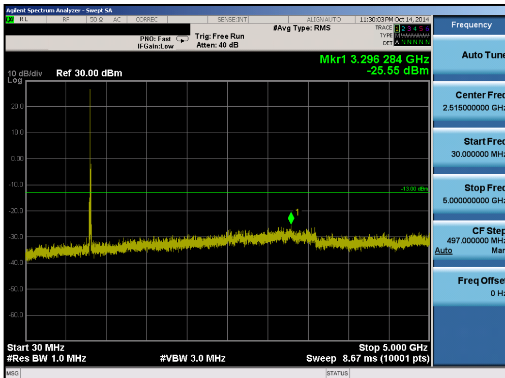
Plot 6-29. Conducted Spurious Plot (Band 26 – 10.0MHz QPSK – RB Size 1, RB Offset 0– Low Channel)
