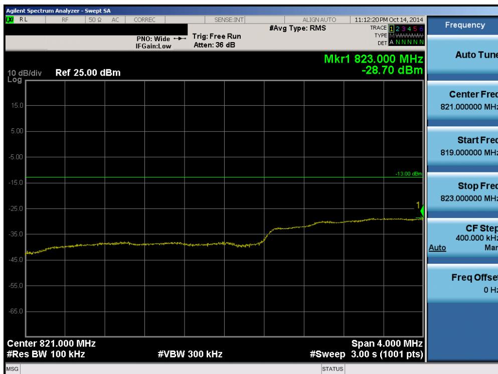
Plot 6-55. Lower Extended Band Edge Plot (Band 26 – 3.0MHz QPSK – RB Size 15)
