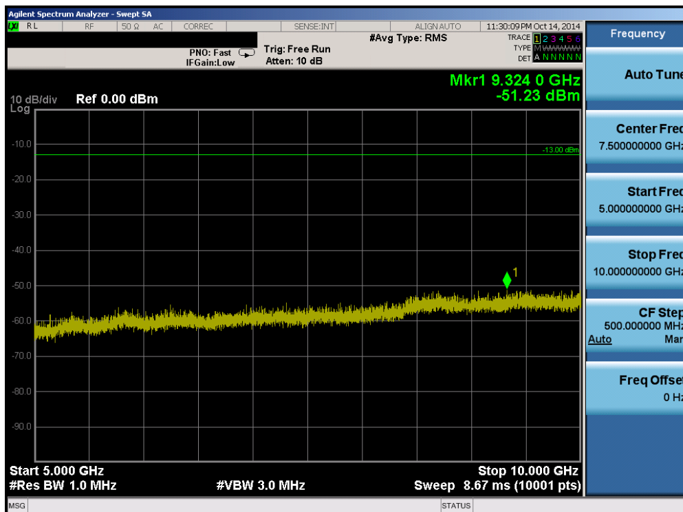
Plot 6-30. Conducted Spurious Plot (Band 26 – 10.0MHz QPSK – RB Size 1, RB Offset 0 – Low Channel)
