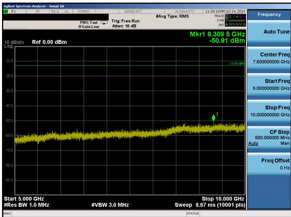
Plot 6-32. Conducted Spurious Plot (Band 26 – 10.0MHz QPSK – RB Size 1, RB Offset 0 – Mid Channel)
