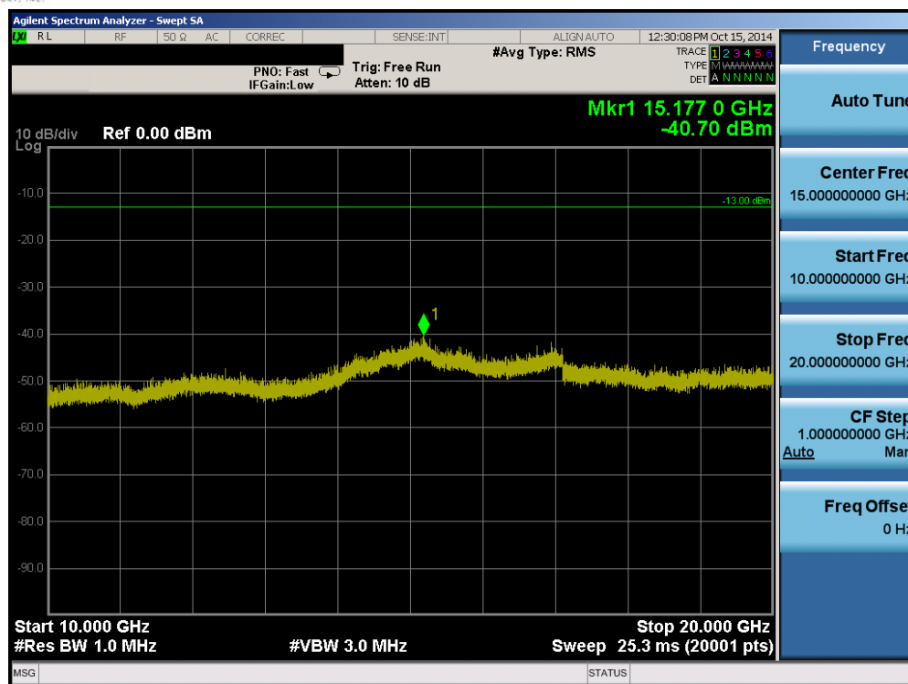
Plot 6-38. Conducted Spurious Plot (Band 25 – 10.0MHz QPSK – RB Size 1, RB Offset 0 – Mid Channel)
