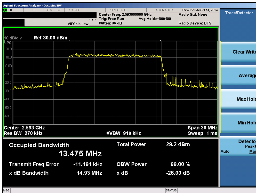
Plot 6-26. Occupied Bandwidth Plot (Band 41 – 15.0MHz 16-QAM – RB Size 75)
