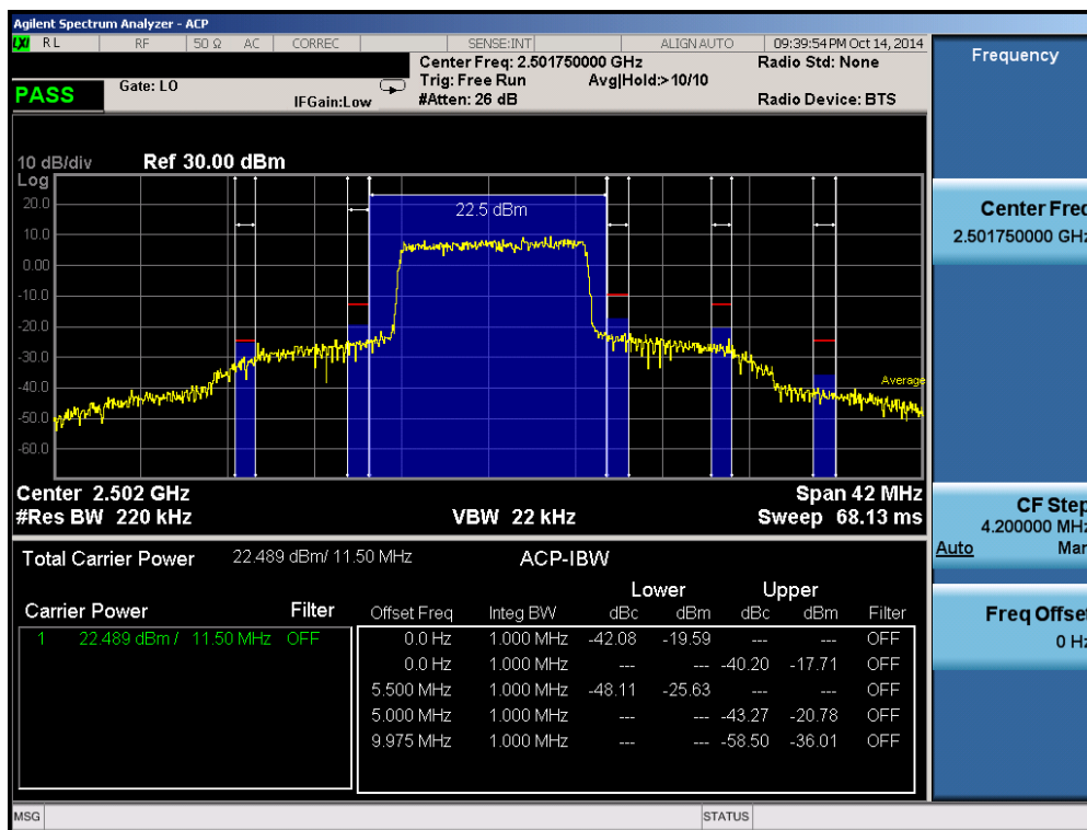
Plot 6-93. Lower ACP Plot (Band 41 – 10.0MHz QPSK – RB Size 50)
