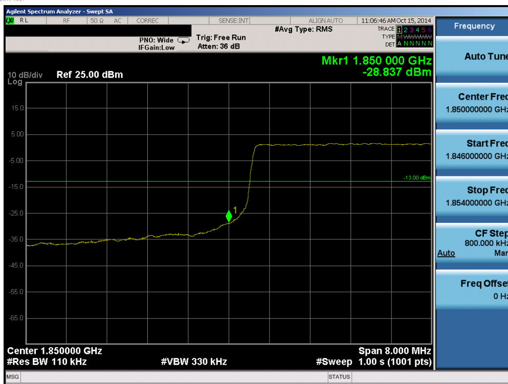
Plot 6-78. Lower Band Edge Plot (Band 25 – 10.0MHz QPSK – RB Size 50)
