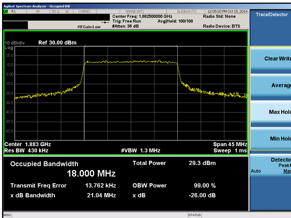
Plot 6-20. Occupied Bandwidth Plot (Band 25 – 20.0MHz 16-QAM – RB Size 100)
