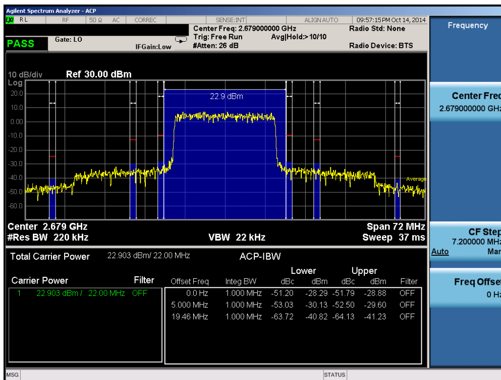
Plot 6-101. Upper ACP Plot (Band 41 – 20.0MHz QPSK – RB Size 100)
