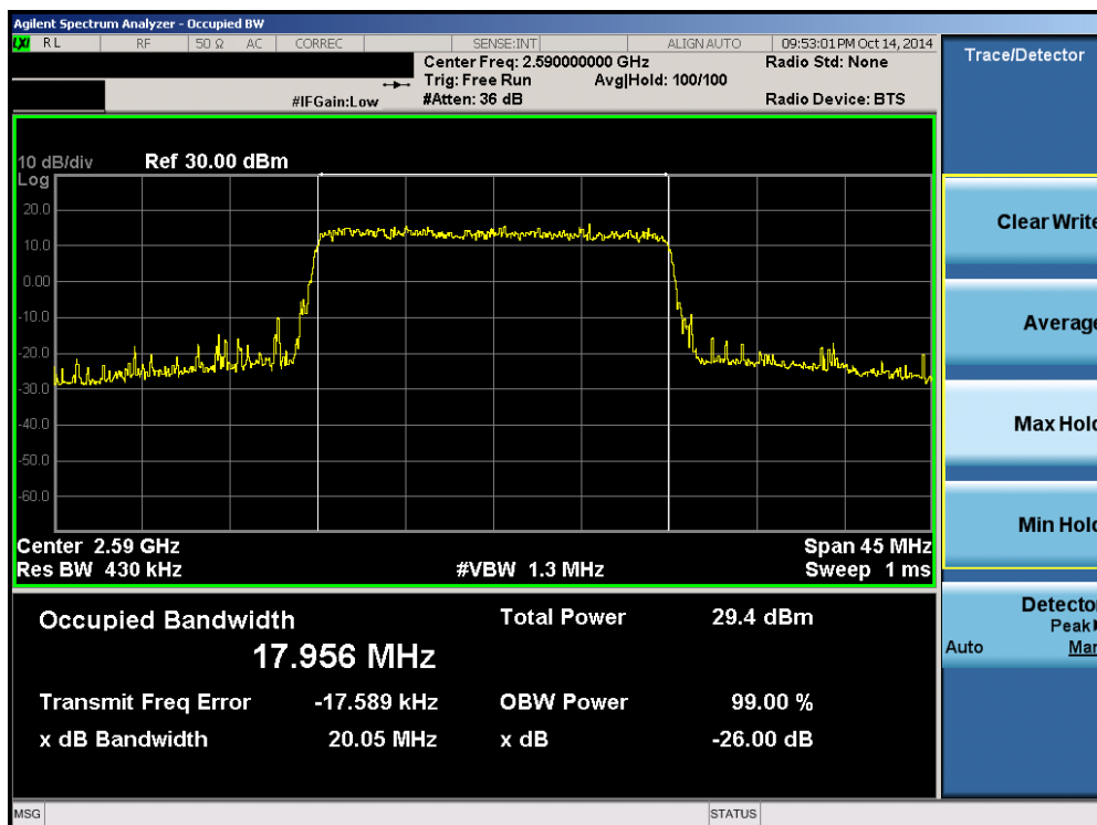
Plot 6-28. Occupied Bandwidth Plot (Band 41 – 20.0MHz 16-QAM – RB Size 100)
