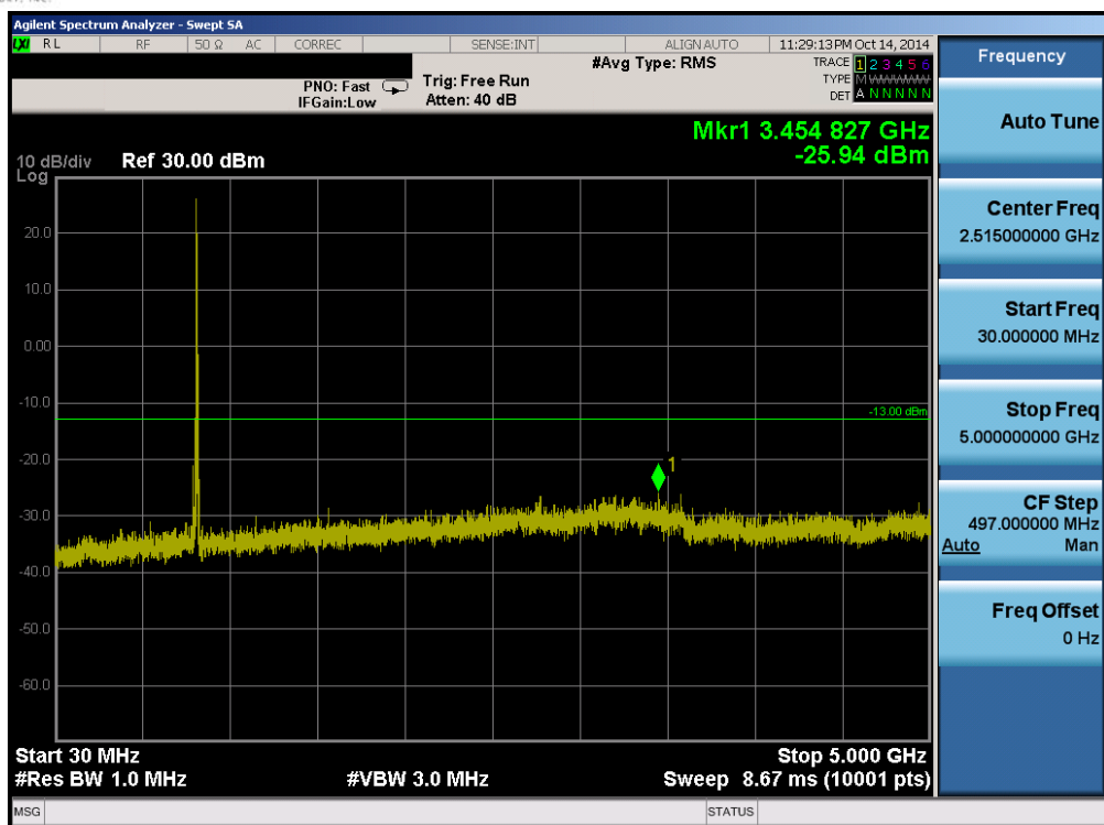
Plot 6-31. Conducted Spurious Plot (Band 26 – 10.0MHz QPSK – RB Size 1, RB Offset 0 – Mid Channel)
