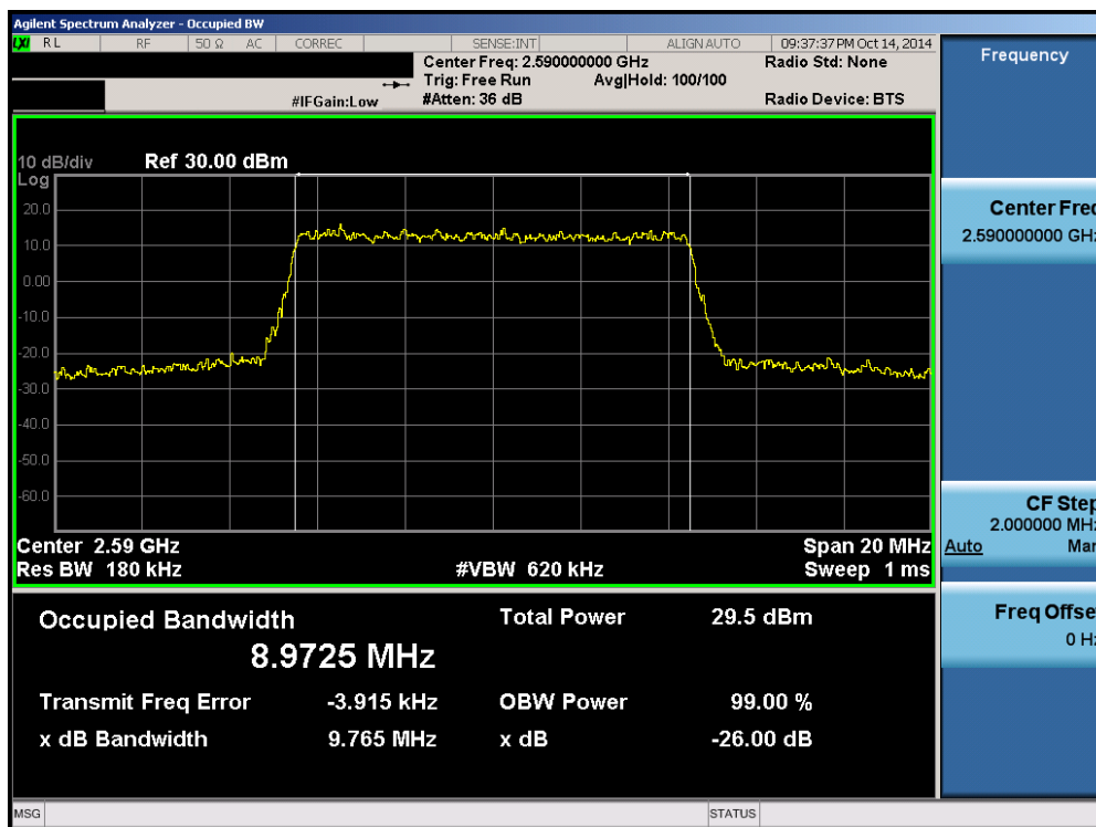
Plot 6-24. Occupied Bandwidth Plot (Band 41 – 10.0MHz 16-QAM – RB Size 50)
