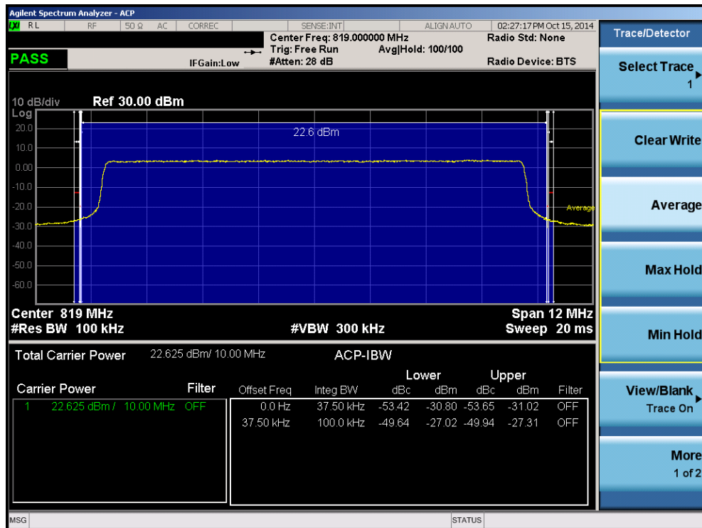
Plot 8-33. Channel Edge Plot (10MHz QPSK – RB Size 50)
