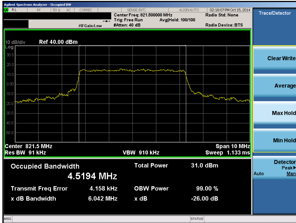
Plot 8-28. Occupied Bandwidth Plot (5MHz 16-QAM – RB Size 25 – High Channel)
