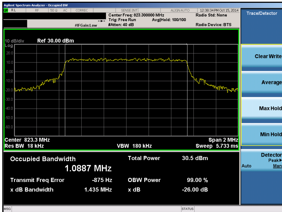
Plot 8-9. Occupied Bandwidth Plot (1.4MHz QPSK – RB Size 6 – High Channel)
