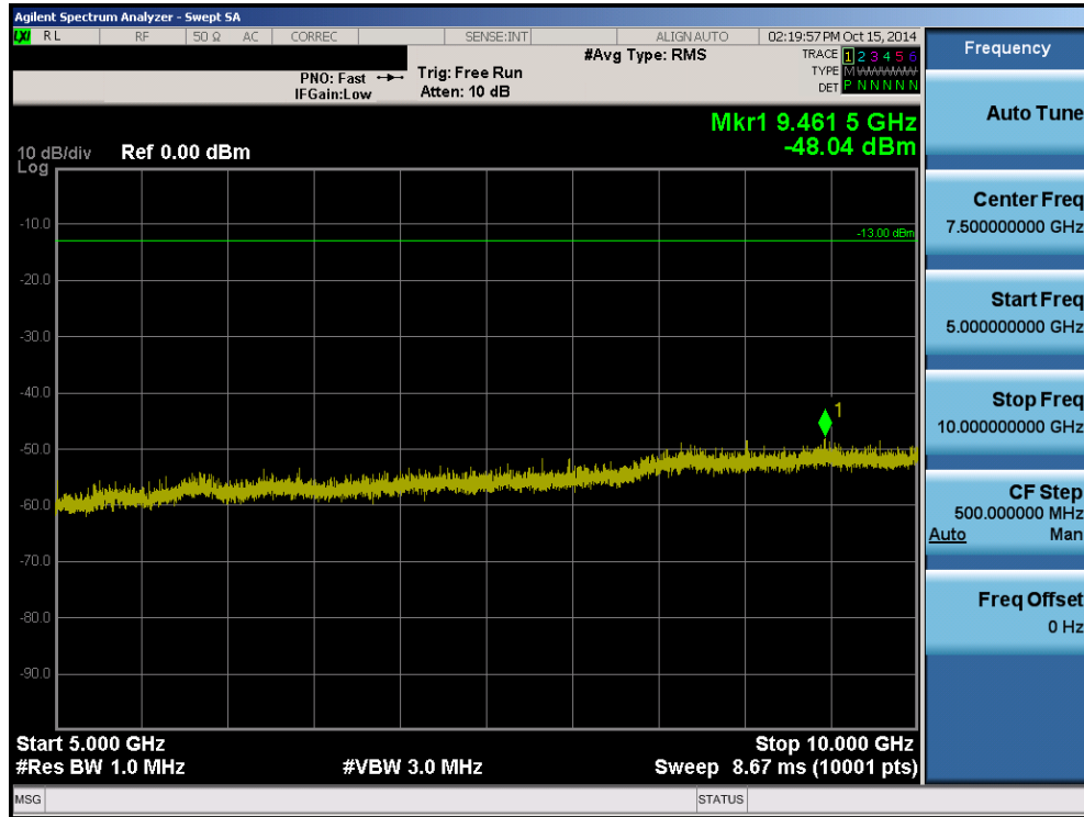
Plot 8-30. Conducted Spurious Plot (5MHz QPSK – RB Size 1, Offset 0 – High Channel)
