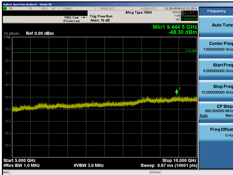
Plot 8-13. Conducted Spurious Plot (3MHz QPSK – RB Size 1, RB Offset 0 – Low Channel)
