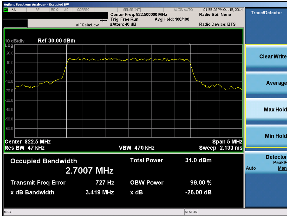
Plot 8-18. Occupied Bandwidth Plot (3MHz 16-QAM – RB Size 15 – High Channel)
