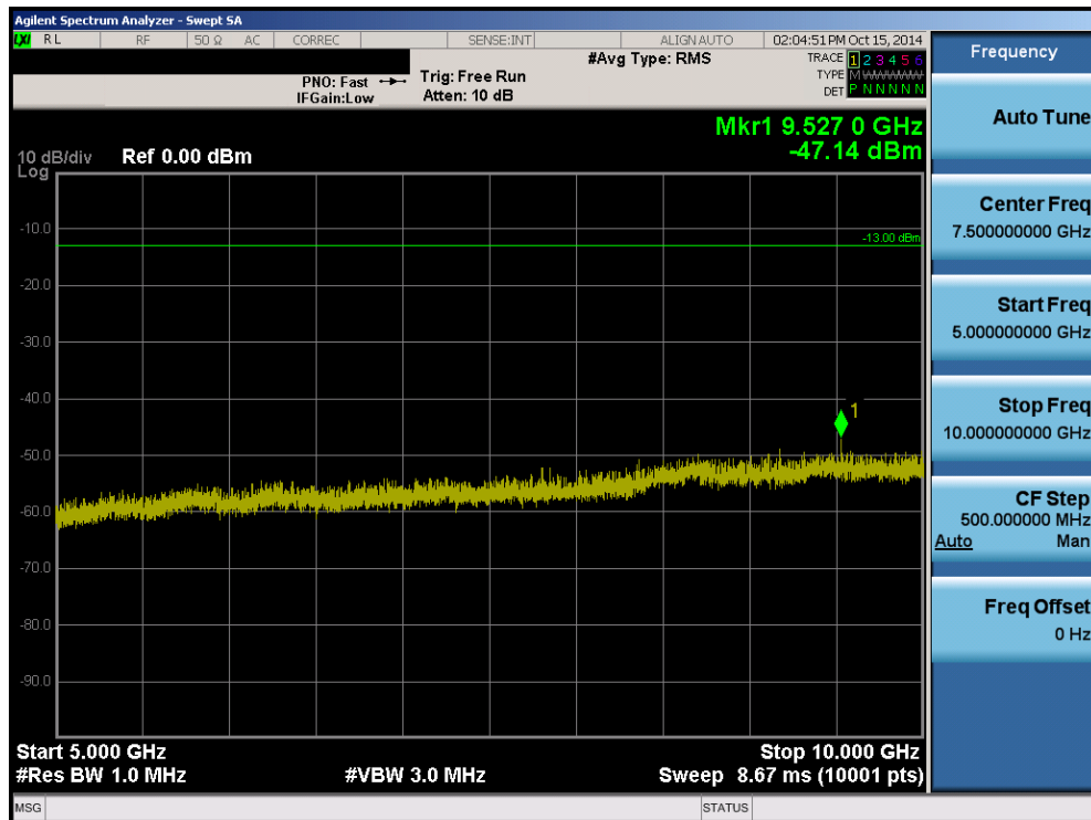
Plot 8-25. Conducted Spurious Plot (5MHz QPSK – RB Size 1, Offset 0 – Low Channel)
