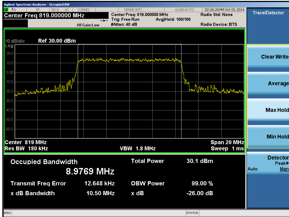
Plot 8-32. Occupied Bandwidth Plot (10MHz 16-QAM – RB Size 50)
