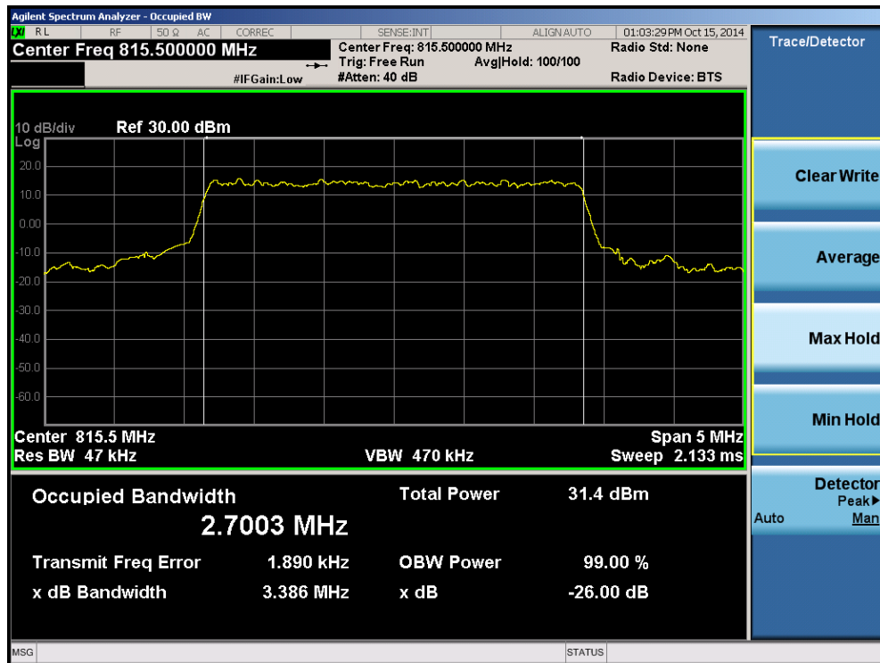
Plot 8-15. Occupied Bandwidth Plot (3MHz 16-QAM – RB Size 15– Low Channel)
