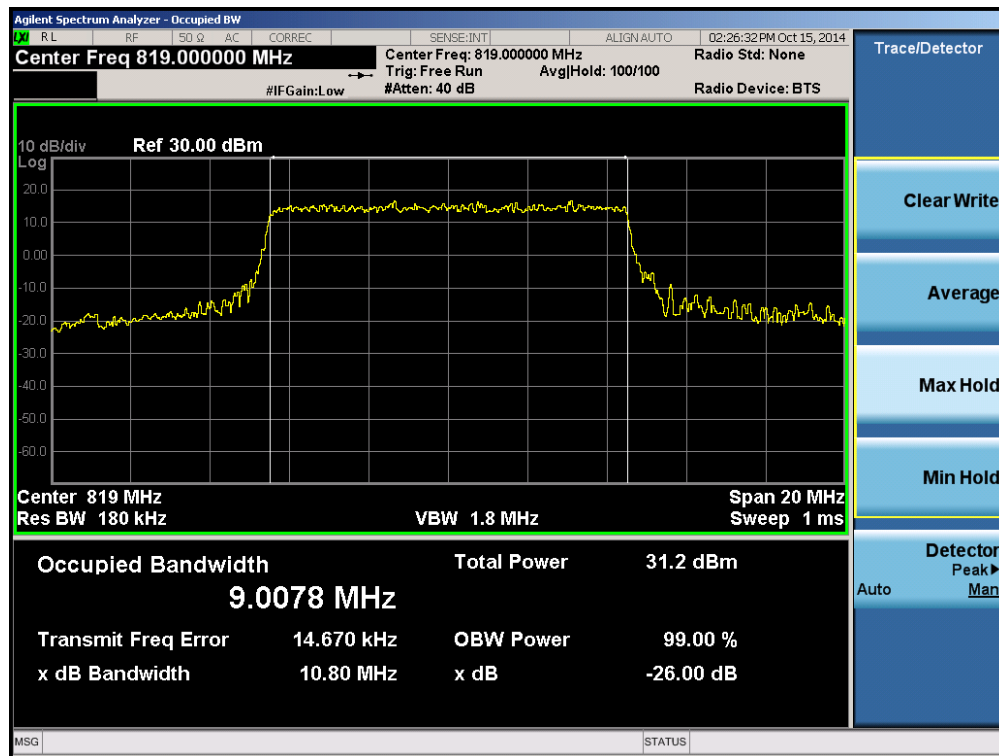
Plot 8-31. Occupied Bandwidth Plot (10MHz QPSK – RB Size 50)
