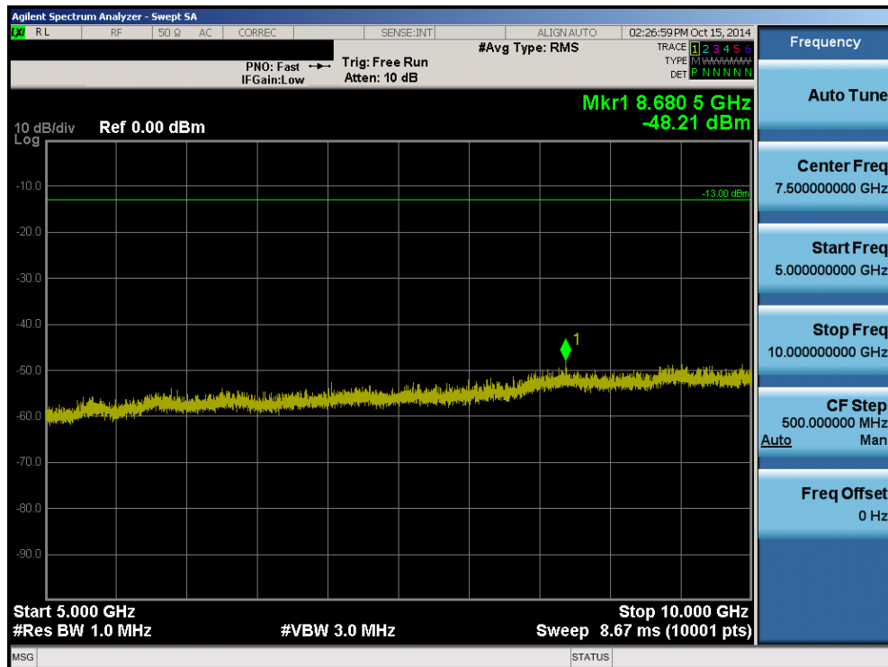
Plot 8-35. Conducted Spurious Plot (10MHz QPSK – RB Size 1, Offset 0)
