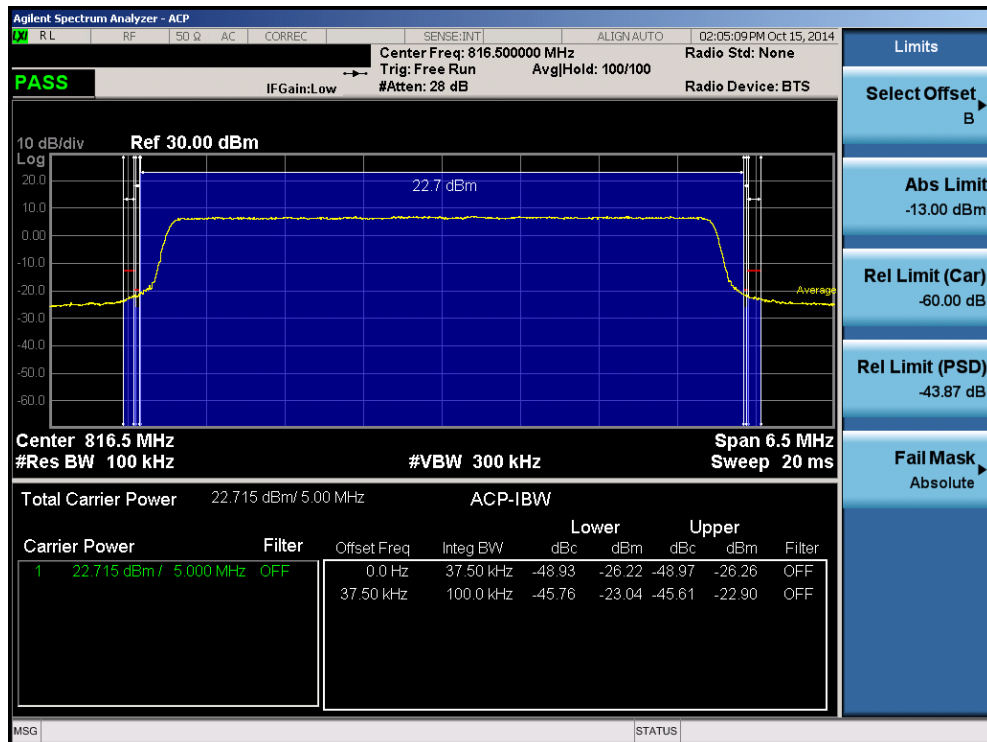
Plot 8-21. Channel Edge Plot (5MHz QPSK – RB Size 25– Low Channel)
