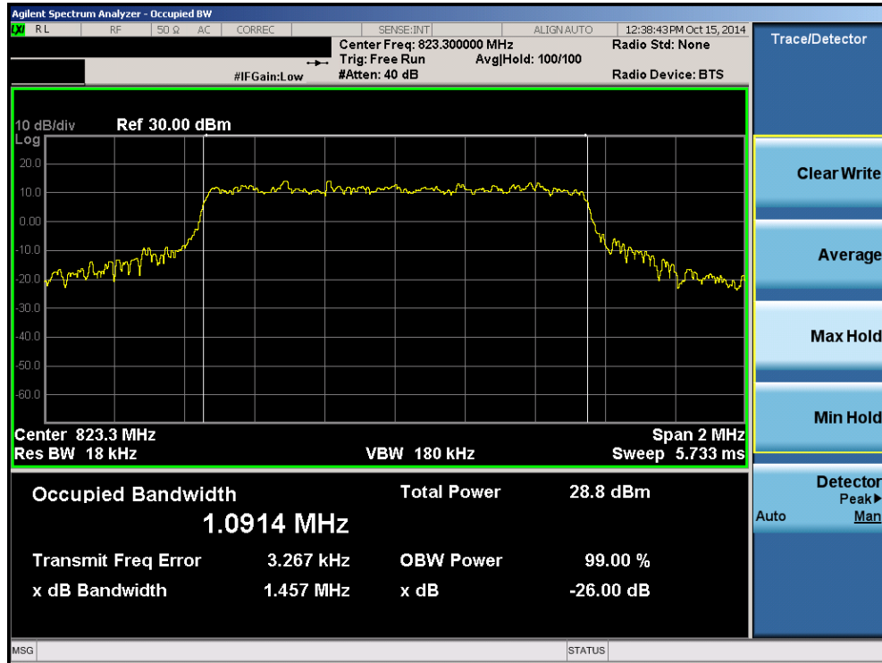
Plot 8-10. Occupied Bandwidth Plot (1.4MHz – RB Size 6 – High Channel)
