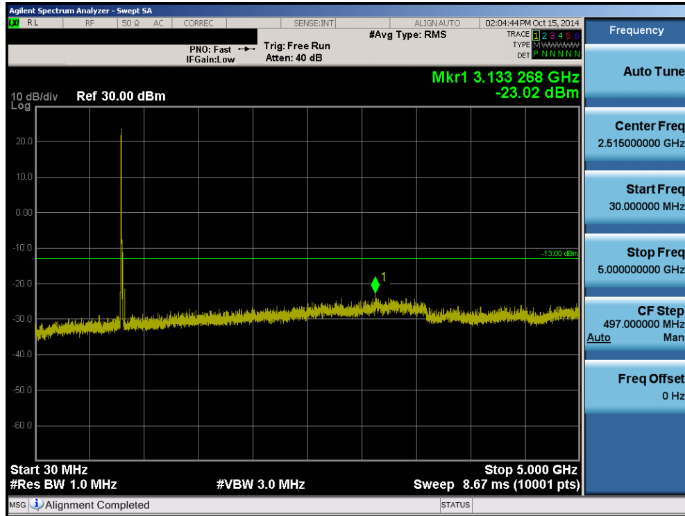
Plot 8-24. Conducted Spurious Plot (5MHz QPSK – RB Size 1, Offset 0 – Low Channel)
