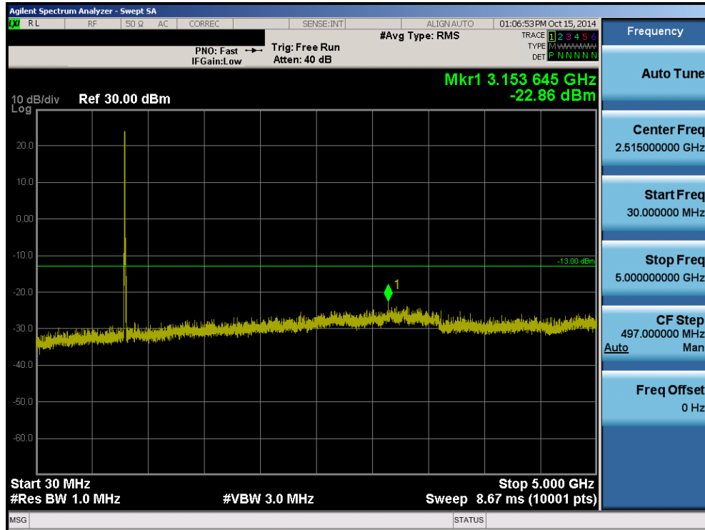
Plot 8-12. Conducted Spurious Plot (3MHz QPSK – RB Size 1, RB Offset 0 – Low Channel)
