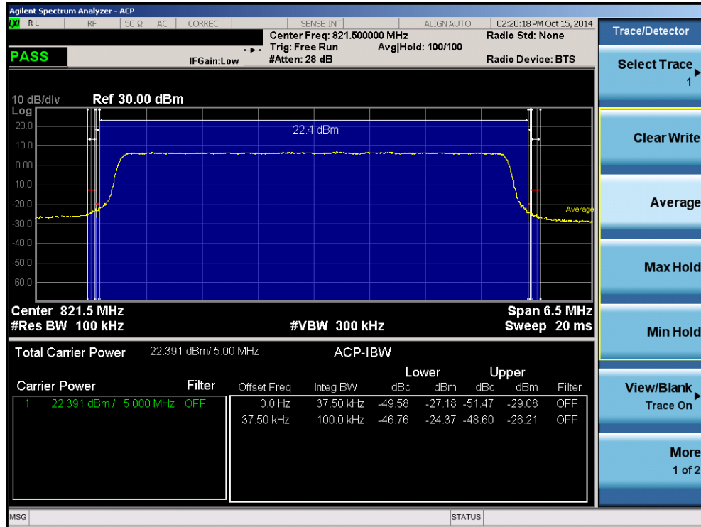
Plot 8-26. Channel Edge Plot (5MHz QPSK - RB Size 25 - High Channel)
