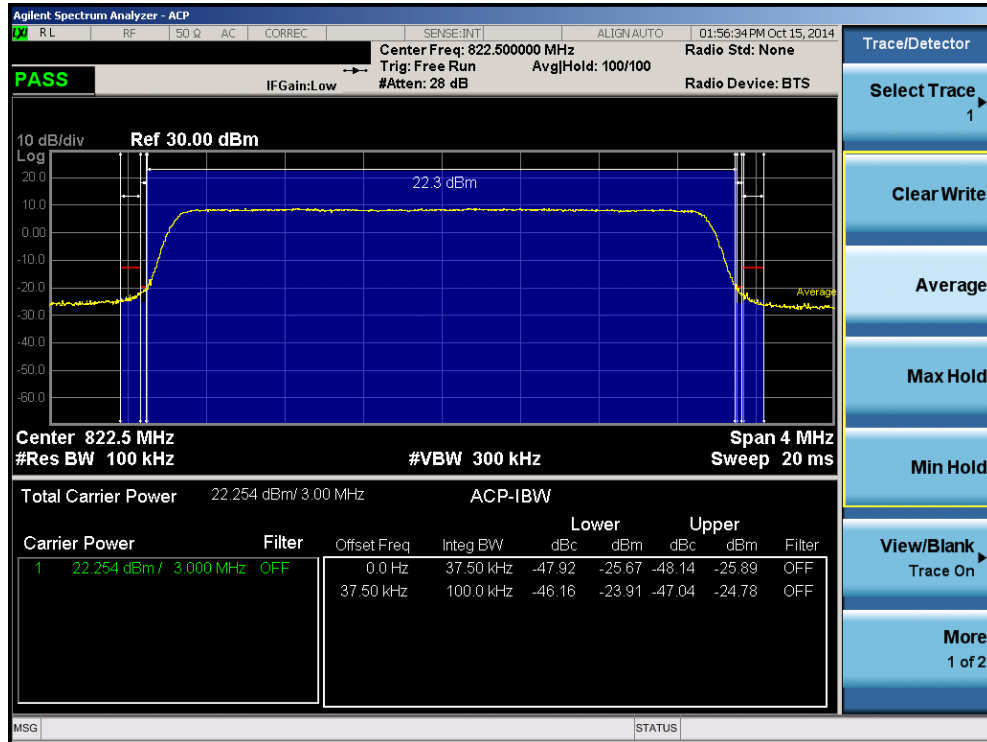
Plot 8-16. Channel Edge Plot (3MHz QPSK - RB Size 15 - High Channel)
