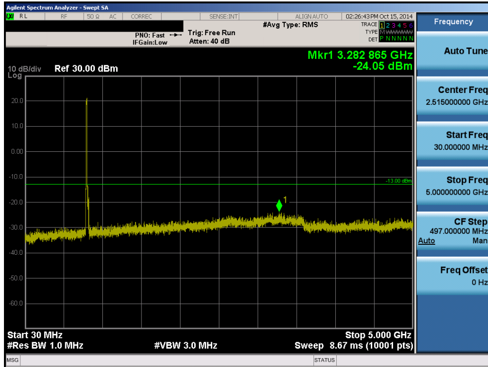
Plot 8-34. Conducted Spurious Plot (10MHz QPSK – RB Size 1, Offset 0)
