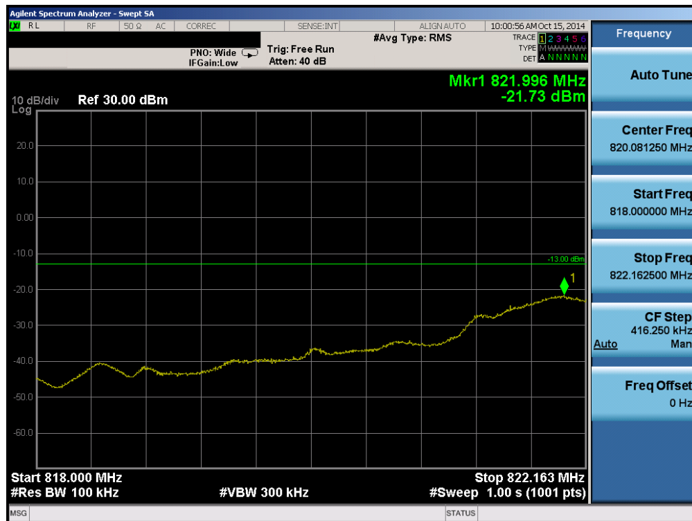
Plot 7-9. Inner Extended Band Edge Plot (Ch. 684)
