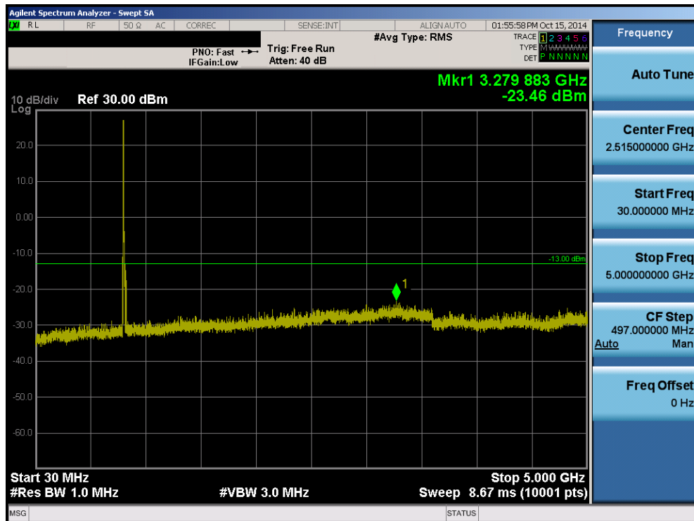
Plot 8-19. Conducted Spurious Plot (3MHz 16-QAM – RB Size 1, RB Offset 0 – High Channel)
