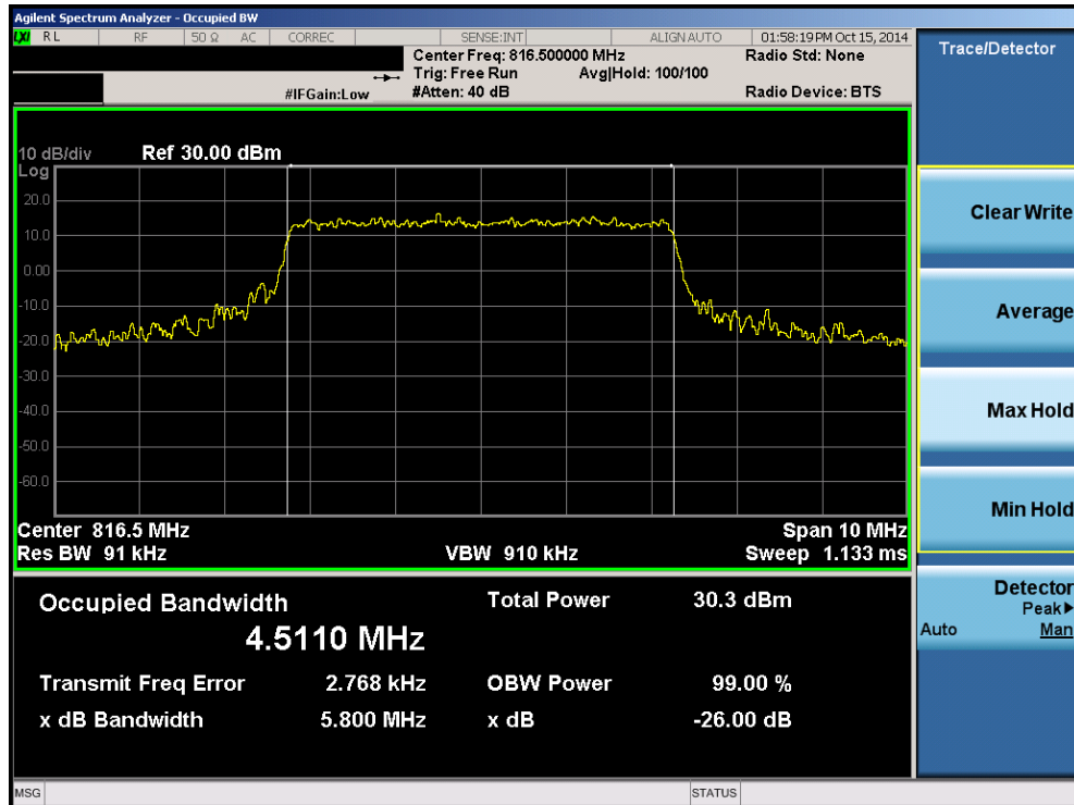
Plot 8-23. Occupied Bandwidth Plot (5MHz 16-QAM – RB Size 25– Low Channel)
