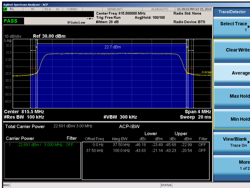
Plot 8-11. Channel Edge Plot (3MHz QPSK – RB Size 15– Low Channel)
