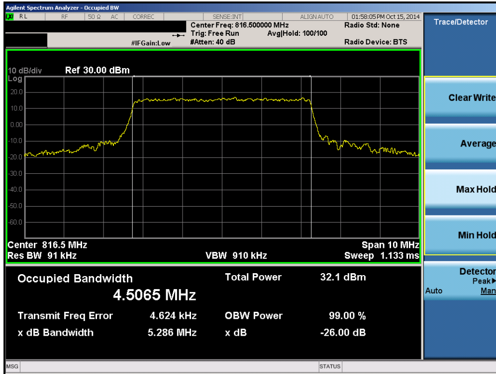
Plot 8-22. Occupied Bandwidth Plot (5MHz QPSK – RB Size 25– Low Channel)
