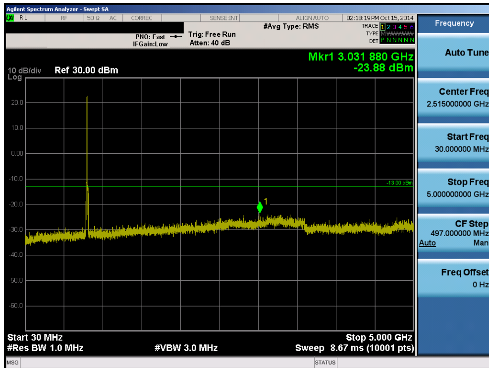
Plot 8-29. Conducted Spurious Plot (5MHz QPSK – RB Size 1, Offset 0 – High Channel)
