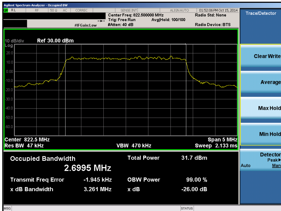
Plot 8-17. Occupied Bandwidth Plot (3MHz QPSK - RB Size 15 - High Channel)
