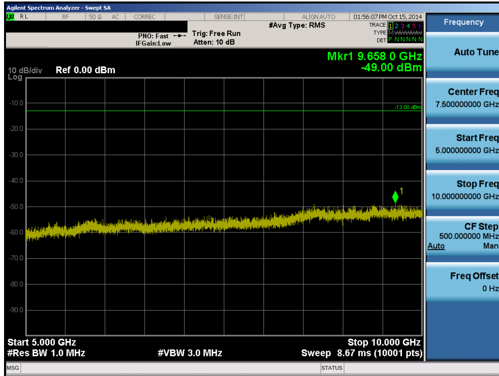
Plot 8-20. Conducted Spurious Plot (3MHz 16-QAM – RB Size 1, RB Offset 0 – High Channel)
