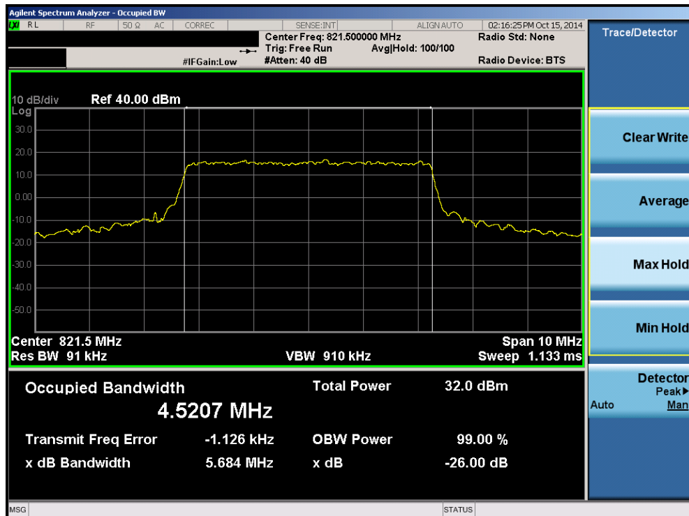
Plot 8-27. Occupied Bandwidth Plot (5MHz QPSK - RB Size 25 - High Channel)
