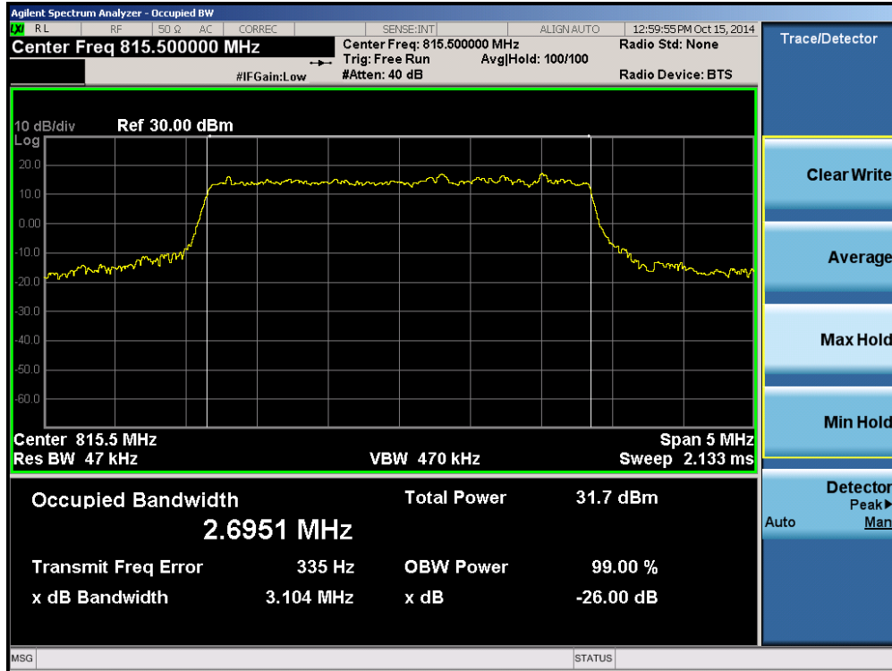
Plot 8-14. Occupied Bandwidth Plot (3MHz QPSK – RB Size 15– Low Channel)
