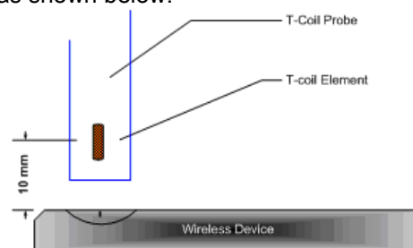
Figure 5-10 Measurement Distance
