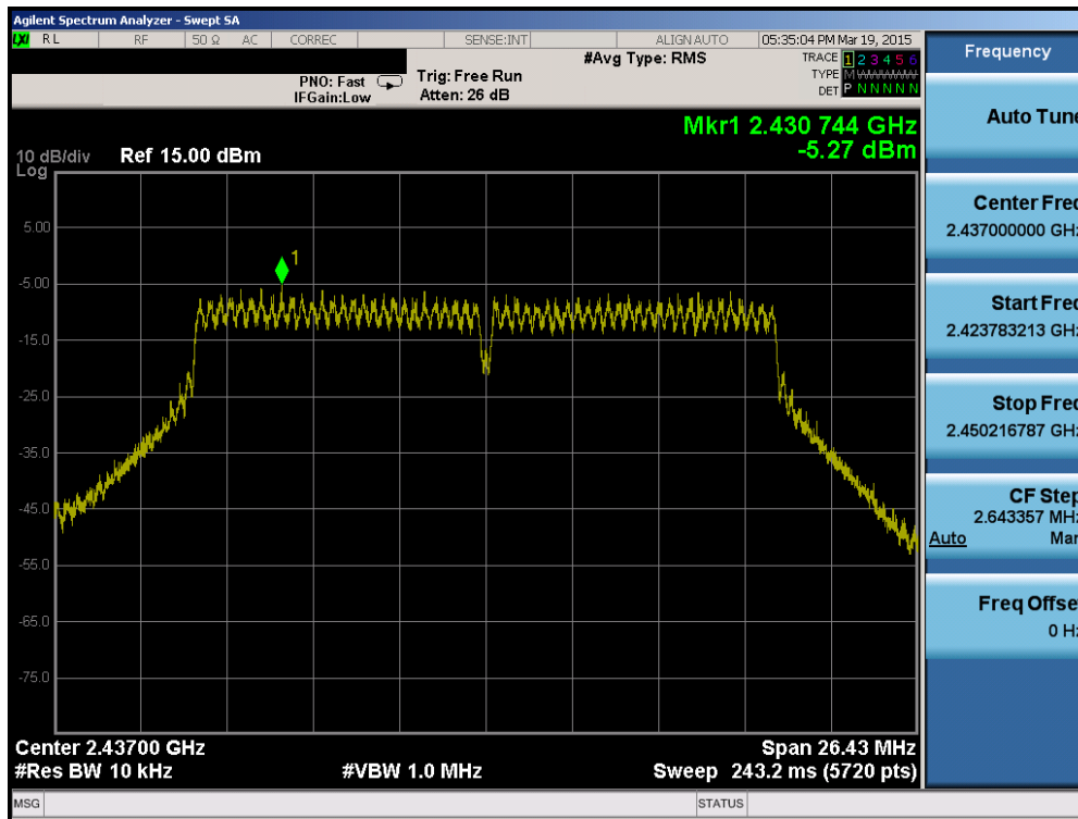
Plot 6-17. Power Spectral Density Plot (802.11n (2.4GHz) – Ch. 6)
