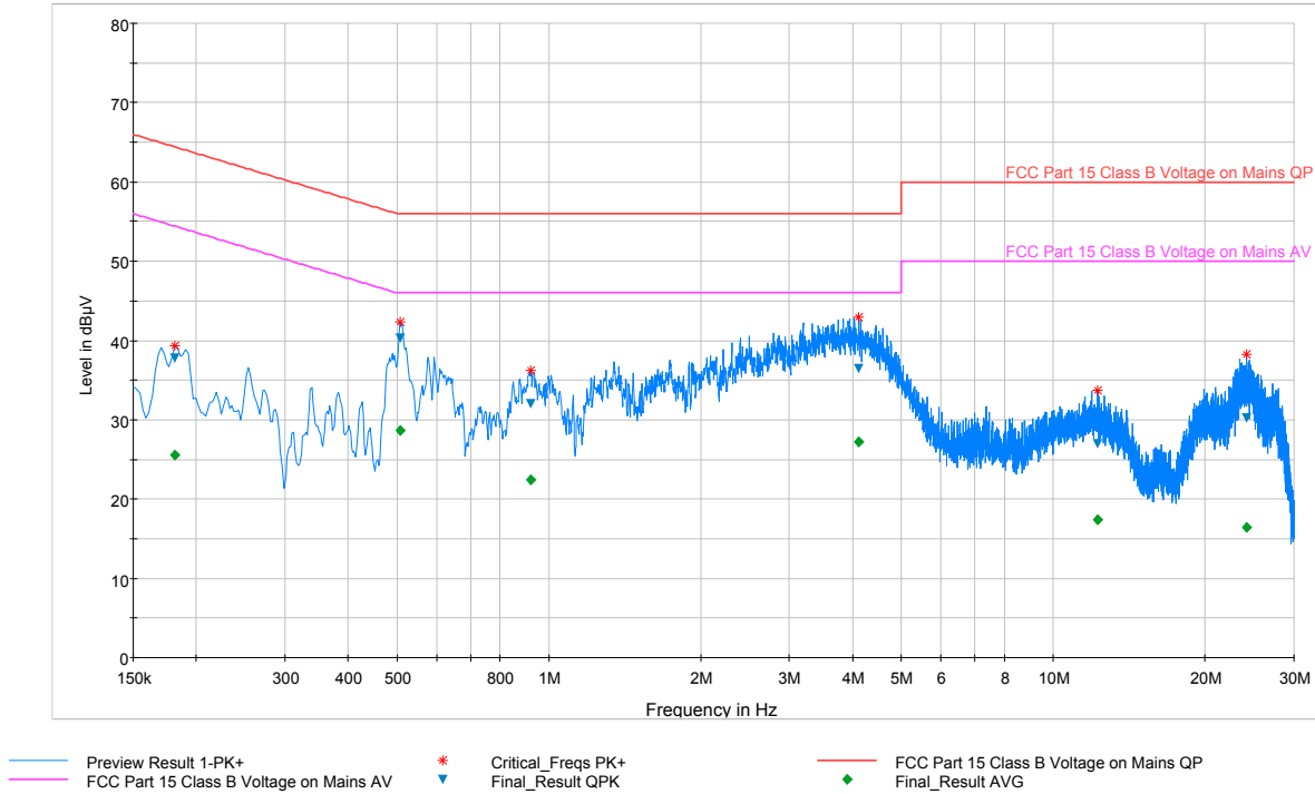
Plot 6-45. Line Conducted Plot with 802.11b (L1)
