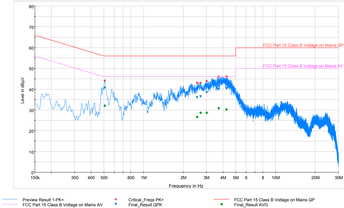
Plot 6-46. Line Conducted Plot with 802.11b (N)
