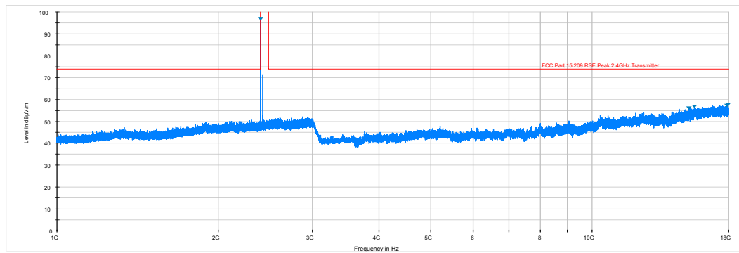
Plot 6-19. Radiated Spurious Plot above 1GHz (BTLE – Ch. 0, Ant. Pol. V)
