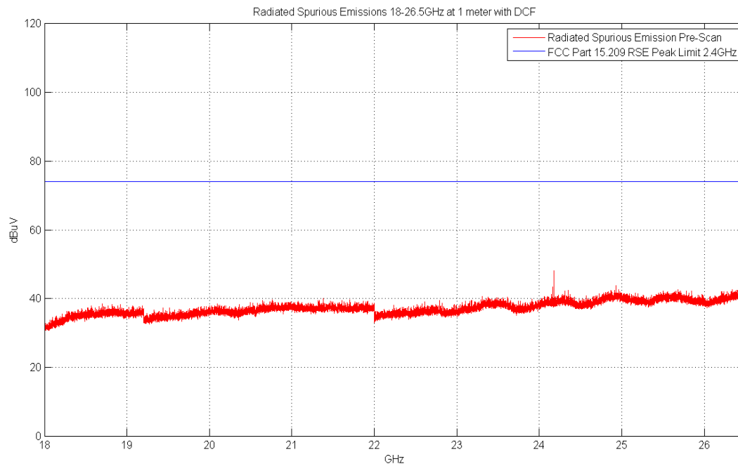
Plot 6-25. Radiated Spurious Plot above 18GHz (Pol. V)
