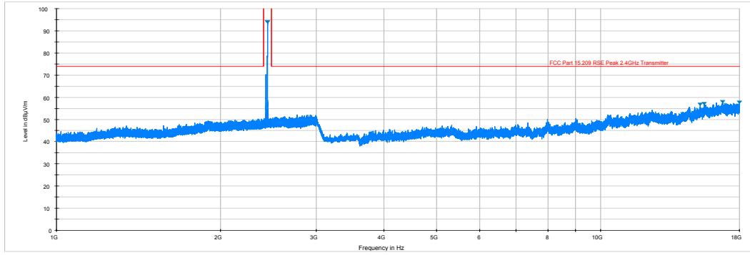
Plot 6-21. Radiated Spurious Plot above 1GHz (BTLE – Ch. 19, Ant. Pol. V)
