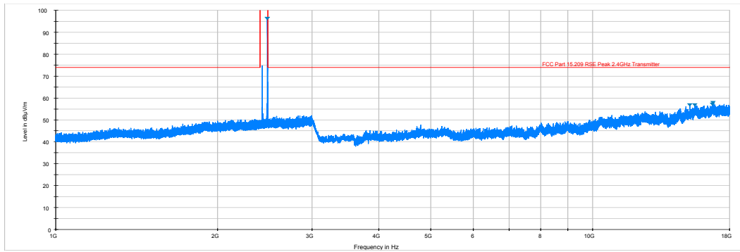
Plot 6-22. Radiated Spurious Plot above 1GHz (BTLE – Ch. 39, Ant. Pol. H)
