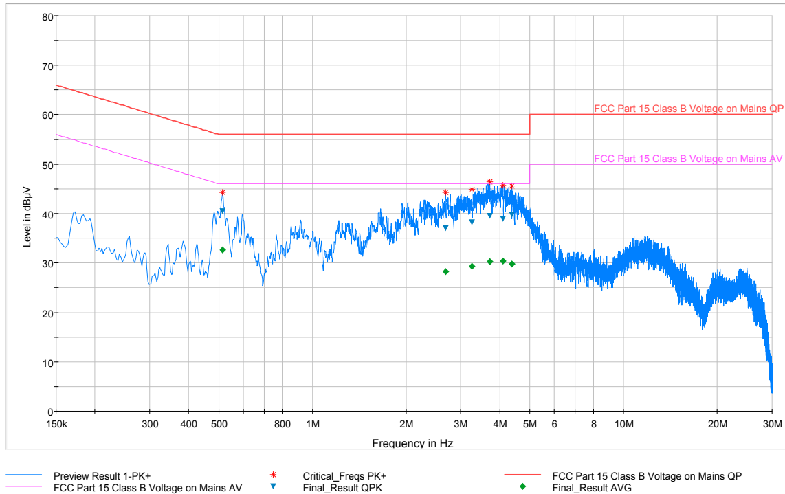
Plot 6-31. Line Conducted Plot with Bluetooth LE (N)
