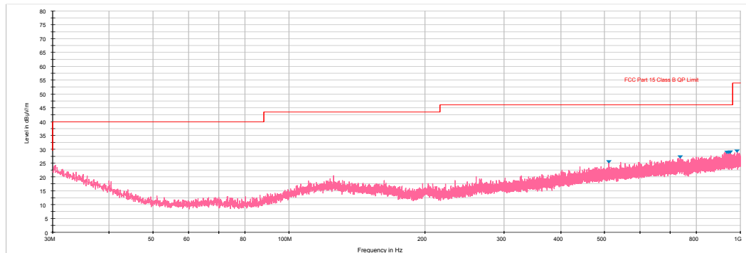
Plot 6-28. Radiated Spurious Plot below 1GHz (Pol. H)
