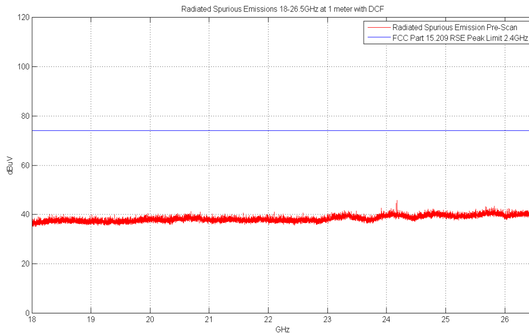
Plot 6-24. Radiated Spurious Plot above 18GHz (Pol. H)
