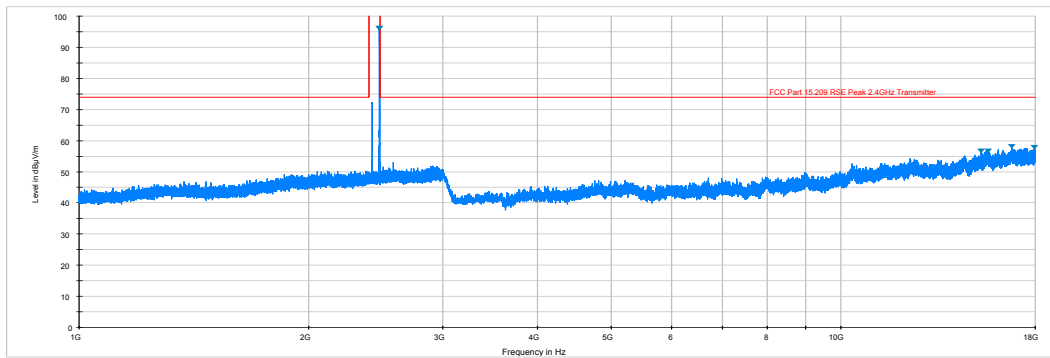
Plot 6-23. Radiated Spurious Plot above 1GHz (BTLE – Ch. 39, Ant. Pol. V)
