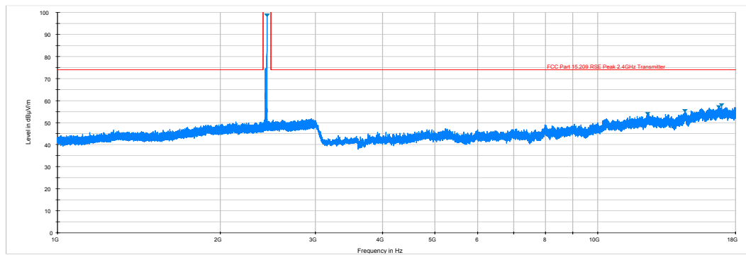
Plot 6-20. Radiated Spurious Plot above 1GHz (BTLE – Ch. 19, Ant. Pol. H)
