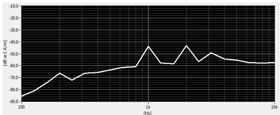
Figure 7-4 Worst-case ABM2 Plot for LTE
