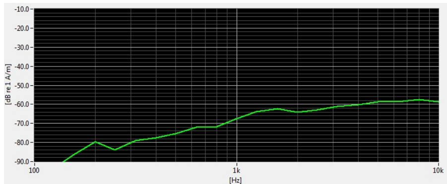
Figure 7-3 Worst-case ABM2 Plot for UMTS
