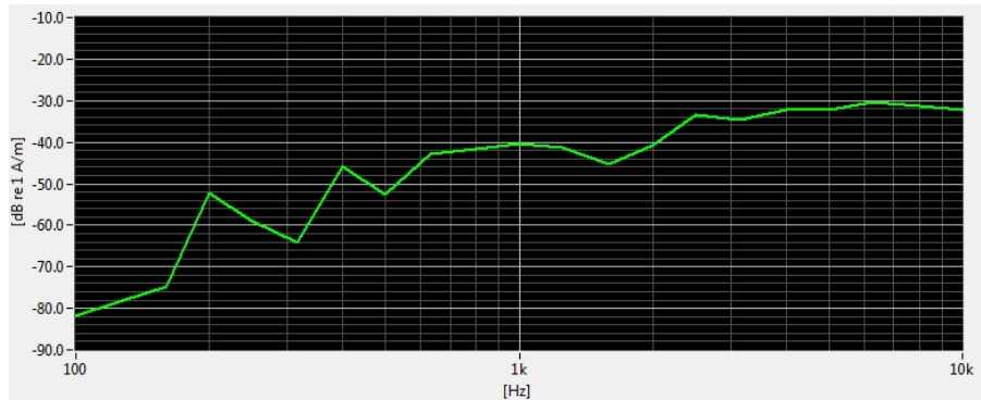
Figure 7-2 Worst-case ABM2 Plot for GSM
