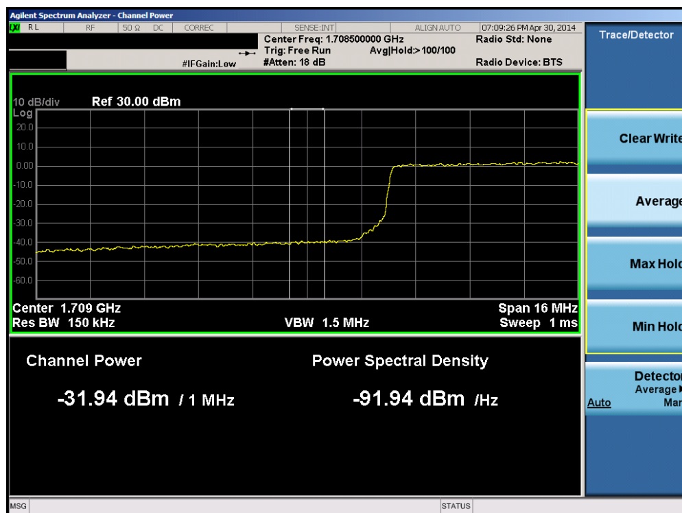
Plot 6-118. Lower Extended Band Edge Plot (Band 4 – 20.0MHz QPSK – RB Size 100)
