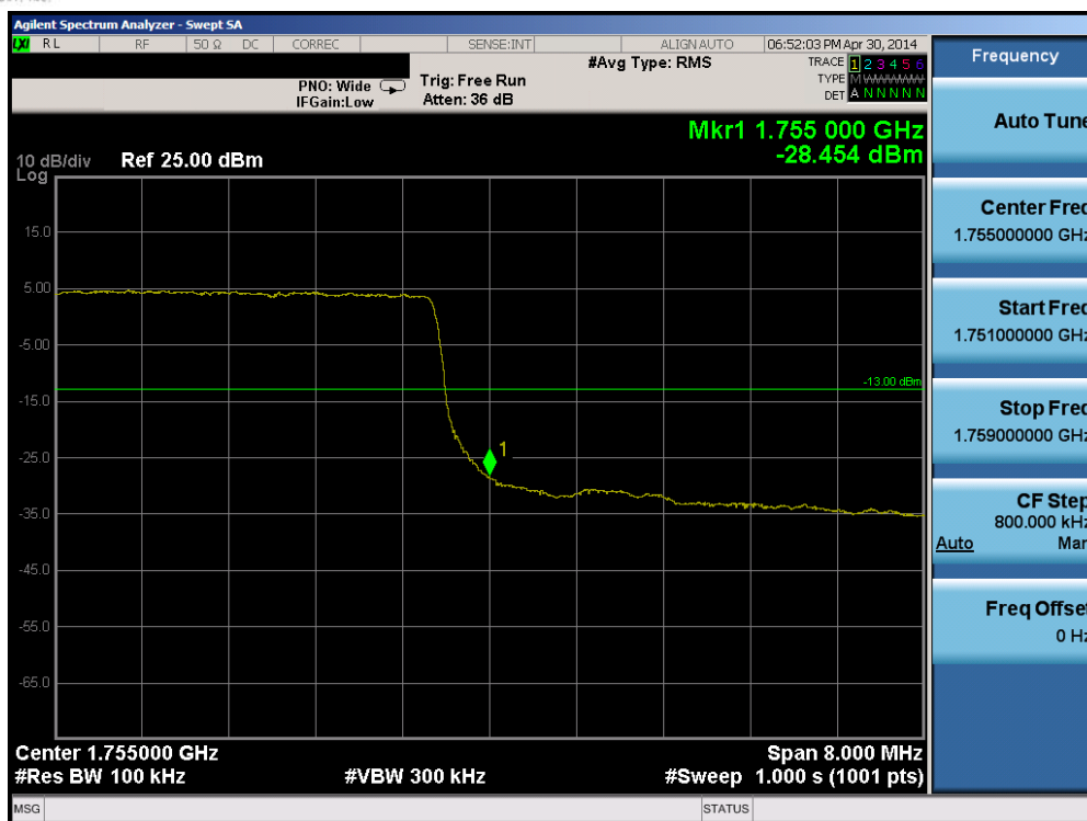
Plot 6-111. Upper Band Edge Plot (Band 4 – 10.0MHz QPSK – RB Size 50)
