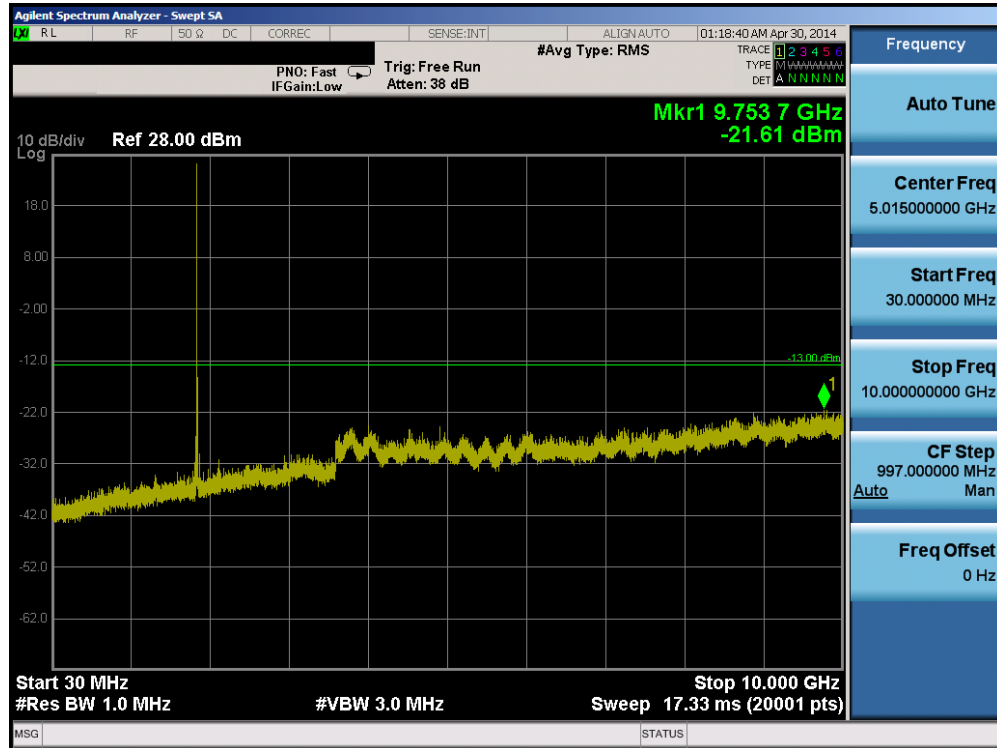
Plot 6-59. Conducted Spurious Plot (Band 2 – 20.0MHz QPSK – RB Size 1, RB Offset 0– Low Channel)
