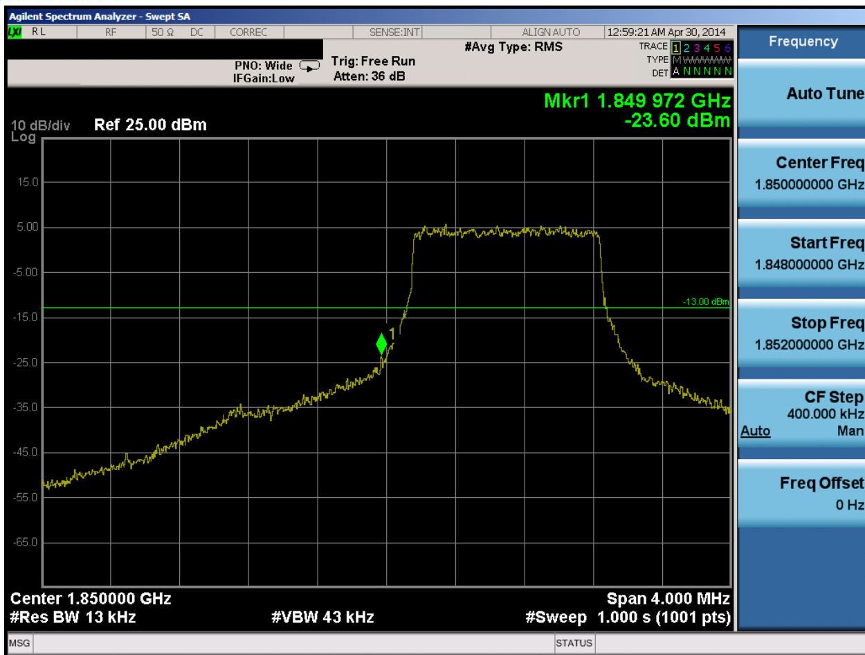
Plot 6-121. Lower Band Edge Plot (Band 2 – 1.4MHz QPSK – RB Size 6)
