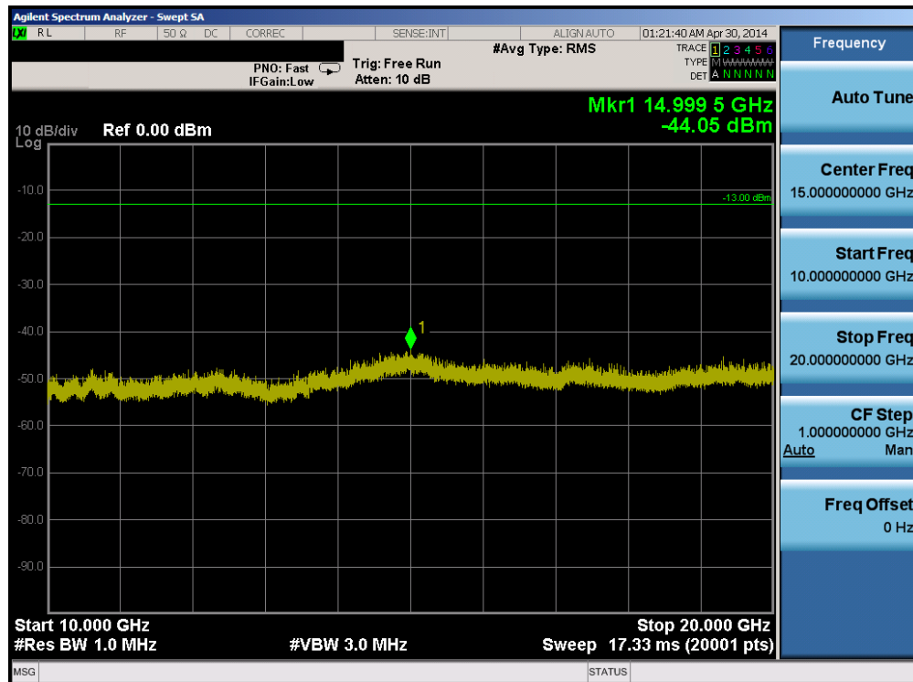
Plot 6-64. Conducted Spurious Plot (Band 2 – 20.0MHz QPSK – RB Size 1, RB Offset 0 – High Channel)
