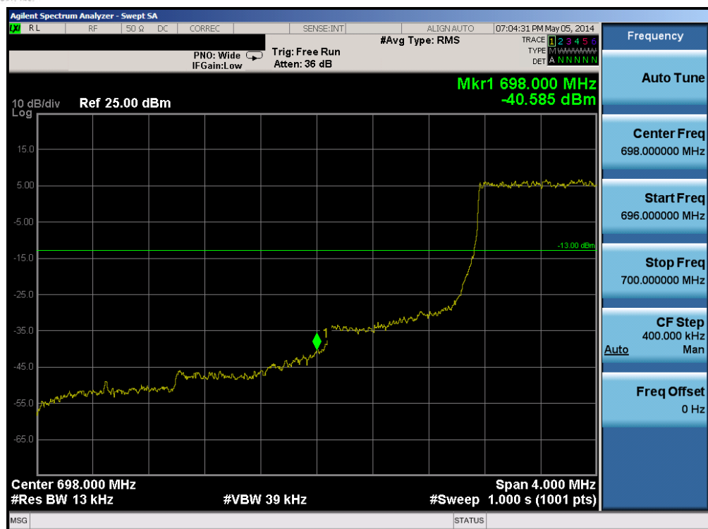
Plot 6-65. Lower Band Edge Plot (Band 12 – 1.4MHz QPSK – RB Size 6)
