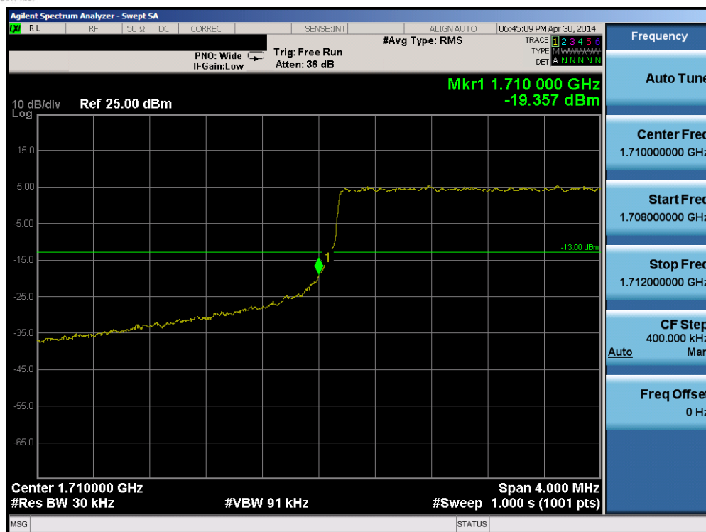
Plot 6-101. Lower Band Edge Plot (Band 4 – 3.0MHz QPSK – RB Size 15)
