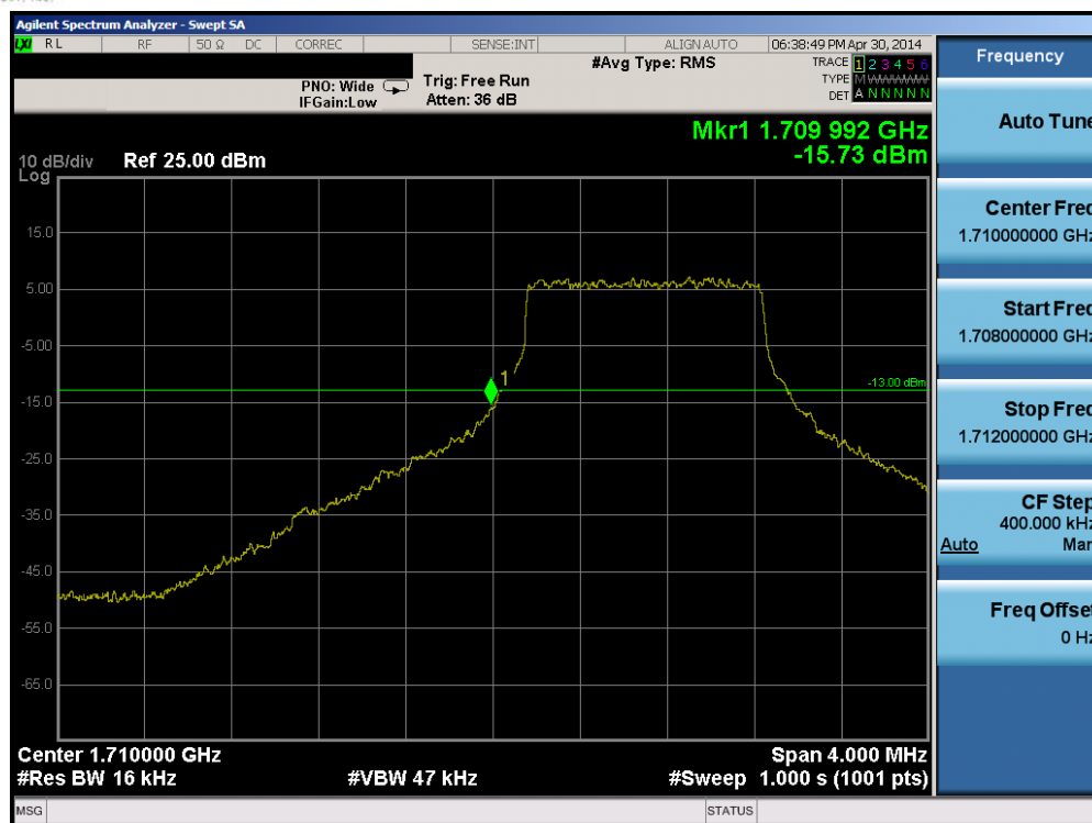
Plot 6-97. Lower Band Edge Plot (Band 4 – 1.4MHz QPSK – RB Size 6)
