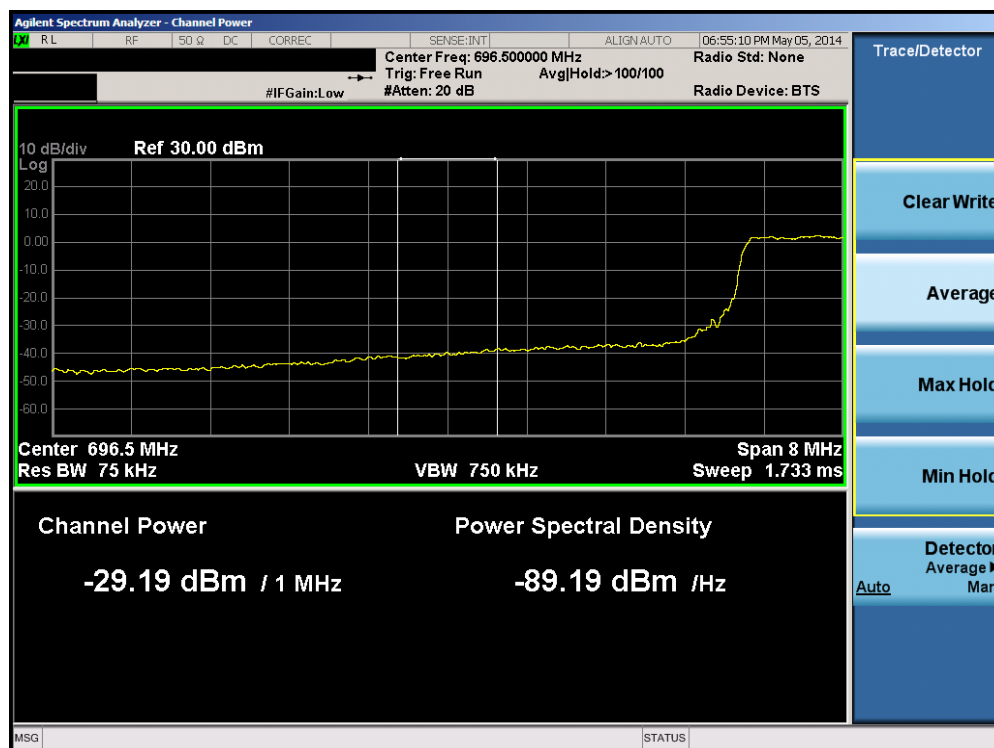
Plot 6-78. Lower Extended Band Edge Plot (Band 12 – 10.0MHz QPSK – RB Size 50)
