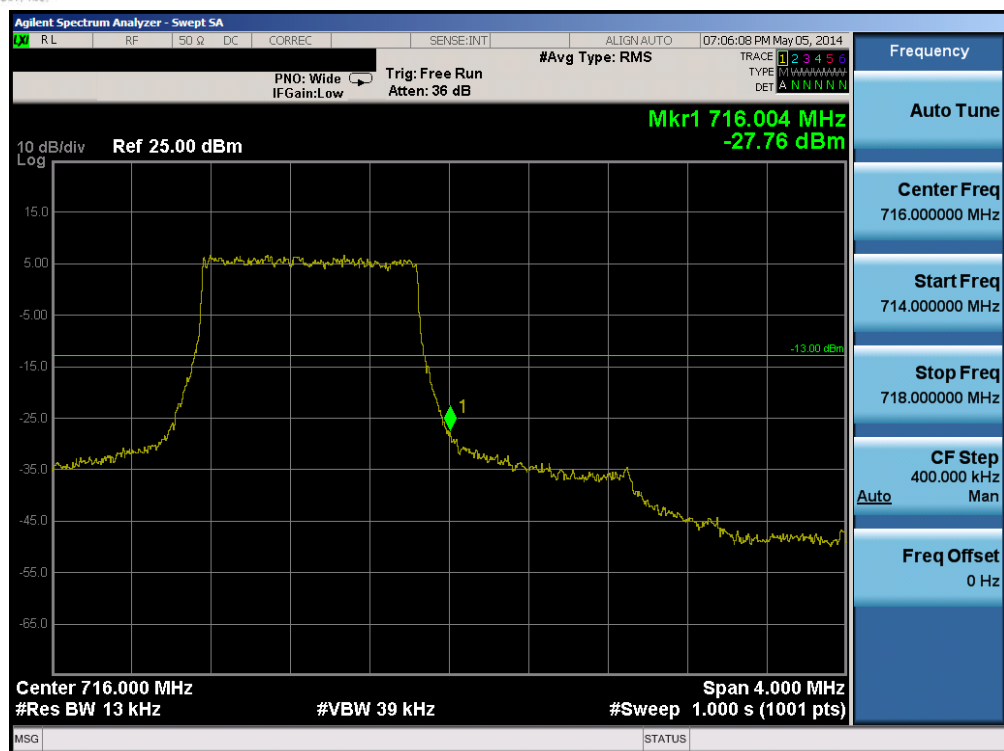
Plot 6-67. Upper Band Edge Plot (Band 12 – 1.4MHz QPSK – RB Size 6)
