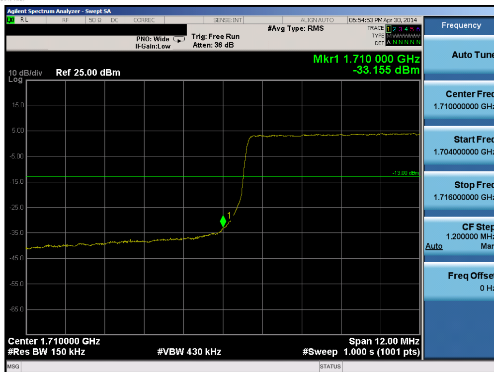
Plot 6-113. Lower Band Edge Plot (Band 4 – 15.0MHz QPSK – RB Size 75)
