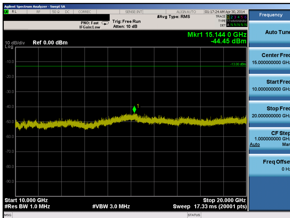
Plot 6-62. Conducted Spurious Plot (Band 2 – 20.0MHz QPSK – RB Size 1, RB Offset 0 – Mid Channel)
