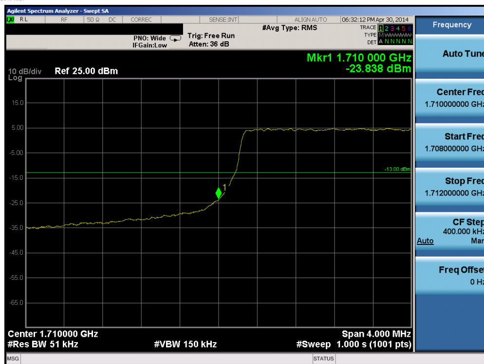
Plot 6-105. Lower Band Edge Plot (Band 4 – 5.0MHz QPSK – RB Size 25)
