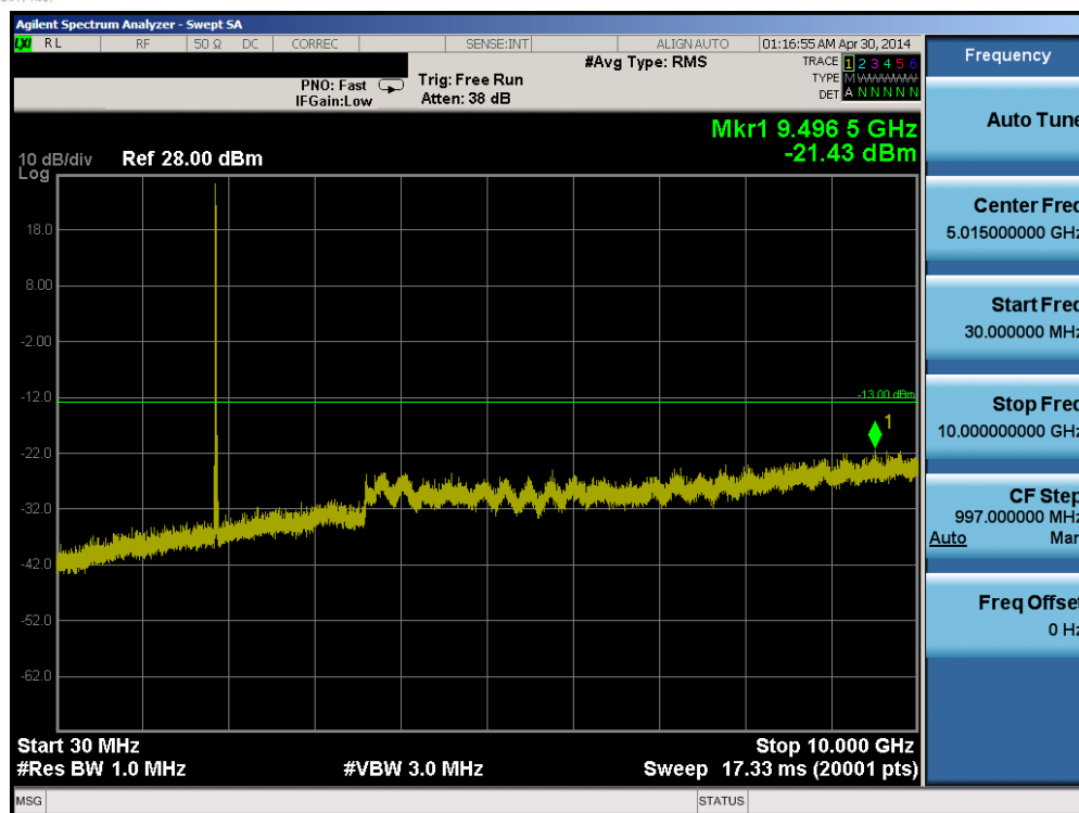
Plot 6-61. Conducted Spurious Plot (Band 2 – 20.0MHz QPSK – RB Size 1, RB Offset 0 – Mid Channel)
