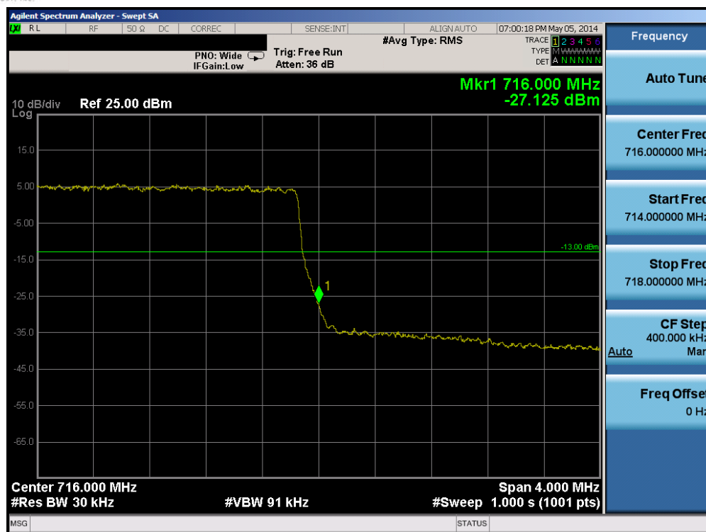
Plot 6-71. Upper Band Edge Plot (Band 12 – 3.0MHz QPSK – RB Size 15)
