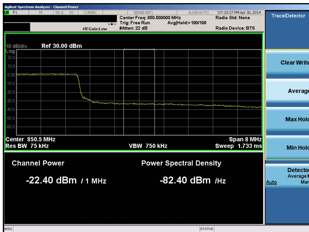
Plot 6-96. Upper Extended Band Edge Plot (Band 5 – 10.0MHz QPSK – RB Size 50)
