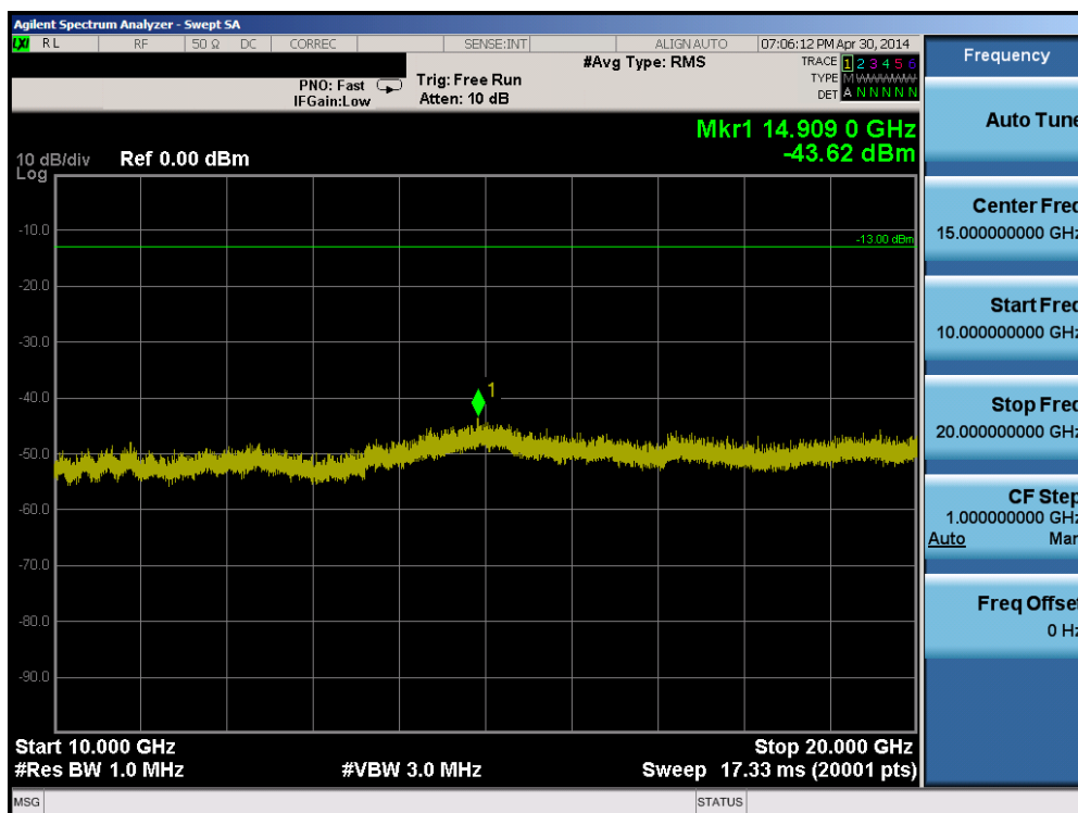
Plot 6-56. Conducted Spurious Plot (Band 4 – 20.0MHz QPSK – RB Size 1, RB Offset 0 – Mid Channel)
