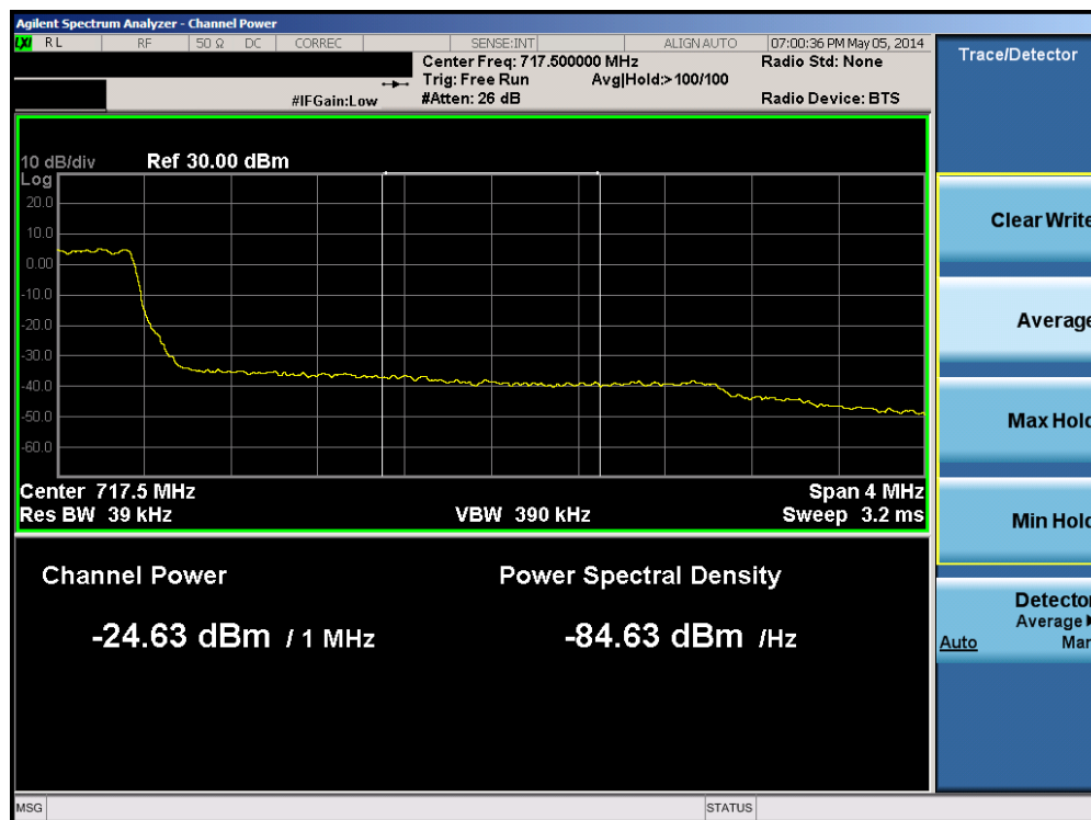
Plot 6-72. Upper Extended Band Edge Plot (Band 12 – 3.0MHz QPSK – RB Size 15)
