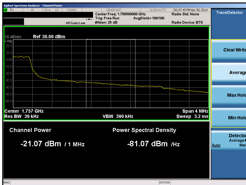
Plot 6-104. Upper Extended Band Edge Plot (Band 4 – 3.0MHz QPSK – RB Size 15)
