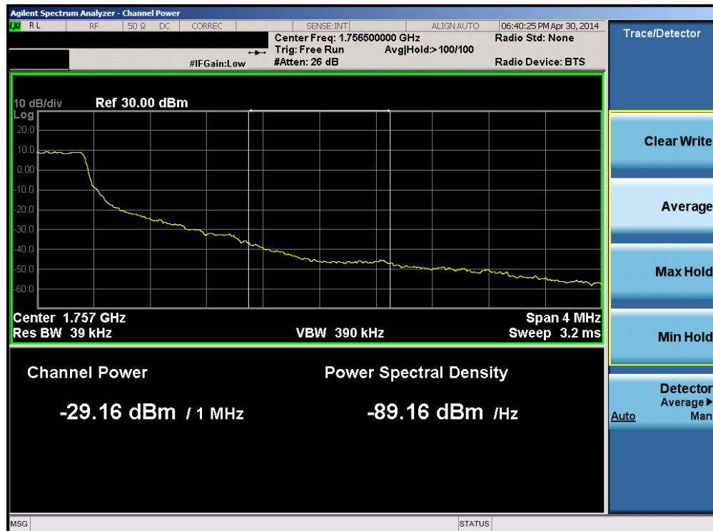
Plot 6-100. Upper Extended Band Edge Plot (Band 4 – 1.4MHz QPSK – RB Size 6)
