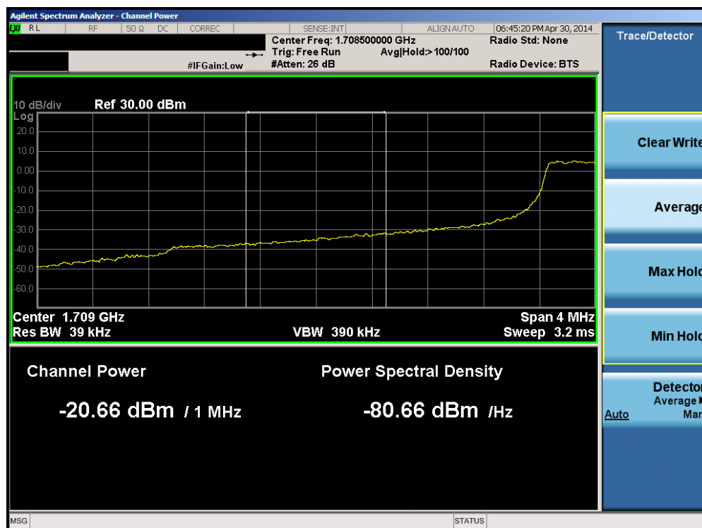
Plot 6-102. Lower Extended Band Edge Plot (Band 4 – 3.0MHz QPSK – RB Size 15)
