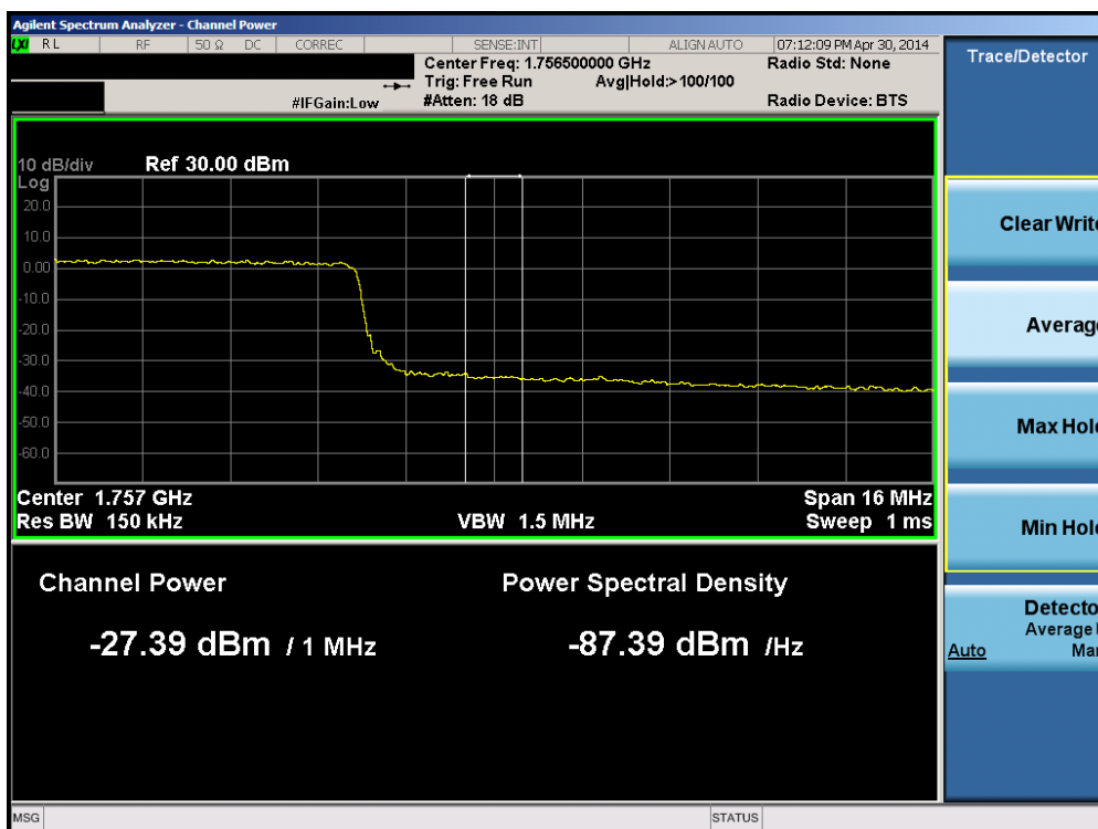
Plot 6-120. Upper Extended Band Edge Plot (Band 4 – 20.0MHz QPSK – RB Size 100)
