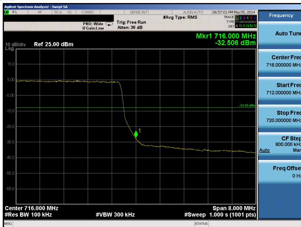
Plot 6-79. Upper Band Edge Plot (Band 12 – 10.0MHz QPSK – RB Size 50)
