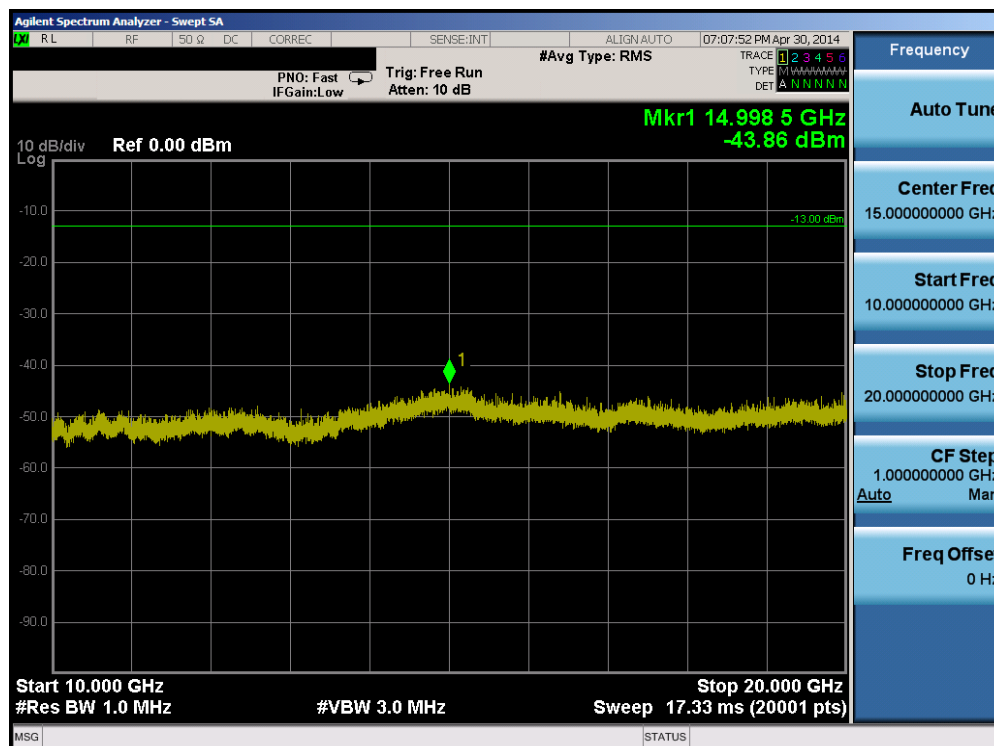
Plot 6-54. Conducted Spurious Plot (Band 4 – 20.0MHz QPSK – RB Size 1, RB Offset 0 – Low Channel)
