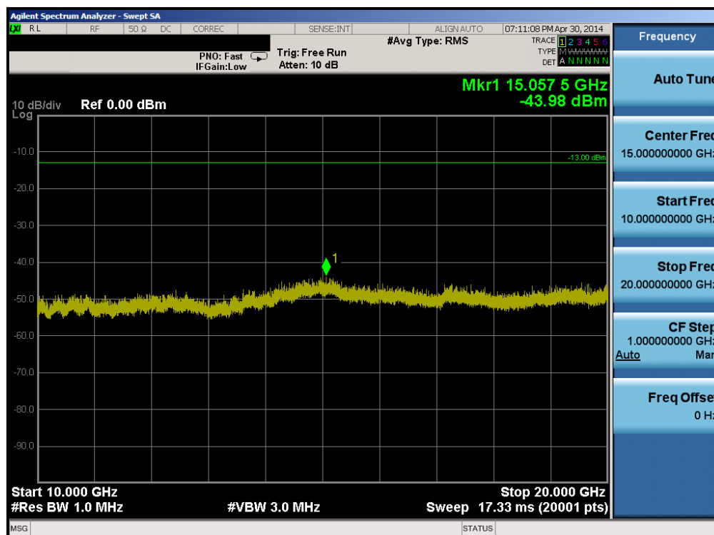
Plot 6-58. Conducted Spurious Plot (Band 4 – 20.0MHz QPSK – RB Size 1, RB Offset 0 – High Channel)
