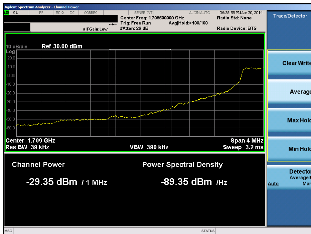
Plot 6-98. Lower Extended Band Edge Plot (Band 4 – 1.4MHz QPSK – RB Size 6)
