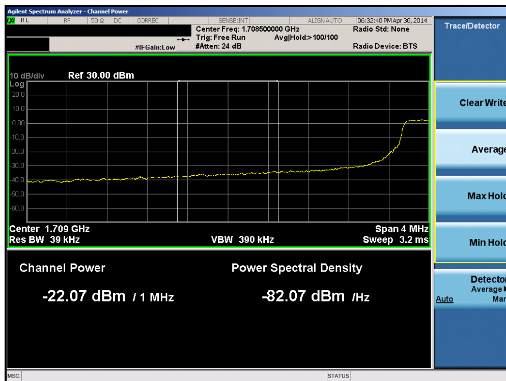
Plot 6-106. Lower Extended Band Edge Plot (Band 4 – 5.0MHz QPSK – RB Size 25)
