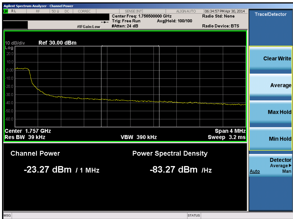
Plot 6-108. Upper Extended Band Edge Plot (Band 4 – 5.0MHz QPSK – RB Size 25)
