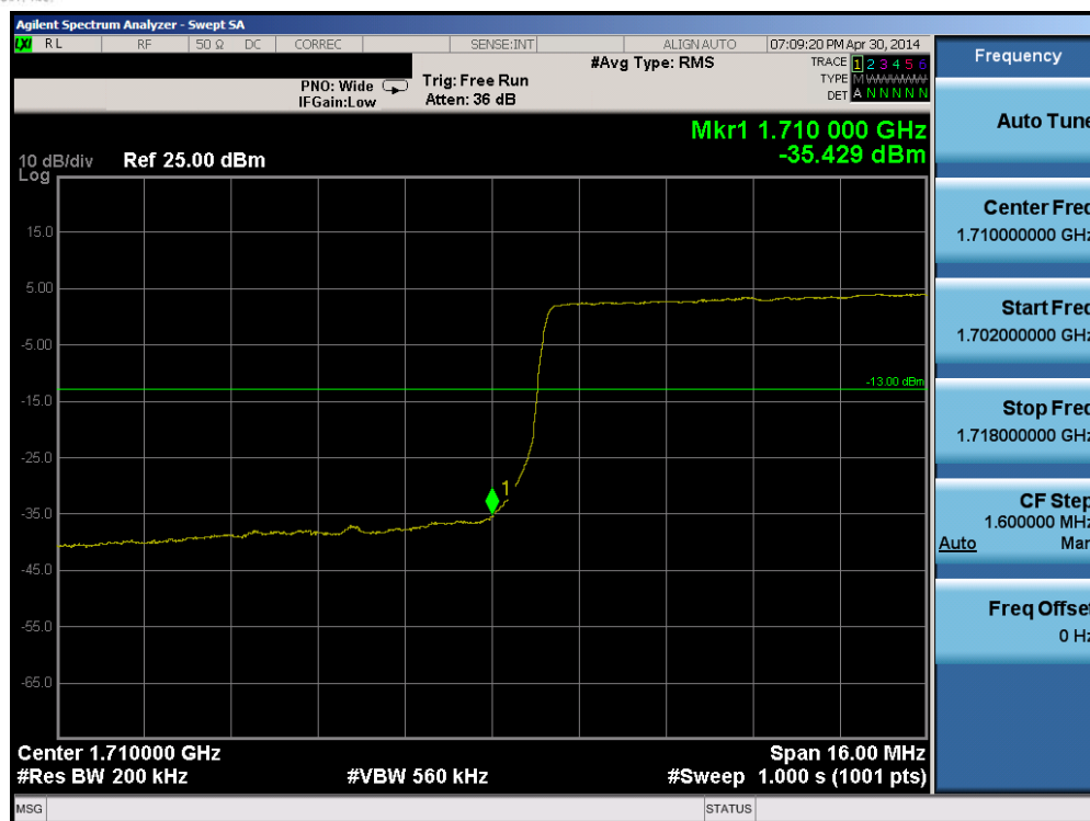
Plot 6-117. Lower Band Edge Plot (Band 4 – 20.0MHz QPSK – RB Size 100)
