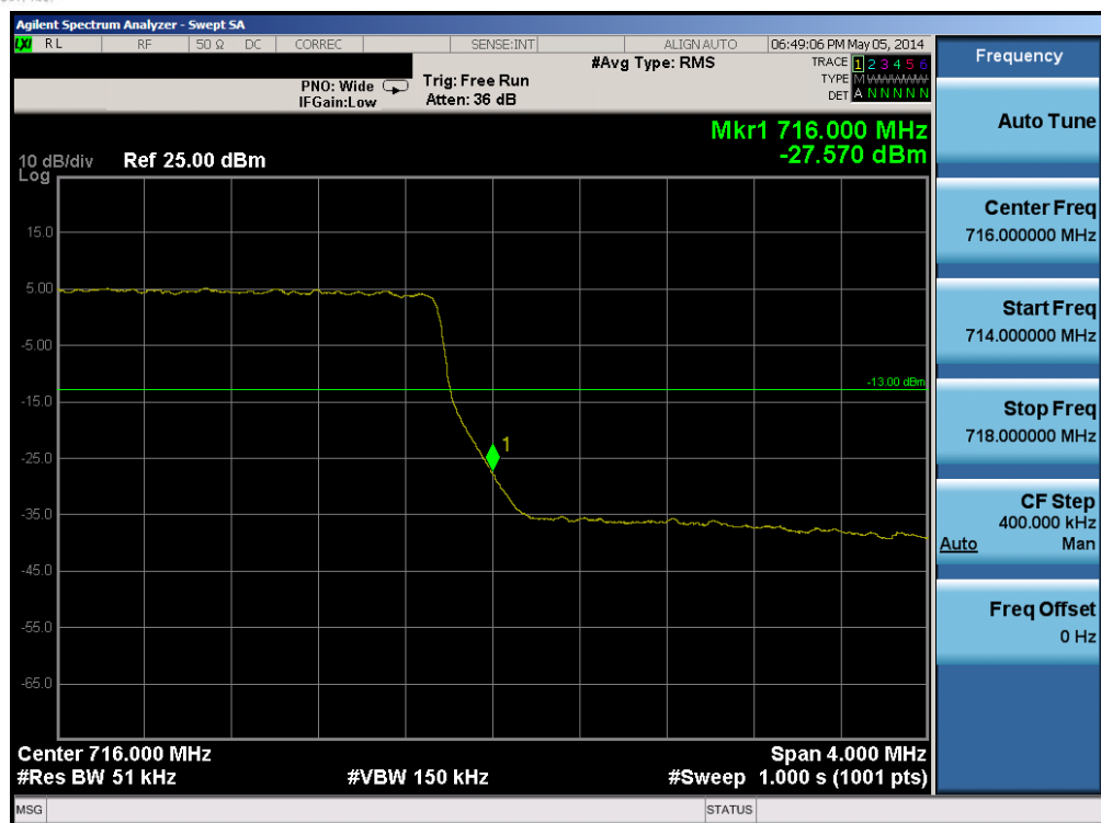
Plot 6-75. Upper Band Edge Plot (Band 12 – 5.0MHz QPSK – RB Size 25)
