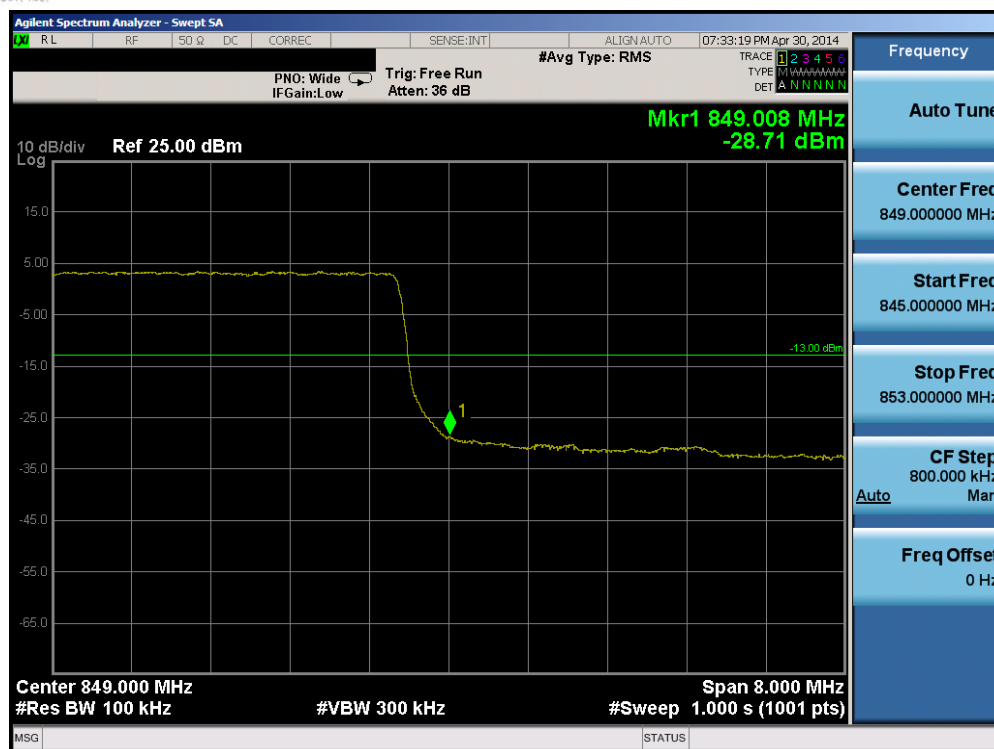
Plot 6-95. Upper Band Edge Plot (Band 5 – 10.0MHz QPSK – RB Size 50)
