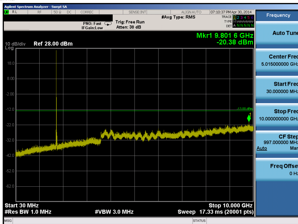
Plot 6-57. Conducted Spurious Plot (Band 4 – 20.0MHz QPSK – RB Size 1, RB Offset 0 – High Channel)
