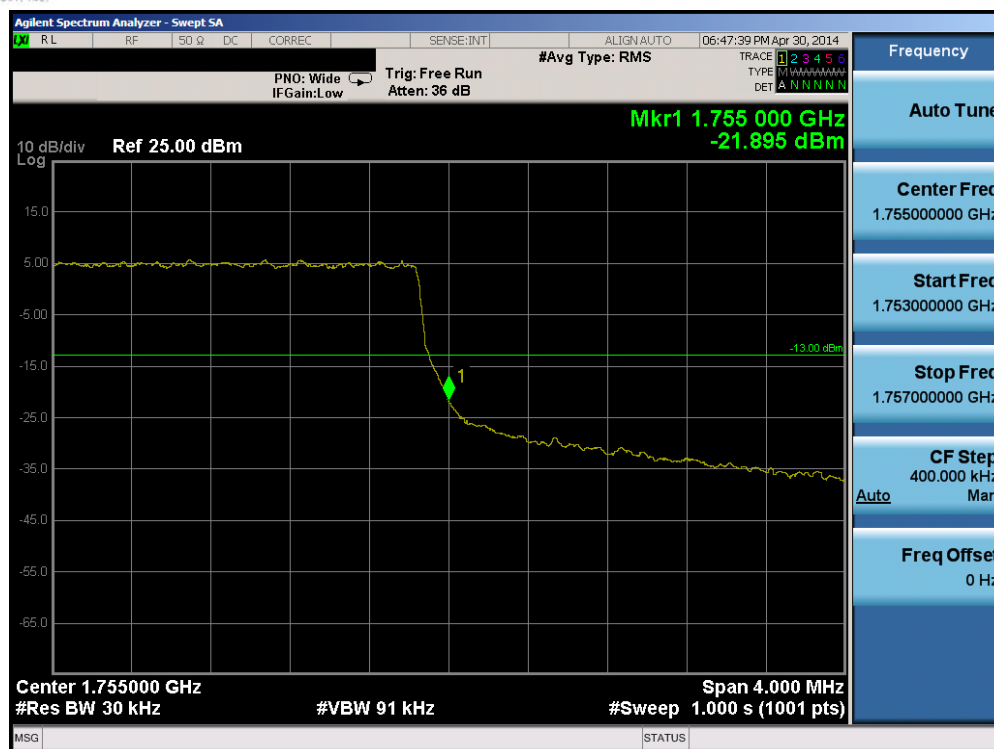
Plot 6-103. Upper Band Edge Plot (Band 4 – 3.0MHz QPSK – RB Size 15)
