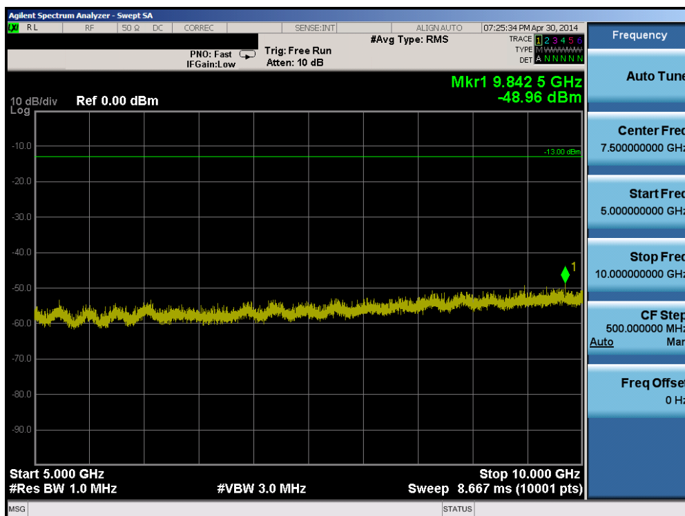
Plot 6-50. Conducted Spurious Plot (Band 5 – 10.0MHz QPSK – RB Size 1, RB Offset 0 – Mid Channel)
