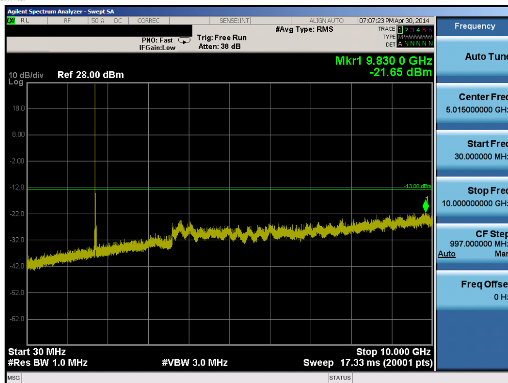
Plot 6-53. Conducted Spurious Plot (Band 4 – 20.0MHz QPSK – RB Size 1, RB Offset 0– Low Channel)
