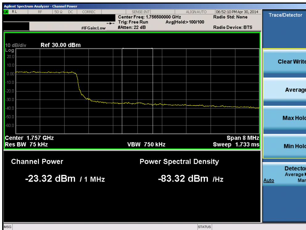
Plot 6-112. Upper Extended Band Edge Plot (Band 4 – 10.0MHz QPSK – RB Size 50)
