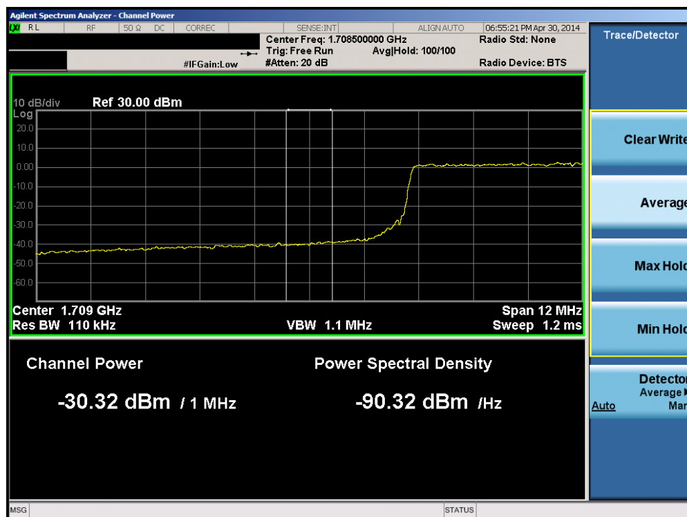
Plot 6-114. Lower Extended Band Edge Plot (Band 4 – 15.0MHz QPSK – RB Size 75)
