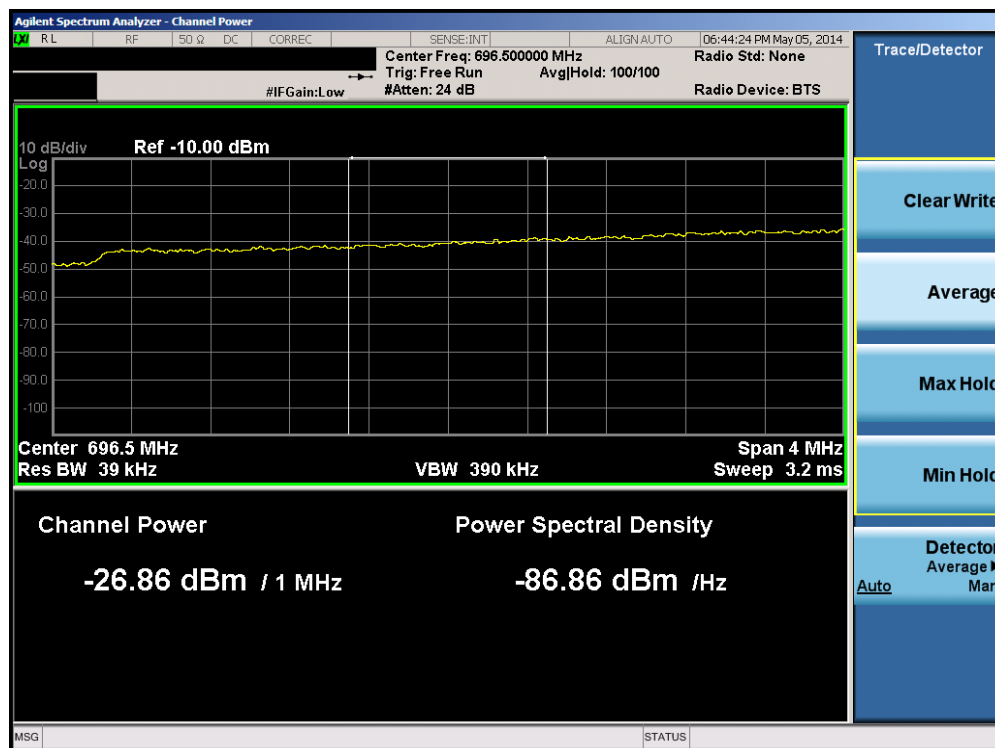
Plot 6-74. Lower Extended Band Edge Plot (Band 12 – 5.0MHz QPSK – RB Size 25)
