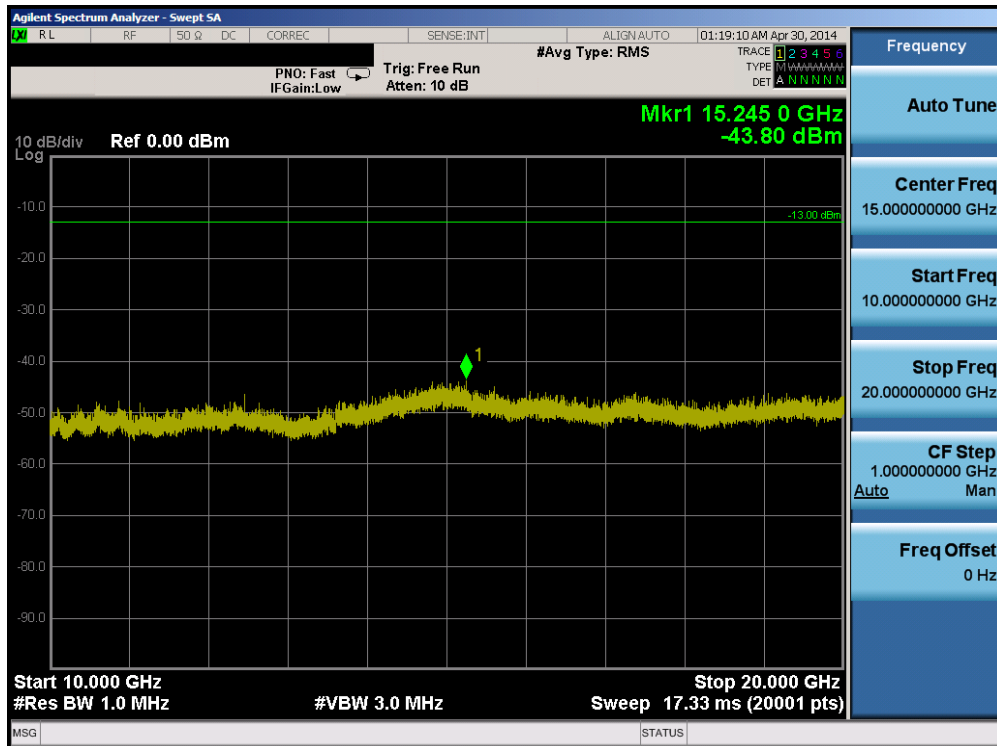
Plot 6-60. Conducted Spurious Plot (Band 2 – 20.0MHz QPSK – RB Size 1, RB Offset 0 – Low Channel)
