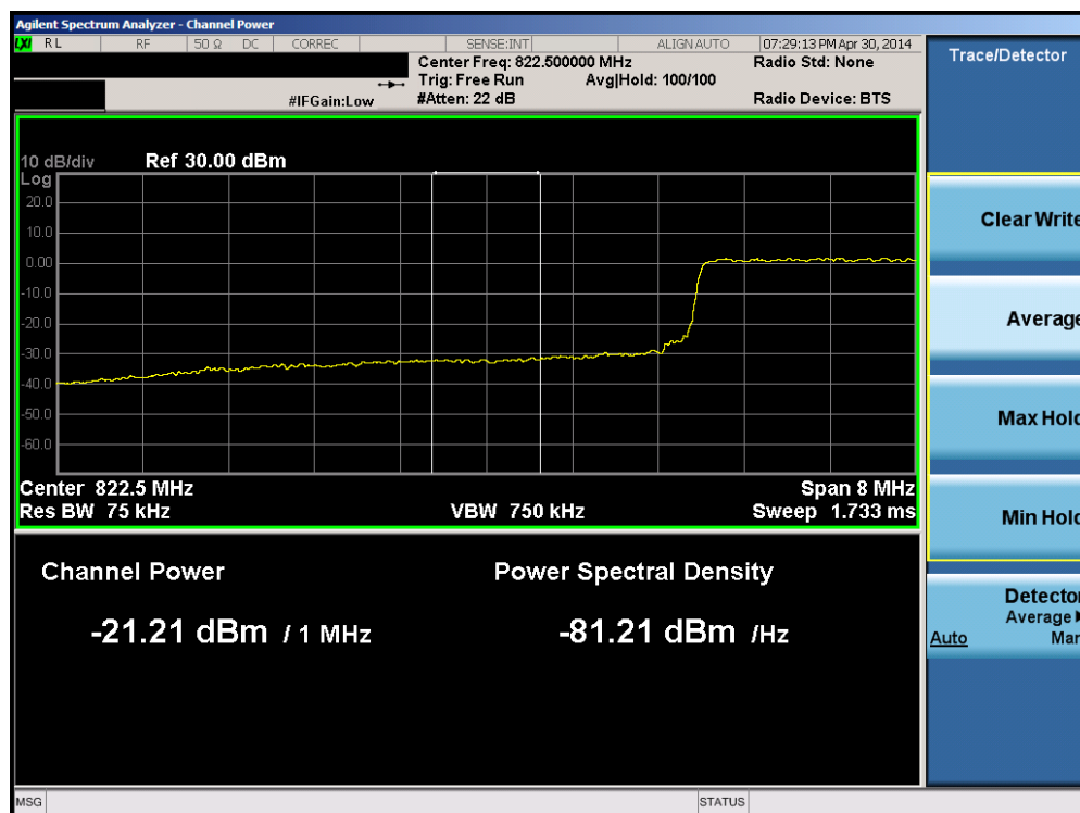
Plot 6-94. Lower Extended Band Edge Plot (Band 5 – 10.0MHz QPSK – RB Size 50)
