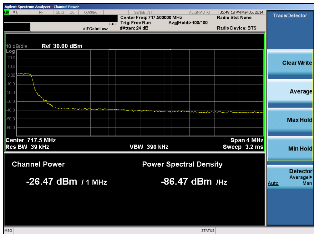
Plot 6-76. Upper Extended Band Edge Plot (Band 12 – 5.0MHz QPSK – RB Size 25)
