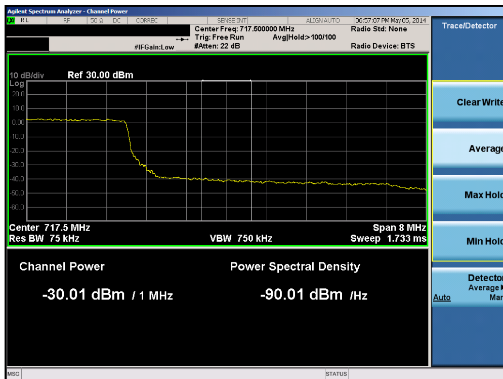
Plot 6-80. Upper Extended Band Edge Plot (Band 12 – 10.0MHz QPSK – RB Size 50)
