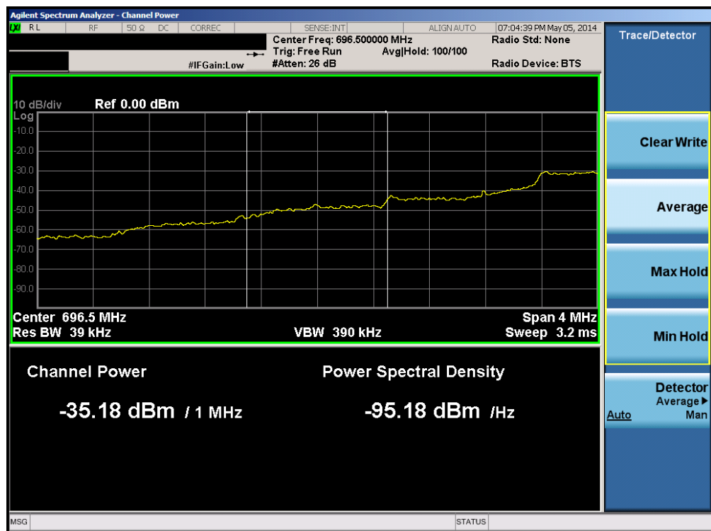
Plot 6-66. Lower Extended Band Edge Plot (Band 12 – 1.4MHz QPSK – RB Size 6)
