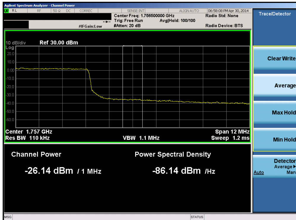
Plot 6-116. Upper Extended Band Edge Plot (Band 4 – 15.0MHz QPSK – RB Size 75)
