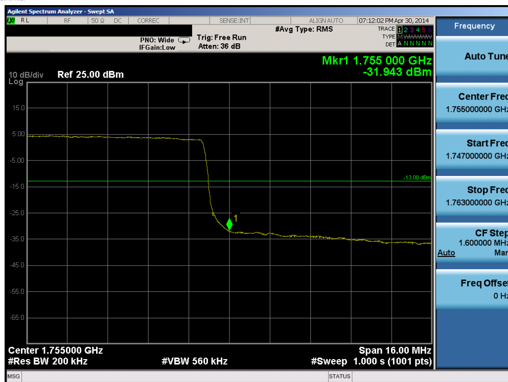
Plot 6-119. Upper Band Edge Plot (Band 4 – 20.0MHz QPSK – RB Size 100)
