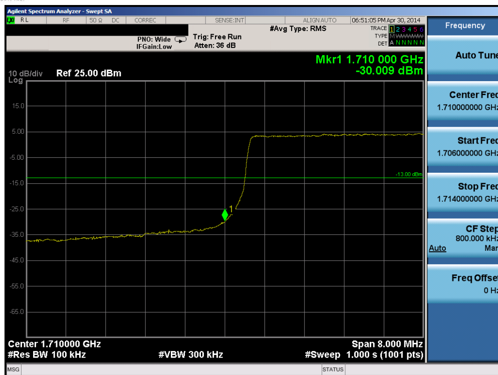
Plot 6-109. Lower Band Edge Plot (Band 4 – 10.0MHz QPSK – RB Size 50)
