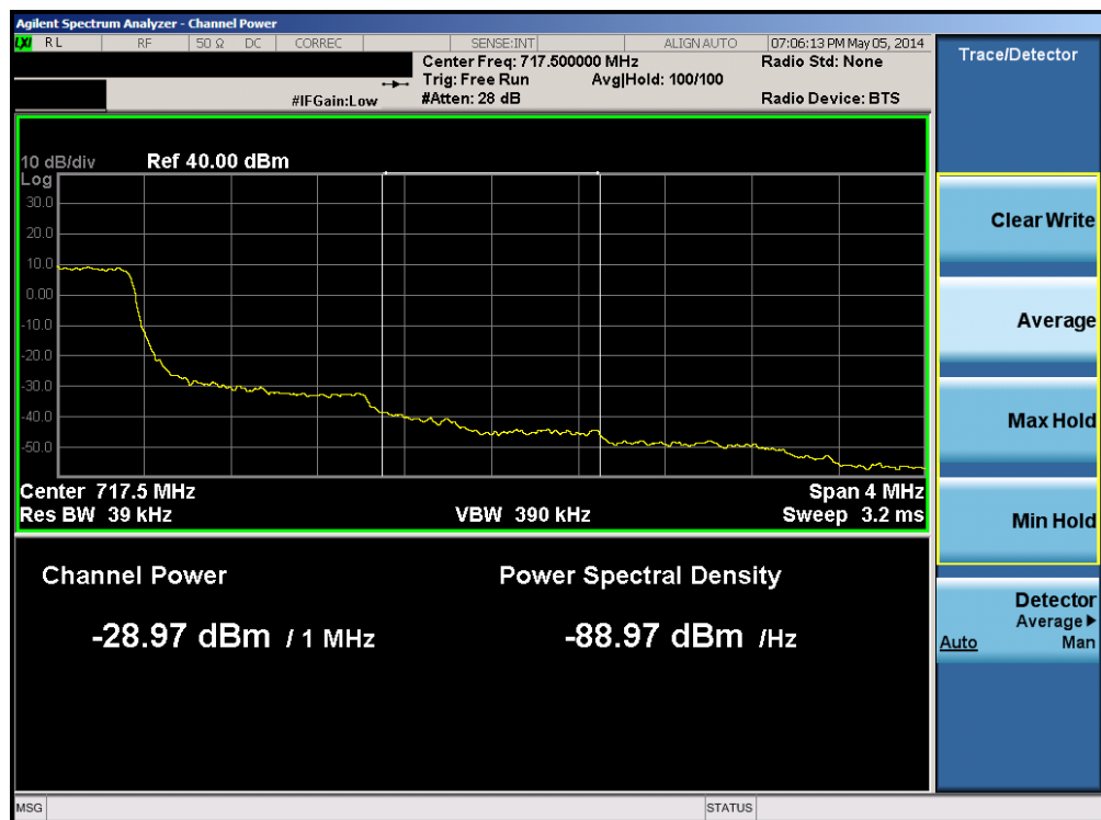
Plot 6-68. Upper Extended Band Edge Plot (Band 12 – 1.4MHz QPSK – RB Size 6)
