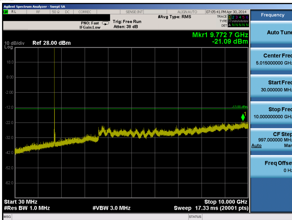
Plot 6-55. Conducted Spurious Plot (Band 4 – 20.0MHz QPSK – RB Size 1, RB Offset 0 – Mid Channel)
