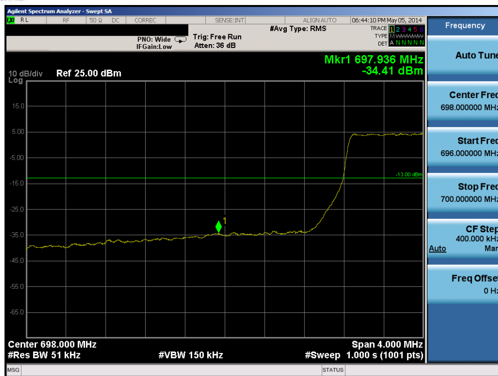
Plot 6-73. Lower Band Edge Plot (Band 12 – 5.0MHz QPSK – RB Size 25)
