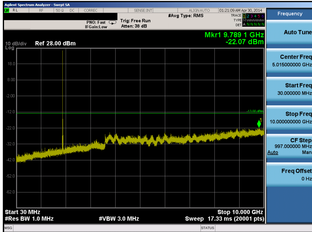
Plot 6-63. Conducted Spurious Plot (Band 2 – 20.0MHz QPSK – RB Size 1, RB Offset 0 – High Channel)
