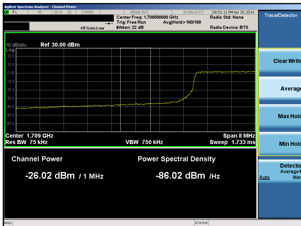
Plot 6-110. Lower Extended Band Edge Plot (Band 4 – 10.0MHz QPSK – RB Size 50)
