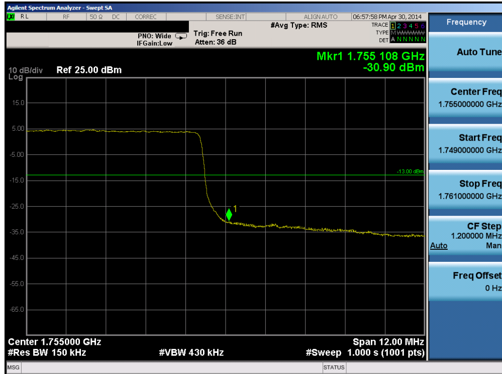
Plot 6-115. Upper Band Edge Plot (Band 4 – 15.0MHz QPSK – RB Size 75)
