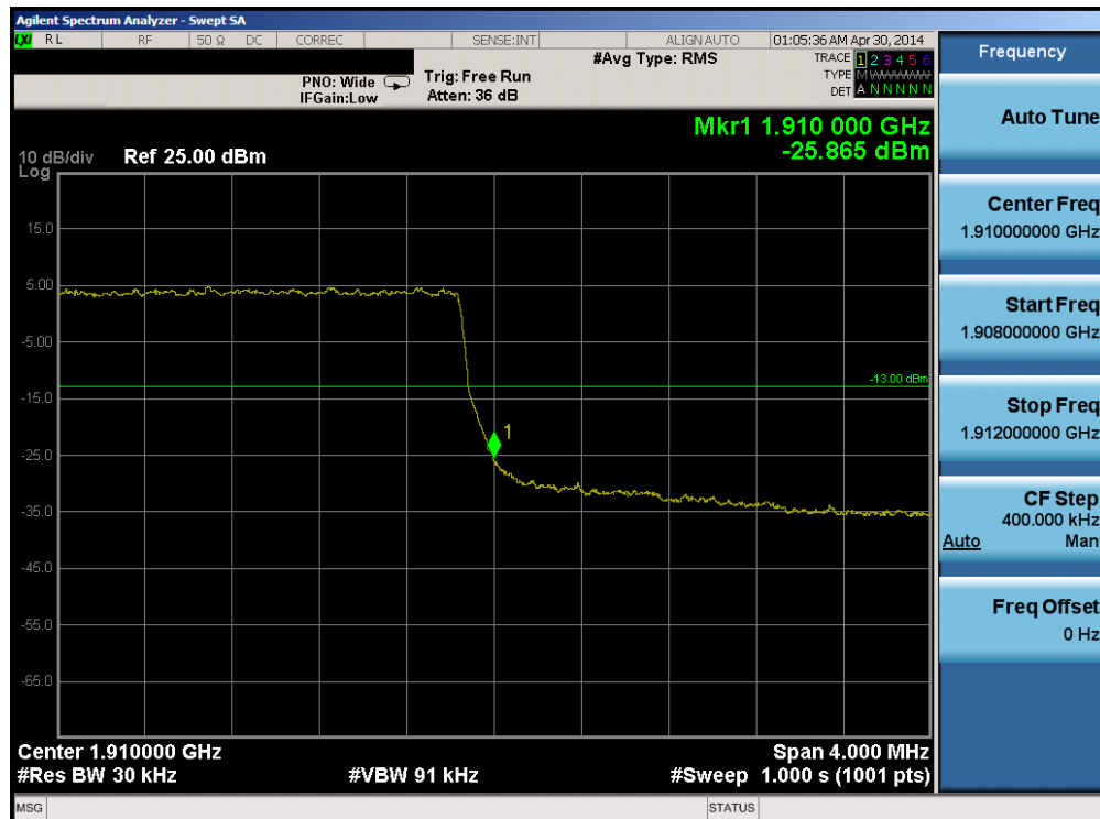
Plot 6-127. Upper Band Edge Plot (Band 2 – 3.0MHz QPSK – RB Size 15)
