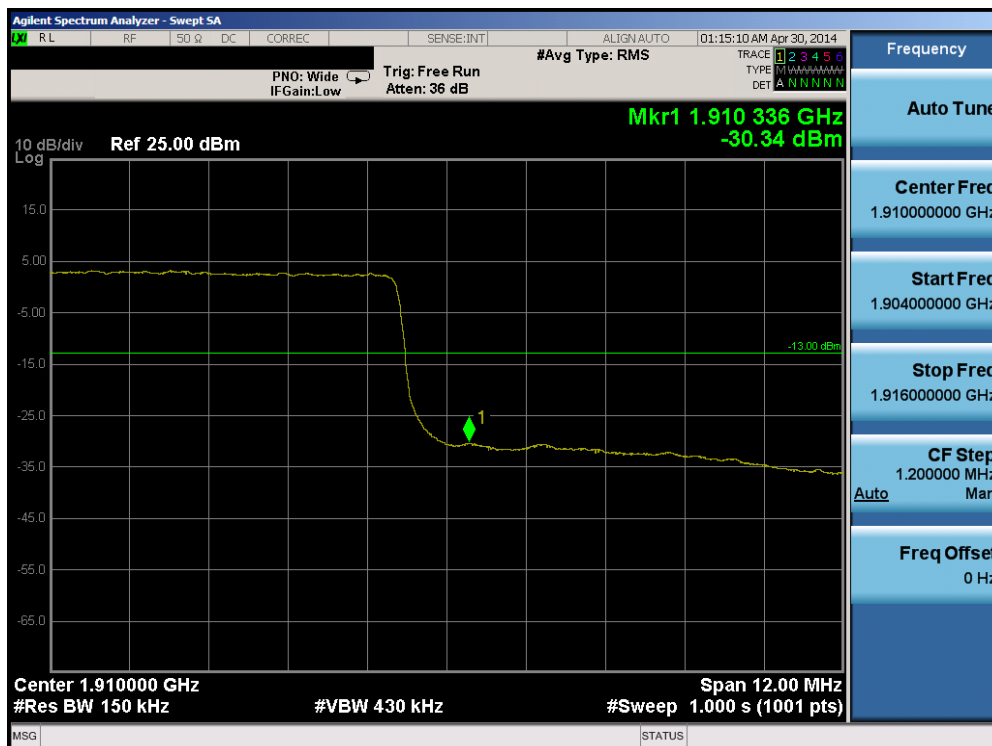
Plot 6-139. Upper Band Edge Plot (Band 2 – 15.0MHz QPSK – RB Size 75)
