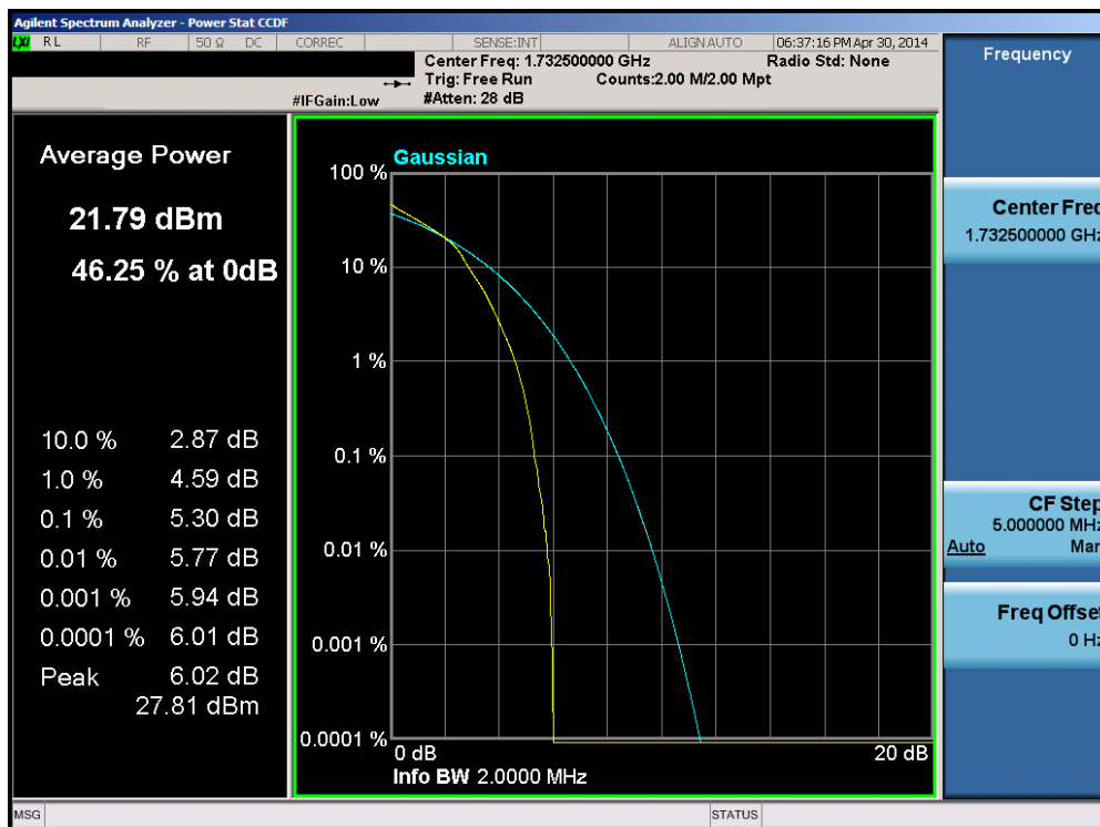
Plot 6-146. PAR Plot (Band 4 – 1.4MHz 16-QAM – RB Size 6)
