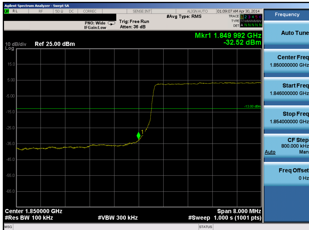
Plot 6-133. Lower Band Edge Plot (Band 2 – 10.0MHz QPSK – RB Size 50)
