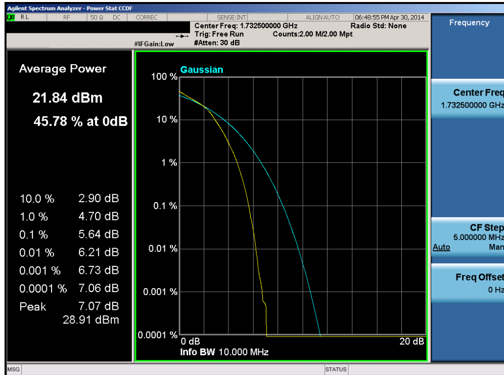
Plot 6-152. PAR Plot (Band 4 – 10.0MHz 16-QAM – RB Size 50)
