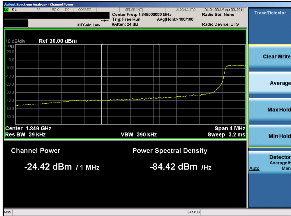
Plot 6-126. Lower Extended Band Edge Plot (Band 2 – 3.0MHz QPSK – RB Size 15)
