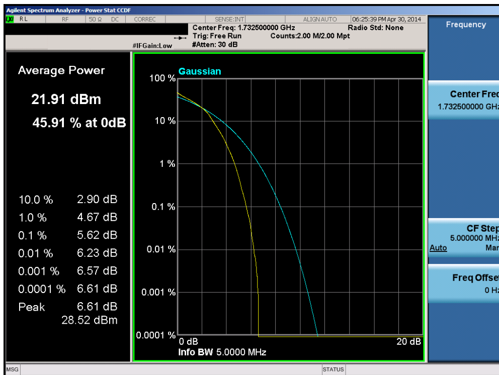
Plot 6-150. PAR Plot (Band 4 – 5.0MHz 16-QAM – RB Size 25)
