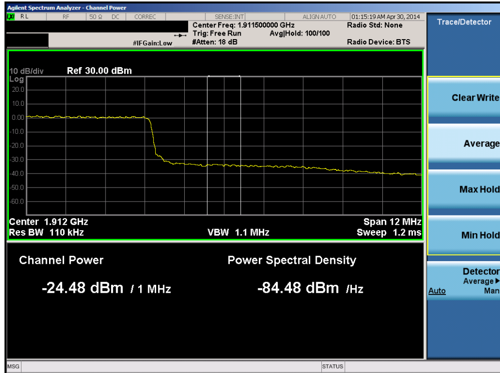
Plot 6-140. Upper Extended Band Edge Plot (Band 2 – 15.0MHz QPSK – RB Size 75)
