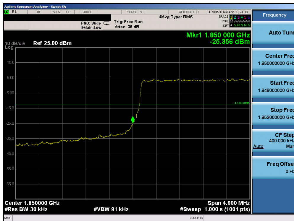
Plot 6-125. Lower Band Edge Plot (Band 2 – 3.0MHz QPSK – RB Size 15)
