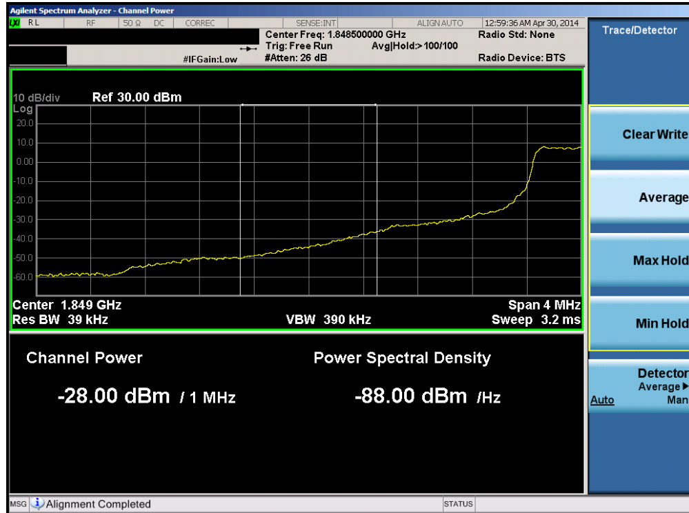
Plot 6-122. Lower Extended Band Edge Plot (Band 2 – 1.4MHz QPSK – RB Size 6)
