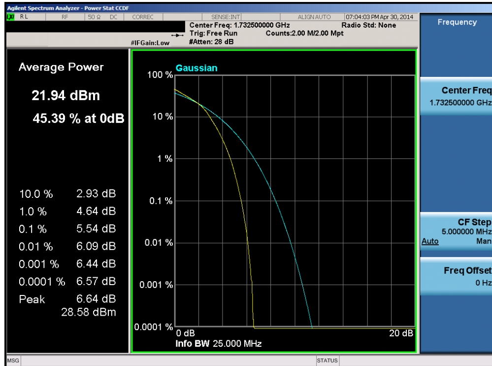
Plot 6-156. PAR Plot (Band 4 – 20.0MHz 16-QAM – RB Size 100)
