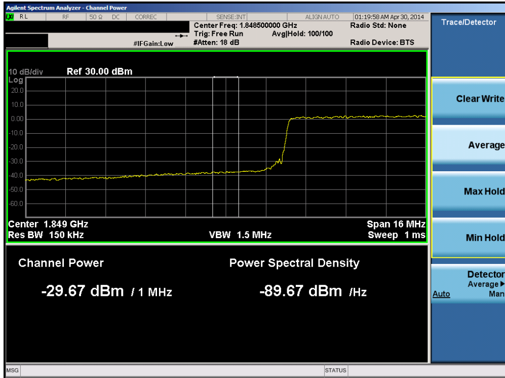
Plot 6-142. Lower Extended Band Edge Plot (Band 2 – 20.0MHz QPSK – RB Size 100)
