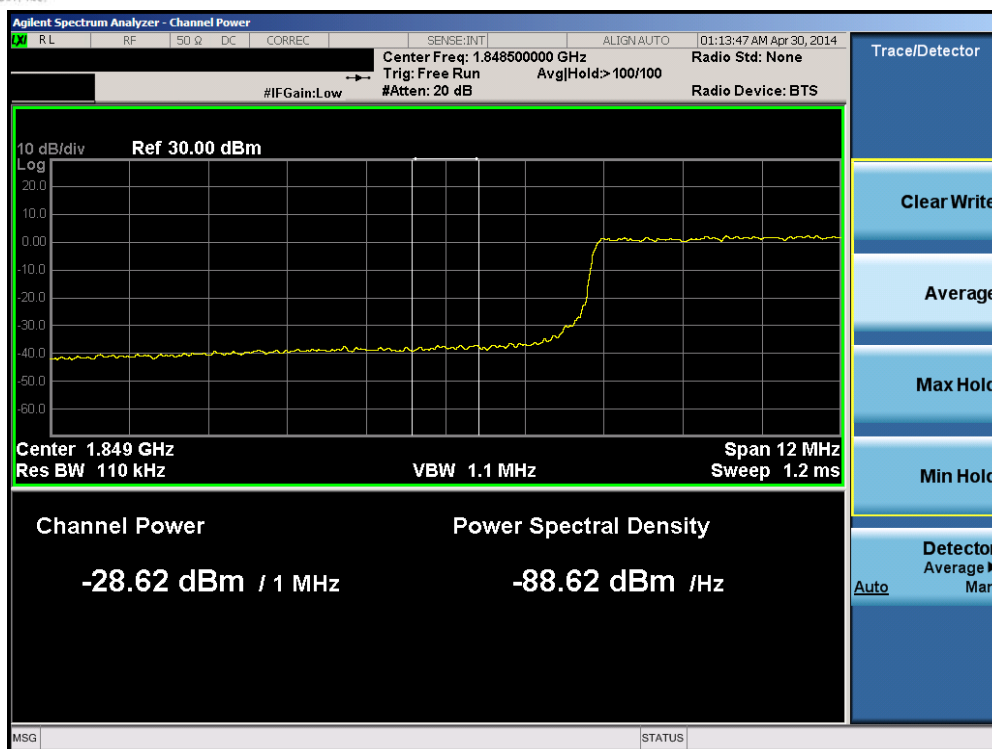
Plot 6-138. Lower Extended Band Edge Plot (Band 2 – 15.0MHz QPSK – RB Size 75)
