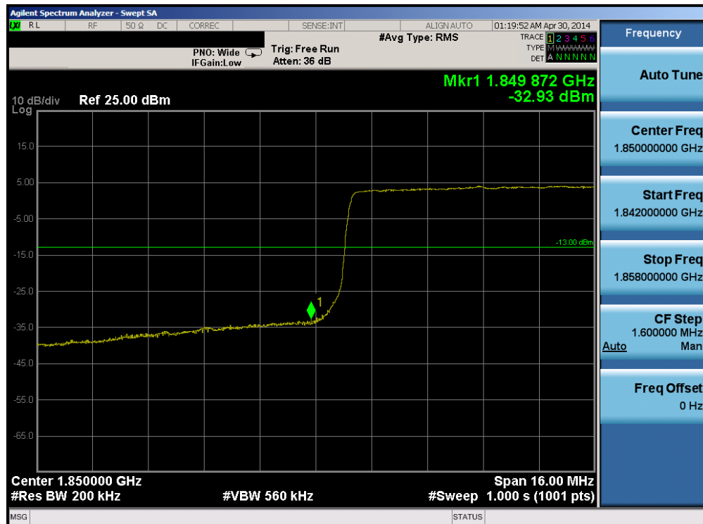
Plot 6-141. Lower Band Edge Plot (Band 2 – 20.0MHz QPSK – RB Size 100)
