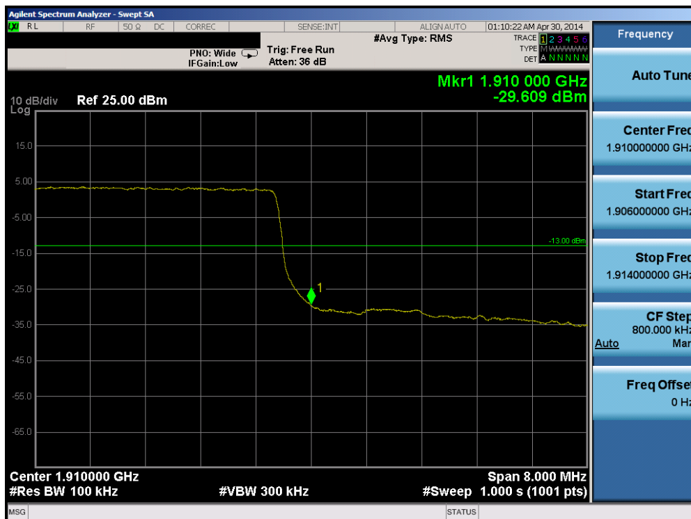
Plot 6-135. Upper Band Edge Plot (Band 2 – 10.0MHz QPSK – RB Size 50)
