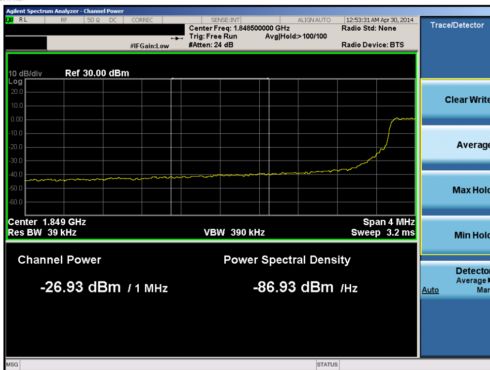
Plot 6-130. Lower Extended Band Edge Plot (Band 2 – 5.0MHz QPSK – RB Size 25)
