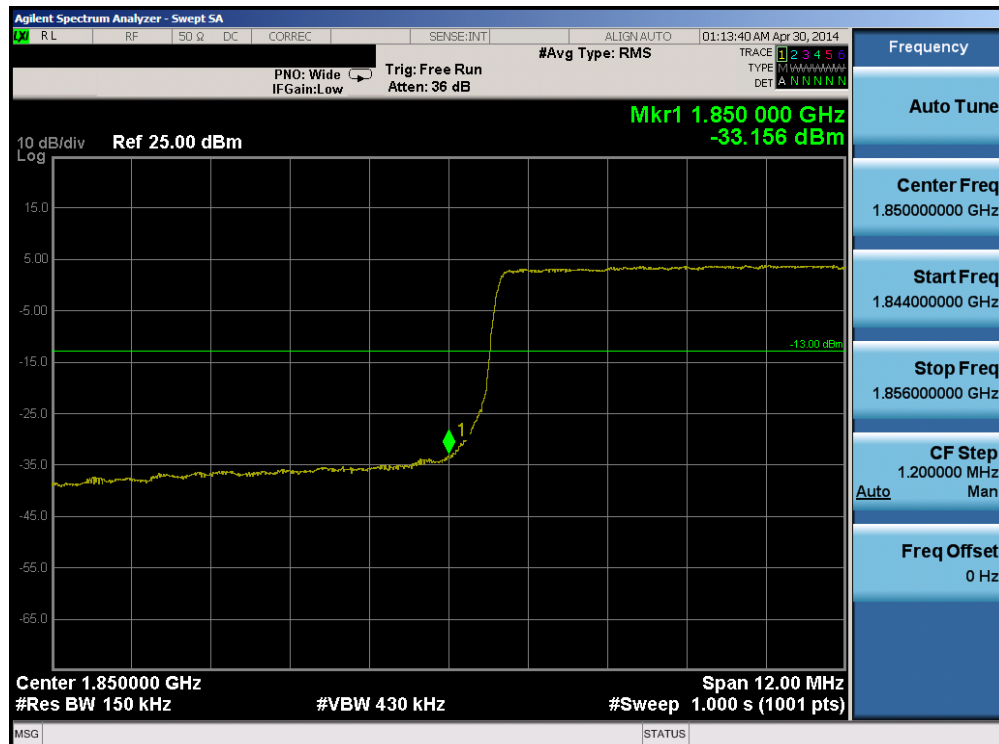
Plot 6-137. Lower Band Edge Plot (Band 2 – 15.0MHz QPSK – RB Size 75)
