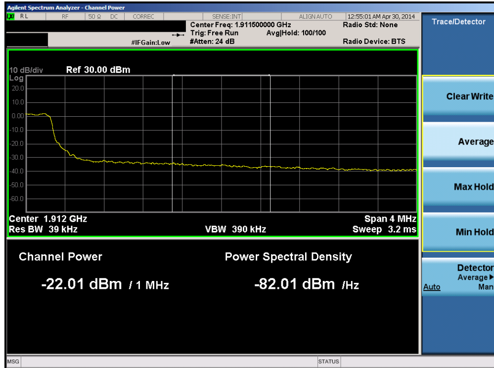
Plot 6-132. Upper Extended Band Edge Plot (Band 2 – 5.0MHz QPSK – RB Size 25)
