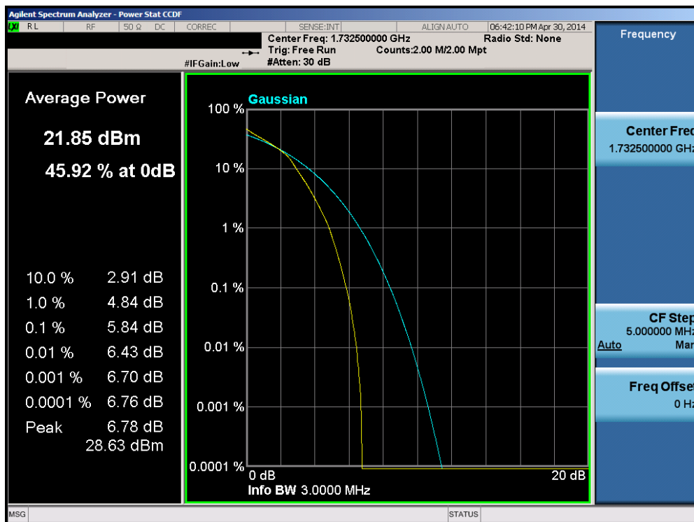
Plot 6-148. PAR Plot (Band 4 – 3.0MHz 16-QAM – RB Size 15)
