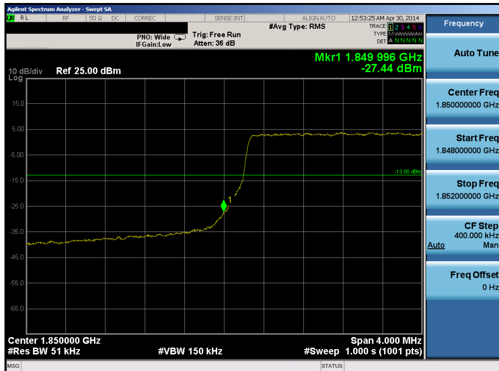
Plot 6-129. Lower Band Edge Plot (Band 2 – 5.0MHz QPSK – RB Size 25)
