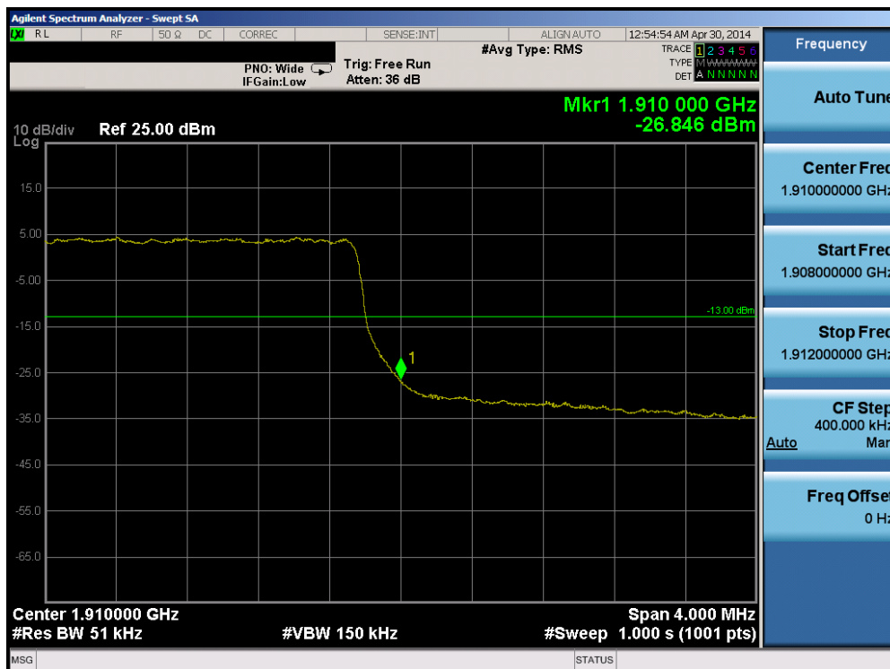
Plot 6-131. Upper Band Edge Plot (Band 2 – 5.0MHz QPSK – RB Size 25)
