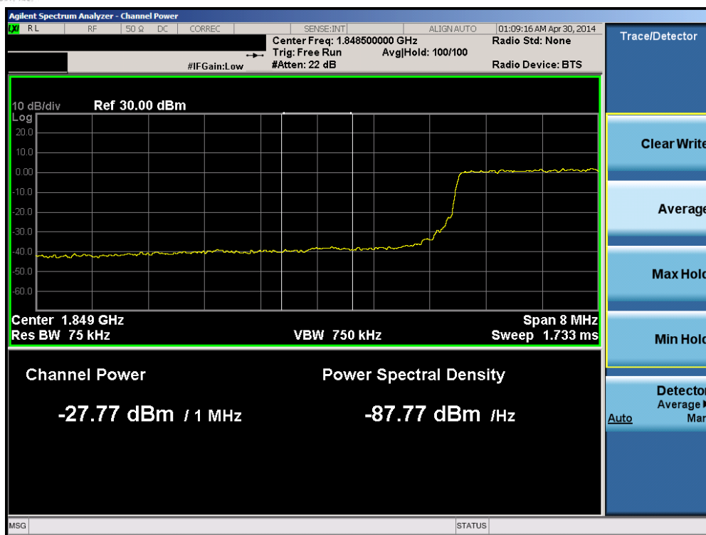
Plot 6-134. Lower Extended Band Edge Plot (Band 2 – 10.0MHz QPSK – RB Size 50)
