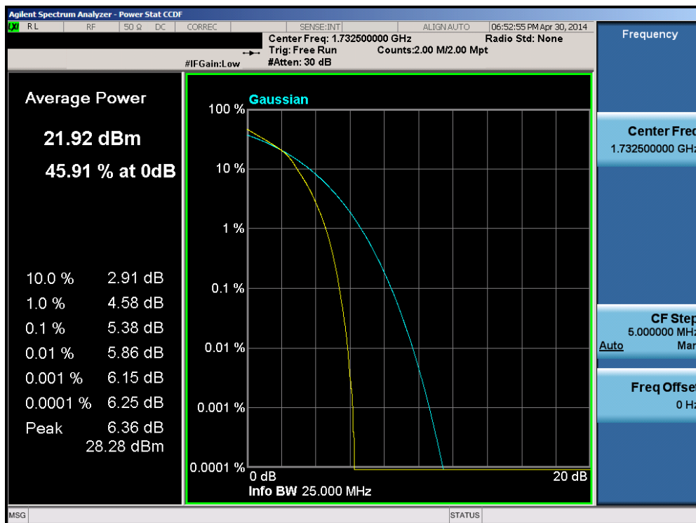
Plot 6-154. PAR Plot (Band 4 – 15.0MHz 16-QAM – RB Size 75)
