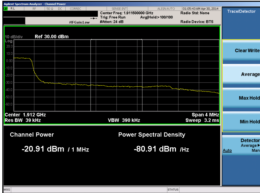
Plot 6-128. Upper Extended Band Edge Plot (Band 2 – 3.0MHz QPSK – RB Size 15)
