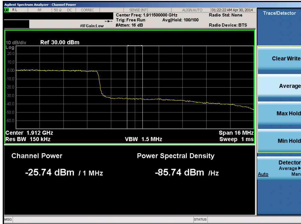
Plot 6-144. Upper Extended Band Edge Plot (Band 2 – 20.0MHz QPSK – RB Size 100)
