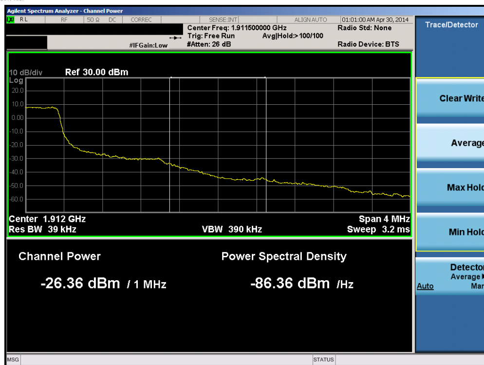
Plot 6-124. Upper Extended Band Edge Plot (Band 2 – 1.4MHz QPSK – RB Size 6)
