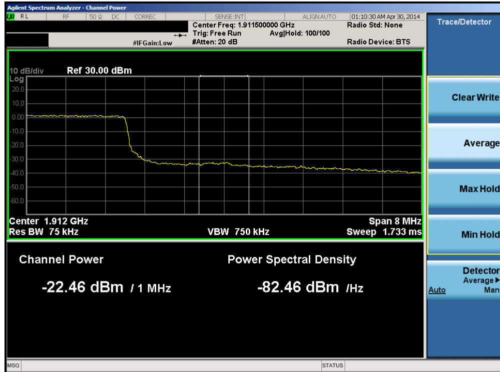
Plot 6-136. Upper Extended Band Edge Plot (Band 2 – 10.0MHz QPSK – RB Size 50)
