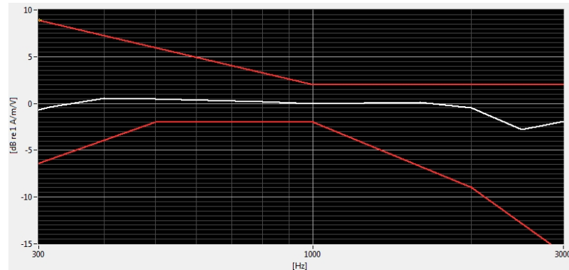
Figure 7-1 Axial Frequency Response
