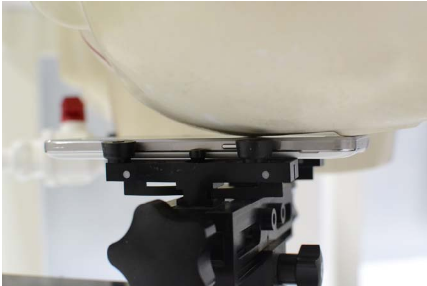
SAR Test Setup Photo 3: Left Cheek
