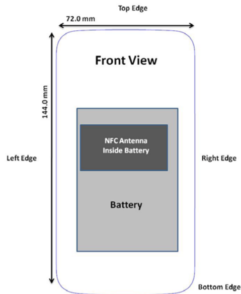
Figure F-2 NFC Antenna Location
