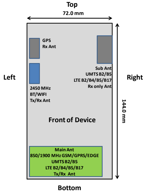
Figure F-1 DUT Antenna Locations
