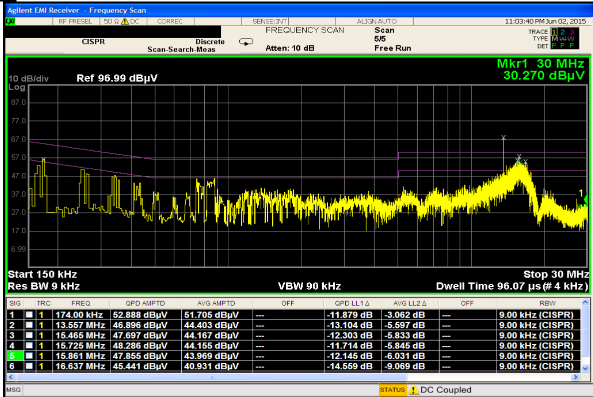
Plot 7-2. Line-Conducted Test Plot (N)
