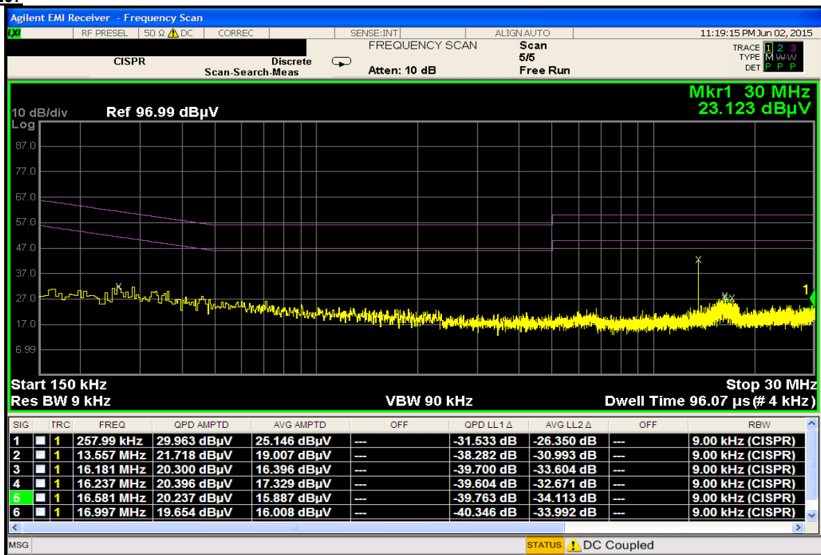
Plot 7-1. Line-Conducted Test Plot (L1)
