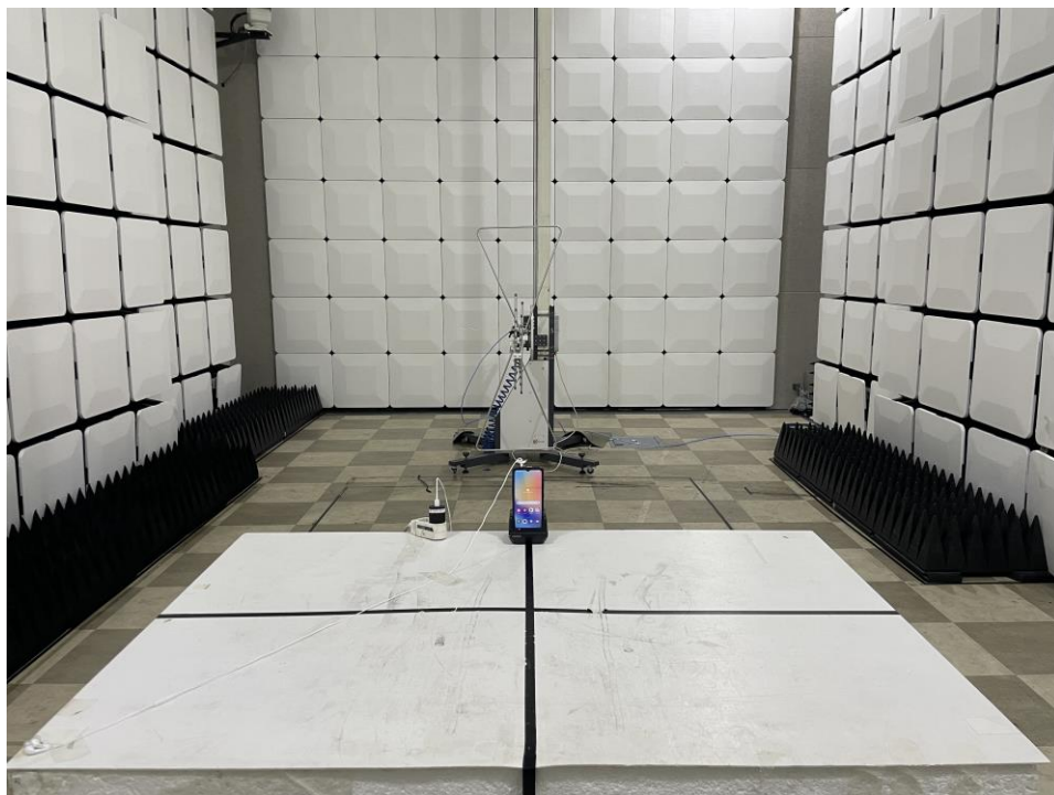
[EUT+TA+Earphone+Cradle]
