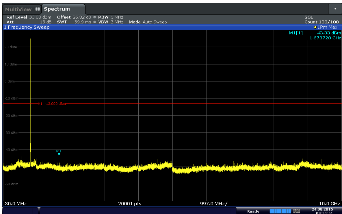
Plot 6-9. Conducted Spurious Plot (Band 5–1.4MHz–QPSK–RB Size 1–RB Offset 5–Ch.20407)
