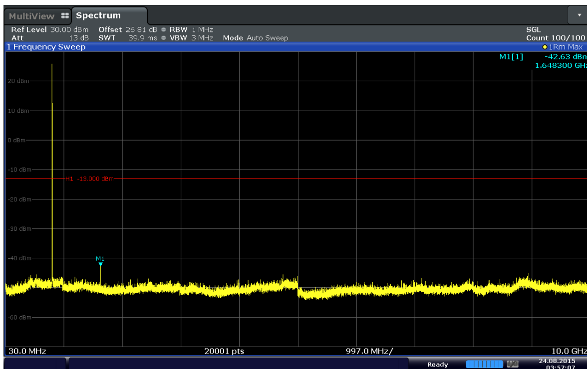
Plot 6-12. Conducted Spurious Plot (Band 5–3.0MHz–QPSK–RB Size 1–RB Offset 0– Ch.20415)
