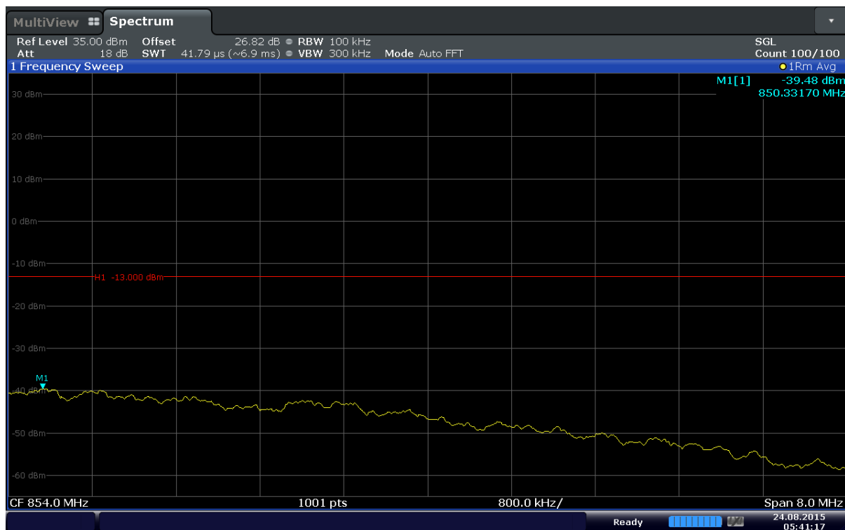
Plot 6-32. Extended Upper Band Edge Plot (Band 5 – 5.0MHz – QPSK – RB Size 25)
