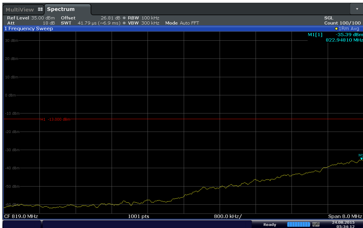
Plot 6-26. Extended Lower Band Edge Plot (Band 5 – 3.0MHz – QPSK – RB Size 15)
