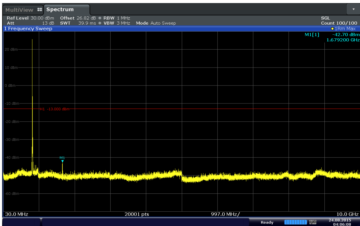
Plot 6-20. Conducted Spurious Plot (Band 5–10.0MHz–QPSK–RB Size 1–RB Offset 0– Ch.20600)
