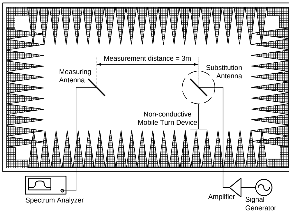
Figure 6-7. Test Instruments & Measurement Setup
