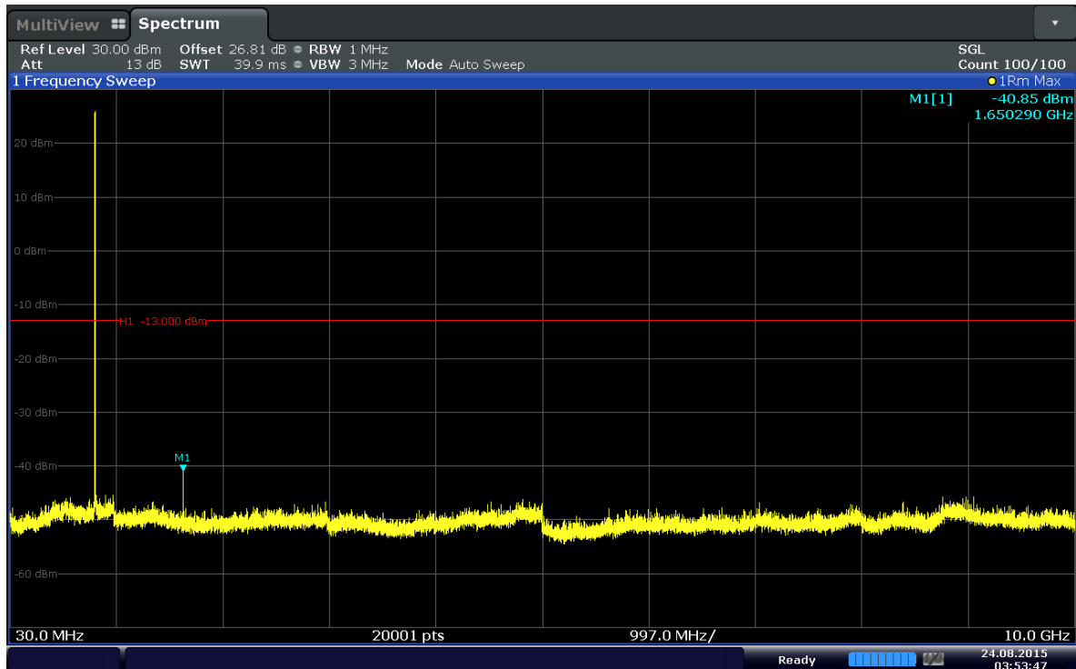
Plot 6-9. Conducted Spurious Plot (Band 5–1.4MHz–QPSK–RB Size 1–RB Offset 5–Ch.20407)
