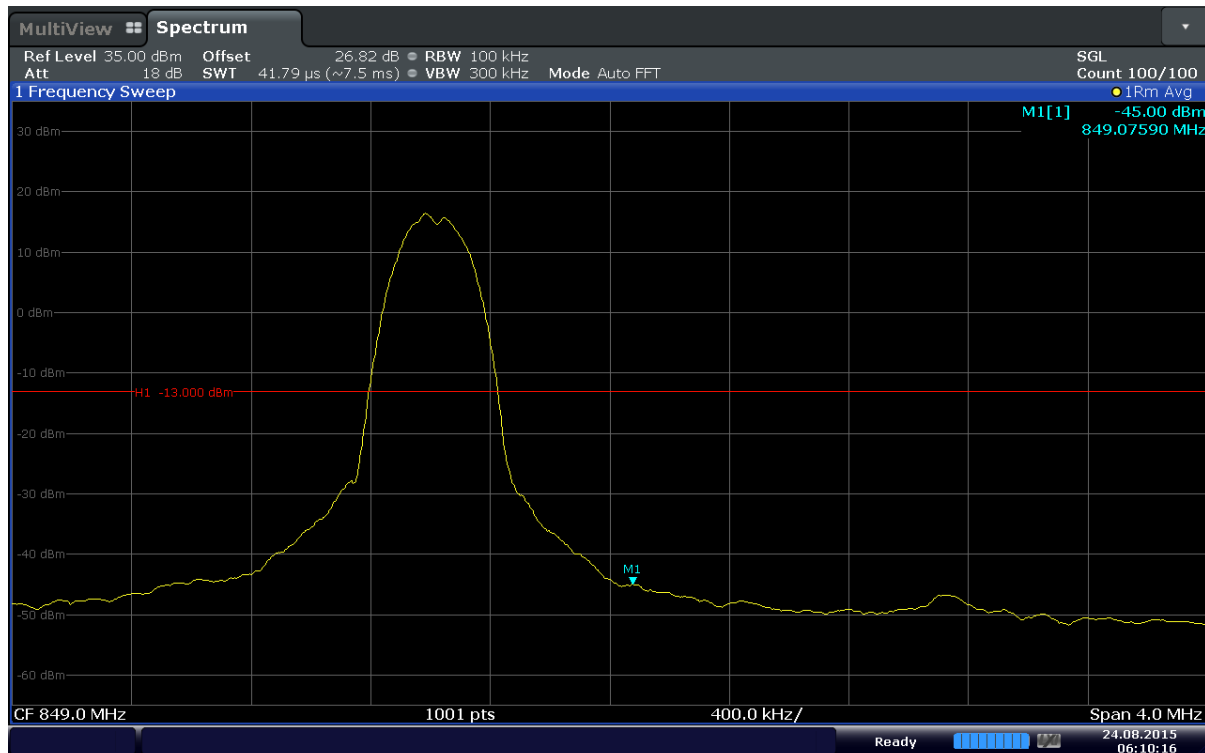
Plot 6-36. Upper Band Edge Plot (Band 5 – 10.0MHz – QPSK – RB Size 1 – RB Offset 49)
