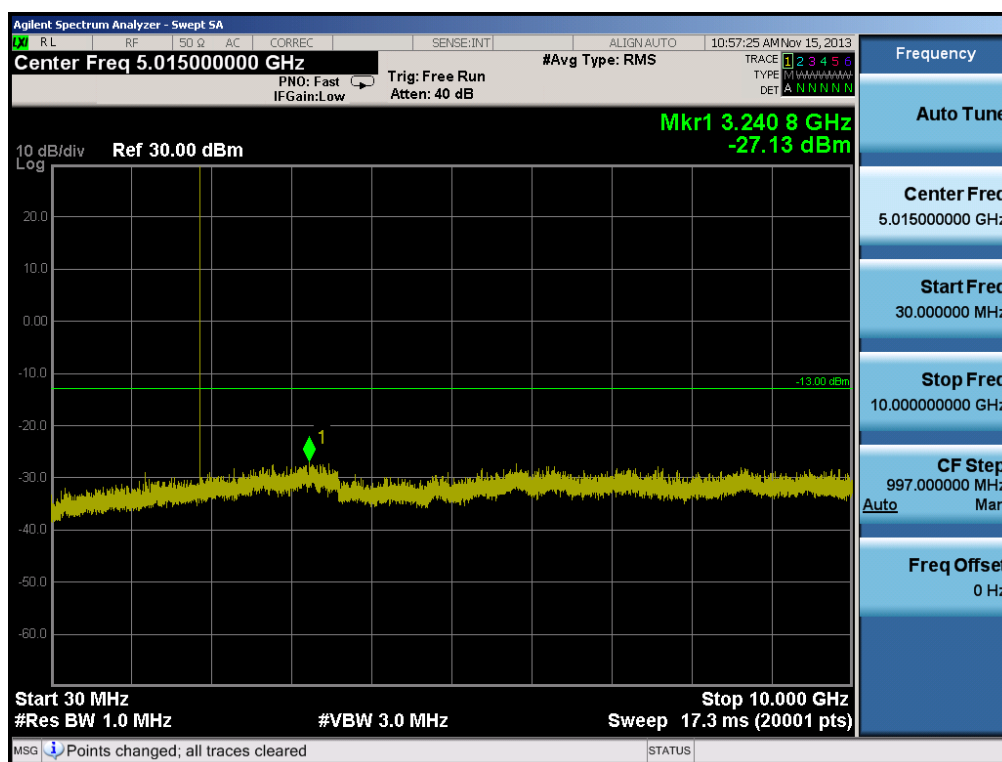
Plot 6-18. Conducted Spurious Plot (PCS GSM Mode – Ch. 661)
