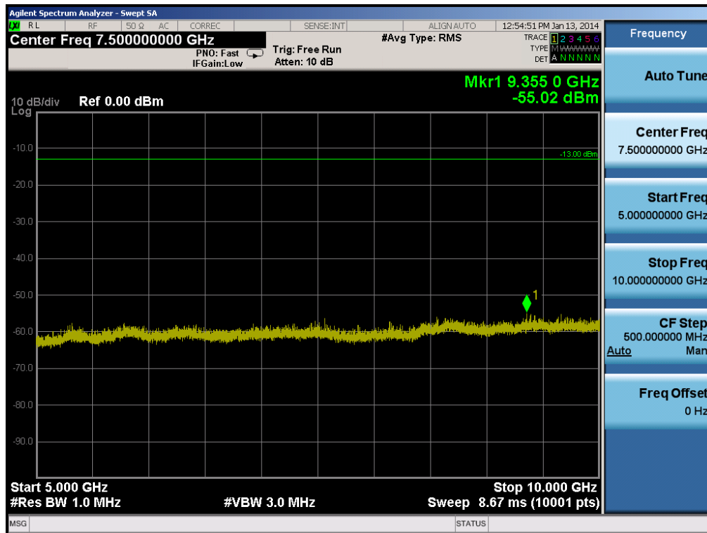
Plot 6-12. Conducted Spurious Plot (Cellular CDMA Mode – Ch. 1013)
