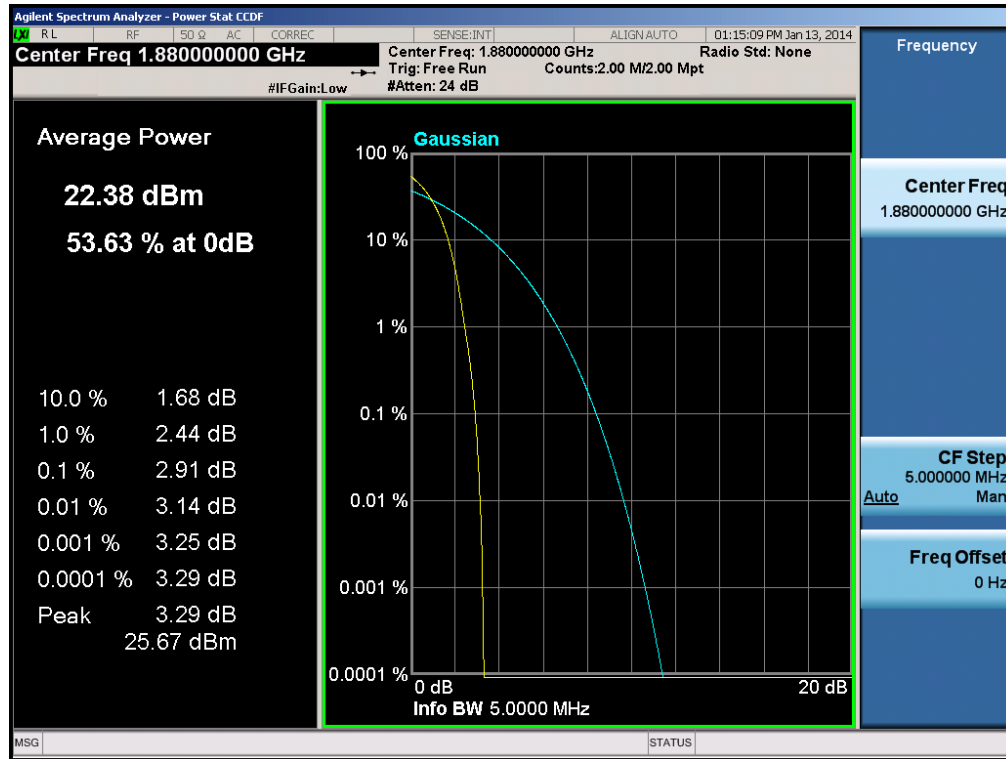
Plot 6-35. Peak-Average Ratio Plot (PCS WCDMA Mode – Ch. 9400)
