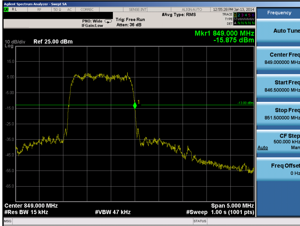
Plot 6-27. Band Edge Plot (Cellular CDMA Mode – Ch. 777)
