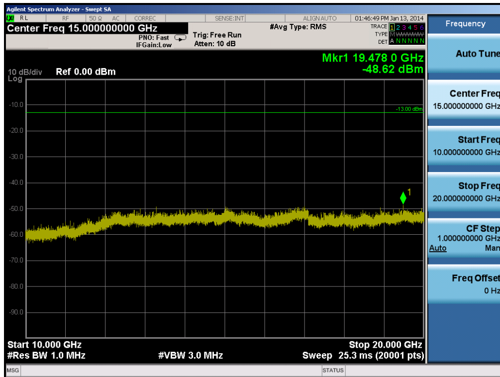
Plot 6-10. Conducted Spurious Plot (PCS GSM Mode – Ch. 810)
