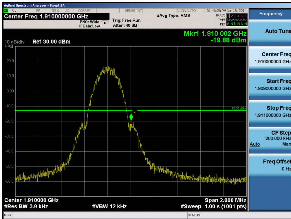
Plot 6-24. Band Edge Plot (PCS GSM Mode – Ch. 810)
