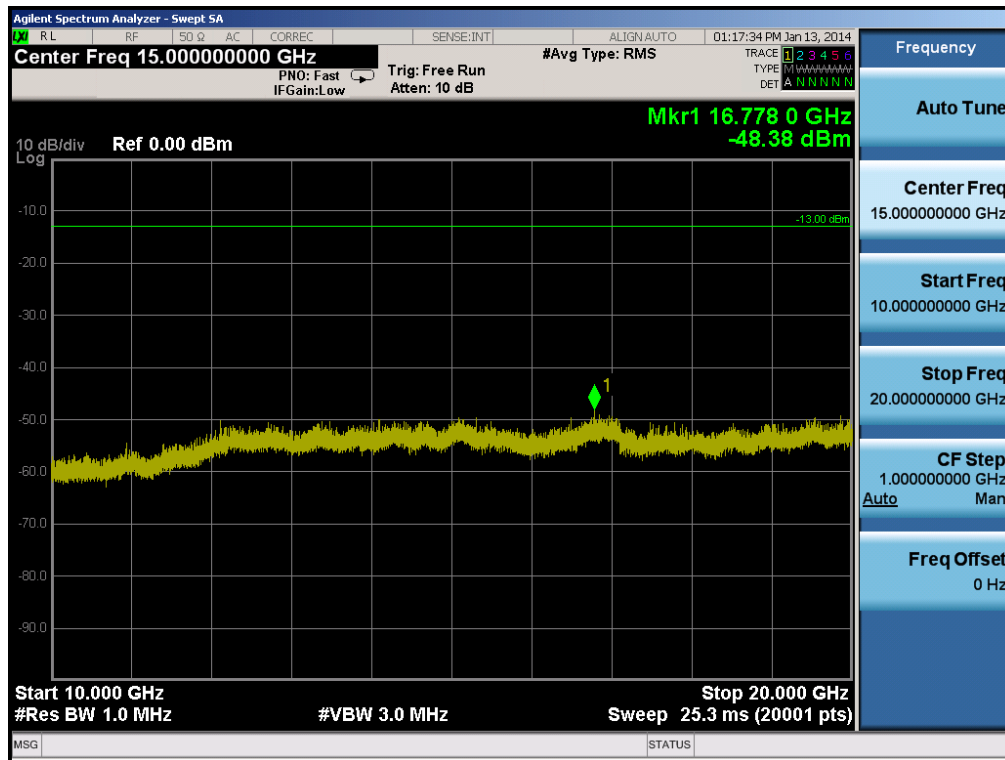
Plot 6-22. Conducted Spurious Plot (PCS WCDMA Mode – Ch. 9538)
