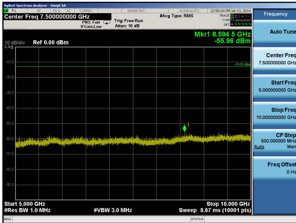
Plot 6-16. Conducted Spurious Plot (Cellular CDMA Mode – Ch. 777)
