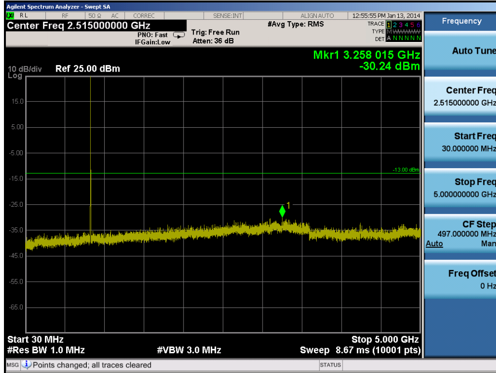
Plot 6-15. Conducted Spurious Plot (Cellular CDMA Mode – Ch. 777)
