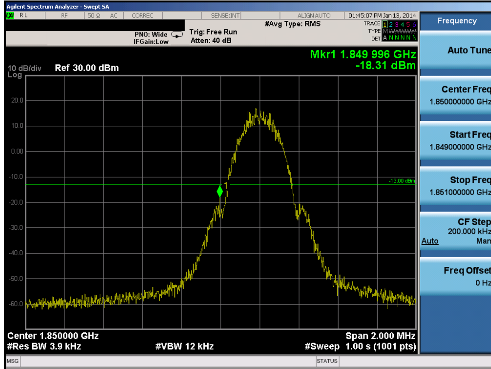
Plot 6-23. Band Edge Plot (PCS GSM Mode – Ch. 512)
