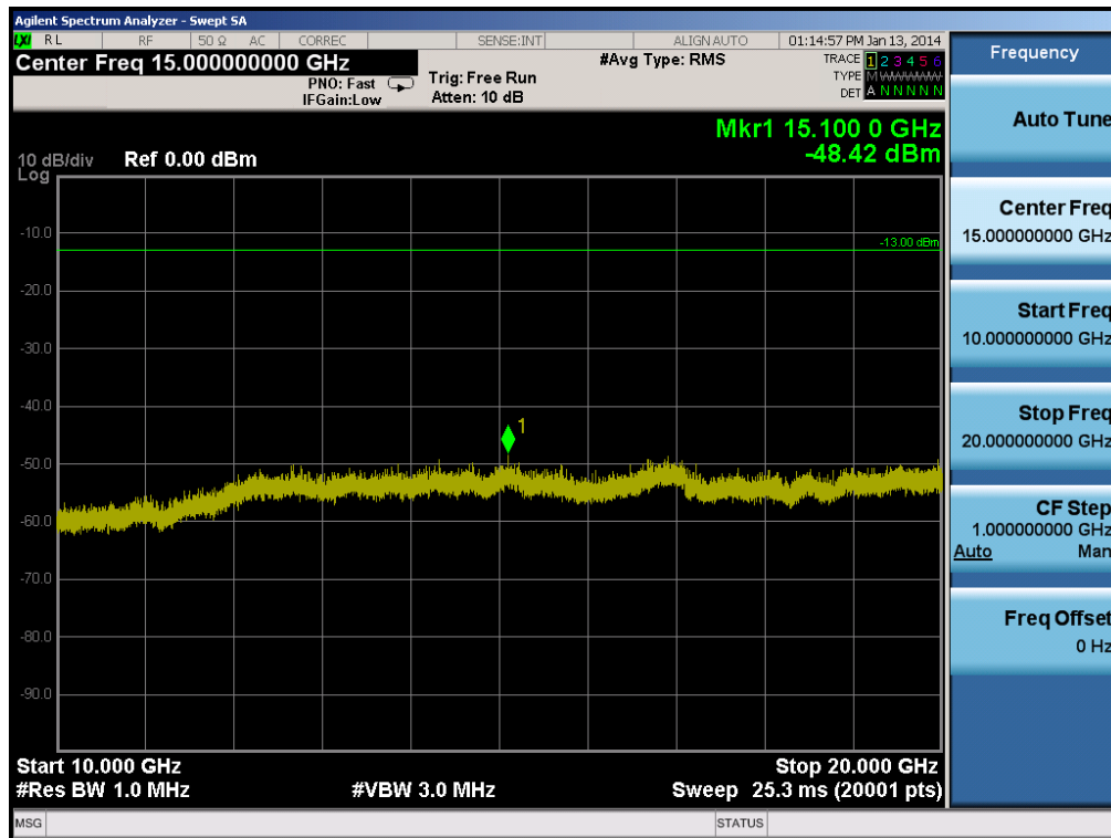
Plot 6-20. Conducted Spurious Plot (PCS WCDMA Mode – Ch. 9400)
