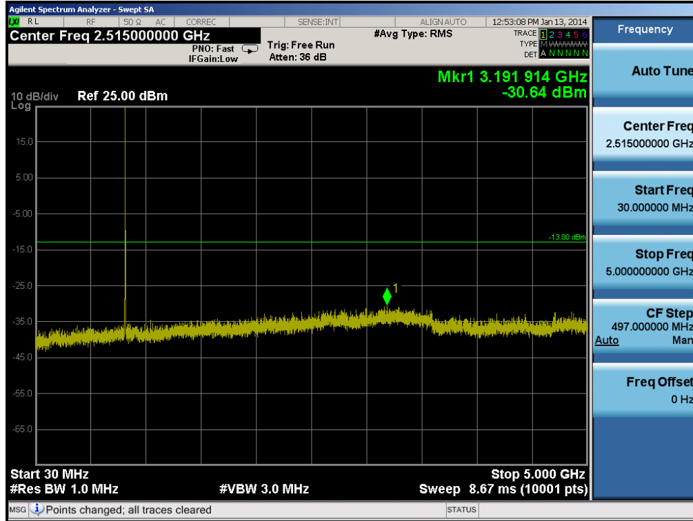
Plot 6-13. Conducted Spurious Plot (Cellular CDMA Mode – Ch. 384)
