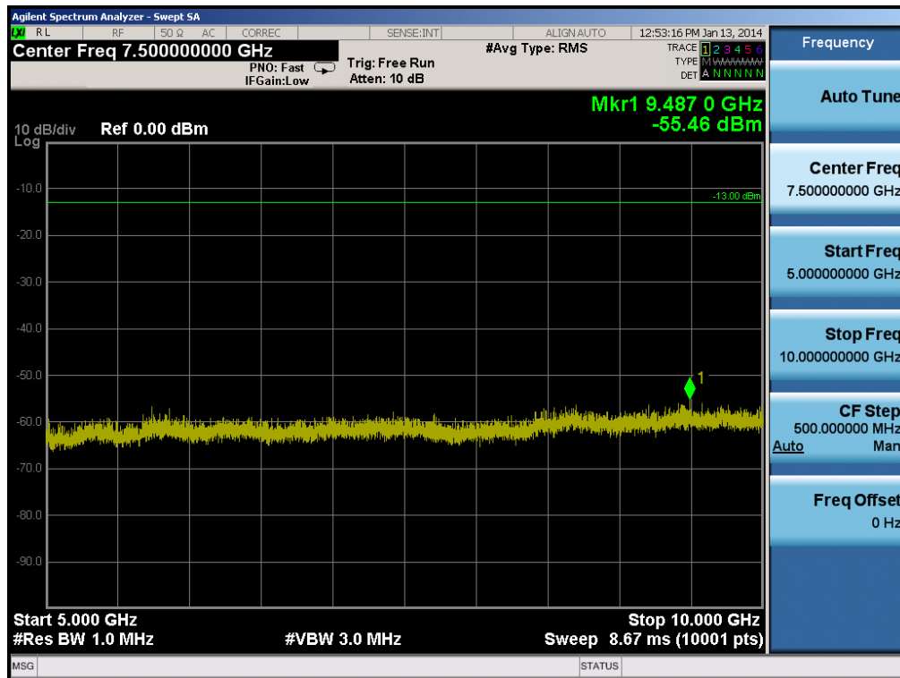
Plot 6-14. Conducted Spurious Plot (Cellular CDMA Mode – Ch. 384)
