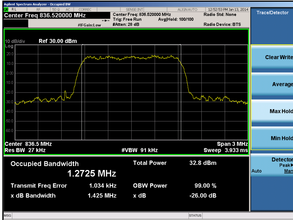
Plot 6-3. Occupied Bandwidth Plot (Cellular CDMA Mode – Ch. 384)
