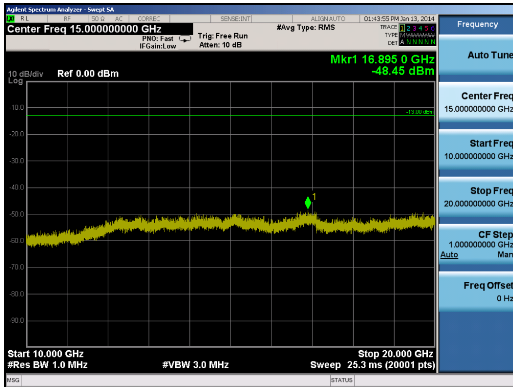
Plot 6-8. Conducted Spurious Plot (PCS GSM Mode – Ch. 661)
