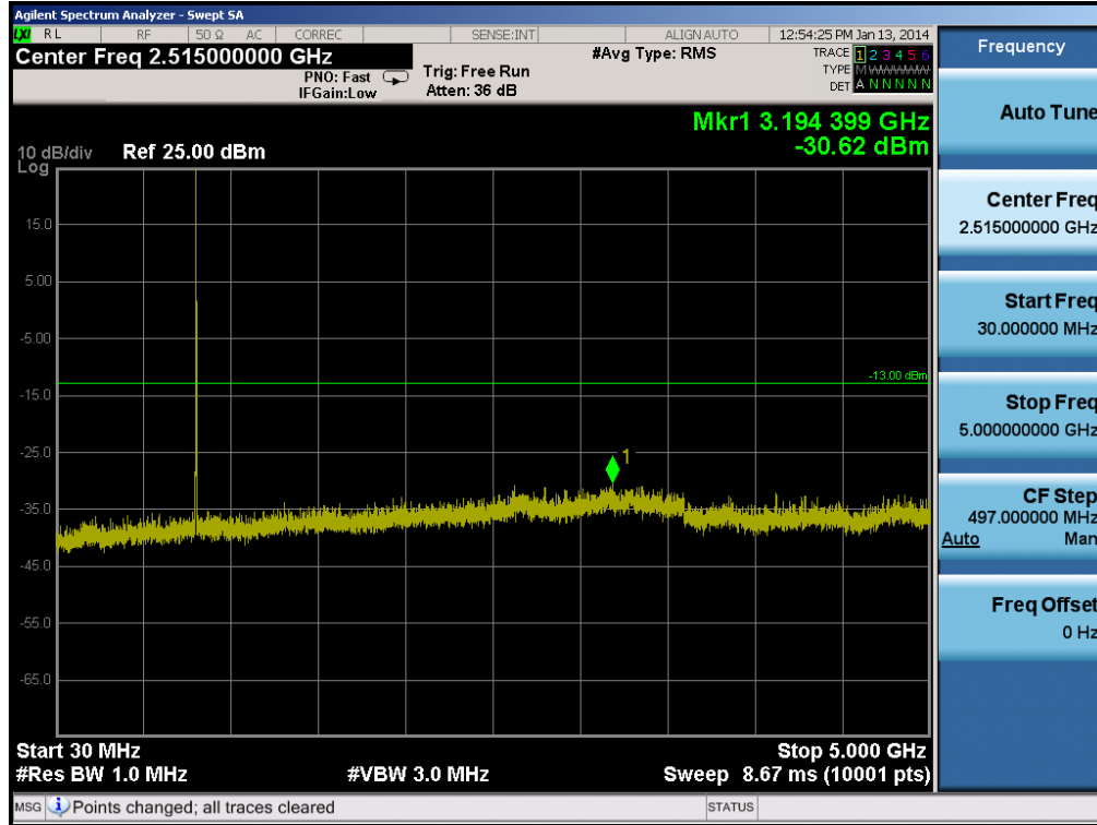
Plot 6-11. Conducted Spurious Plot (Cellular CDMA Mode – Ch. 1013)
