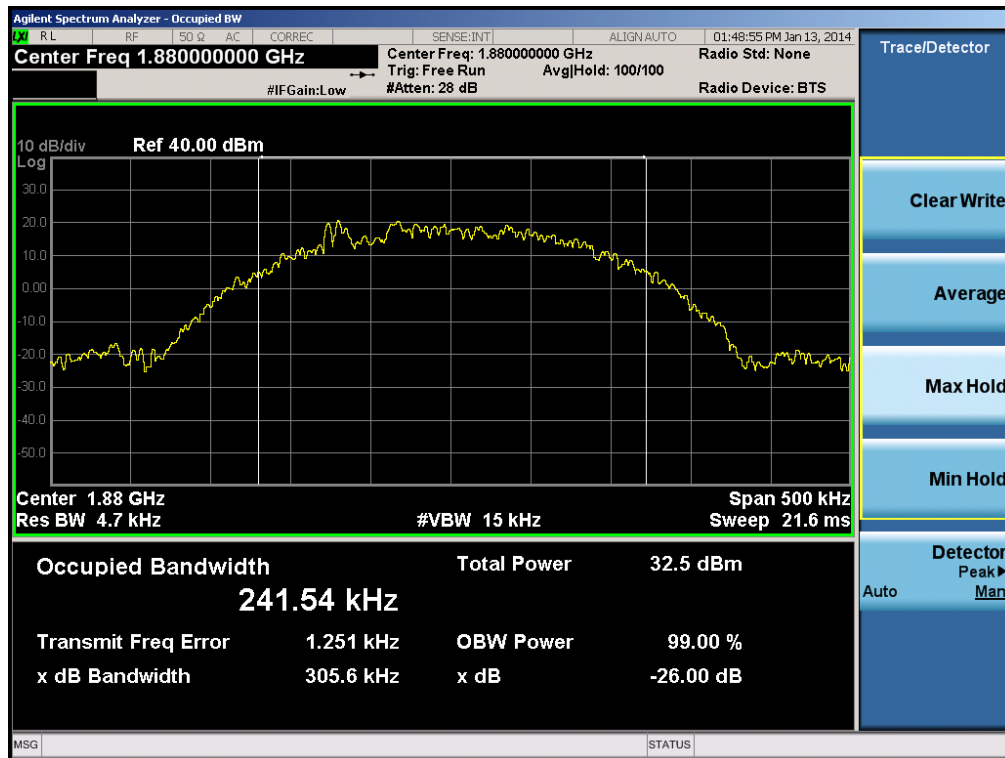
Plot 6-2. Occupied Bandwidth Plot (EDGE1900 Mode – Ch. 661)
