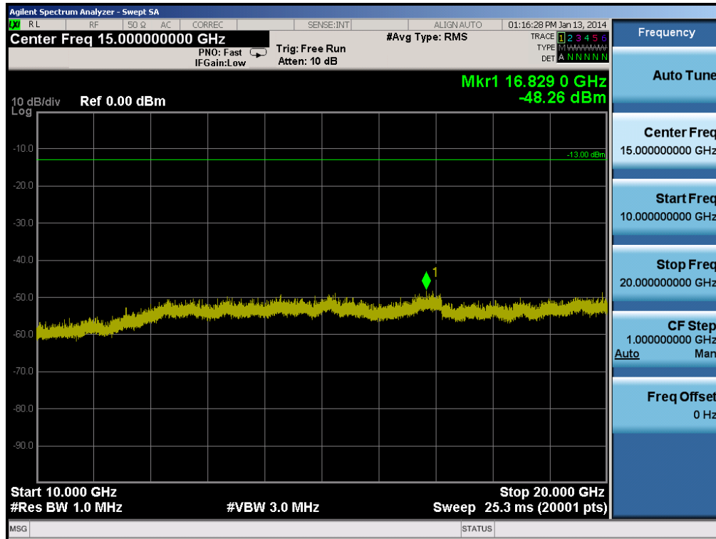
Plot 6-18. Conducted Spurious Plot (PCS WCDMA Mode – Ch. 9262)
