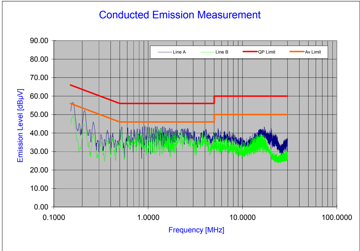
Plot 6-63. Line Conducted Plot with 802.11b
