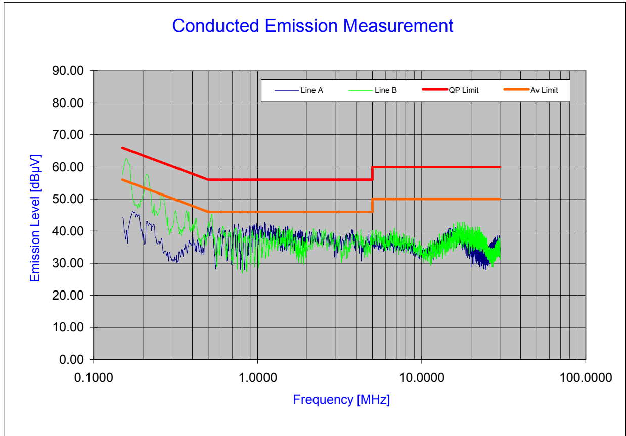
Plot 6-64. Line Conducted Plot with 802.11a
