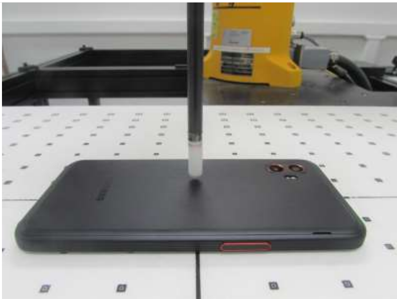
Distance of 2 mm from the EUT
