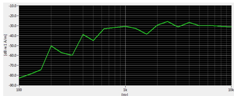
Figure 7-2 Worst-case ABM2 Plot for GSM
