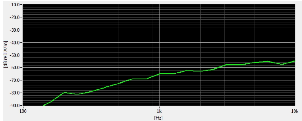
Figure 7-3 Worst-case ABM2 Plot for UMTS
