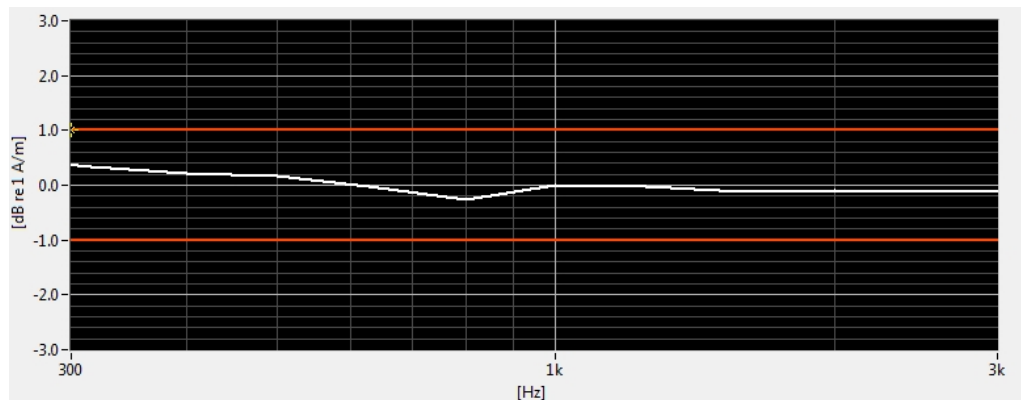
Figure 7-4 Helmholtz Coil Validation for Frequency Response
