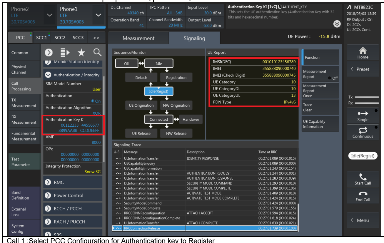
Call 1 :Select PCC Configuration for Authentication key to Register
