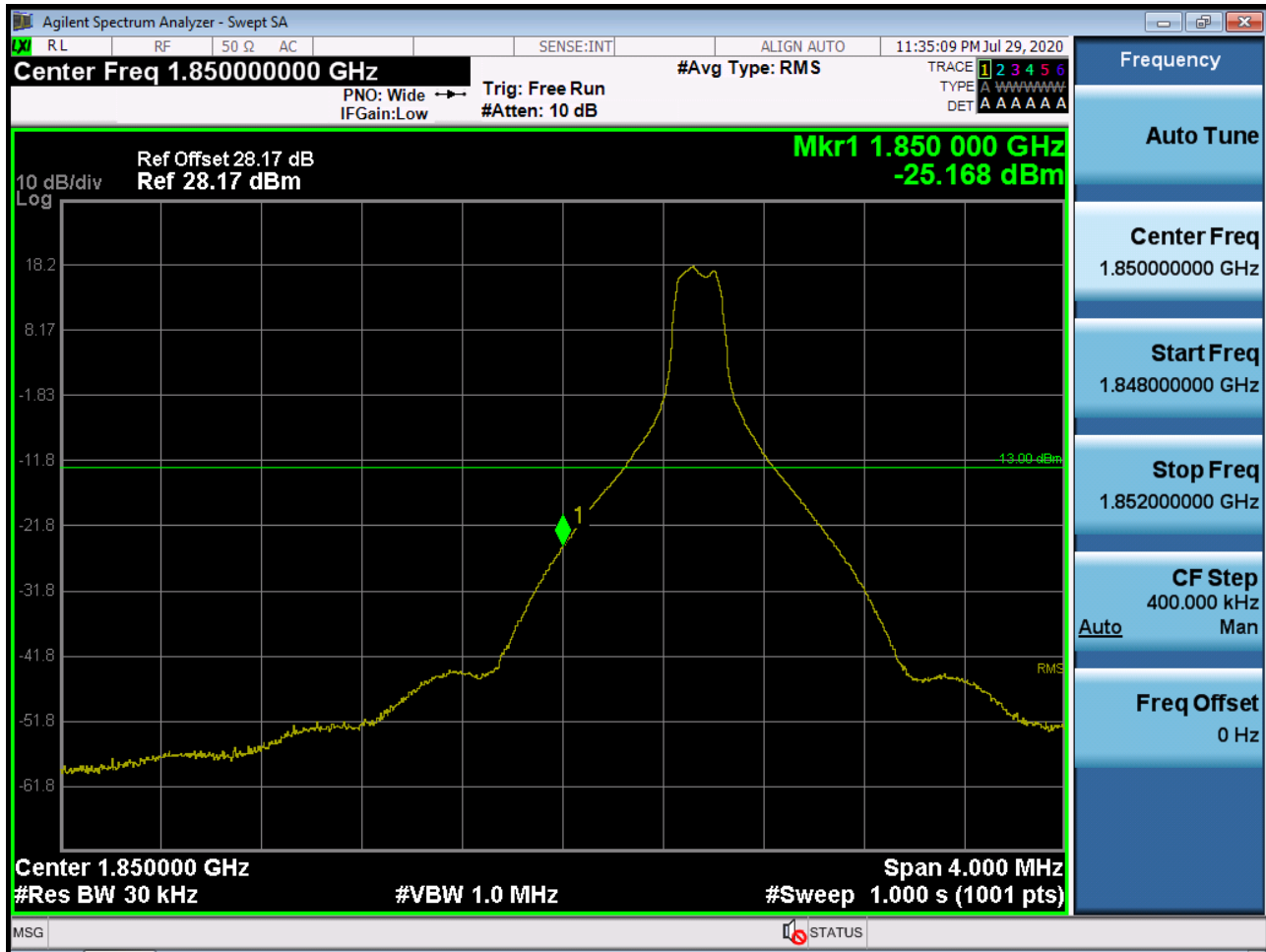
Sub6 n25(2). Lower Band Edge Plot (20M BW Ch.372000 BPSK_RB1_Offset 0)
