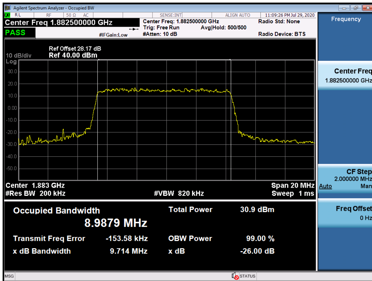
Sub6 n25(2). Occupied Bandwidth Plot (10M BW Ch.376500 64QAM RB 50_0)
