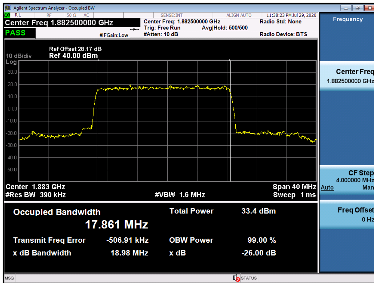
Sub6 n25(2). Occupied Bandwidth Plot (20M BW Ch.376500 BPSK RB 100_0)
