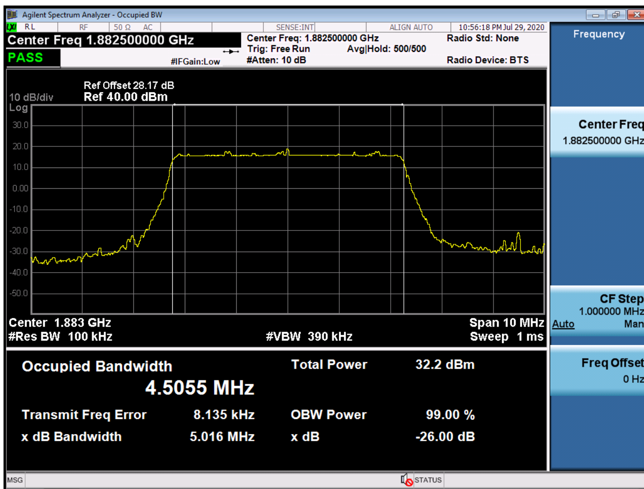
Sub6 n25(2). Occupied Bandwidth Plot (5M BW Ch.376500 16QAM RB 25_0)
