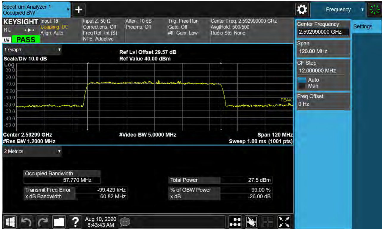
Sub6 n41. Occupied Bandwidth Plot (60 MHz Ch.518598 256-QAM RB 25) _SCS 30 kHz
