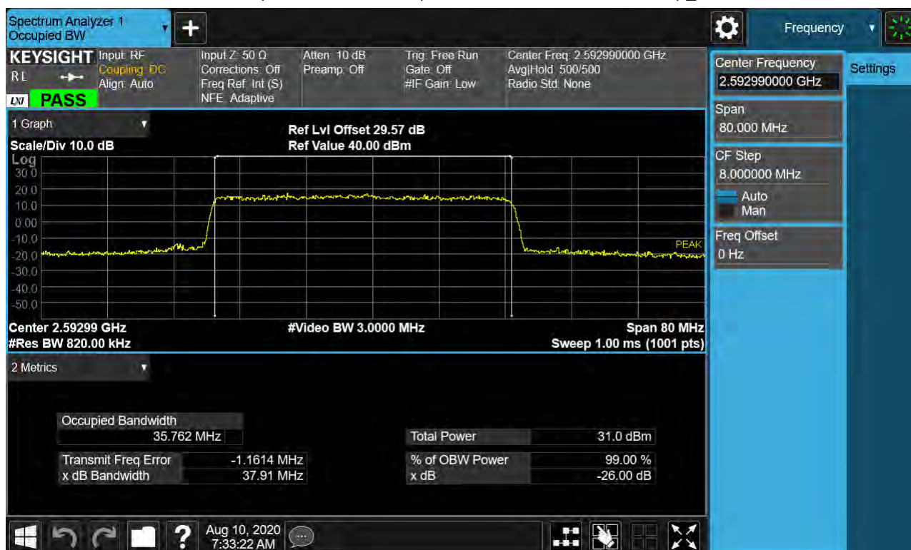
Sub6 n41. Occupied Bandwidth Plot (40 MHz Ch.518598 QPSK RB 25) _SCS 30 kHz
