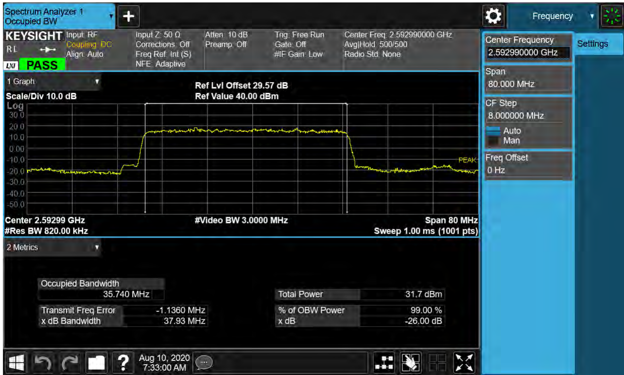
Sub6 n41. Occupied Bandwidth Plot (40 MHz Ch.518598 BPSK RB 25) _SCS 30 kHz
