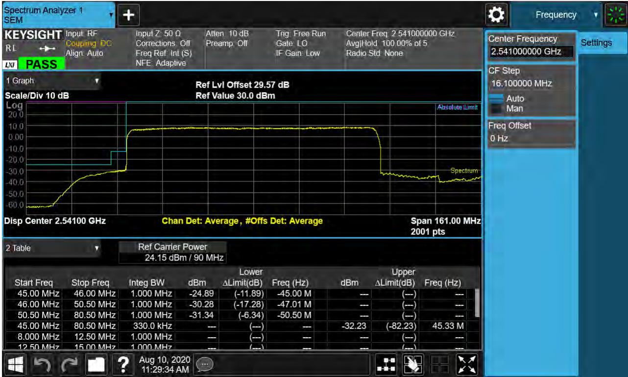
Sub6 n41. Low Channel Edge Plot (90 MHz Ch.508200 BPSK RB 25, Offset 0)-1
