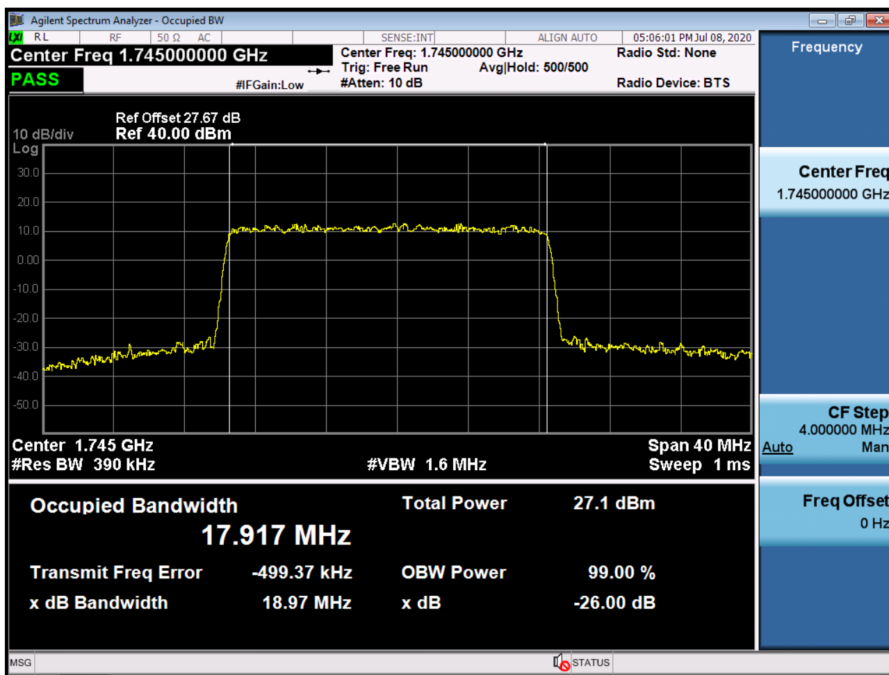
Sub6 n66. Occupied Bandwidth Plot (20M BW Ch.349000 256QAM RB 100)
