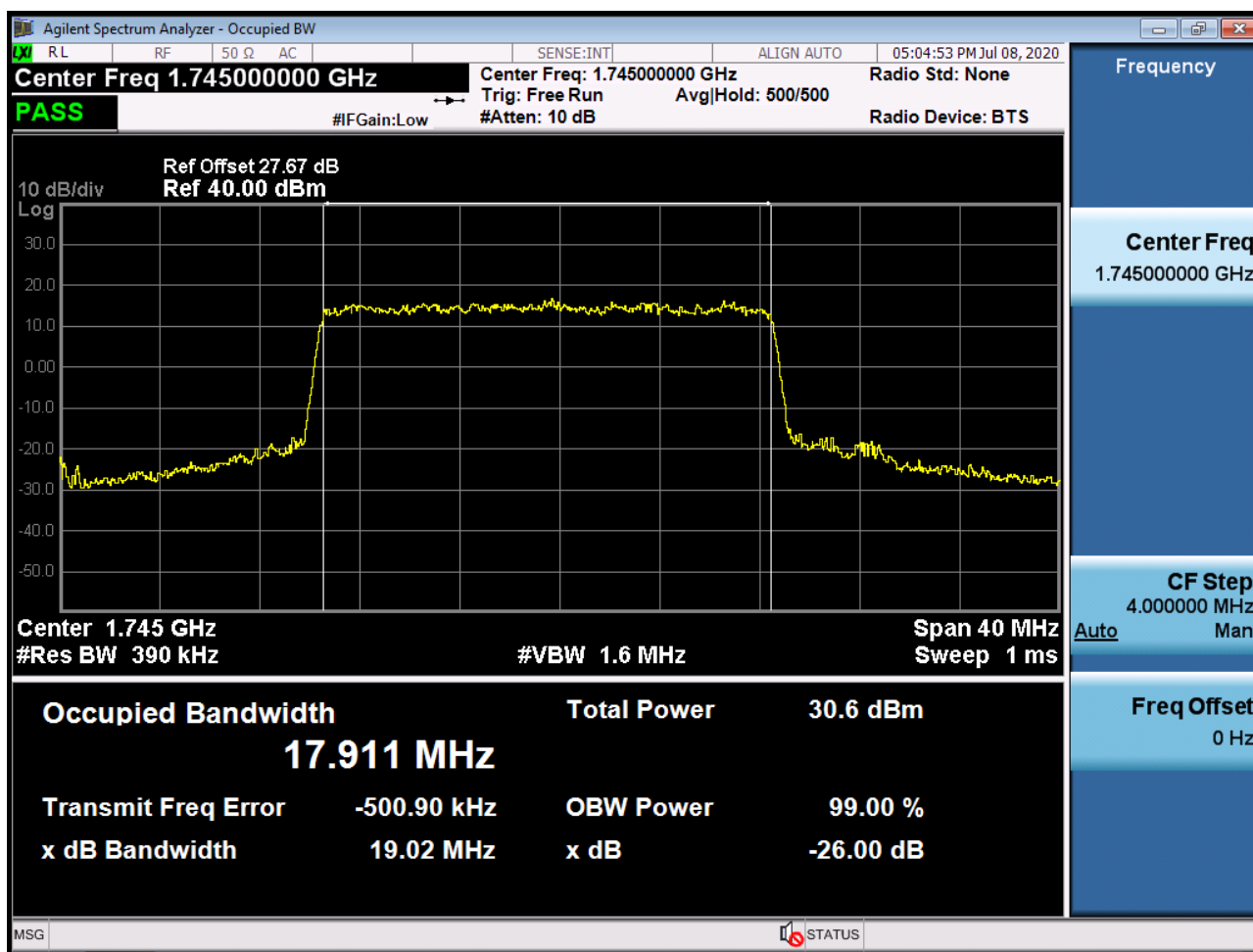
Sub6 n66. Occupied Bandwidth Plot (20M BW Ch.349000 QPSK RB 100)
