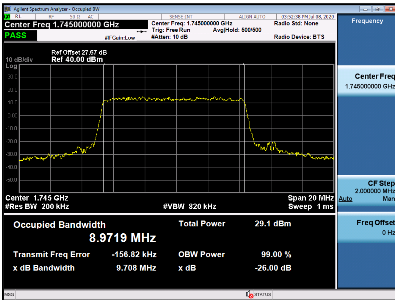
Sub6 n66. Occupied Bandwidth Plot (10M BW Ch.349000 64QAM RB 50)
