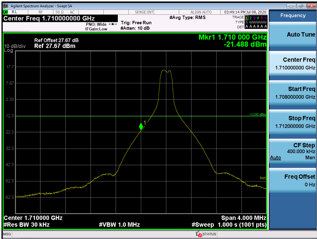
Sub6 n66. Lower Band Edge Plot (10M BW Ch.343000 BPSK RB 1, Offset 0) -1
