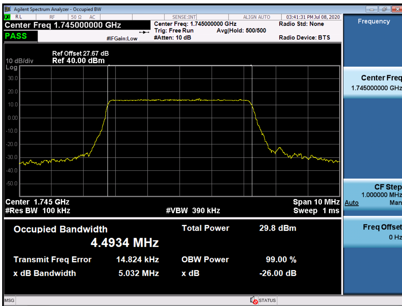
Sub6 n66. Occupied Bandwidth Plot (5M BW Ch.349000 64QAM RB 25)
