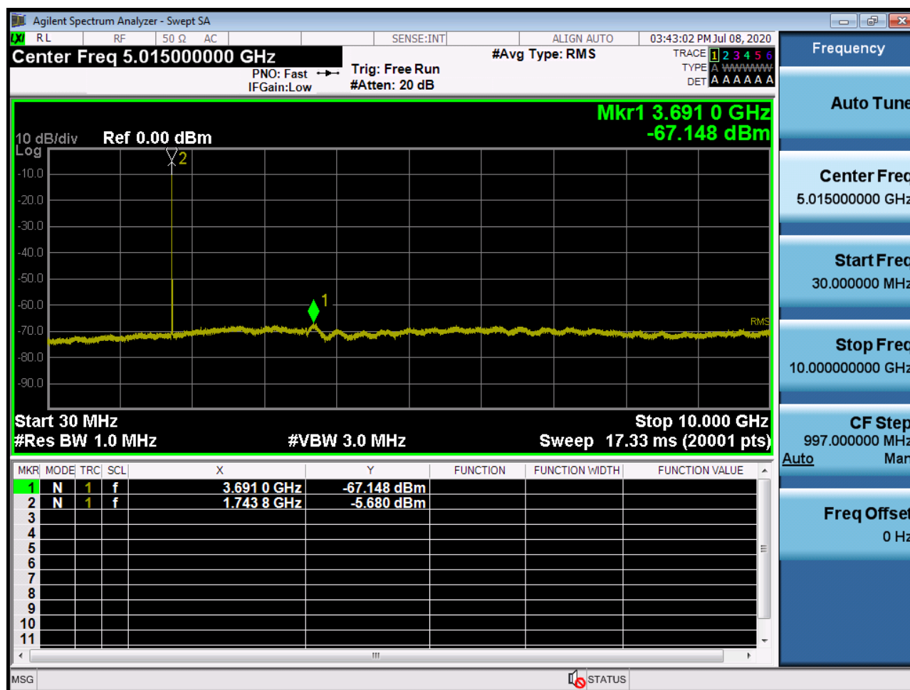
Sub6 n66. Conducted Spurious Plot_1 (349000ch_5MHz_BPSK_ RB 1_0)
