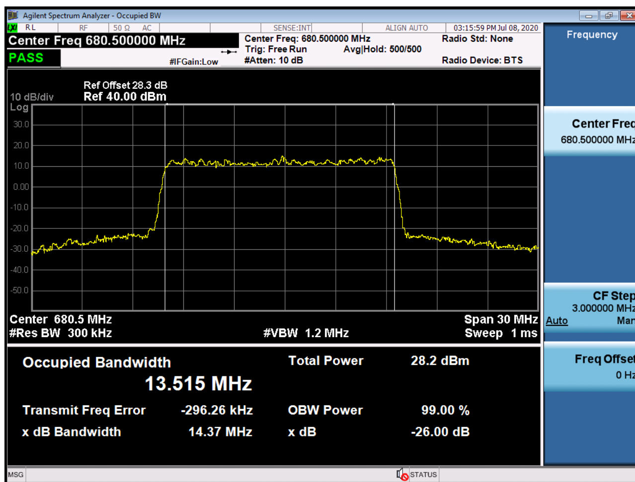
Sub6 n71. Occupied Bandwidth Plot (15M BW Ch.136100 256QAM_RB25_0)
