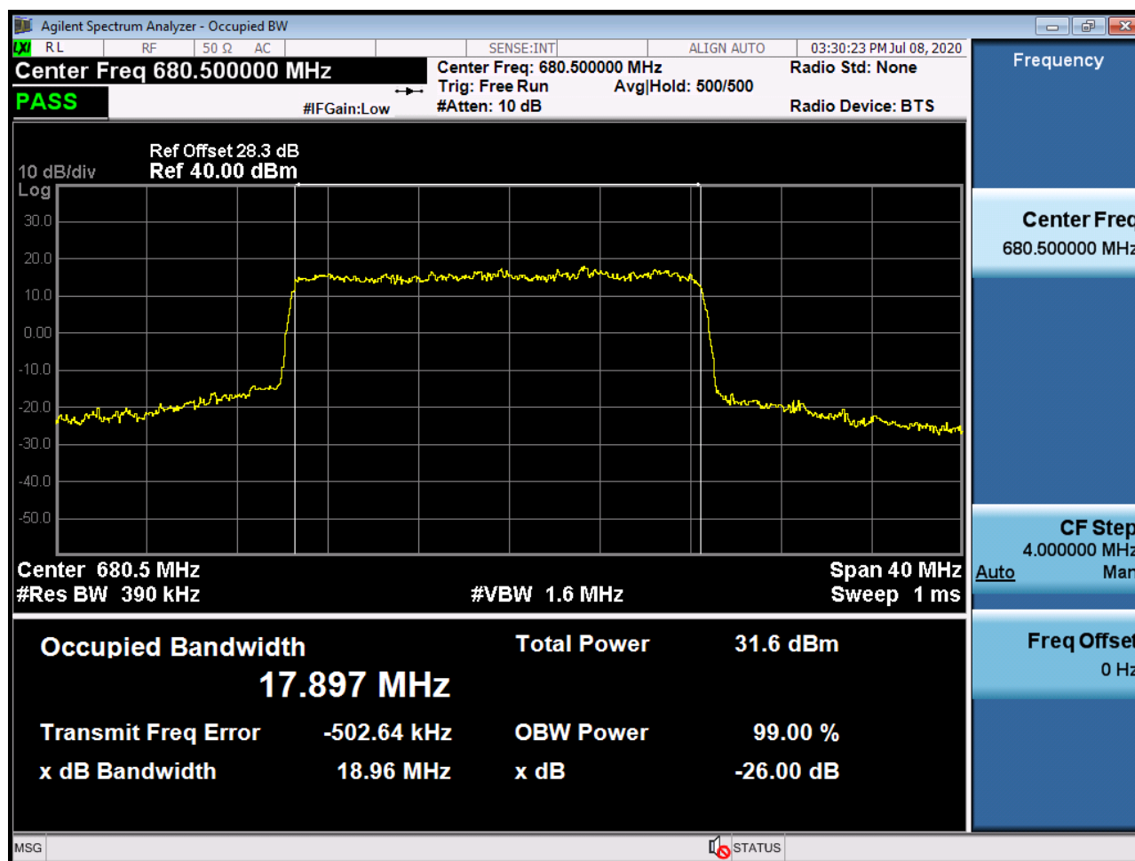
Sub6 n71. Occupied Bandwidth Plot (20M BW Ch.136100 QPSK_RB50_0)
