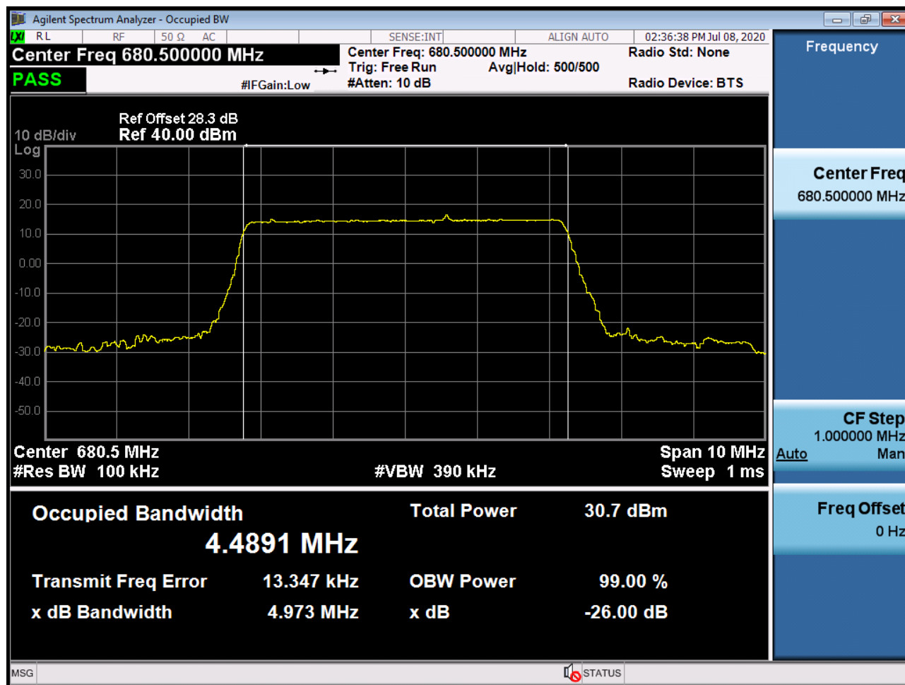
Sub6 n71. Occupied Bandwidth Plot (5M BW Ch.136100 64QAM_RB6_0)
