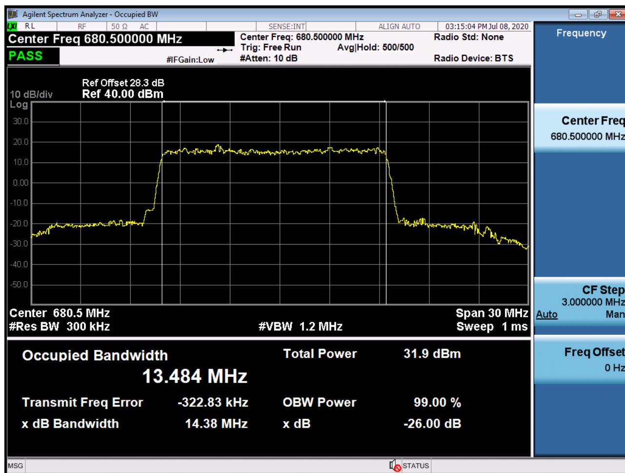
Sub6 n71. Occupied Bandwidth Plot (15M BW Ch.136100 BPSK_RB25_0)
