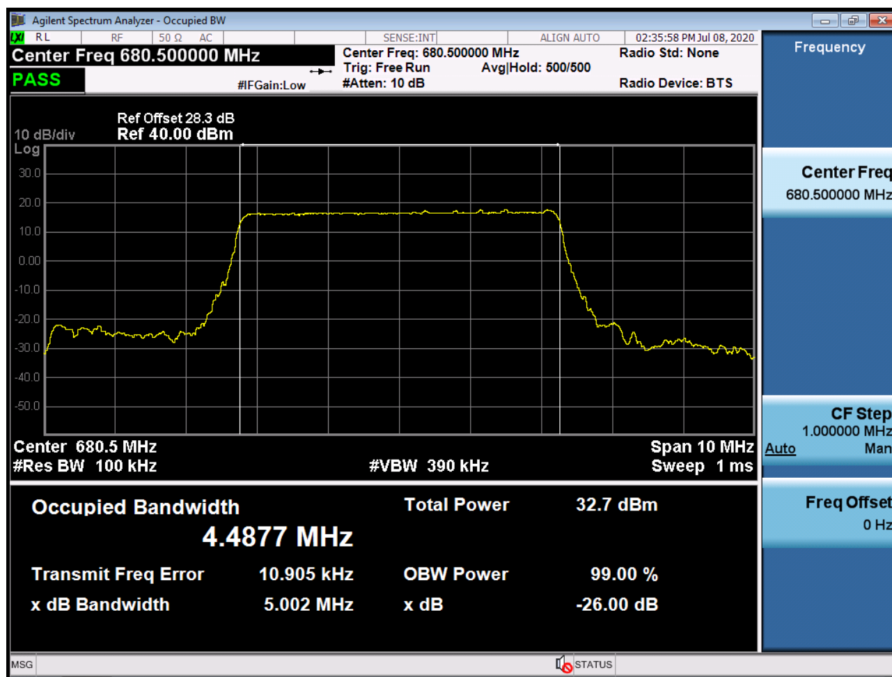
Sub6 n71. Occupied Bandwidth Plot (5M BW Ch.136100 BPSK_RB6_0)
