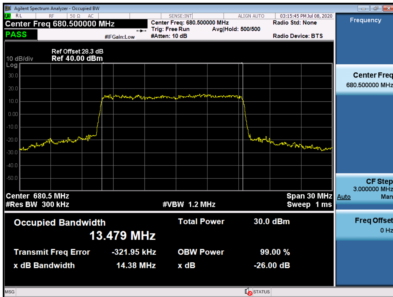
Sub6 n71. Occupied Bandwidth Plot (15M BW Ch.136100 64QAM_RB25_0)
