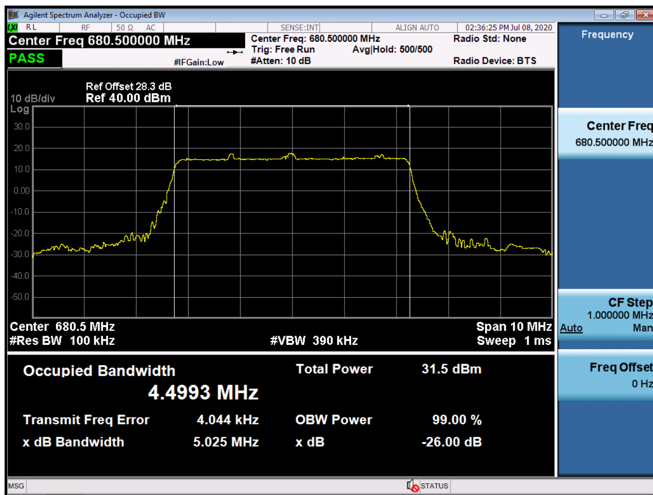
Sub6 n71. Occupied Bandwidth Plot (5M BW Ch.136100 16QAM_RB6_0)
