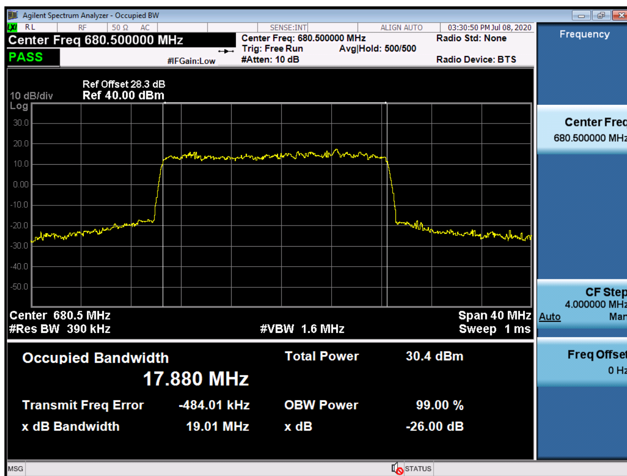
Sub6 n71. Occupied Bandwidth Plot (20M BW Ch.136100 64QAM_RB50_0)
