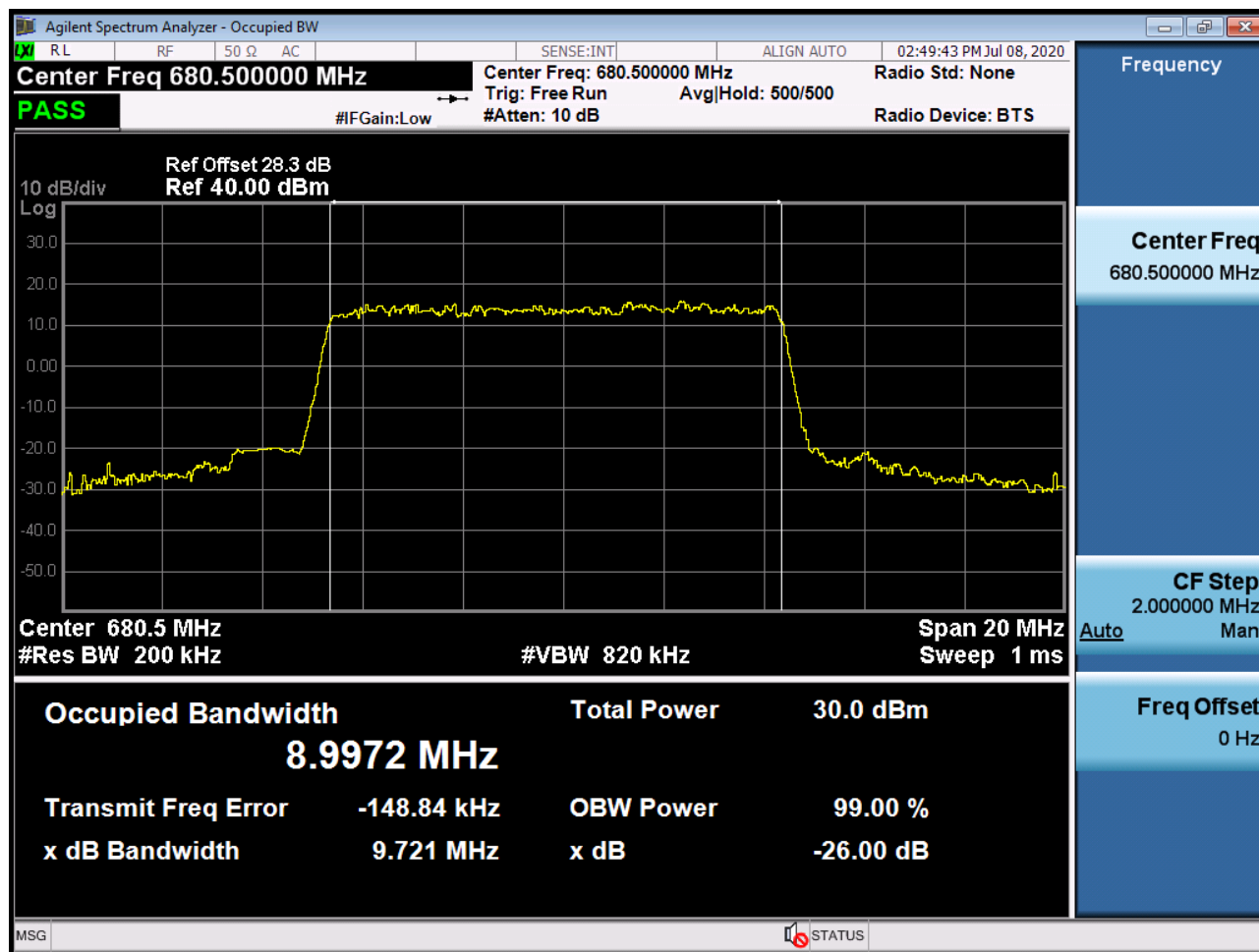
Sub6 n71. Occupied Bandwidth Plot (10M BW Ch.136100 64QAM_RB15_0)
