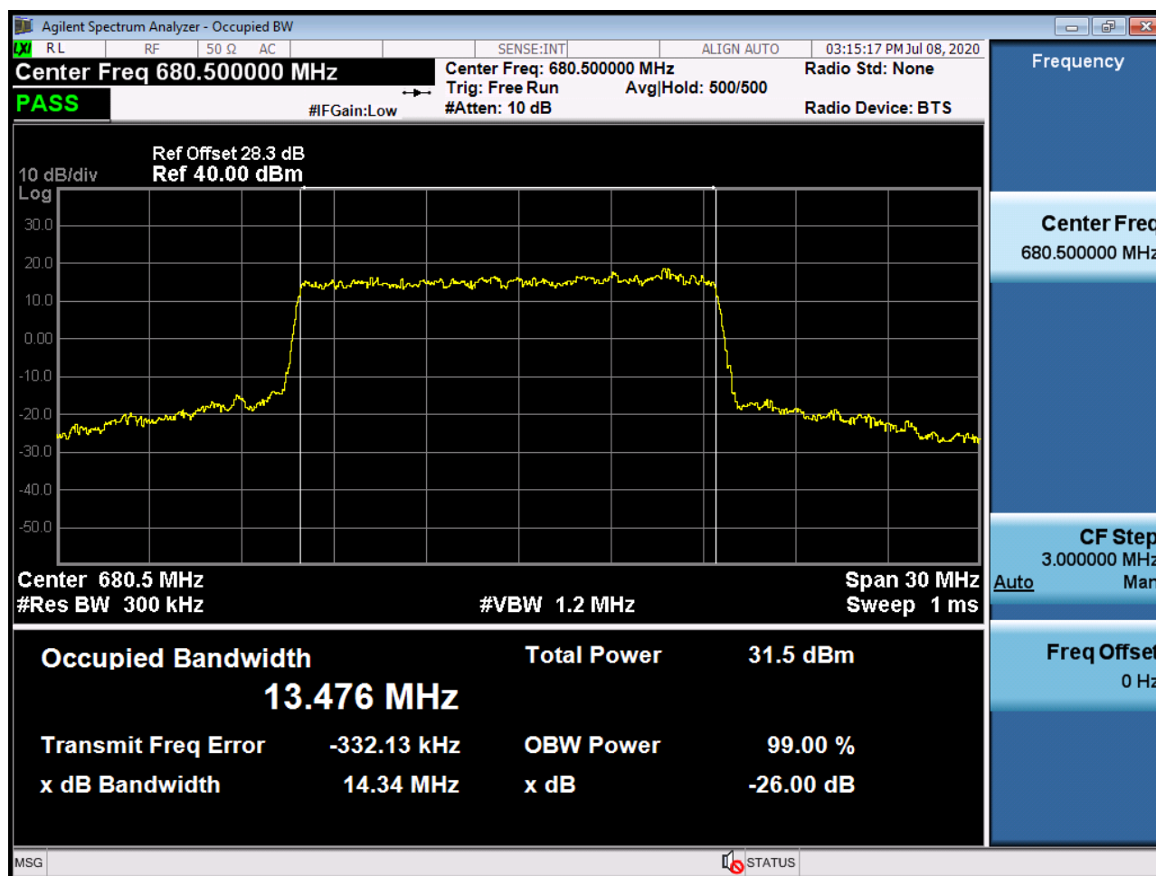
Sub6 n71. Occupied Bandwidth Plot (15M BW Ch.136100 QPSK_RB25_0)
