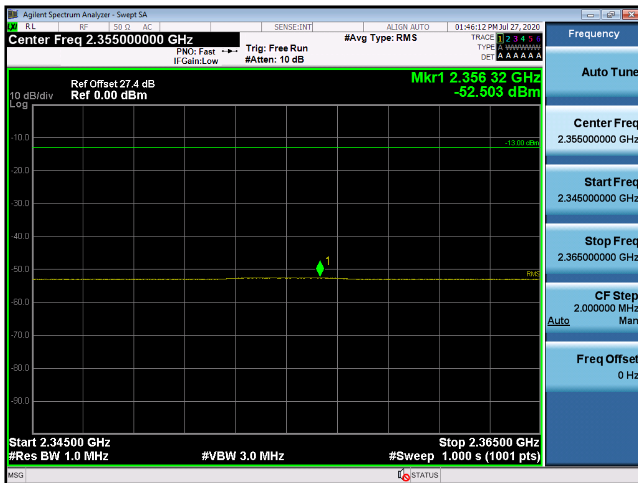
BAND 30. 5M_BandEdge(2345MHz-2365MHz)_Mid_2310MHz_QPSK_1RB
