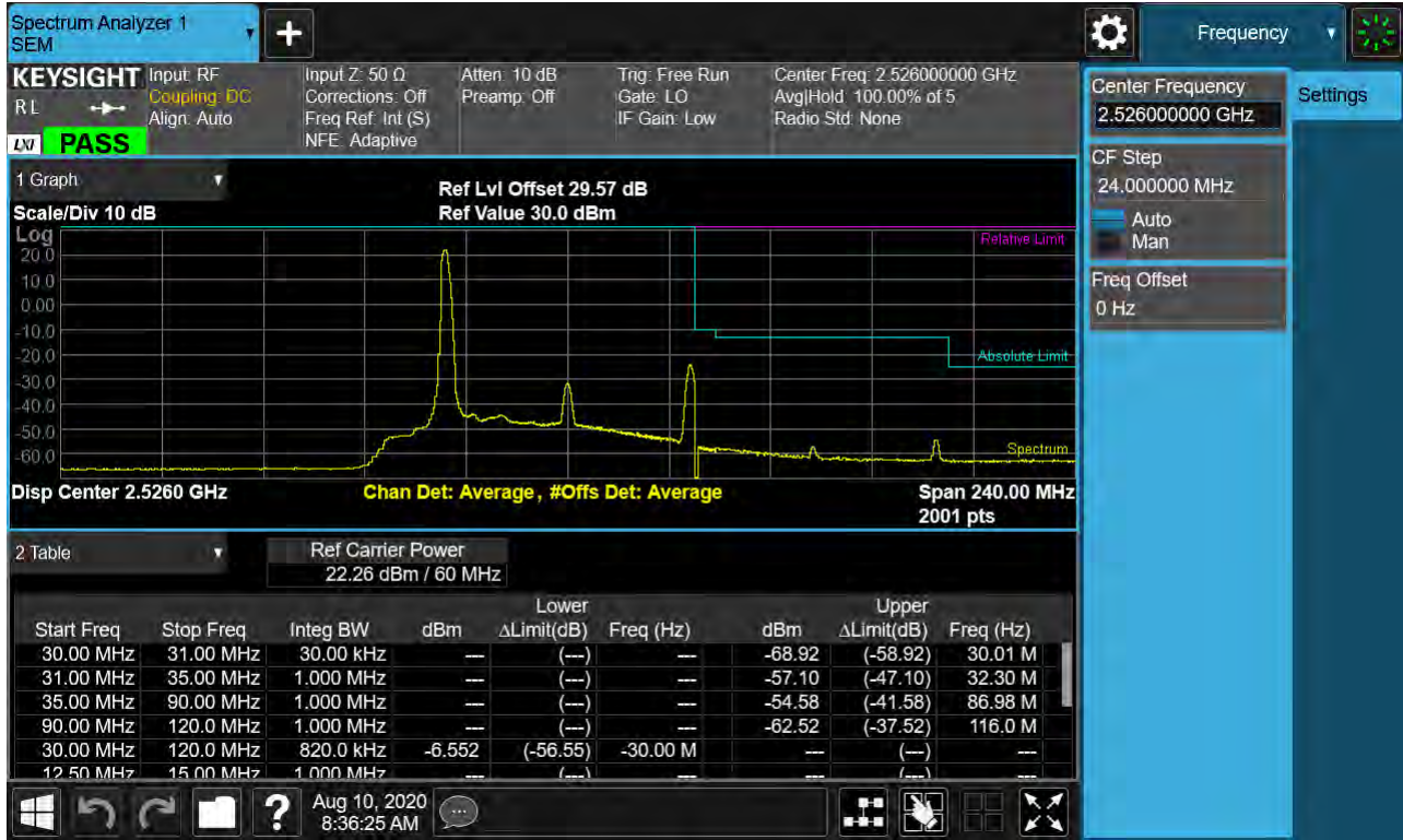
Sub6 n41. Low Channel Edge Plot (60 MHz Ch.505200 BPSK_RB1_Offset 0)-2
