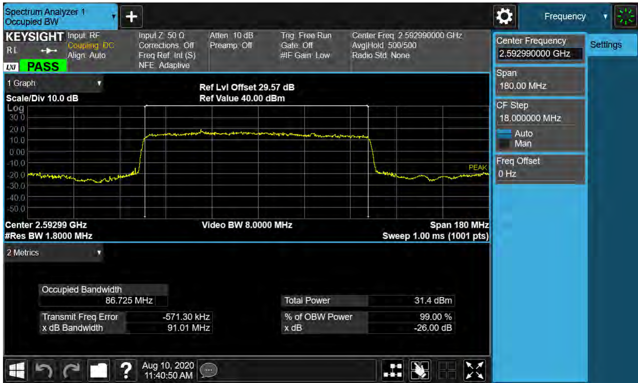
Sub6 n41. Occupied Bandwidth Plot (90 MHz Ch.518598 BPSK RB 25) _SCS 30 kHz
