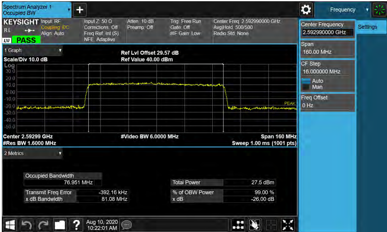
Sub6 n41. Occupied Bandwidth Plot (80 MHz Ch.518598 256-QAM RB 25) _SCS 30 kHz
