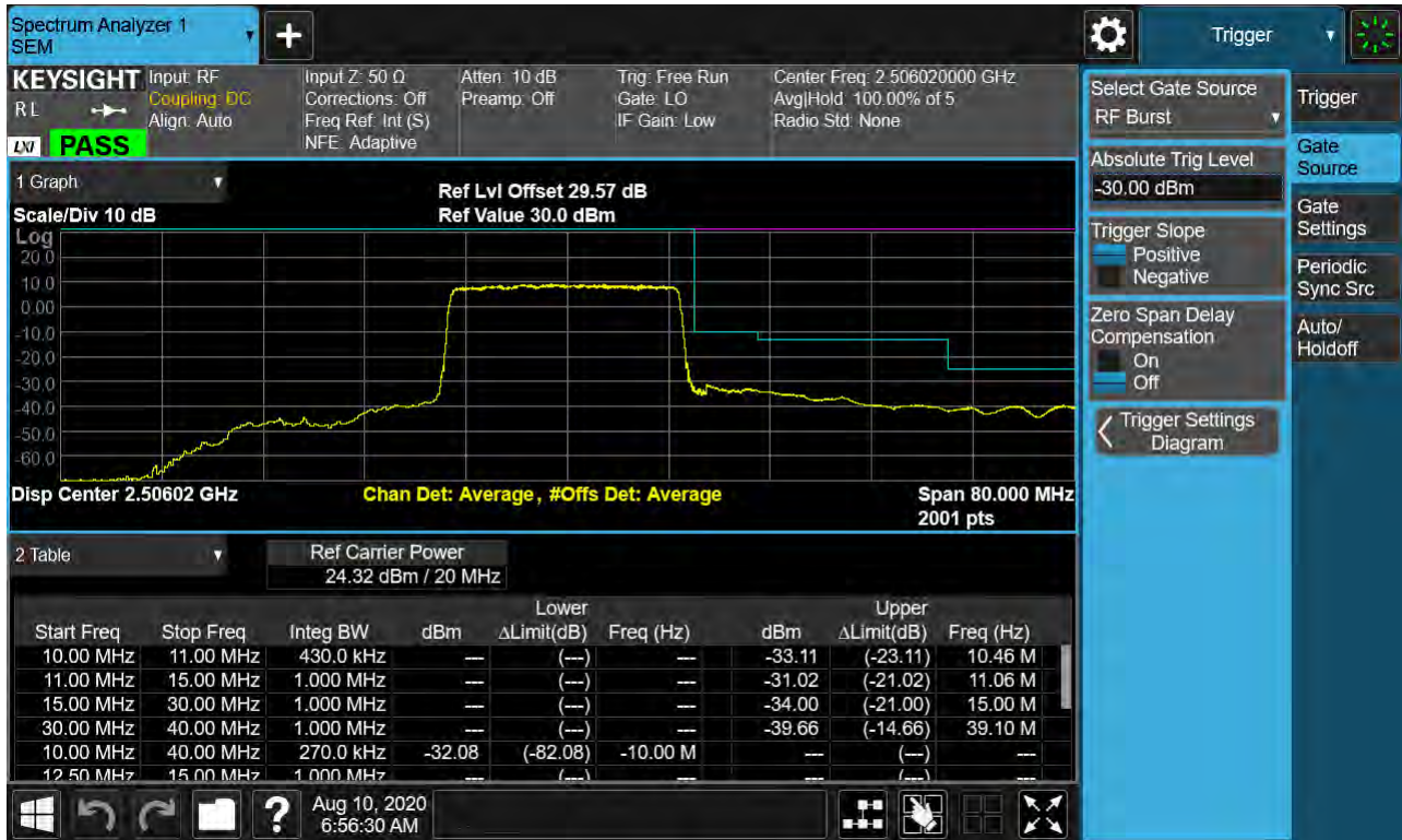
Sub6 n41. Low Channel Edge Plot (20 MHz Ch.501204 BPSK_RB25_Offset 0)-2
