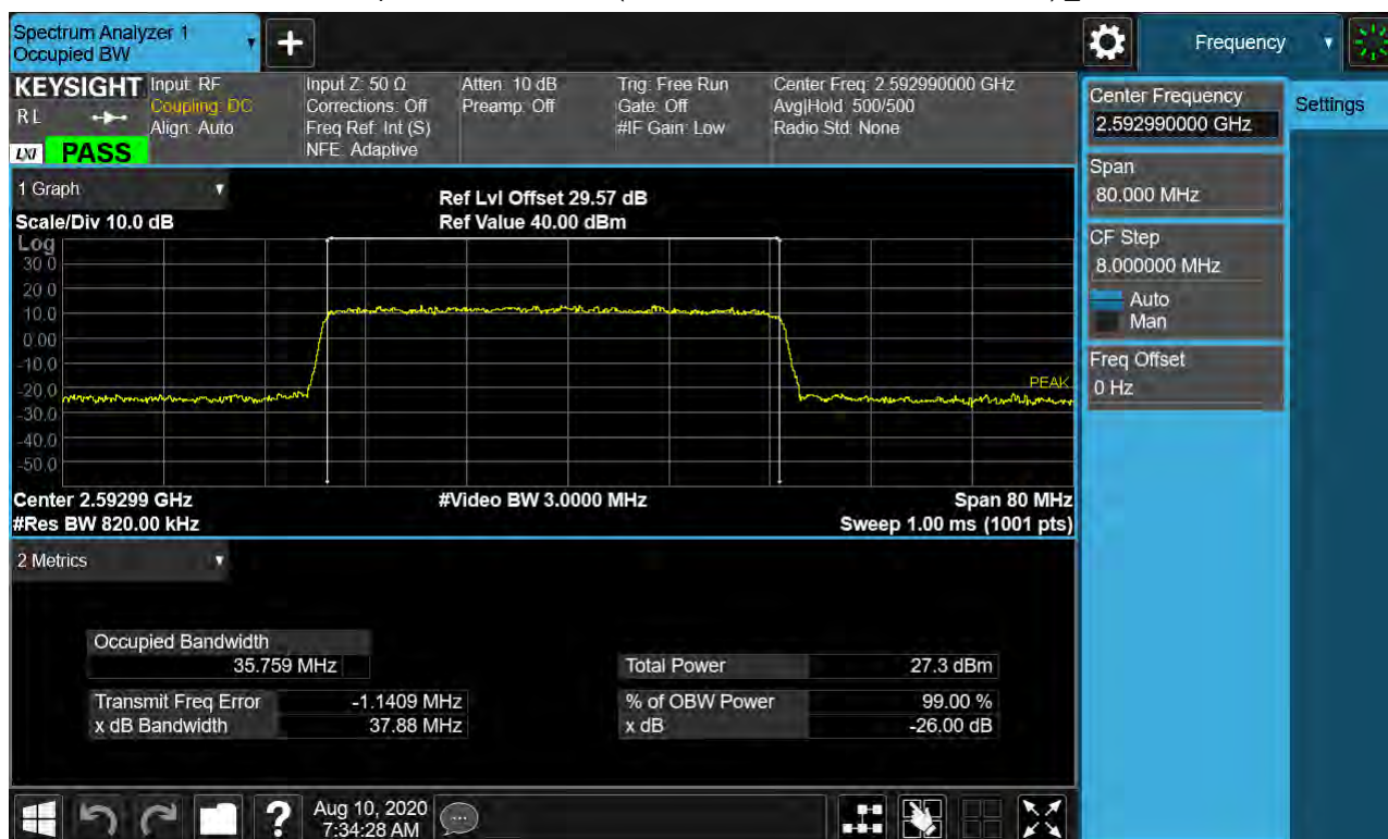
Sub6 n41. Occupied Bandwidth Plot (40 MHz Ch.518598 256-QAM RB 25) _SCS 30 kHz
