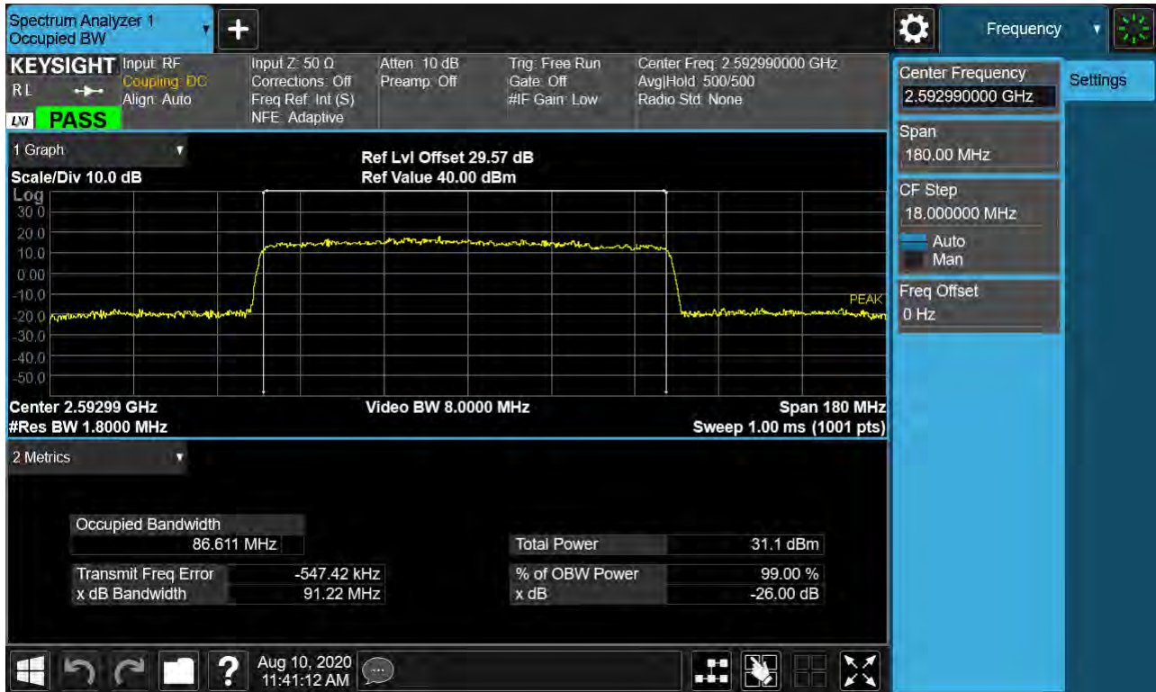
Sub6 n41. Occupied Bandwidth Plot (90 MHz Ch.518598 QPSK RB 25) _SCS 30 kHz
