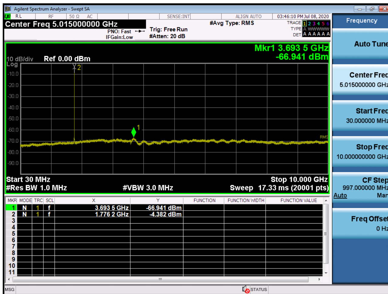
Sub6 n66. Conducted Spurious Plot_1 (355500ch_5MHz_BPSK_ RB 1_0)
