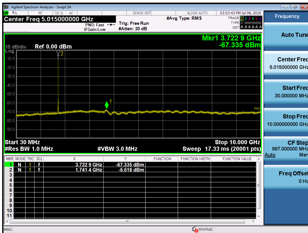
Sub6 n66. Conducted Spurious Plot_1 (349000ch_10MHz_BPSK_ RB 1_0)
