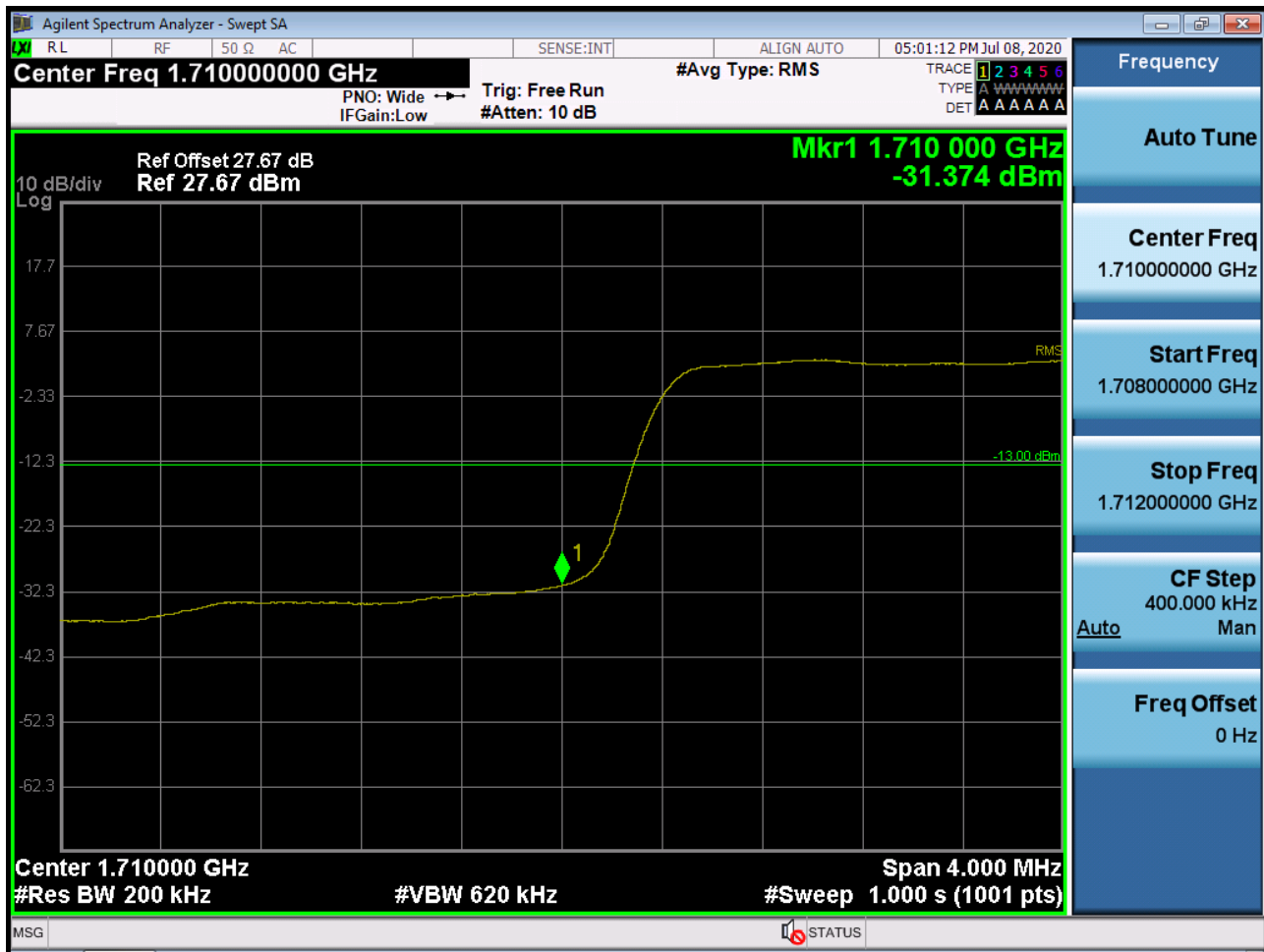
Sub6 n66. Lower Band Edge Plot (20M BW Ch.344000 BPSK RB 100_0) -2
