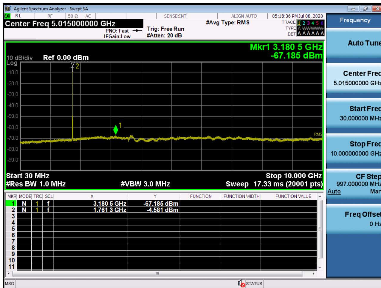
Sub6 n66. Conducted Spurious Plot_1 (354000ch_20MHz_BPSK_ RB 1_0)
