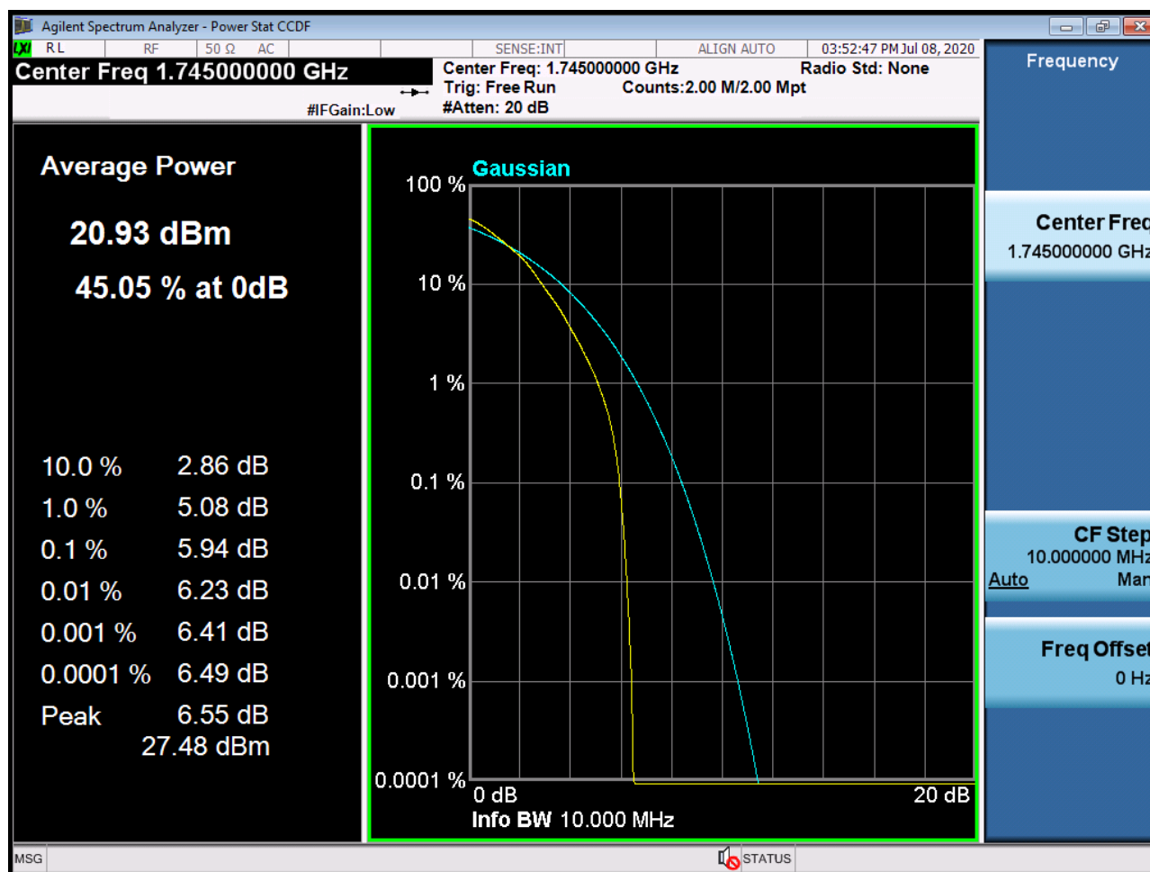
Sub6 n66. PAR Plot (10M BW_Ch.349000_64QAM_RB50_0)
