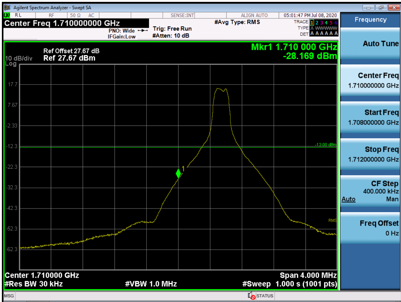
Sub6 n66. Lower Band Edge Plot (20M BW Ch.344000 BPSK RB 1, Offset 0) -1
