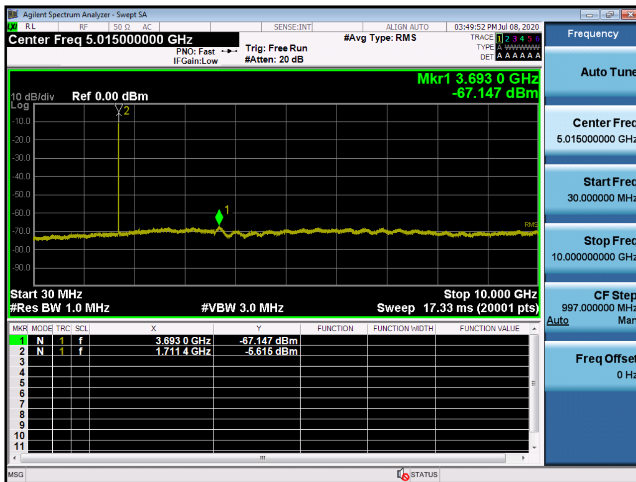
Sub6 n66. Conducted Spurious Plot_1 (343000ch_10MHz_BPSK_ RB 1_0)
