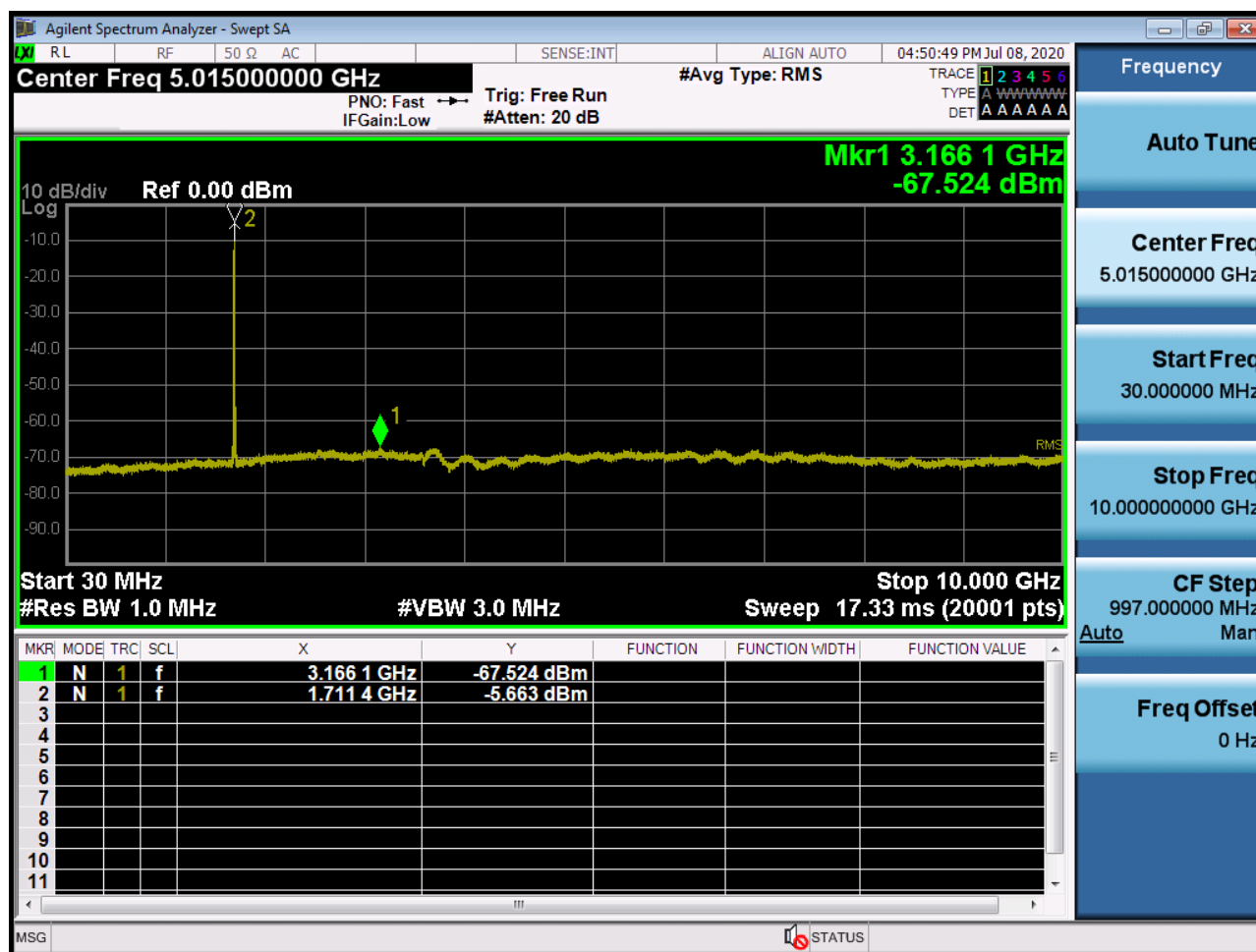
Sub6 n66. Conducted Spurious Plot_1 (343500ch_15MHz_BPSK_ RB 1_0)
