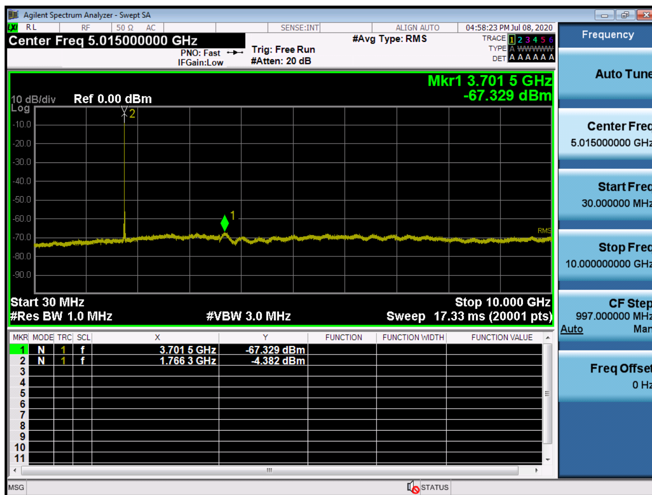
Sub6 n66. Conducted Spurious Plot_1 (354500ch_15MHz_BPSK_ RB 1_0)
