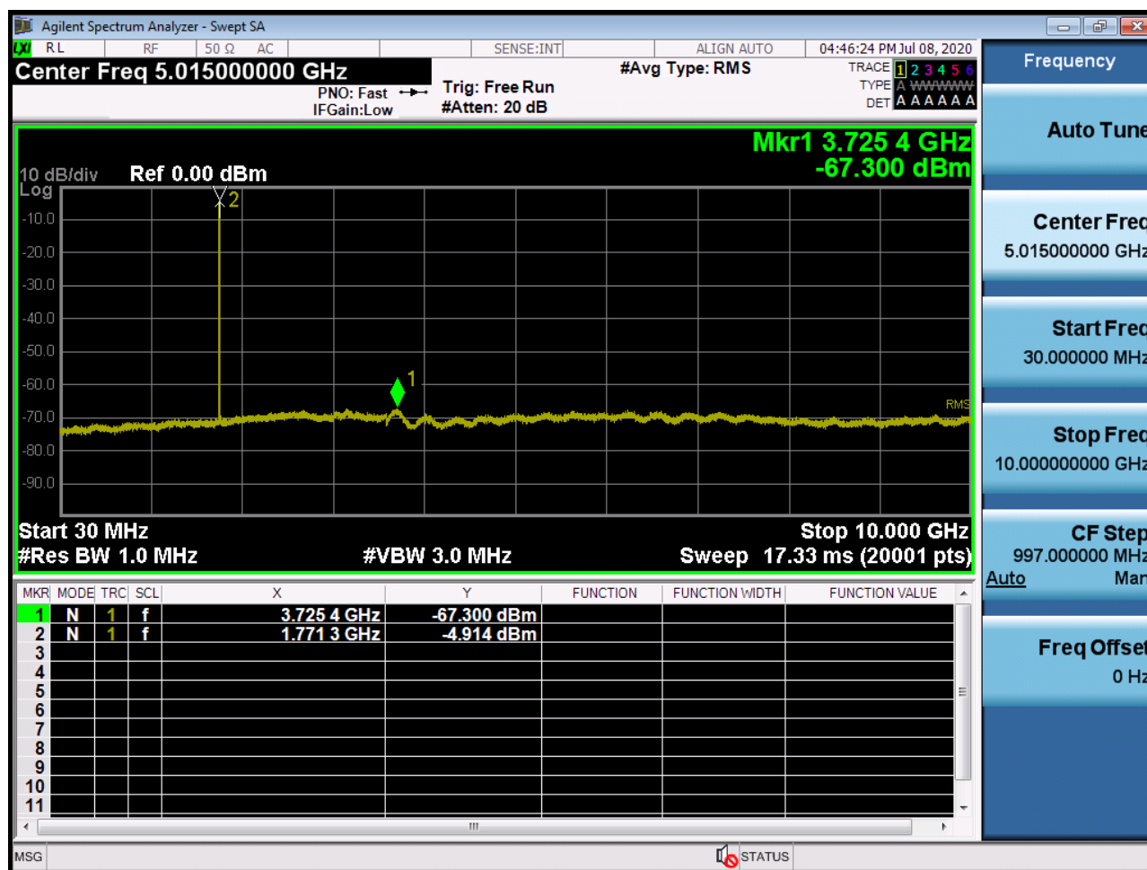
Sub6 n66. Conducted Spurious Plot_1 (355000ch_10MHz_BPSK_ RB 1_0)
