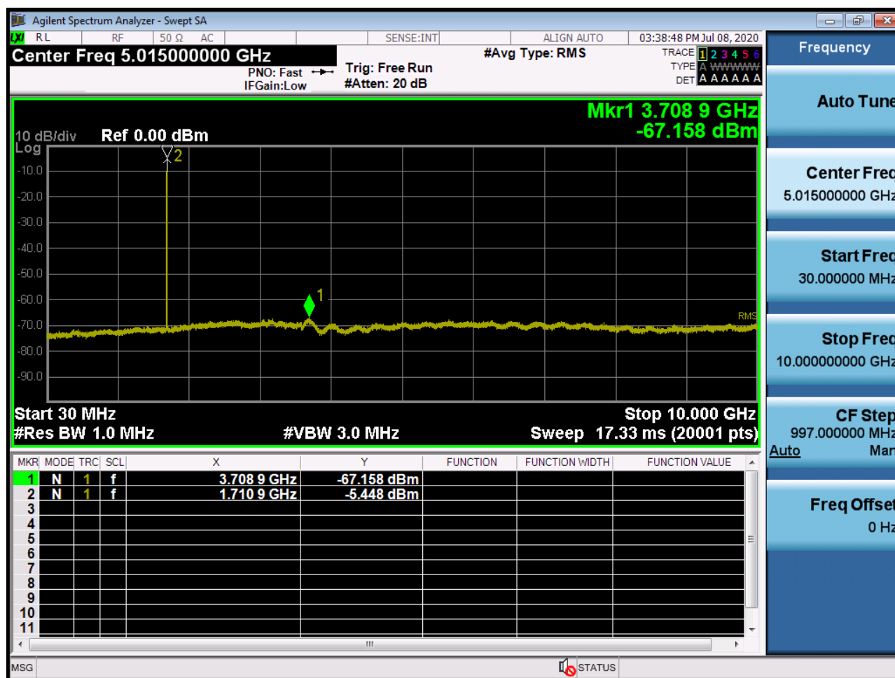
Sub6 n66. Conducted Spurious Plot_1 (342500ch_5MHz_BPSK_ RB 1_0)
