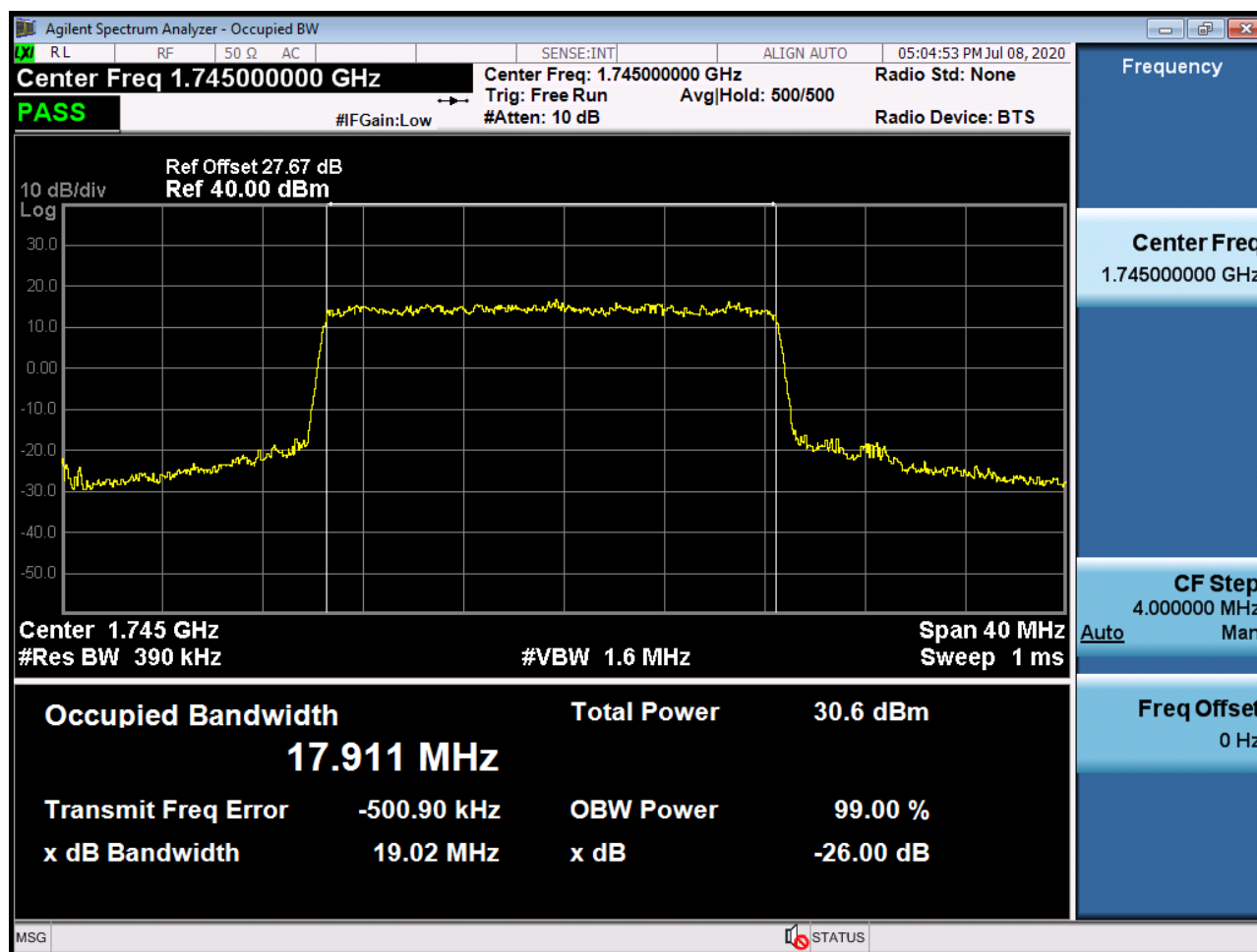
Sub6 n66. Occupied Bandwidth Plot (20M BW Ch.349000 QPSK RB 100)
