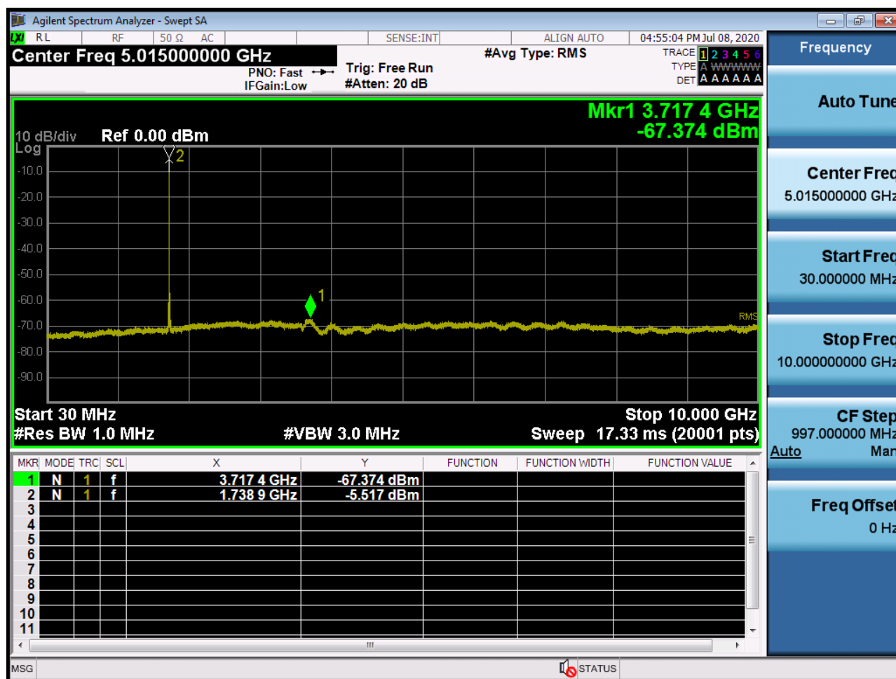
Sub6 n66. Conducted Spurious Plot_1 (349000ch_15MHz_BPSK_ RB 1_0)
