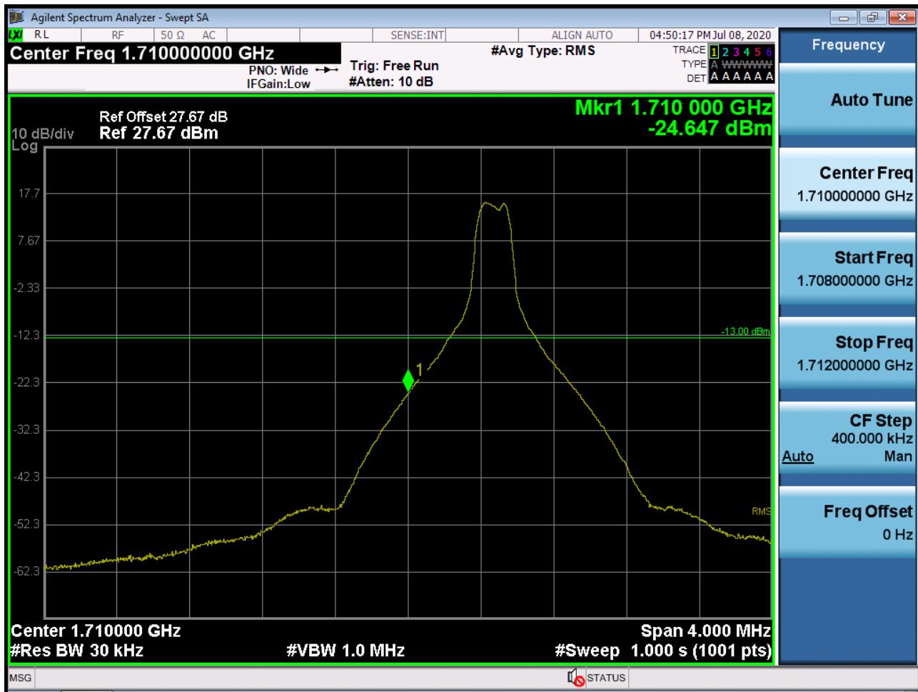
Sub6 n66. Lower Band Edge Plot (15M BW Ch.343500 BPSK RB 1, Offset 0) -1
