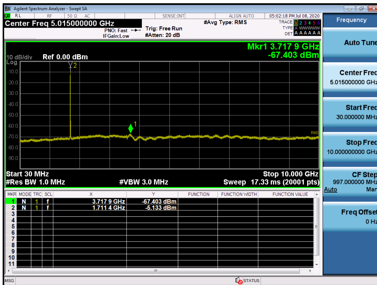
Sub6 n66. Conducted Spurious Plot_1 (344000ch_20MHz_BPSK_ RB 1_0)
