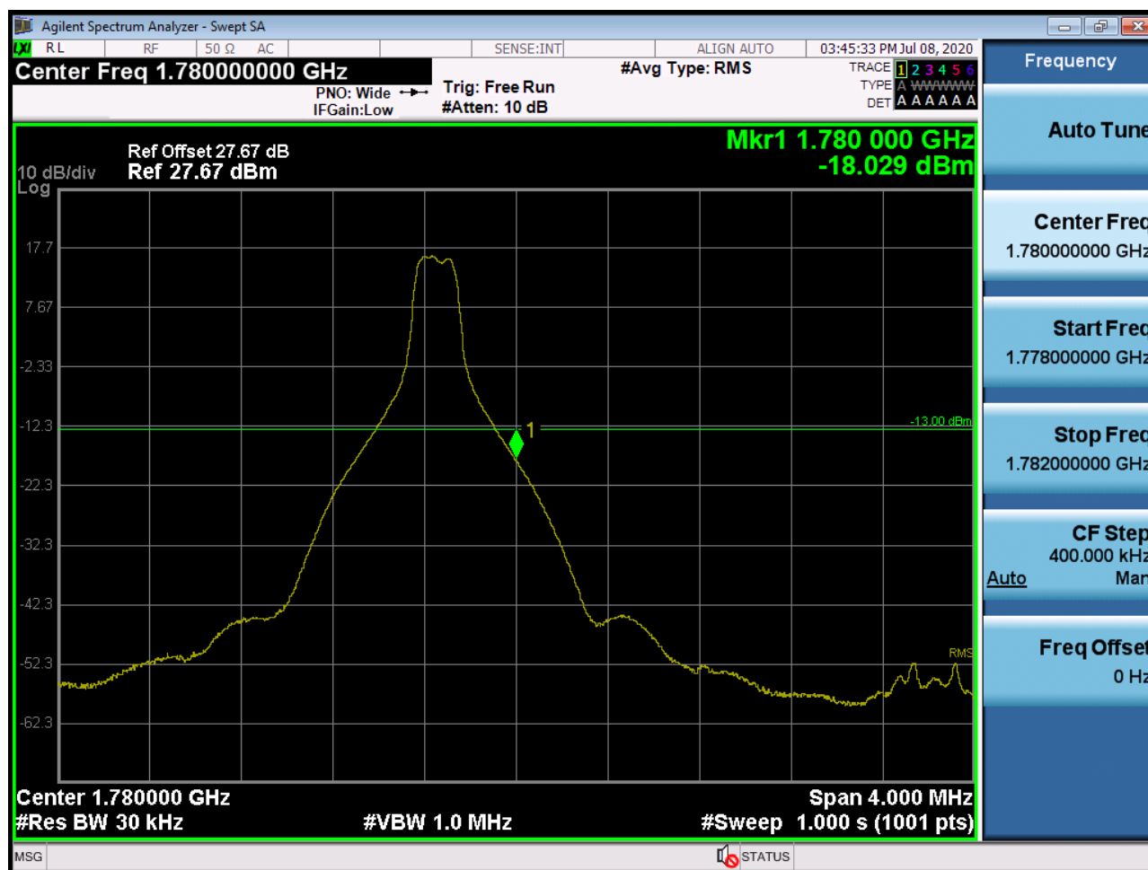
Sub6 n66. Upper Band Edge Plot (5M BW Ch.355500 BPSK_RB1_Offset 24) -1
