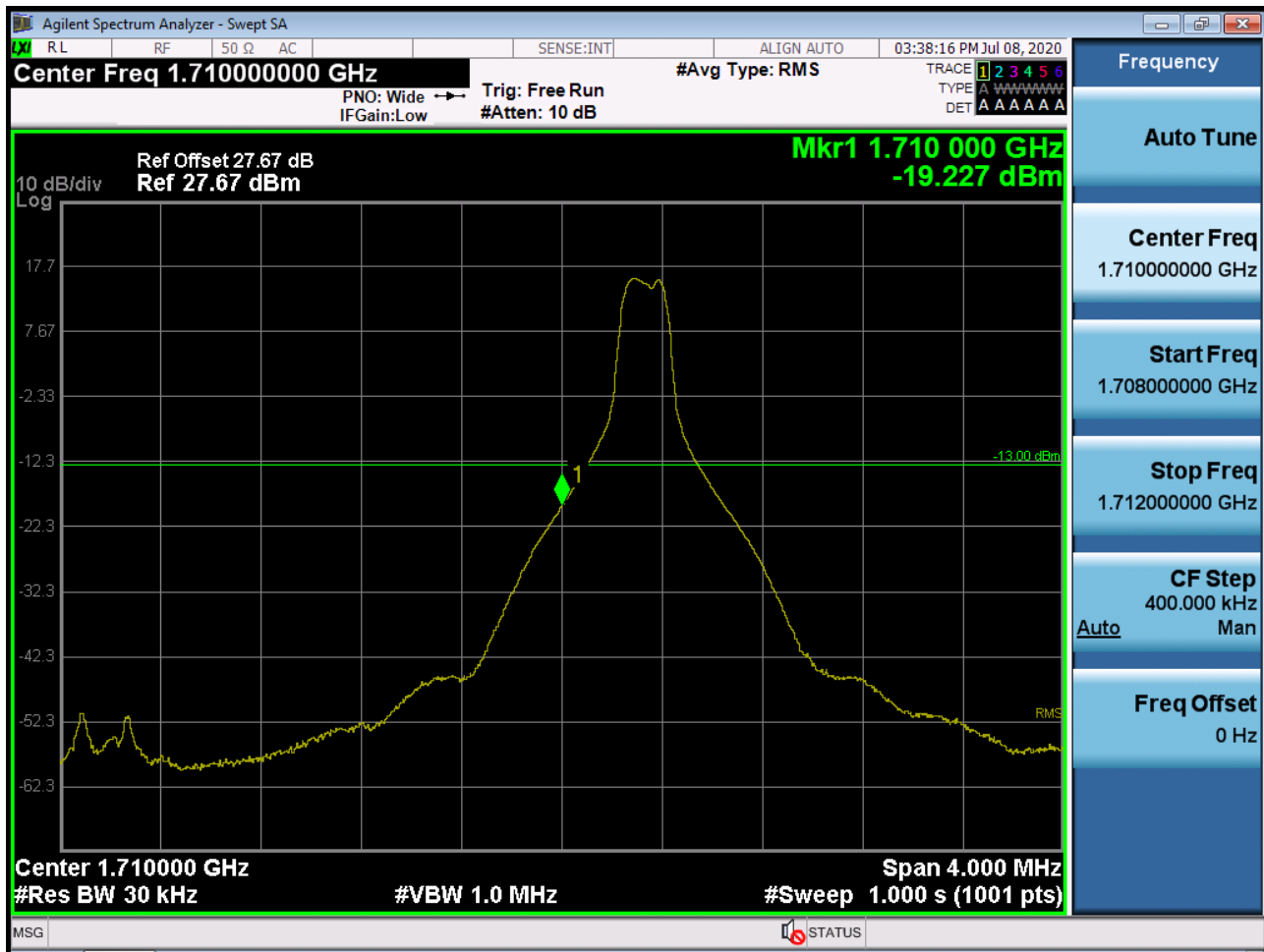
Sub6 n66. Lower Band Edge Plot (5M BW Ch.342500 BPSK RB 1, Offset 0) -1
