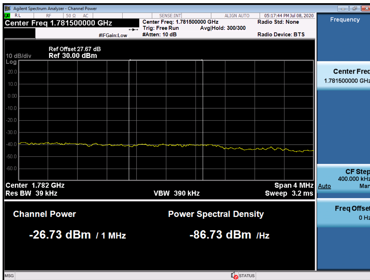
Sub6 n66. Upper Extended Band Edge Plot (20M BW Ch.354000 BPSK_RB100_0) -3
