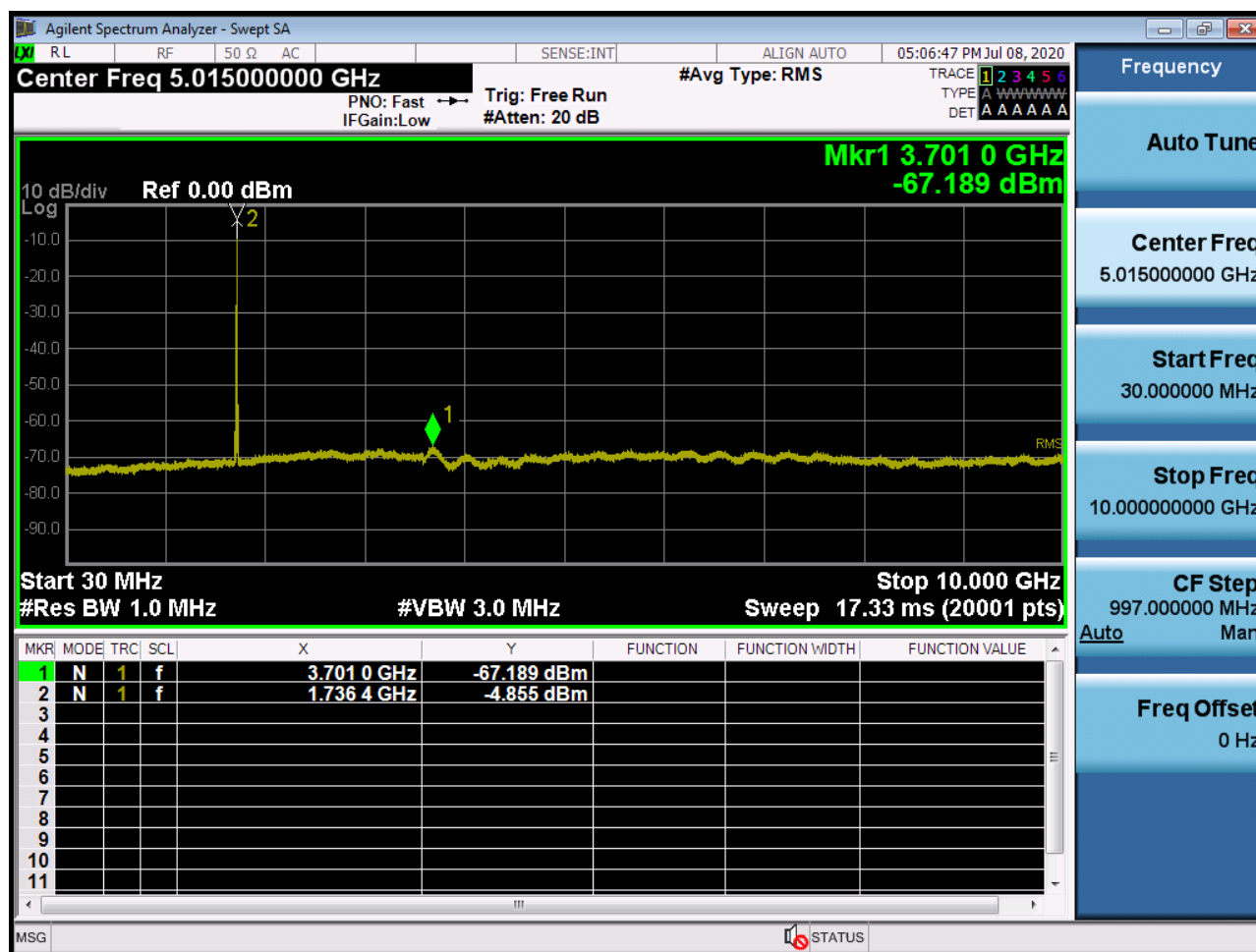
Sub6 n66. Conducted Spurious Plot_1 (349000ch_20MHz_BPSK_ RB 1_0)
