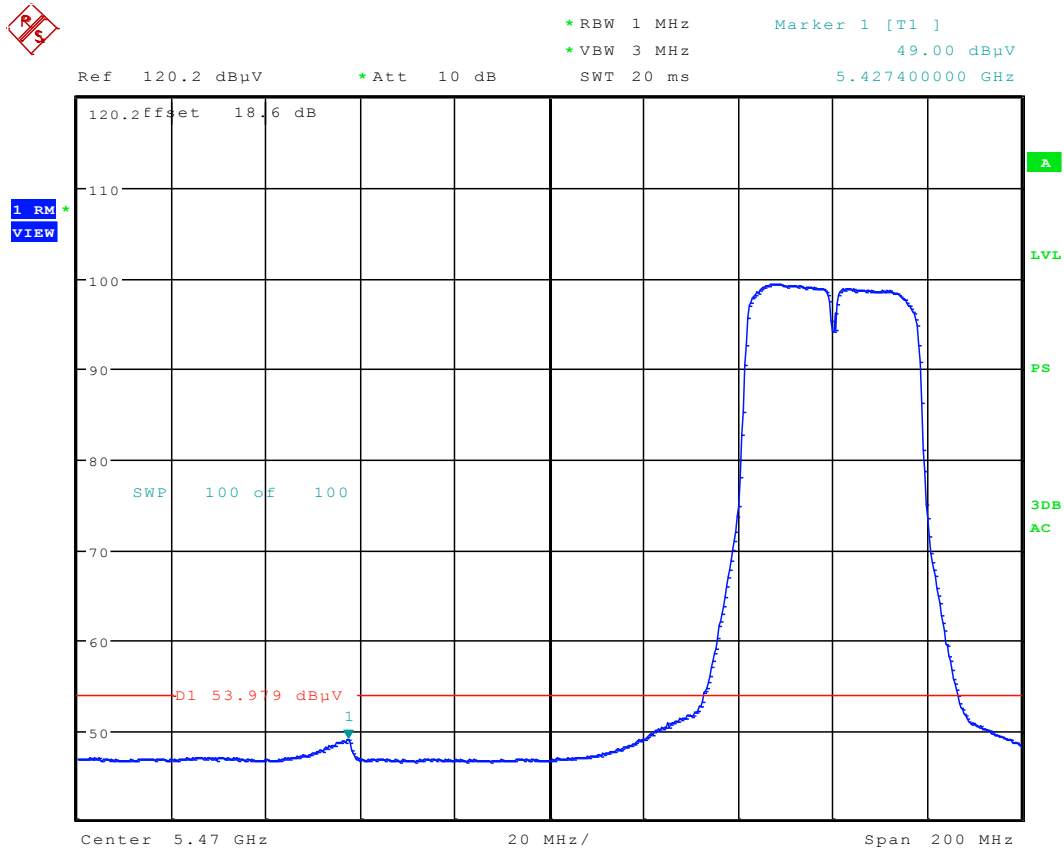
Plot 6-70. Radiated Restricted Lower Band Edge Plot (Average – UNII Band 2C)
