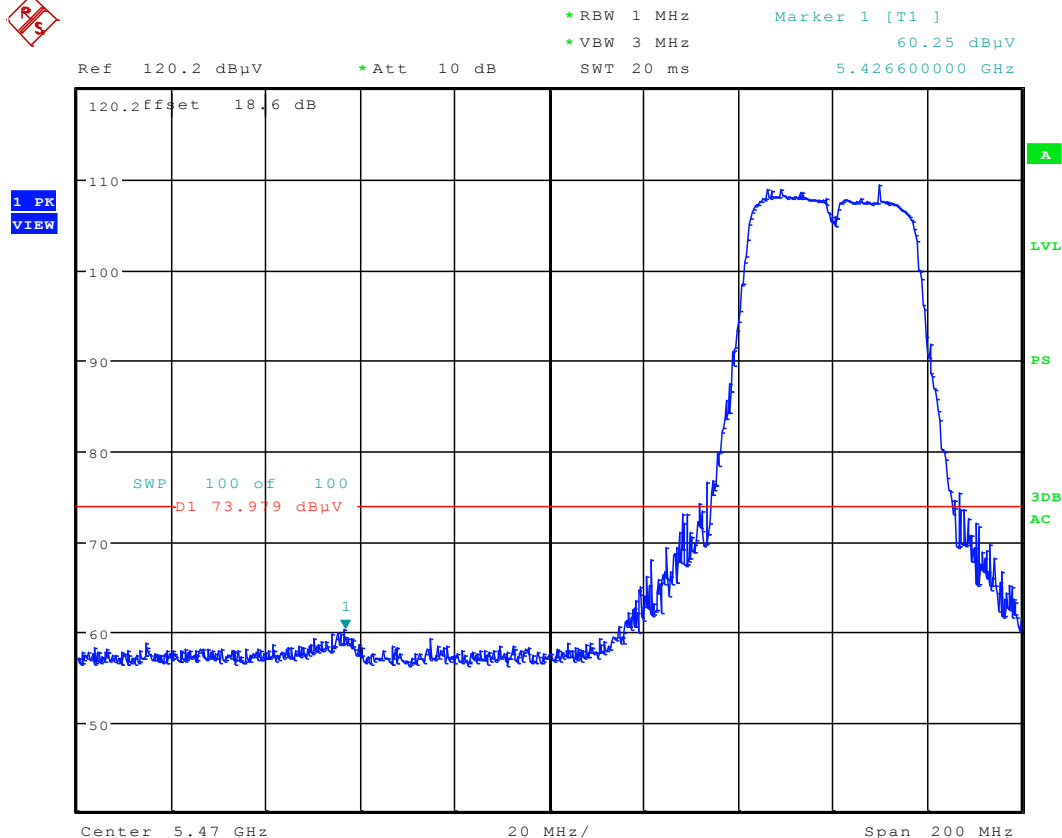
Plot 6-71. Radiated Restricted Lower Band Edge Plot (Peak – UNII Band 2C)
