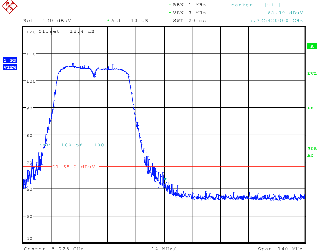
Plot 6-72. Radiated Upper Band Edge Plot (Peak – UNII Band 2C)
