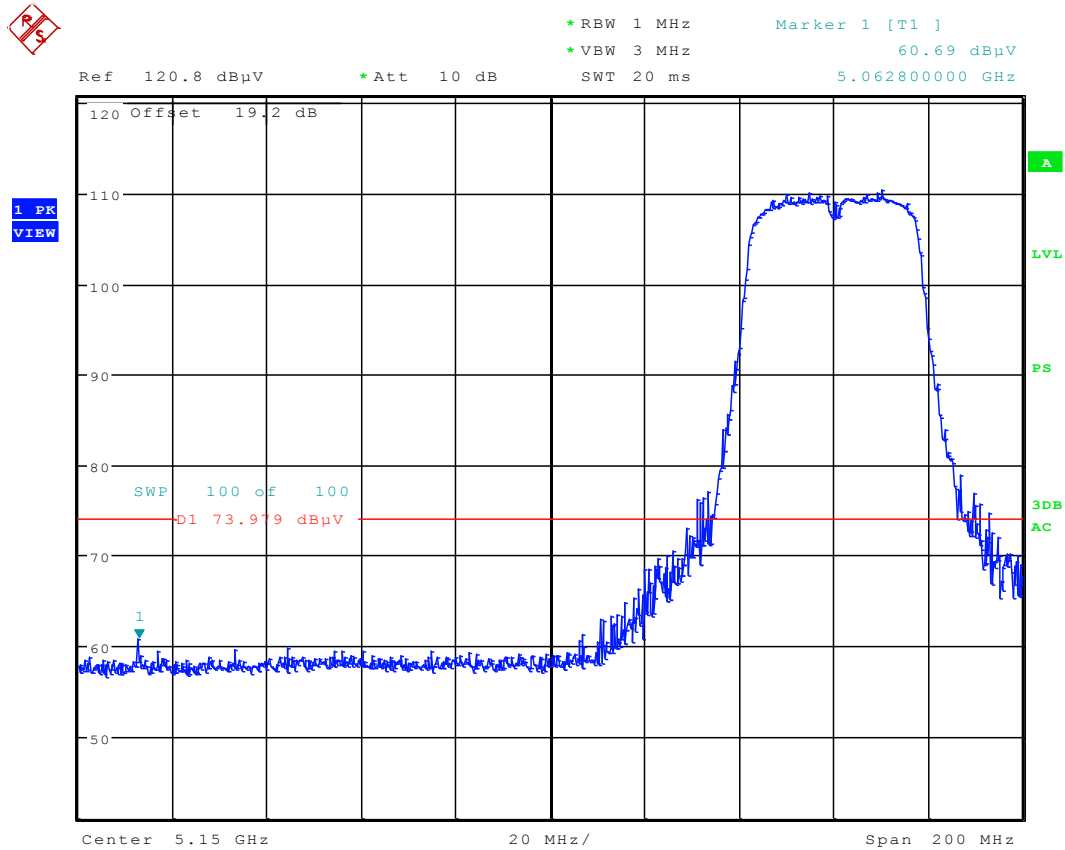
Plot 6-67. Radiated Restricted Lower Band Edge Plot (Peak – UNII Band 1)
