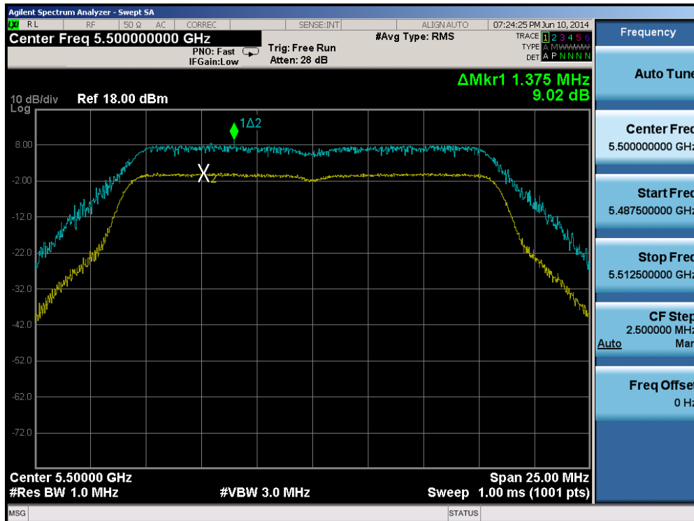
Plot 6-58. Peak Excursion Ratio Plot (802.11a (UNII Band 2C) – Ch. 100)
