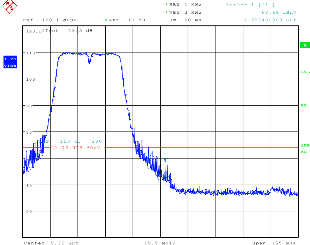
Plot 6-69. Radiated Restricted Upper Band Edge Plot (Peak – UNII Band 2A)
