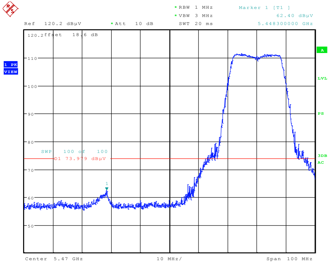
Plot 6-64. Radiated Restricted Lower Band Edge Plot (Peak – UNII Band 2C)
