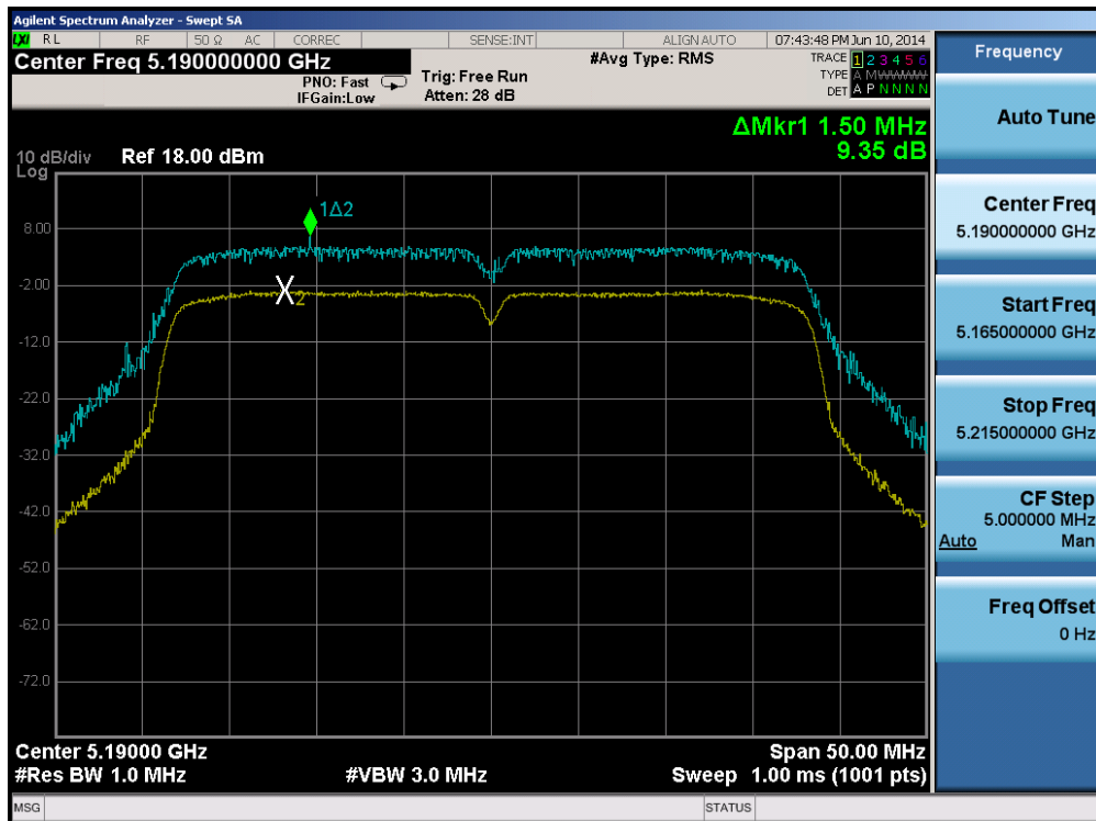
Plot 6-56. Peak Excursion Ratio Plot (40MHz BW 802.11n (UNII Band 1) – Ch. 38)
