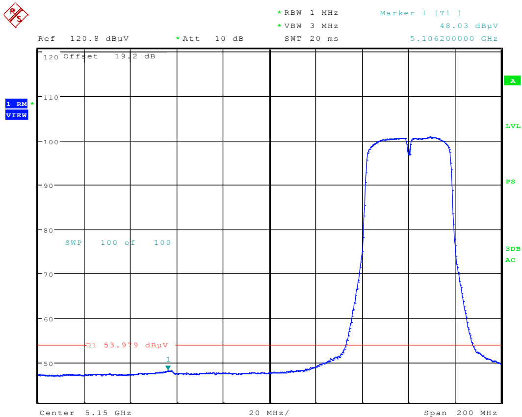
Plot 6-66. Radiated Restricted Lower Band Edge Plot (Average – UNII Band 1)
