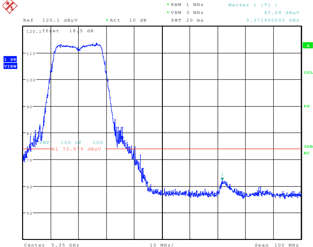
Plot 6-62. Radiated Restricted Upper Band Edge Plot (Peak – UNII Band 2A)
