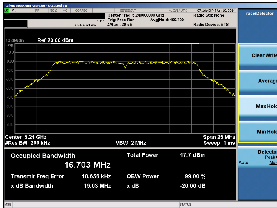
Plot 6-26. 20dB Bandwidth Plot (20MHz BW 802.11a/n (UNII Band 1) – Ch. 48)
