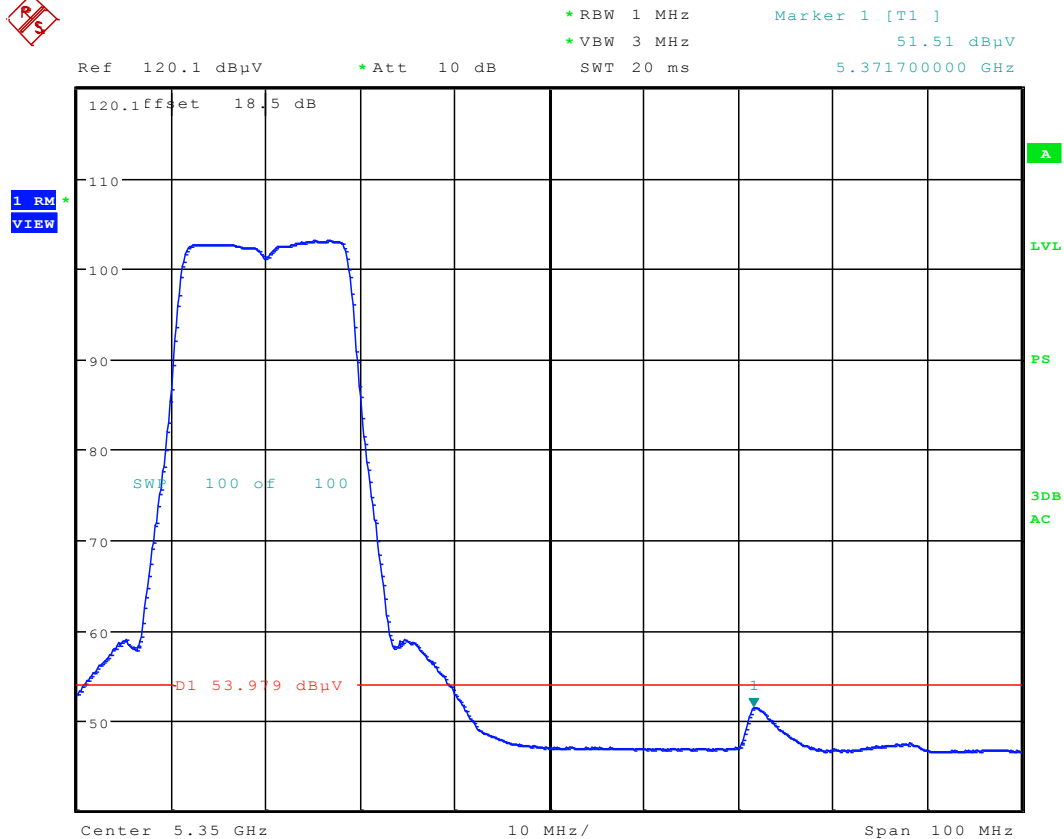
Plot 6-61. Radiated Restricted Upper Band Edge Plot (Average – UNII Band 2A)
