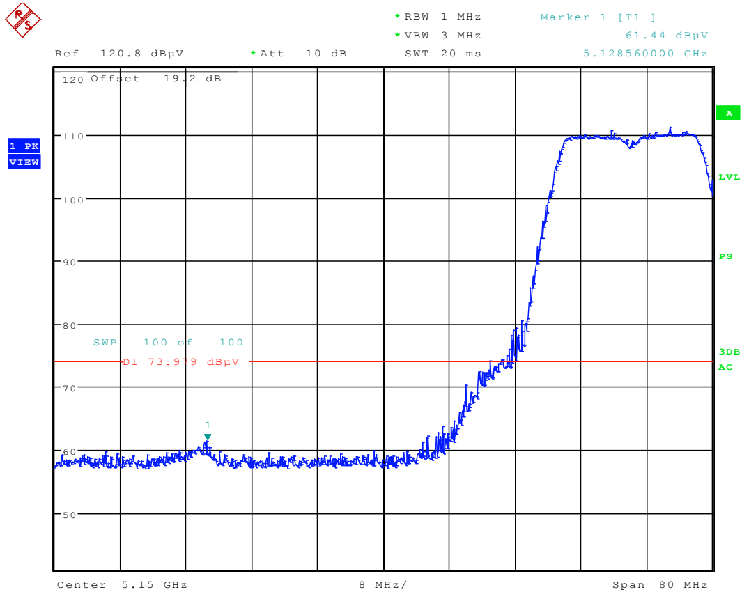
Plot 6-60. Radiated Restricted Lower Band Edge Plot (Peak – UNII Band 1)
