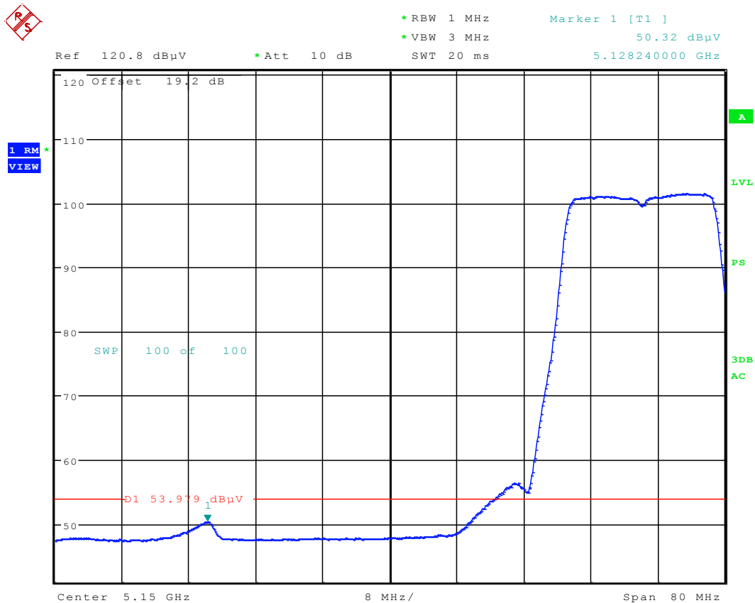
Plot 6-59. Radiated Restricted Lower Band Edge Plot (Average – UNII Band 1)
