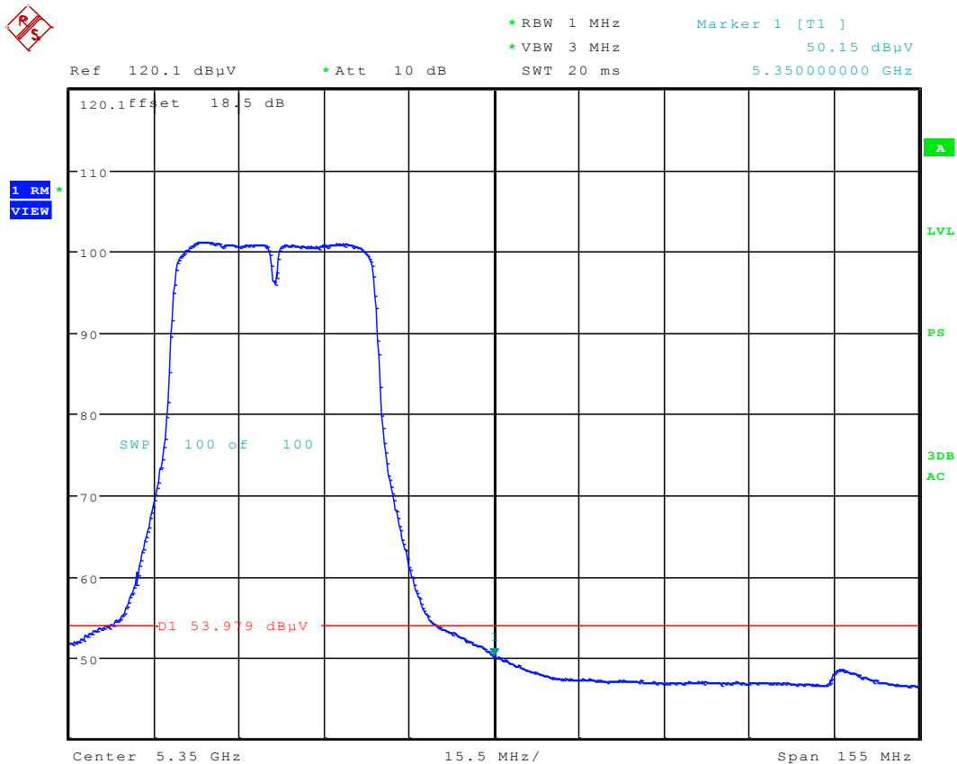
Plot 6-68. Radiated Restricted Upper Band Edge Plot (Average – UNII Band 2A)
