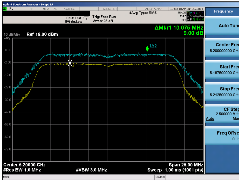
Plot 6-57. Peak Excursion Ratio Plot (20MHz BW 802.11n (UNII Band 1) – Ch. 40)
