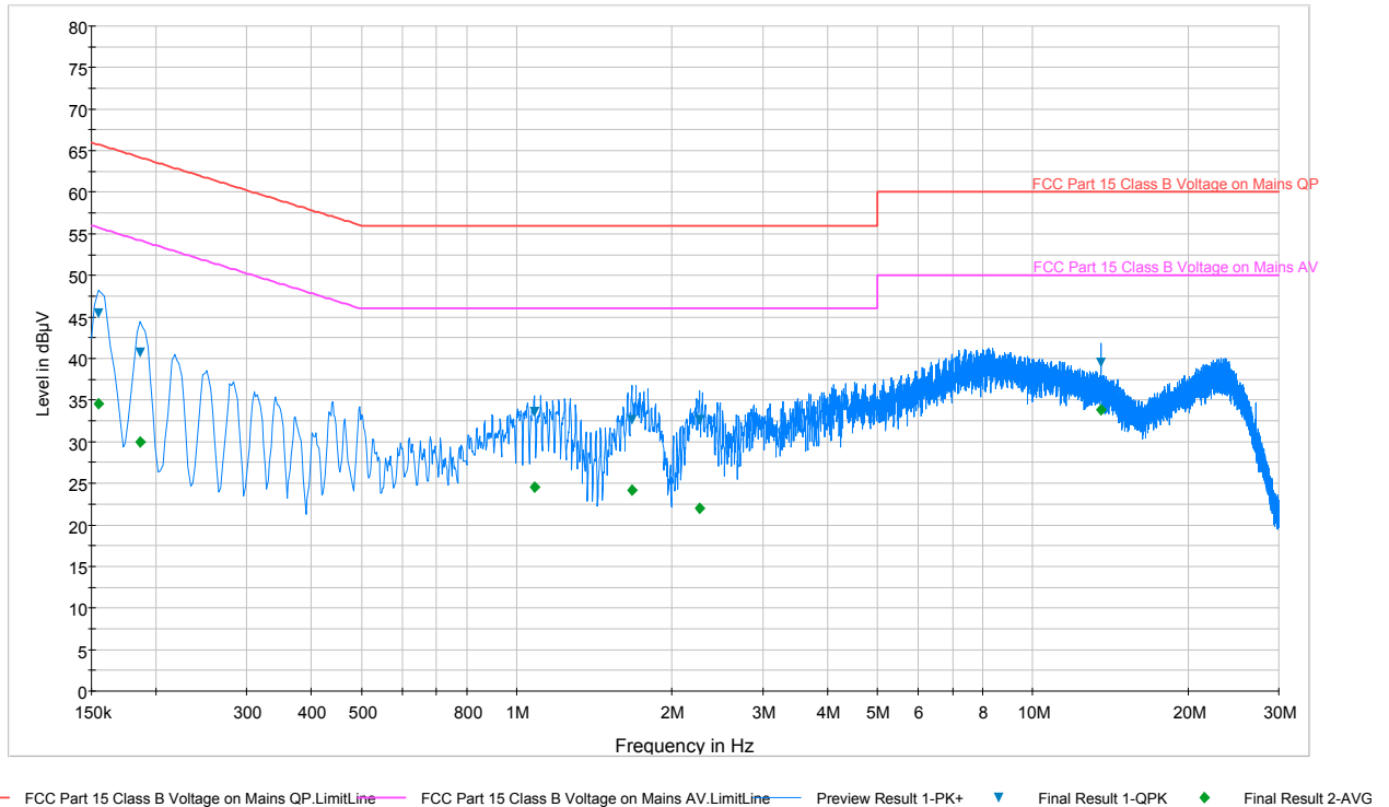
Plot 8-1. Line-Conducted Test Plot (L1)
