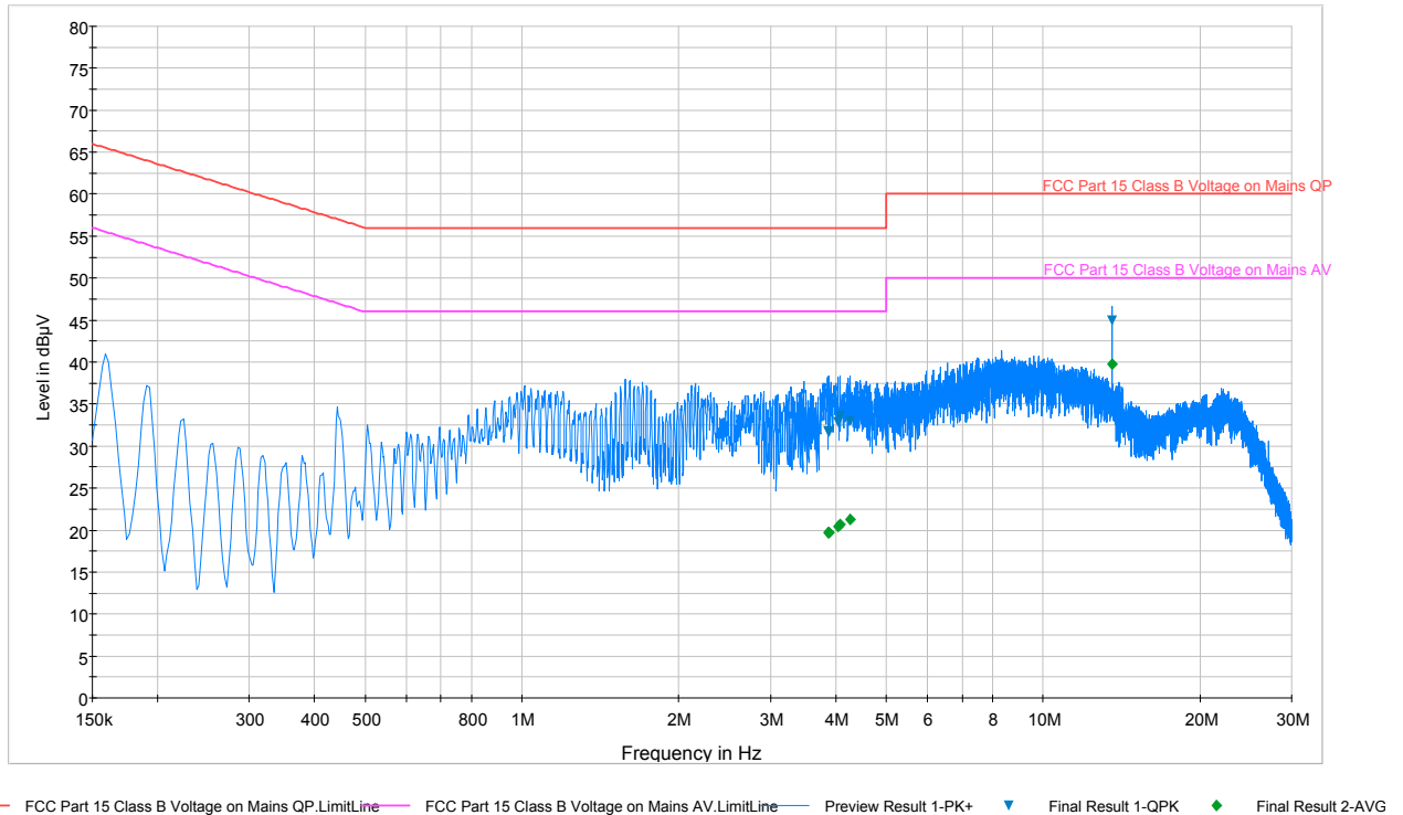
Plot 8-2. Line-Conducted Test Plot (N)
