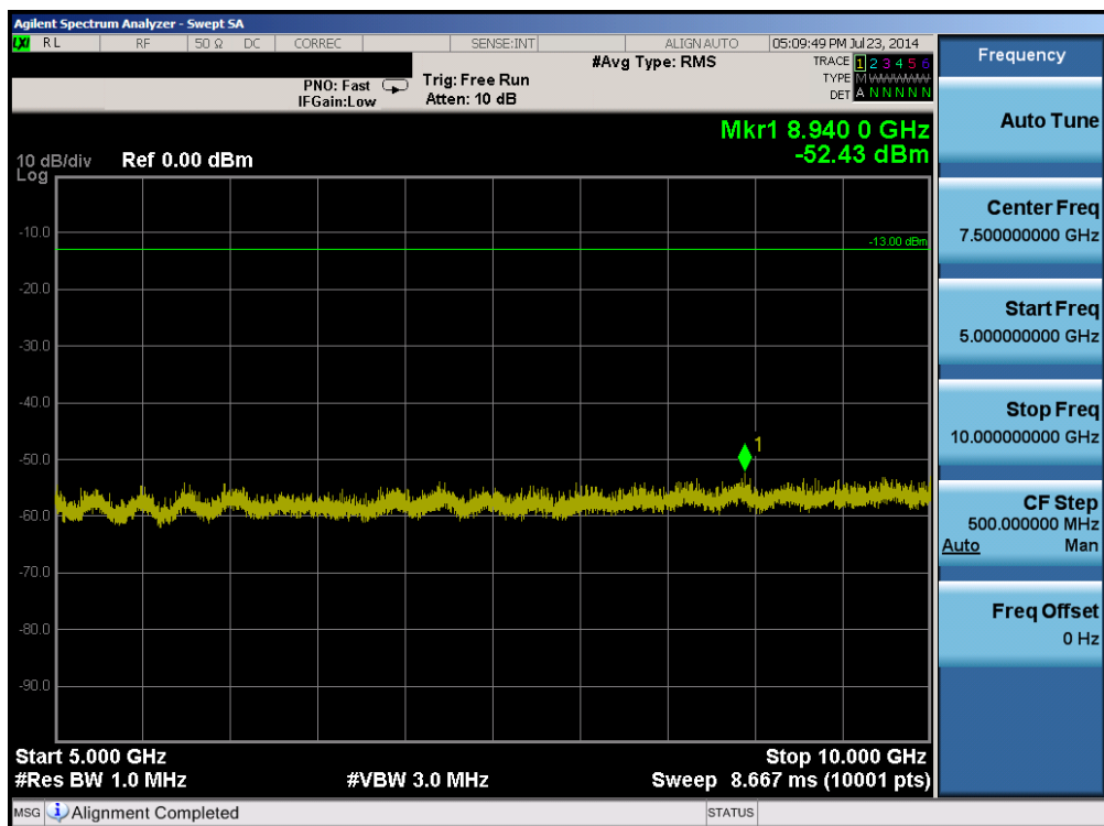
Plot 6-46. Conducted Spurious Plot (Band 5 – 10.0MHz QPSK – RB Size 1, RB Offset 0 – Mid Channel)
