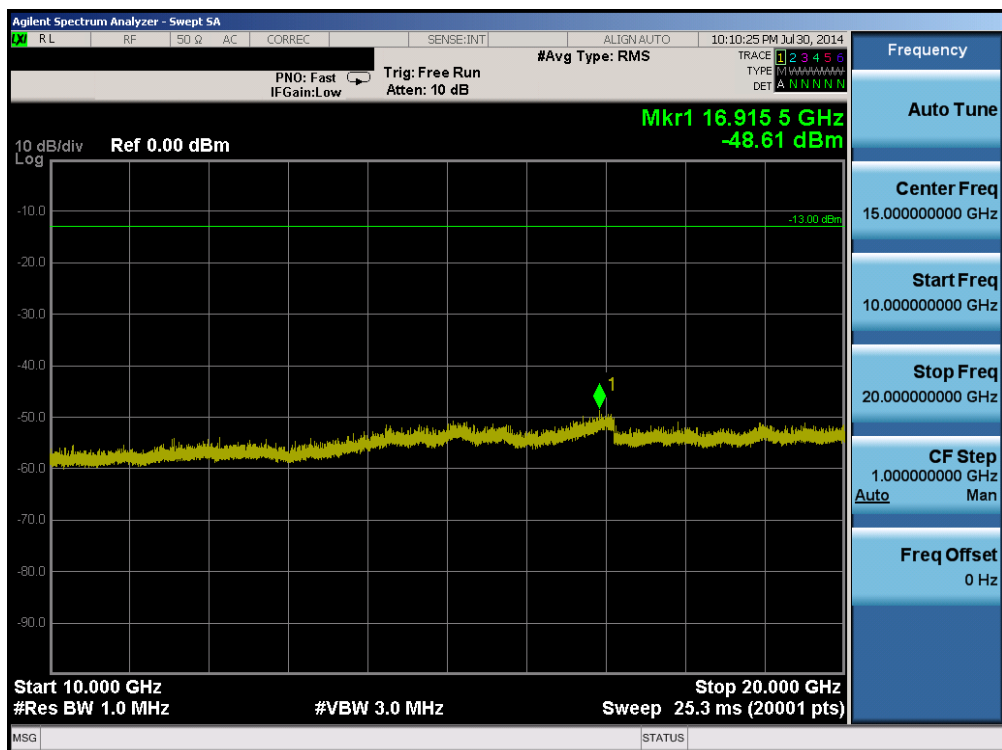
Plot 6-50. Conducted Spurious Plot (Band 4 – 20.0MHz QPSK – RB Size 1, RB Offset 0 – Low Channel)
