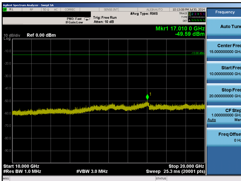
Plot 6-54. Conducted Spurious Plot (Band 4 – 20.0MHz QPSK – RB Size 1, RB Offset 0 – High Channel)
