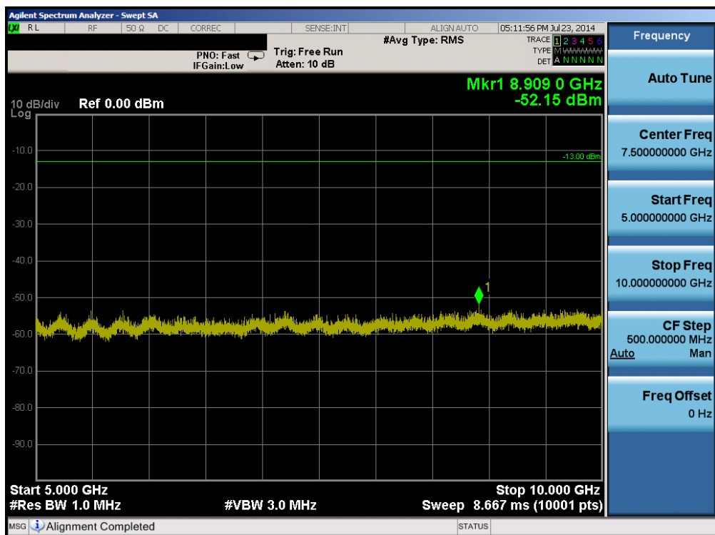
Plot 6-44. Conducted Spurious Plot (Band 5 – 10.0MHz QPSK – RB Size 1, RB Offset 0 – Low Channel)
