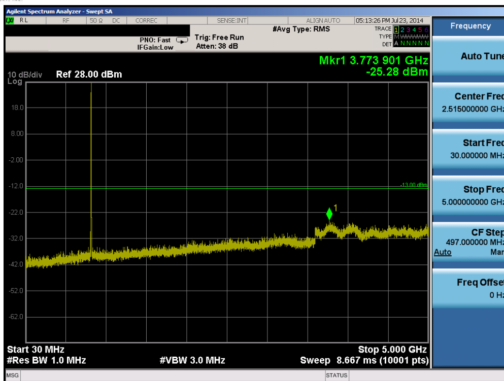
Plot 6-47. Conducted Spurious Plot (Band 5 – 10.0MHz QPSK – RB Size 1, RB Offset 0 – High Channel)
