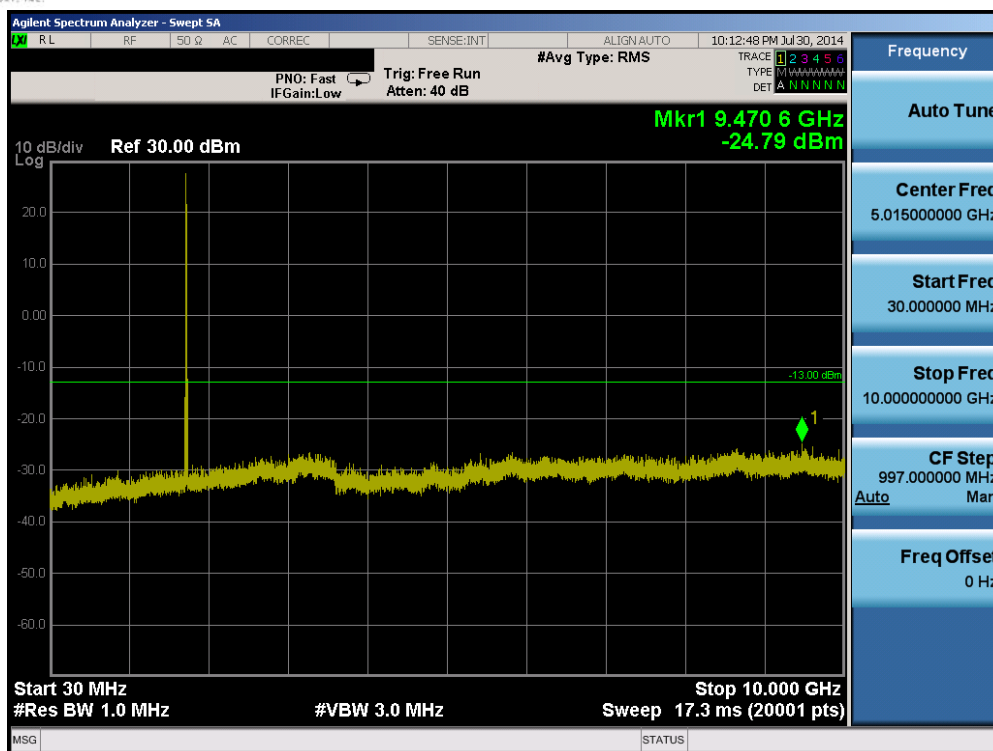
Plot 6-53. Conducted Spurious Plot (Band 4 – 20.0MHz QPSK – RB Size 1, RB Offset 0 – High Channel)
