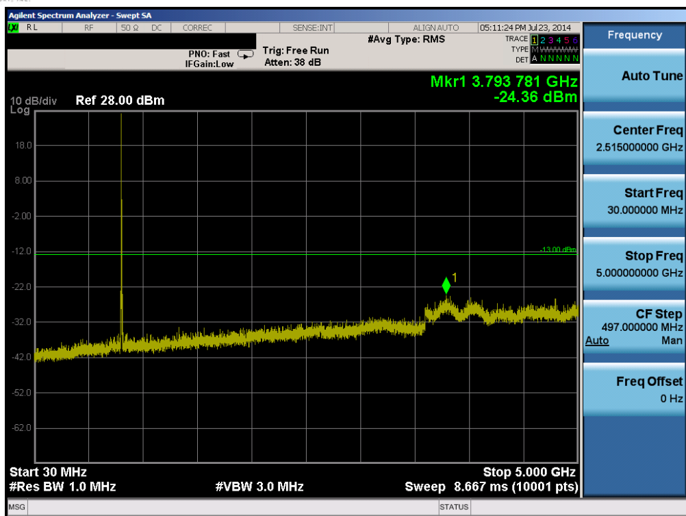
Plot 6-43. Conducted Spurious Plot (Band 5 – 10.0MHz QPSK – RB Size 1, RB Offset 0– Low Channel)
