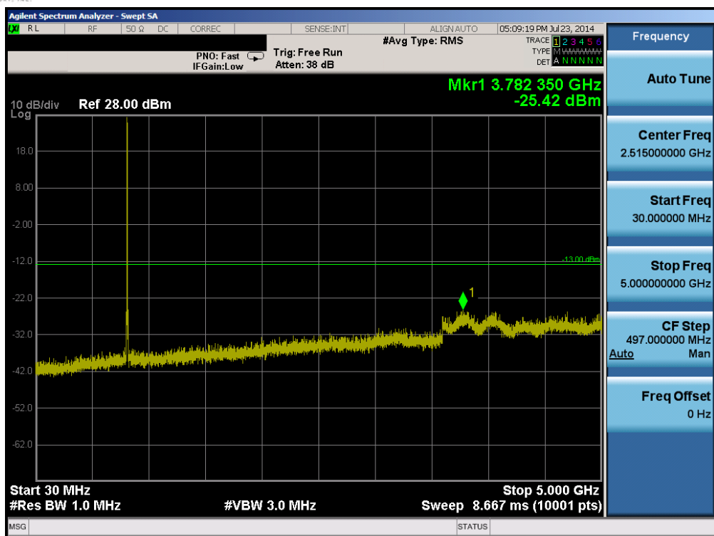
Plot 6-45. Conducted Spurious Plot (Band 5 – 10.0MHz QPSK – RB Size 1, RB Offset 0 – Mid Channel)
