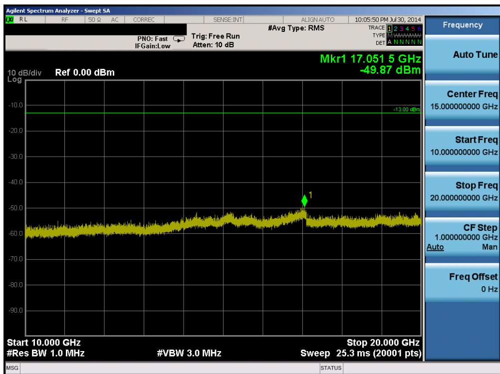
Plot 6-52. Conducted Spurious Plot (Band 4 – 20.0MHz QPSK – RB Size 1, RB Offset 0 – Mid Channel)
