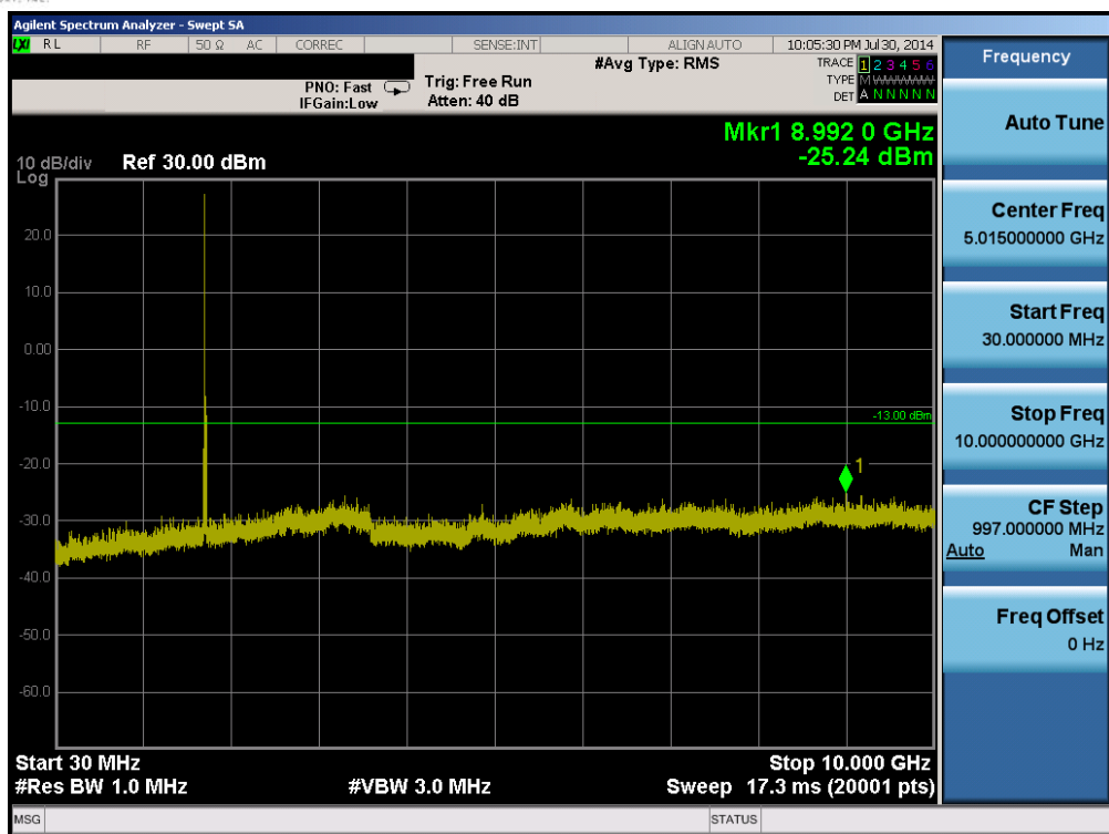
Plot 6-51. Conducted Spurious Plot (Band 4 – 20.0MHz QPSK – RB Size 1, RB Offset 0 – Mid Channel)
