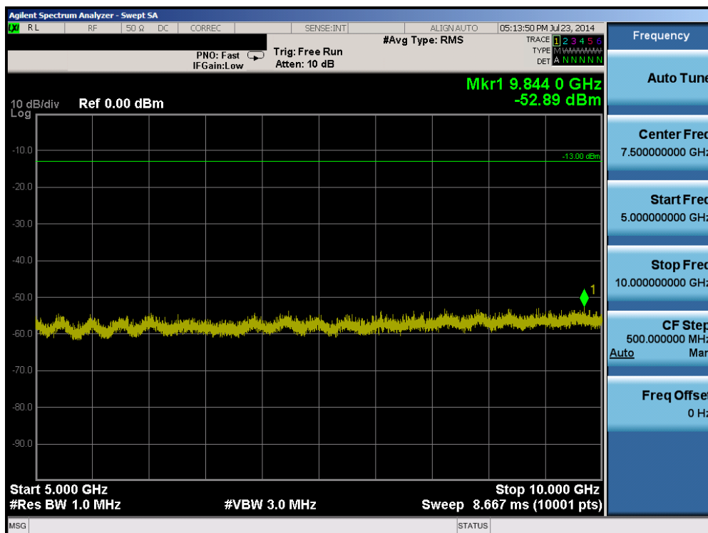
Plot 6-48. Conducted Spurious Plot (Band 5 – 10.0MHz QPSK – RB Size 1, RB Offset 0 – High Channel)
