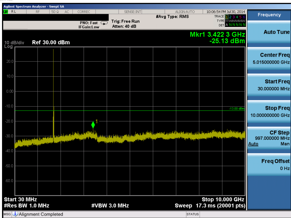
Plot 6-49. Conducted Spurious Plot (Band 4 – 20.0MHz QPSK – RB Size 1, RB Offset 0– Low Channel)
