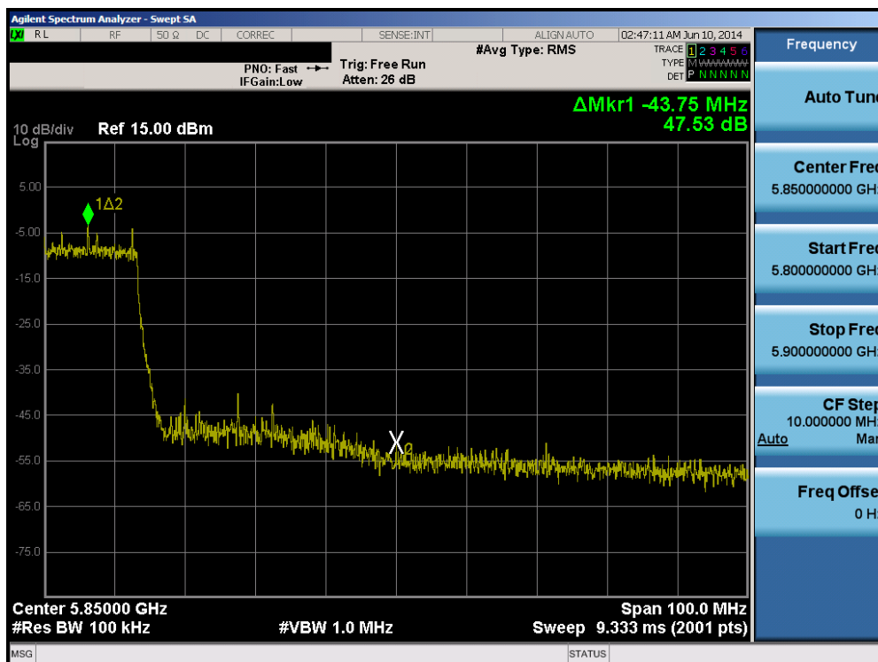
Plot 6-84. Band Edge Plot (40MHz BW 802.11n (5.8GHz) – Ch. 161)
