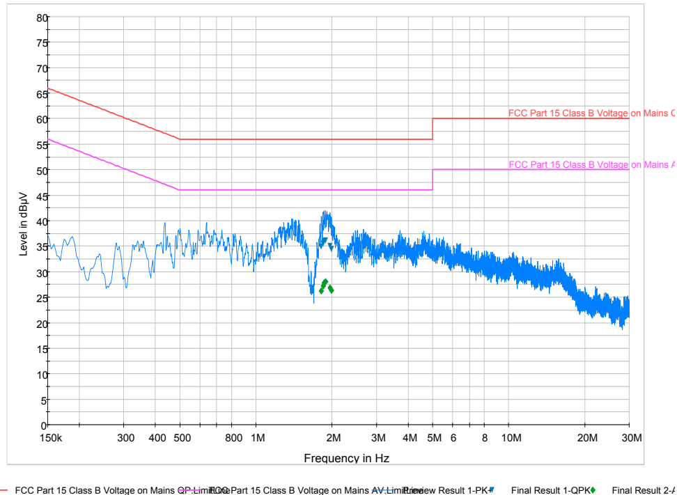
Plot 6-45. Line-Conducted Test Plot (N)
