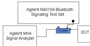
Figure 6-2. Test Instrument & Measurement Setup
