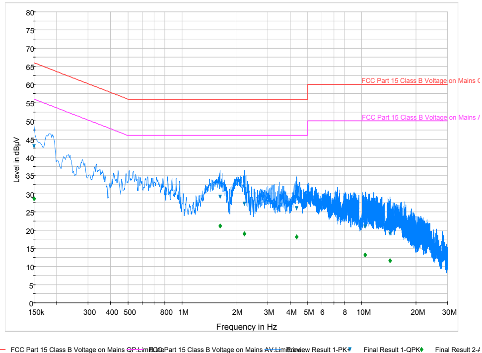
Plot 6-44. Line-Conducted Test Plot (L1)
