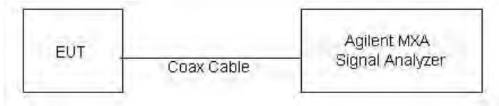
Figure 8-5 Power Measurement Setup for Bandwidths > 50 MHz
