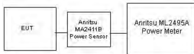
Figure 8-4 Power Measurement Setup for Bandwidths < 50 MHz
