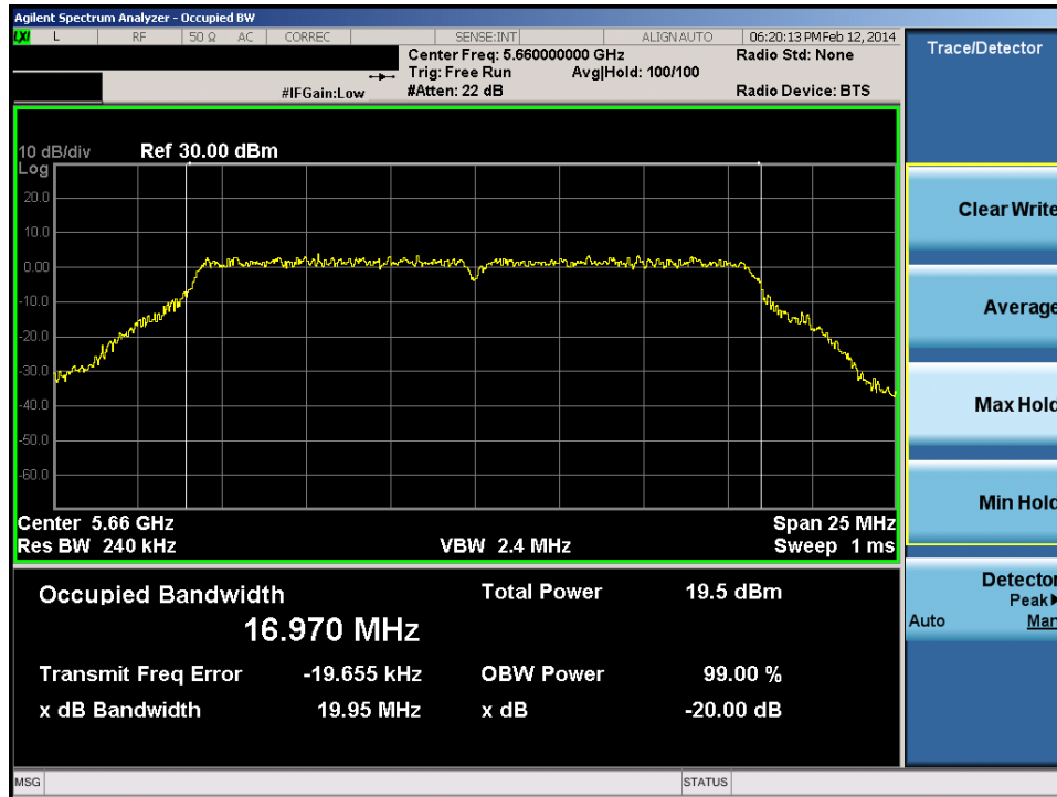
Plot 6-68. 20dB Bandwidth Plot (20MHz BW 802.11a (UNII Band 2C) – Ch. 132)
