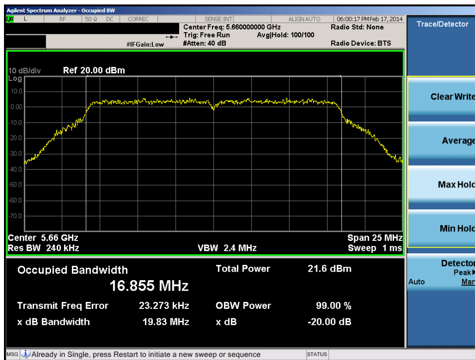
Plot 6-69. 20dB Bandwidth Plot (20MHz BW 802.11n (UNII Band 2C) – Ch. 132)
