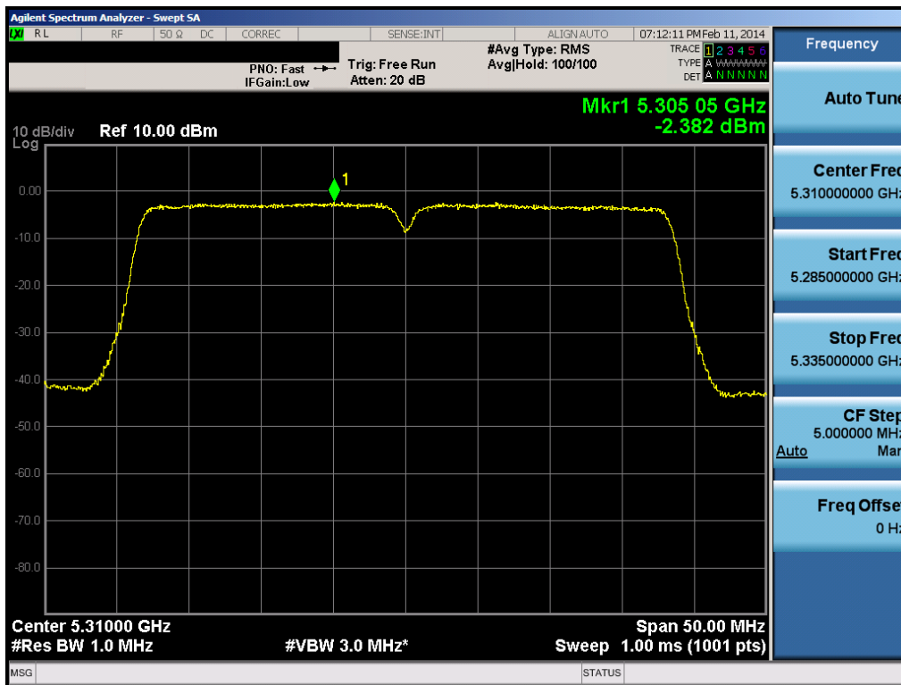
Plot 6-115. Peak Power Spectral Density Plot (40MHz BW 802.11n (UNII Band 2A) – Ch. 62)
