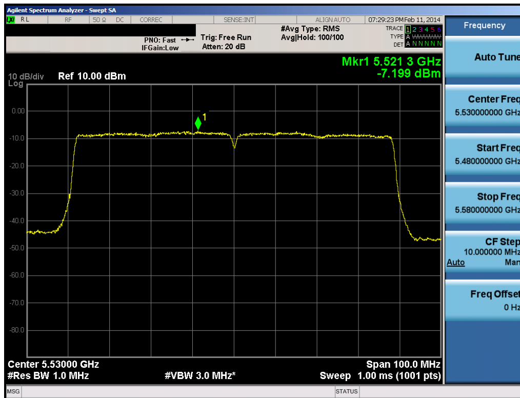
Plot 6-126. Peak Power Spectral Density Plot (80MHz BW 802.11ac (UNII Band 2C) – Ch. 106)
