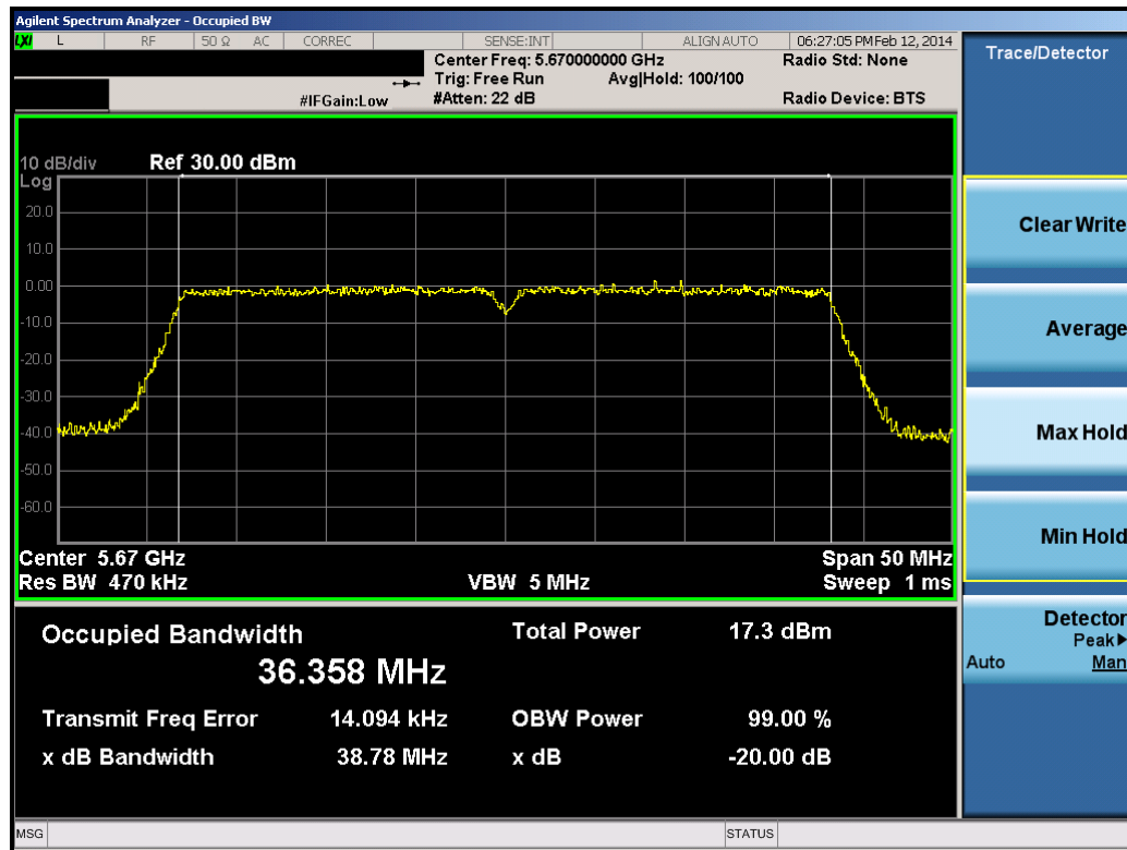
Plot 6-70. 20dB Bandwidth Plot (40MHz BW 802.11N (UNII Band 2C) – Ch. 134)
