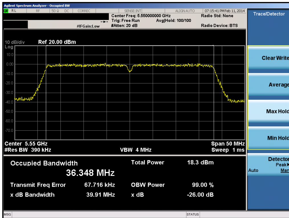
Plot 6-61. 26dB Bandwidth Plot (40MHz BW 802.11n (UNII Band 2C) – Ch. 110)
