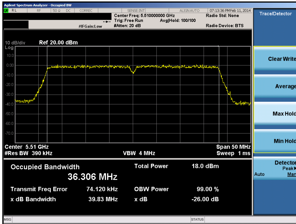
Plot 6-60. 26dB Bandwidth Plot (40MHz BW 802.11n (UNII Band 2C) – Ch. 102)
