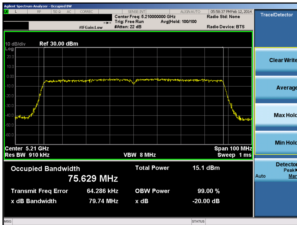
Plot 6-32. 20dB Bandwidth Plot (80MHz BW 802.11ac (UNII Band 1) – Ch. 42)
