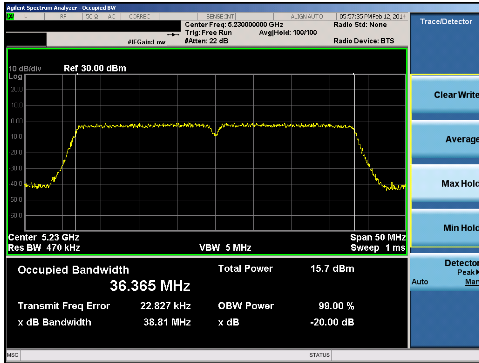
Plot 6-31. 20dB Bandwidth Plot (40MHz BW 802.11n (UNII Band 1) – Ch. 46)
