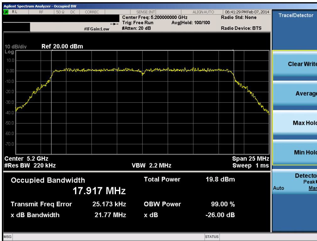
Plot 6-40. 26dB Bandwidth Plot (20MHz BW 802.11n (UNII Band 1) – Ch. 40)
