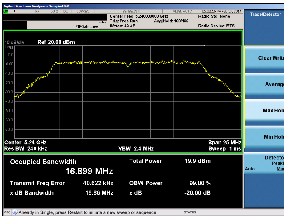
Plot 6-65. 20dB Bandwidth Plot (20MHz BW 802.11n (UNII Band 1) – Ch. 48)
