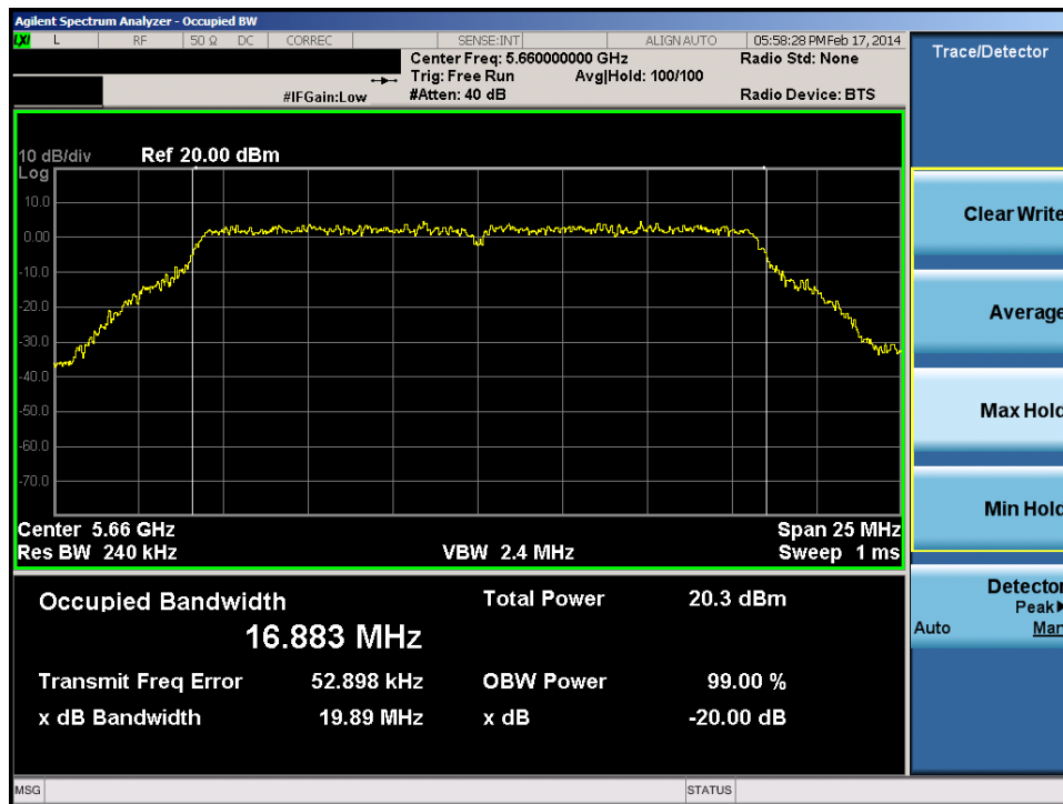
Plot 6-34. 20dB Bandwidth Plot (20MHz BW 802.11n (UNII Band 2C) – Ch. 132)
