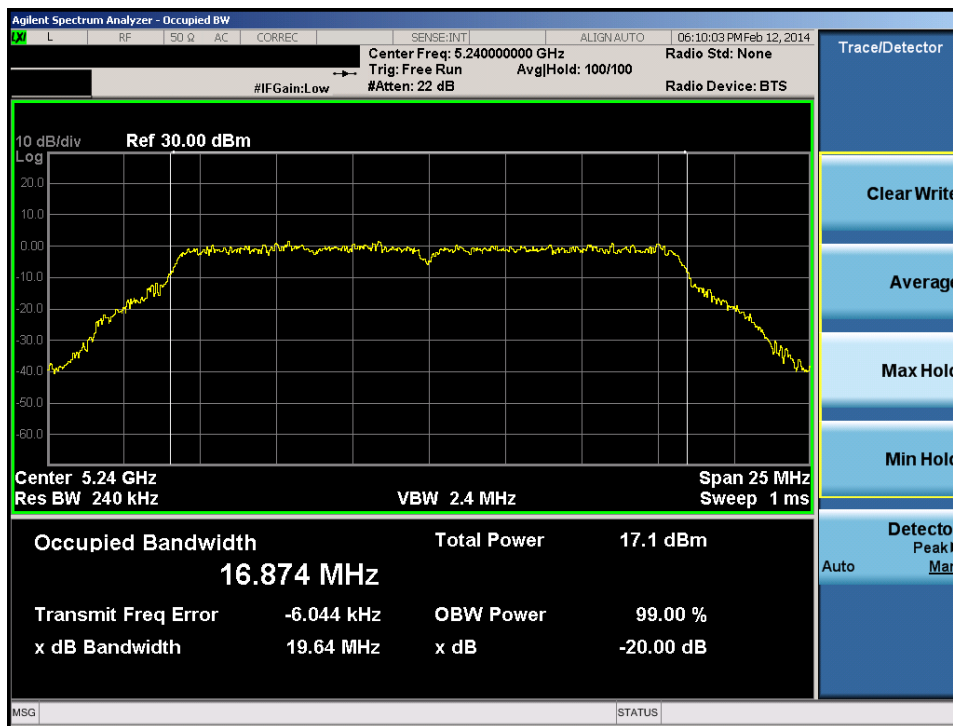
Plot 6-64. 20dB Bandwidth Plot (20MHz BW 802.11a (UNII Band 1) – Ch. 48)
