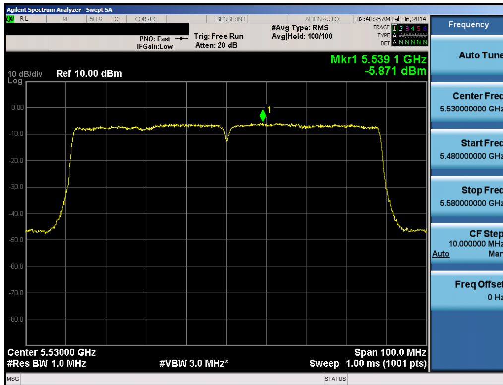
Plot 6-98. Peak Power Spectral Density Plot (80MHz BW 802.11ac (UNII Band 2C) – Ch. 106)
