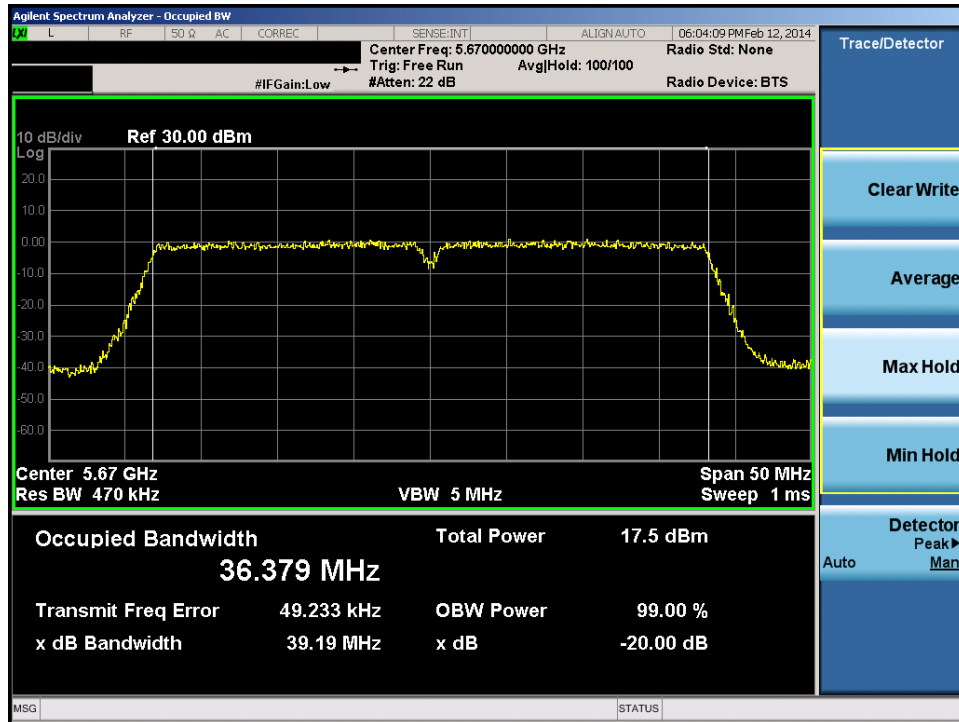
Plot 6-35. 20dB Bandwidth Plot (40MHz BW 802.11N (UNII Band 2C) – Ch. 134)
