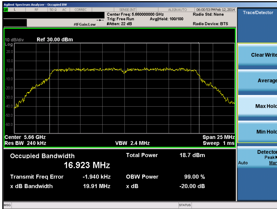
Plot 6-33. 20dB Bandwidth Plot (20MHz BW 802.11a (UNII Band 2C) – Ch. 132)
