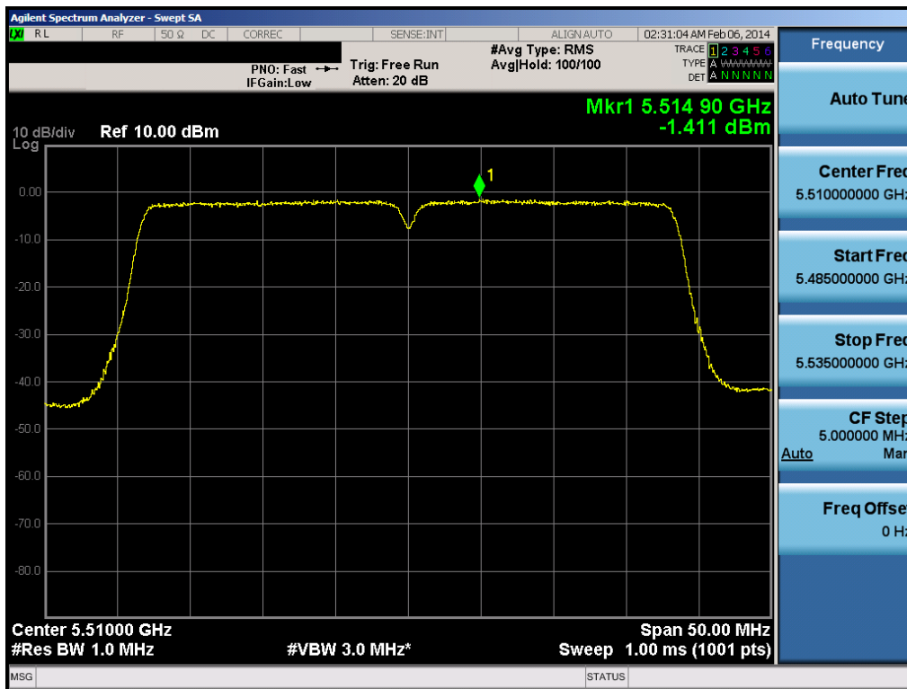
Plot 6-95. Peak Power Spectral Density Plot (40MHz BW 802.11n (UNII Band 2C) – Ch. 102)
