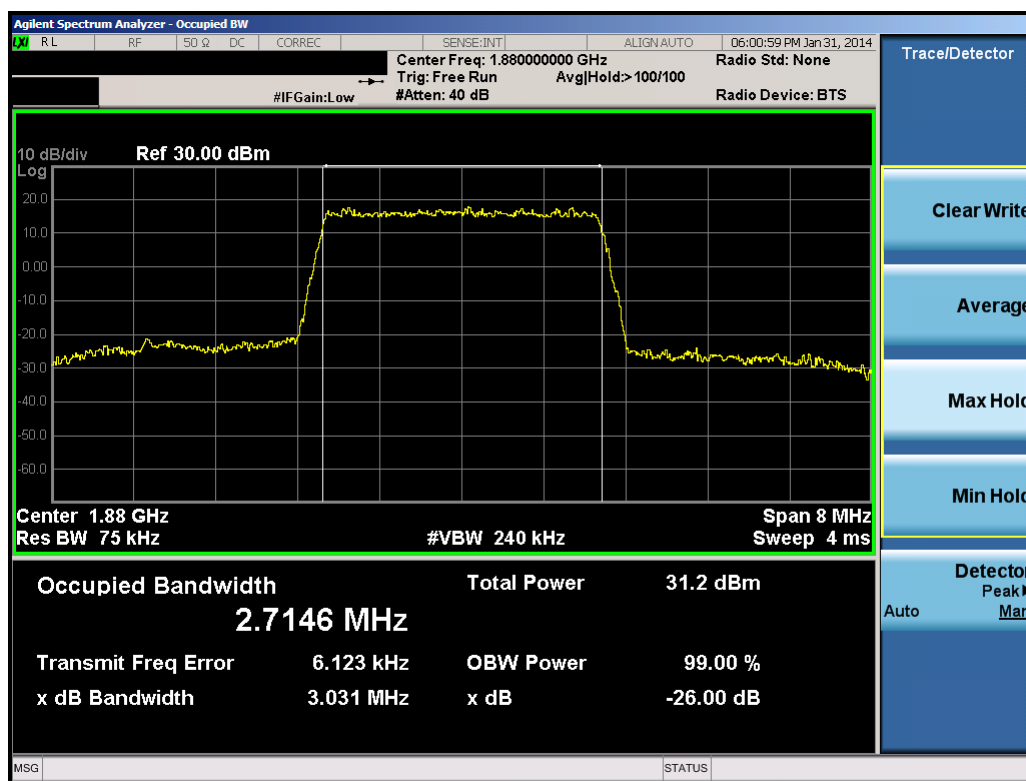
Plot 10-17. Occupied Bandwidth Plot (3.0MHz QPSK – RB Size 15)
