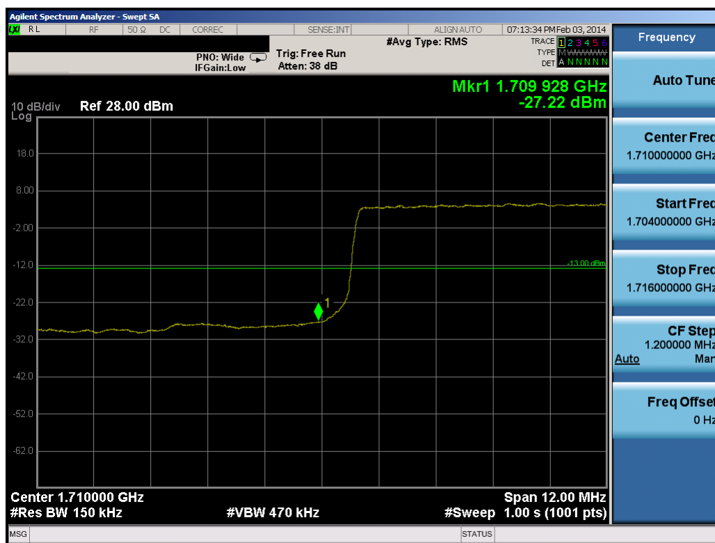
Plot 9-57. Lower Band Edge Plot (15.0MHz QPSK – RB Size 75)
