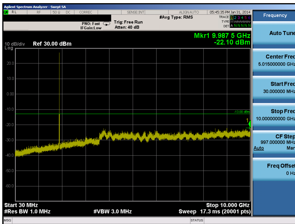
Plot 10-51. Conducted Spurious Plot (10.0MHz QPSK – RB Size 1, RB Offset 0 – High Channel)
