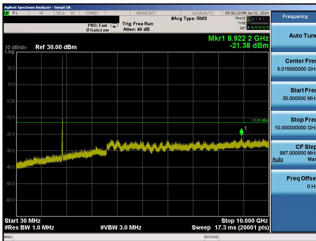
Plot 10-75. Conducted Spurious Plot (20.0MHz QPSK – RB Size 1, RB Offset 0– Low Channel)
