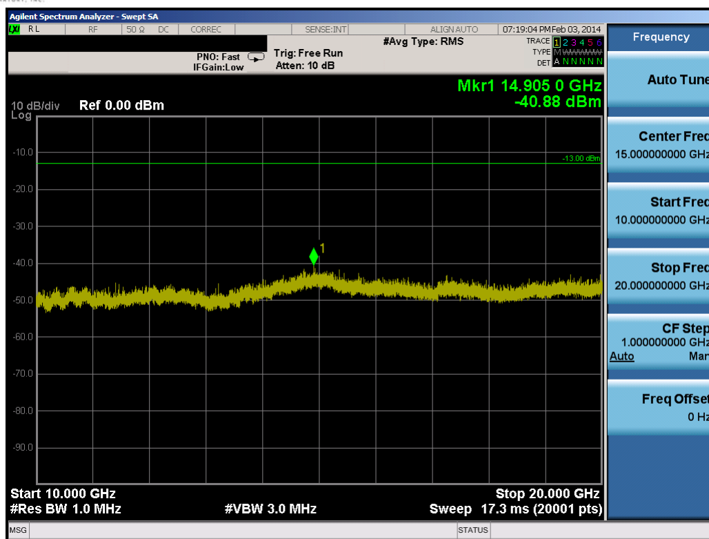
Plot 9-78. Conducted Spurious Plot (20.0MHz QPSK – RB Size 1, RB Offset 0 – Mid Channel)
