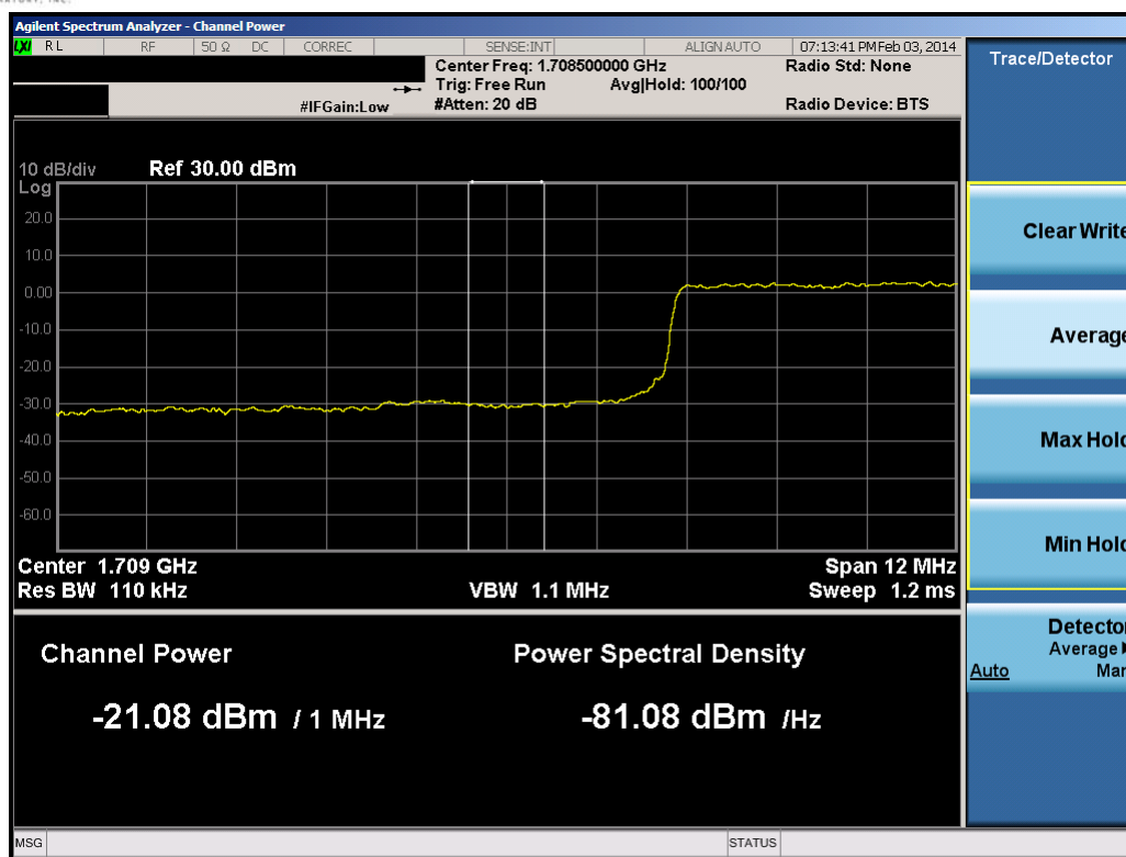
Plot 9-58. Lower Extended Band Edge Plot (15.0MHz QPSK – RB Size 75)
