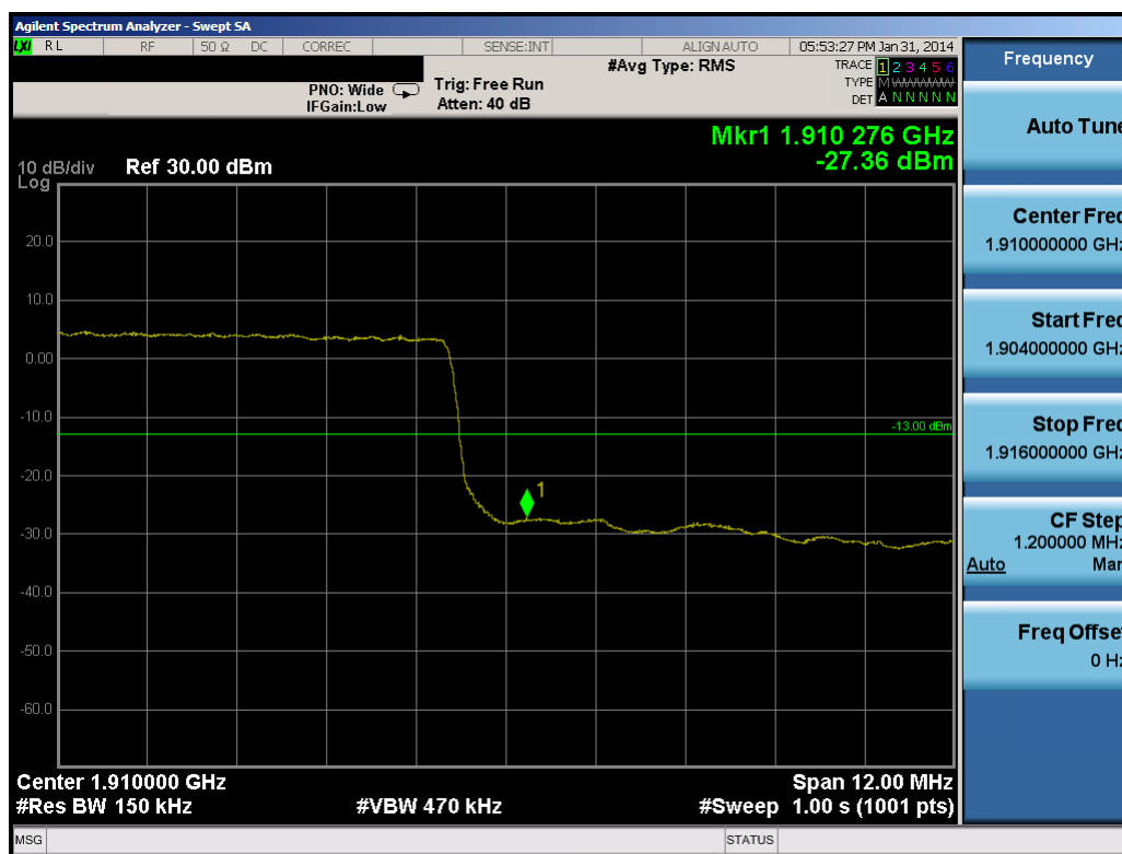
Plot 10-67. Upper Band Edge Plot (15.0MHz QPSK – RB Size 75)
