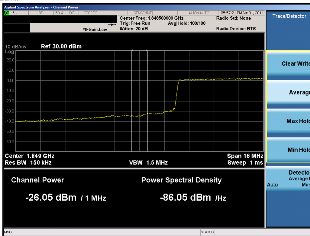
Plot 10-72. Lower Extended Band Edge Plot (20.0MHz QPSK – RB Size 100)
