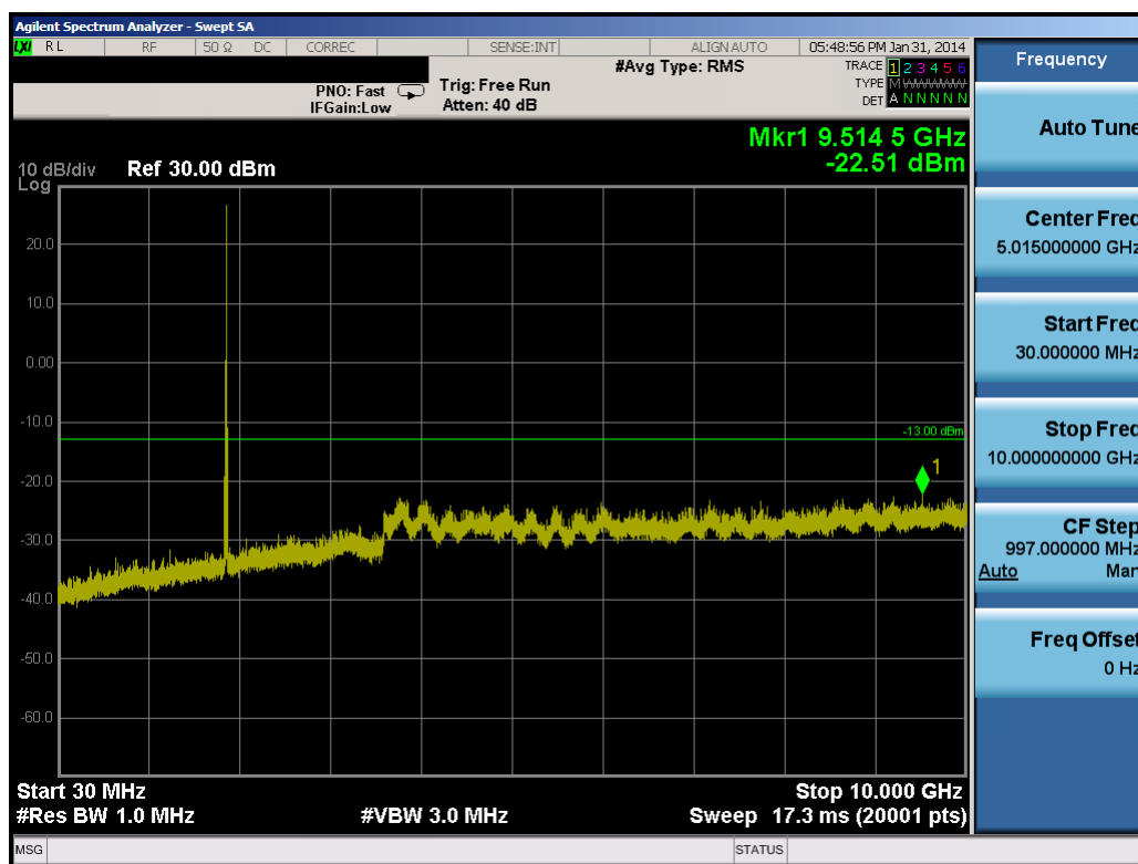
Plot 10-63. Conducted Spurious Plot (15.0MHz QPSK – RB Size 1, RB Offset 0 – Mid Channel)
