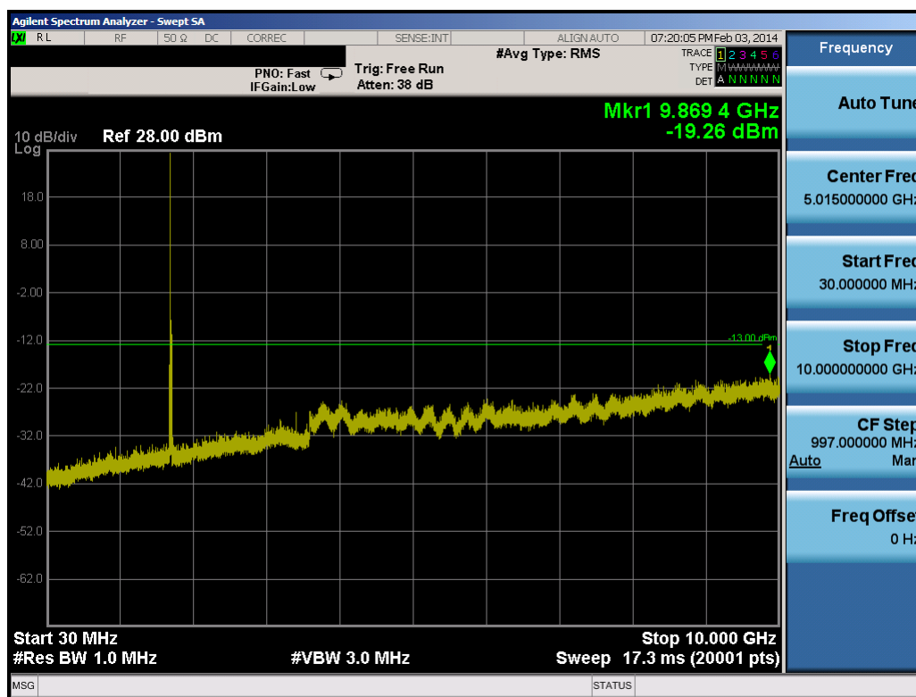
Plot 9-75. Conducted Spurious Plot (20.0MHz QPSK – RB Size 1, RB Offset 0– Low Channel)
