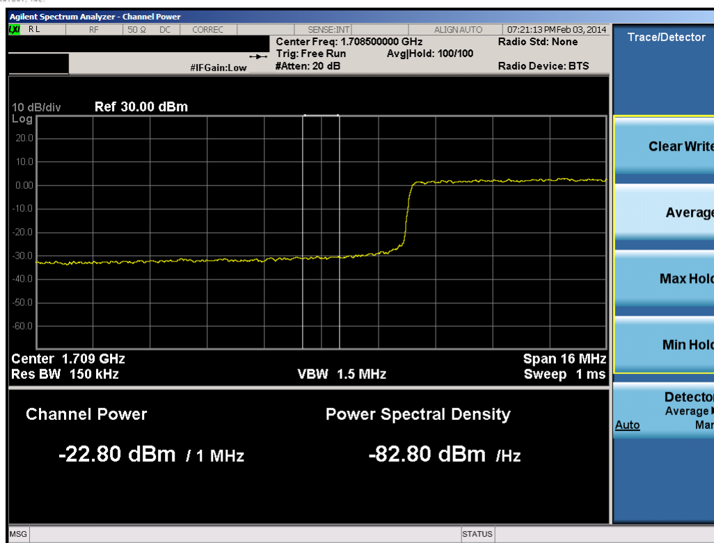
Plot 9-72. Lower Extended Band Edge Plot (20.0MHz QPSK – RB Size 100)
