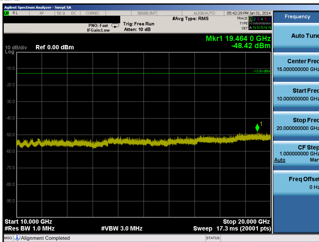
Plot 10-50. Conducted Spurious Plot (10.0MHz QPSK – RB Size 1, RB Offset 0 – Mid Channel)
