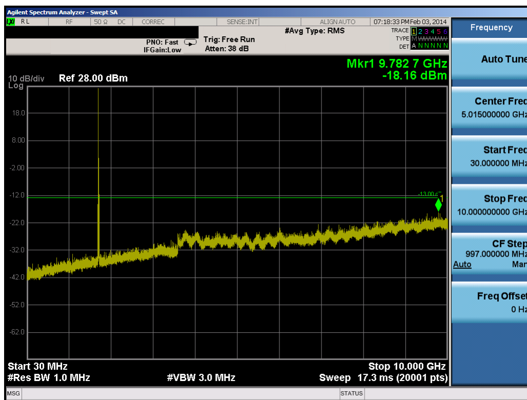
Plot 9-77. Conducted Spurious Plot (20.0MHz QPSK – RB Size 1, RB Offset 0 – Mid Channel)
