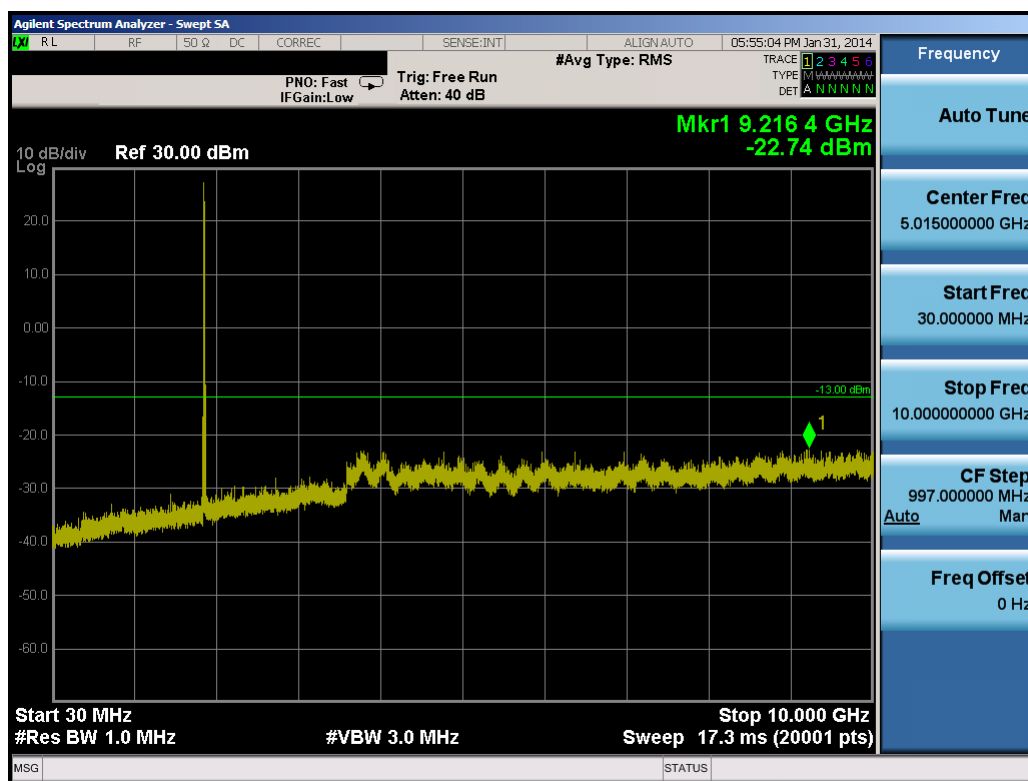
Plot 10-77. Conducted Spurious Plot (20.0MHz QPSK – RB Size 1, RB Offset 0 – Mid Channel)
