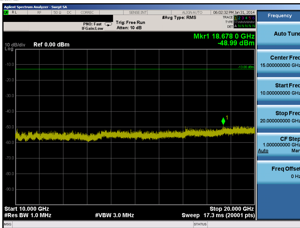
Plot 10-22. Conducted Spurious Plot (3.0MHz QPSK – RB Size 1, RB Offset 0 – Mid Channel)
