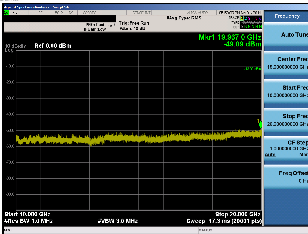
Plot 10-80. Conducted Spurious Plot (20.0MHz QPSK – RB Size 1, RB Offset 0 – High Channel)
