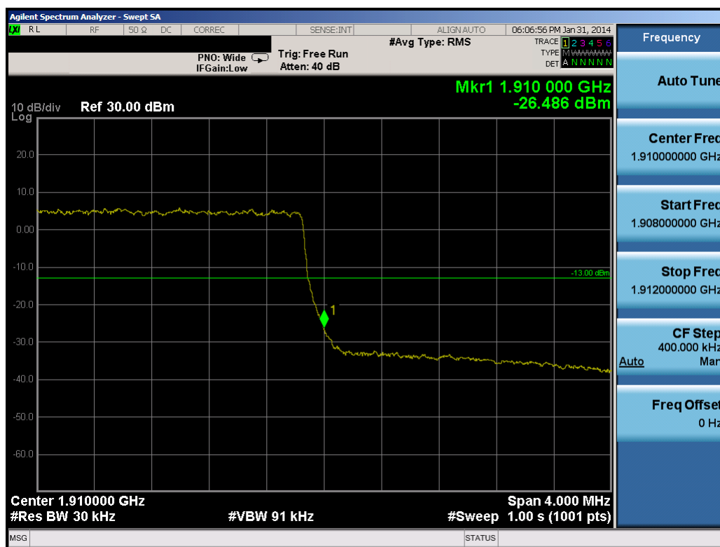
Plot 10-25. Upper Band Edge Plot (3.0MHz QPSK – RB Size 15)
