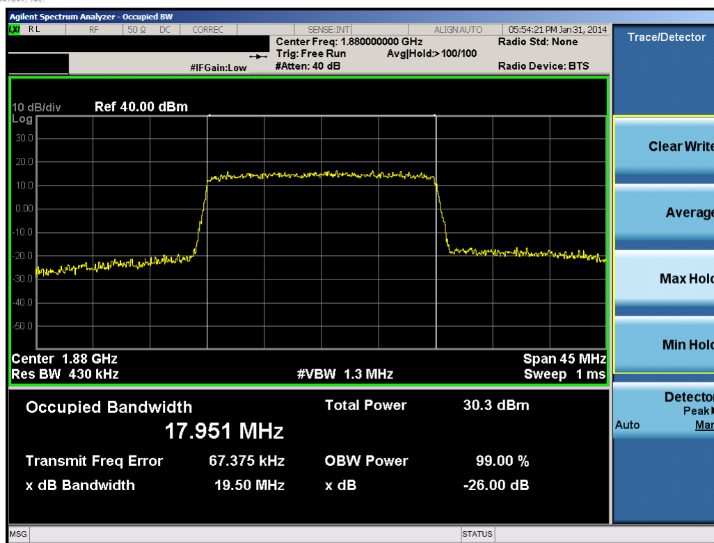
Plot 10-74. Occupied Bandwidth Plot (20.0MHz 16-QAM – RB Size 100)
