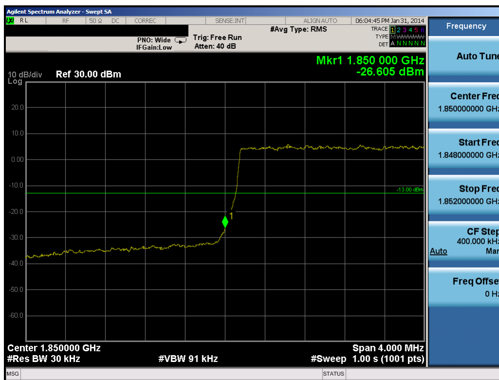
Plot 10-15. Lower Band Edge Plot (3.0MHz QPSK - RB Size 15)
