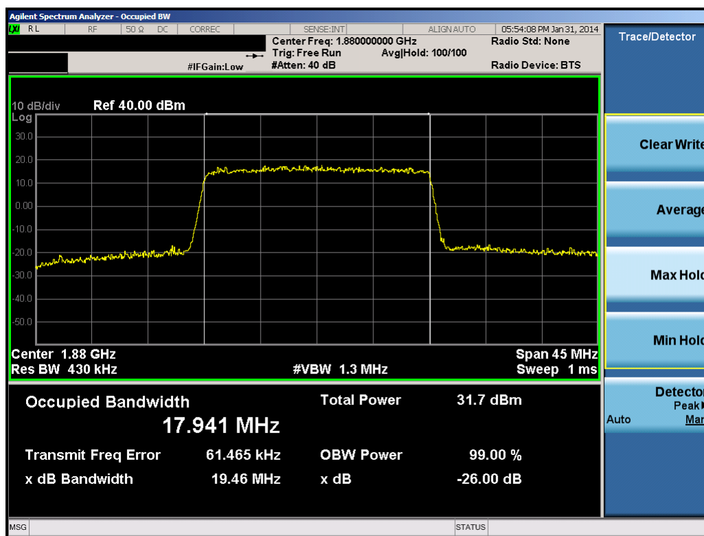
Plot 10-73. Occupied Bandwidth Plot (20.0MHz QPSK – RB Size 100)
