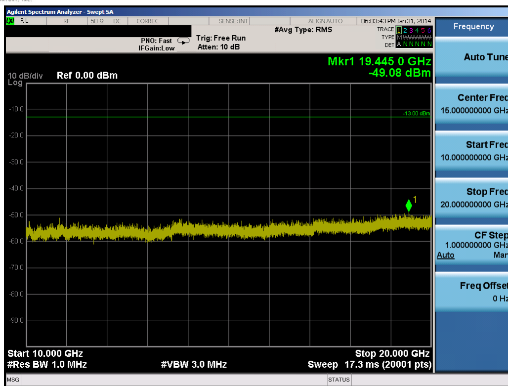
Plot 10-20. Conducted Spurious Plot (3.0MHz QPSK – RB Size 1, RB Offset 0 – Low Channel)
