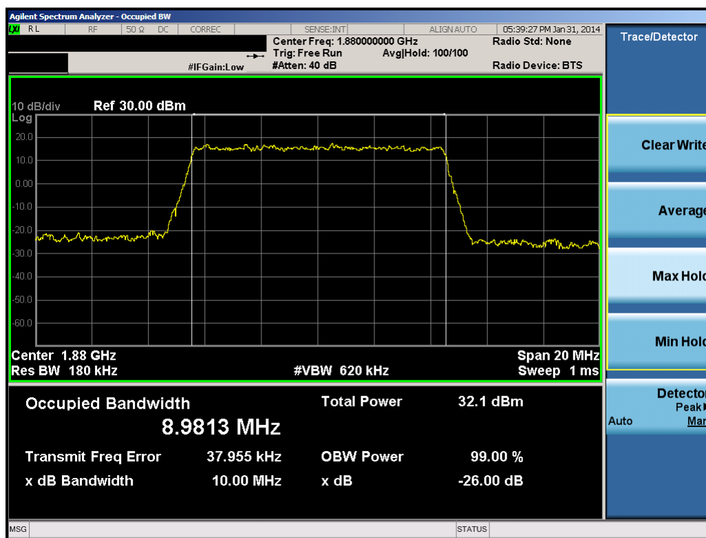
Plot 10-45. Occupied Bandwidth Plot (10.0MHz QPSK – RB Size 50)
