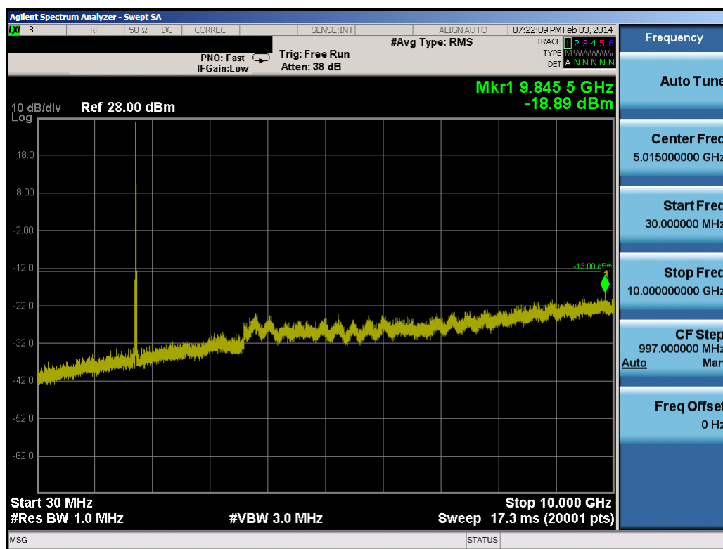
Plot 9-79. Conducted Spurious Plot (20.0MHz QPSK – RB Size 1, RB Offset 0 – High Channel)
