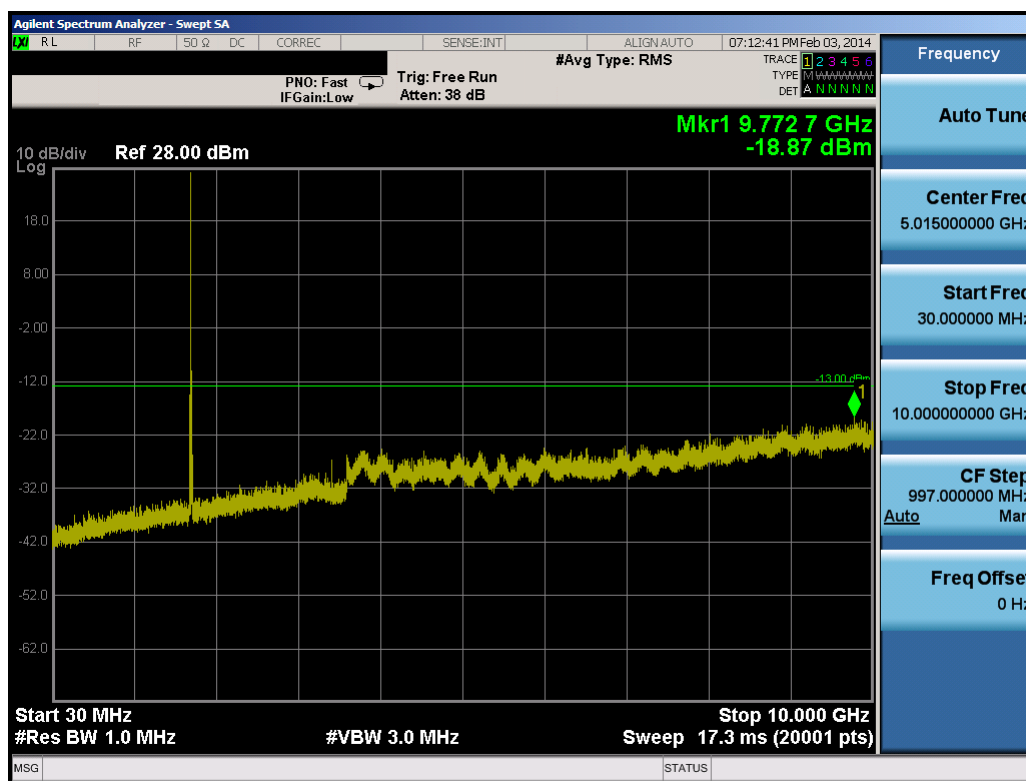
Plot 9-61. Conducted Spurious Plot (15.0MHz QPSK – RB Size 1, RB Offset 0 – Low Channel)
