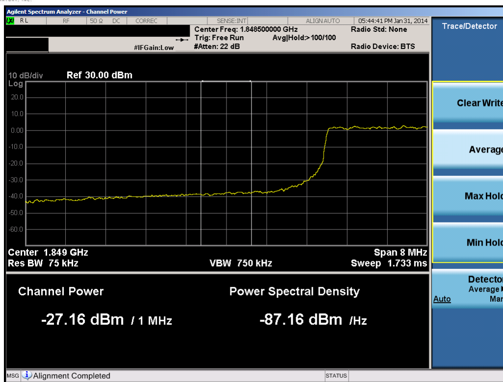
Plot 10-44. Lower Extended Band Edge Plot (10.0MHz QPSK – RB Size 50)
