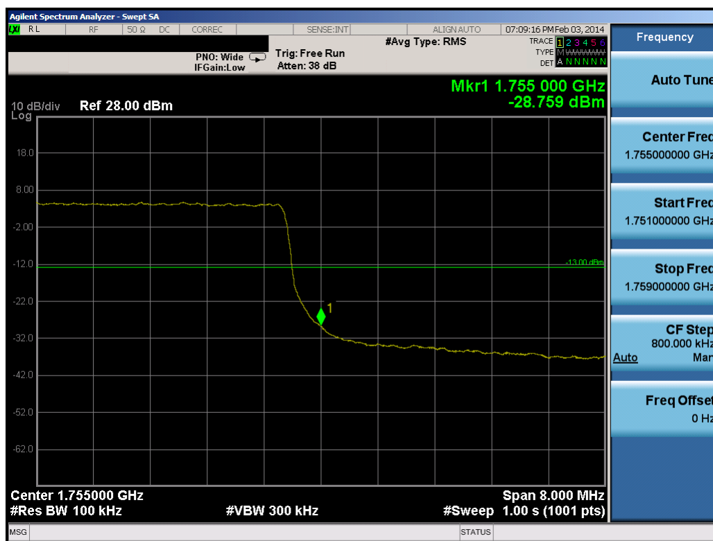
Plot 9-53. Upper Band Edge Plot (10.0MHz QPSK – RB Size 50)
