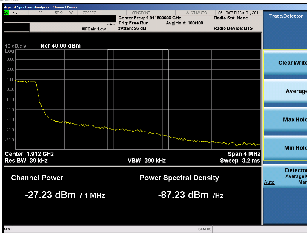
Plot 10-12. Upper Extended Band Edge Plot (1.4MHz QPSK – RB Size 6)
