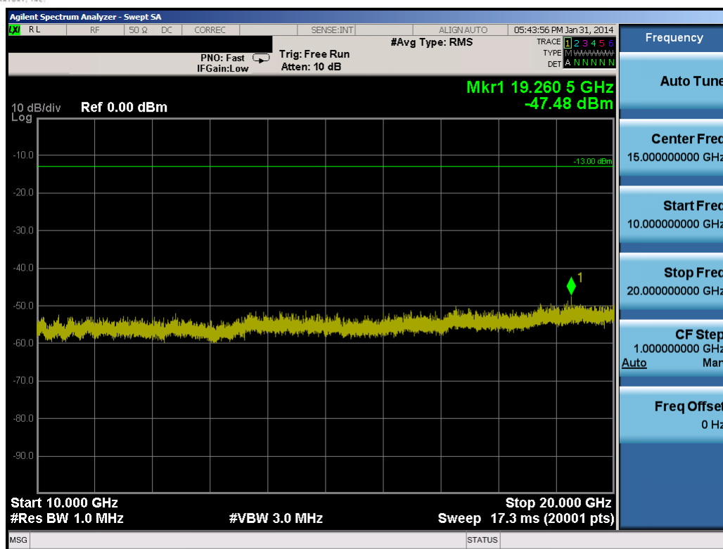
Plot 10-48. Conducted Spurious Plot (10.0MHz QPSK – RB Size 1, RB Offset 0 – Low Channel)
