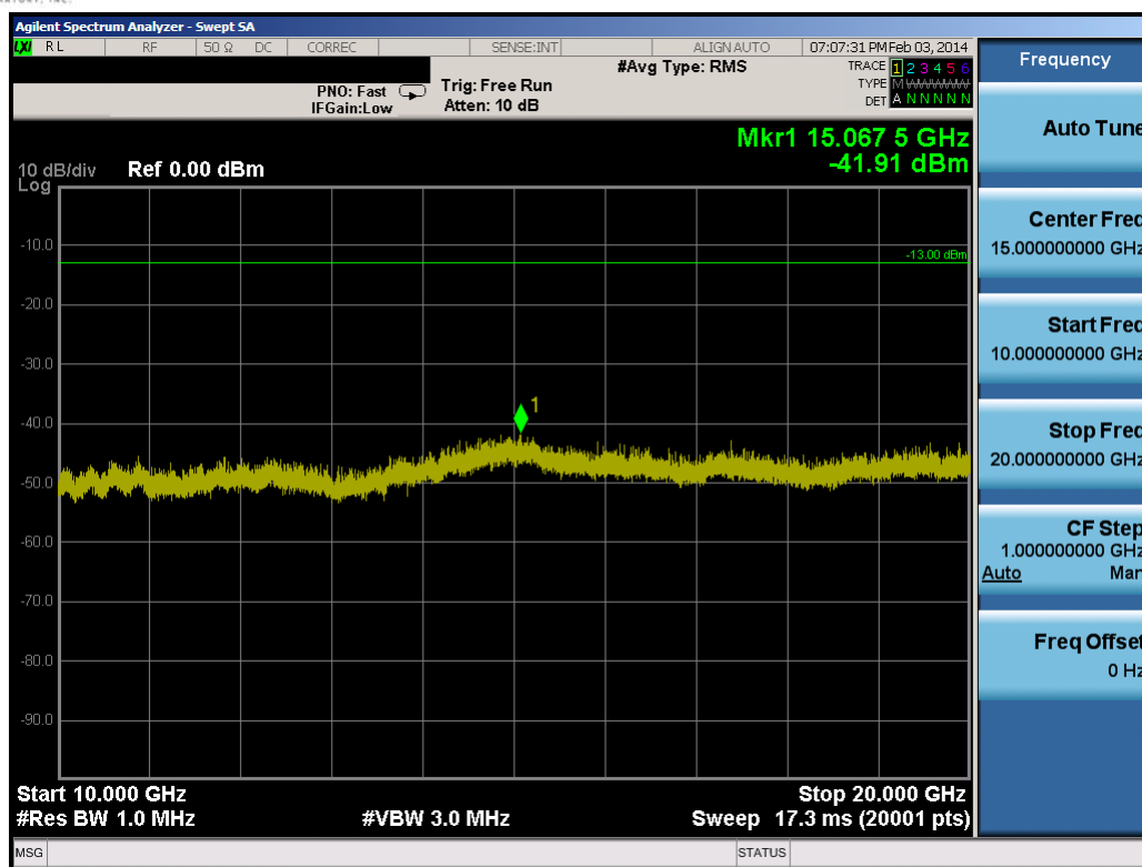
Plot 9-52. Conducted Spurious Plot (10.0MHz QPSK – RB Size 1, RB Offset 0 – High Channel)
