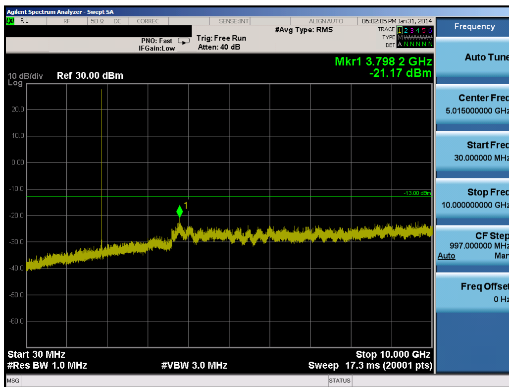
Plot 10-21. Conducted Spurious Plot (3.0MHz QPSK – RB Size 1, RB Offset 0 – Mid Channel)
