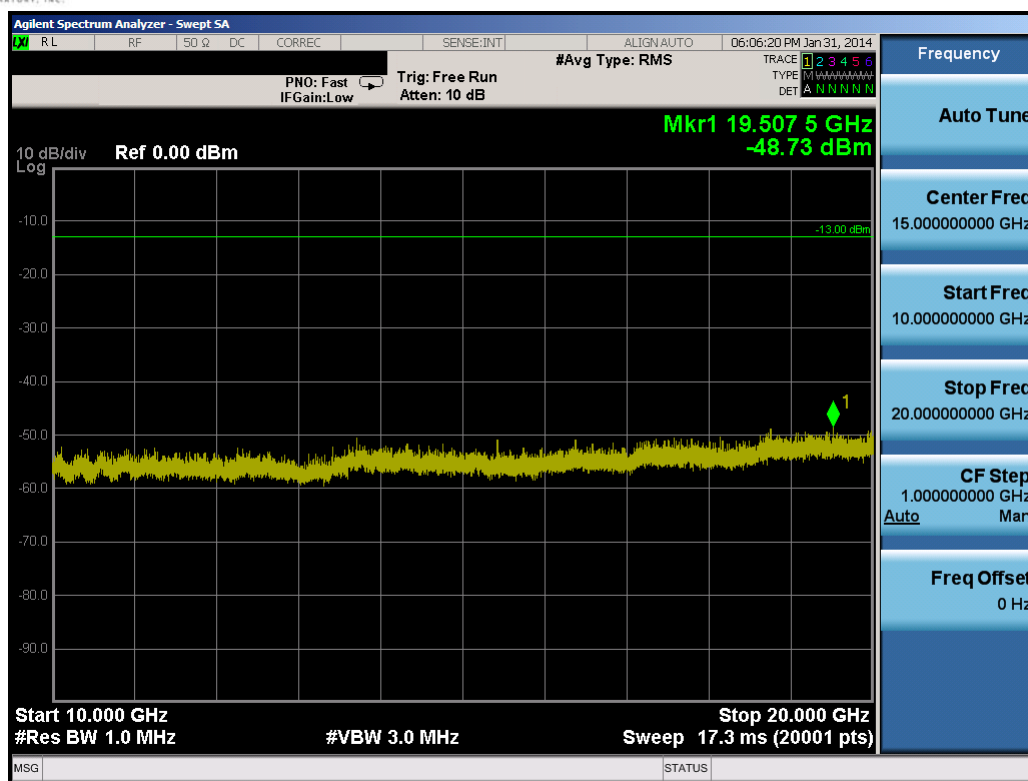
Plot 10-24. Conducted Spurious Plot (3.0MHz QPSK – RB Size 1, RB Offset 0 – High Channel)
