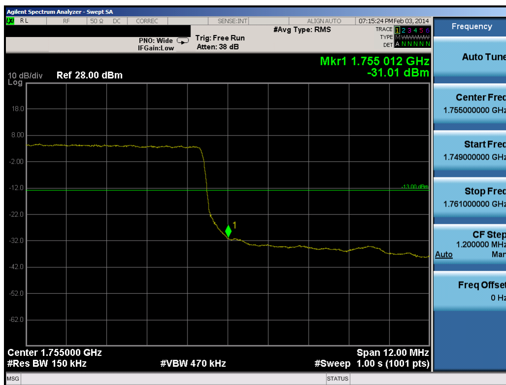
Plot 9-67. Upper Band Edge Plot (15.0MHz QPSK – RB Size 75)
