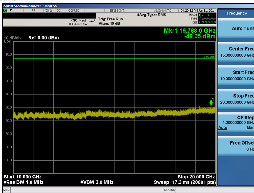
Plot 10-36. Conducted Spurious Plot (5.0MHz QPSK – RB Size 1, RB Offset 0 – Mid Channel)
