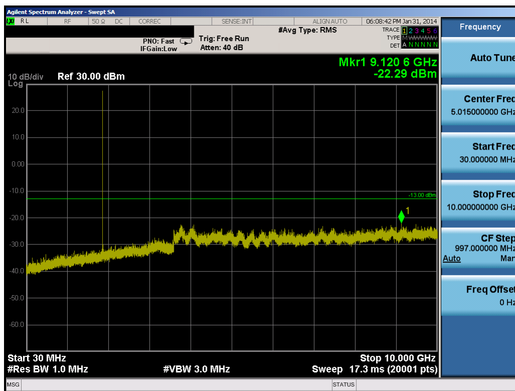
Plot 10-7. Conducted Spurious Plot (1.4MHz QPSK – RB Size 1, RB Offset 0 – Mid Channel)
