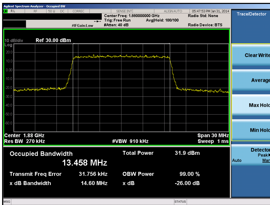
Plot 10-59. Occupied Bandwidth Plot (15.0MHz QPSK – RB Size 75)
