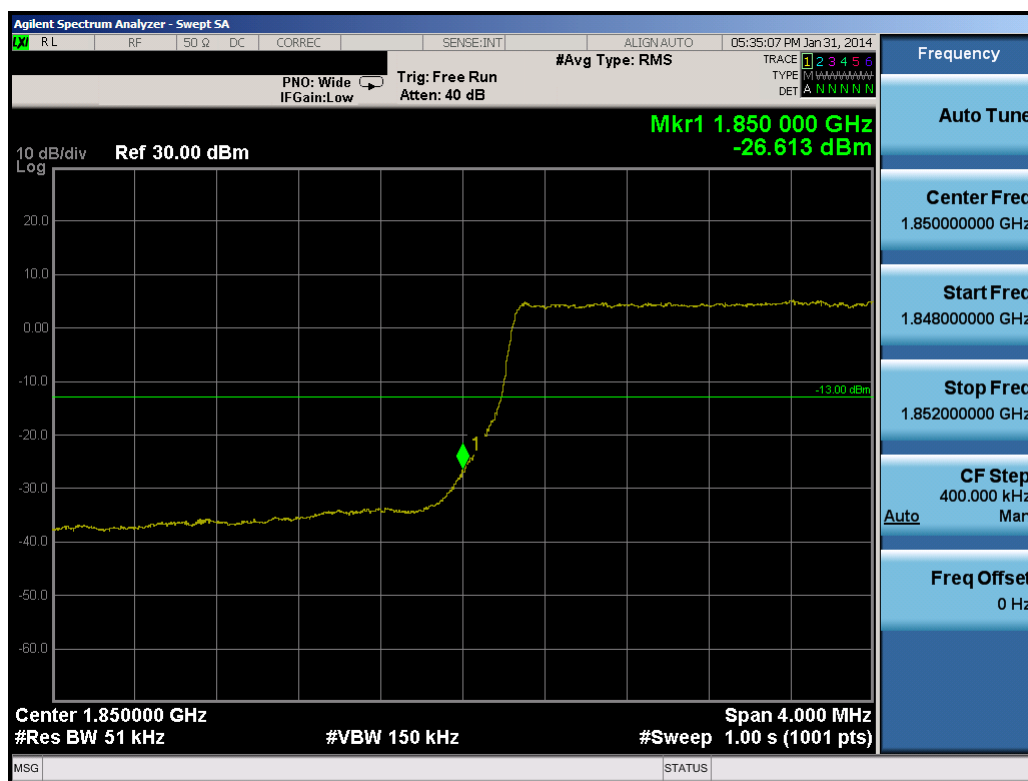
Plot 10-29. Lower Band Edge Plot (5.0MHz QPSK – RB Size 25)
