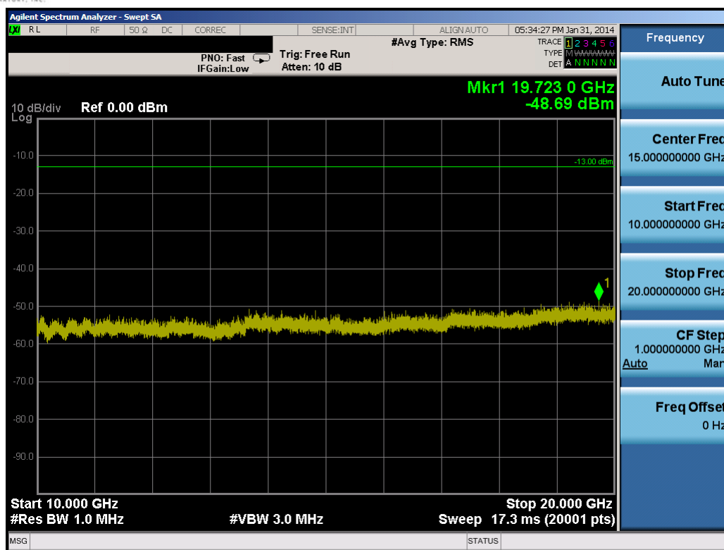
Plot 10-34. Conducted Spurious Plot (5.0MHz QPSK – RB Size 1, RB Offset 0 – Low Channel)
