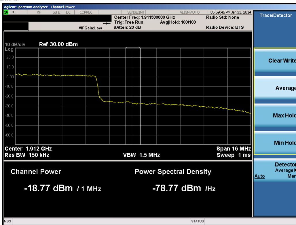
Plot 10-82. Upper Extended Band Edge Plot (20.0MHz QPSK – RB Size 100)
