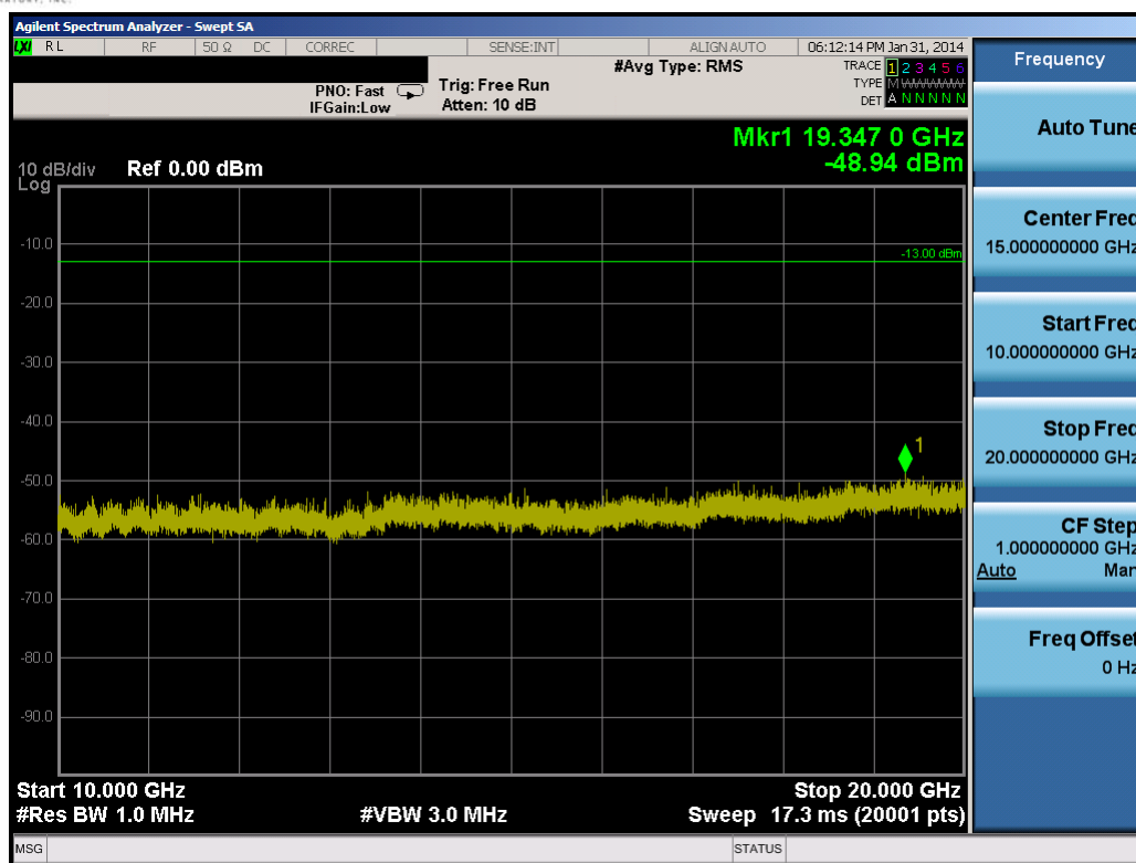
Plot 10-10. Conducted Spurious Plot (1.4MHz QPSK – RB Size 1, RB Offset 0 – High Channel)
