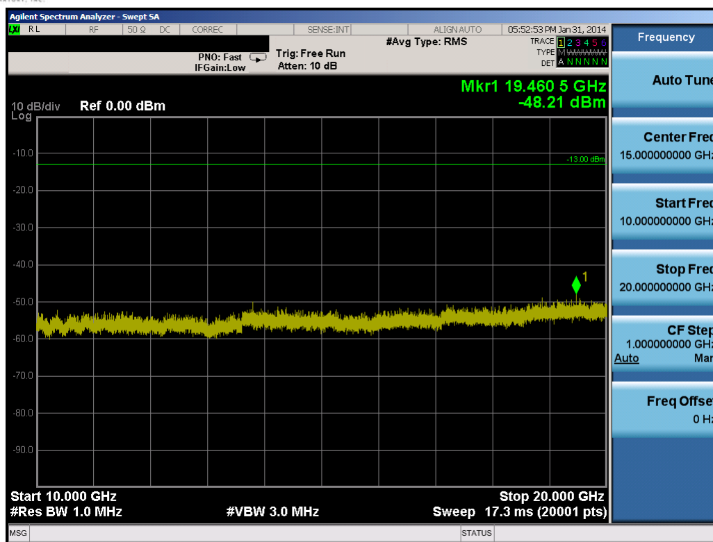
Plot 10-66. Conducted Spurious Plot (15.0MHz QPSK – RB Size 1, RB Offset 0 – High Channel)
