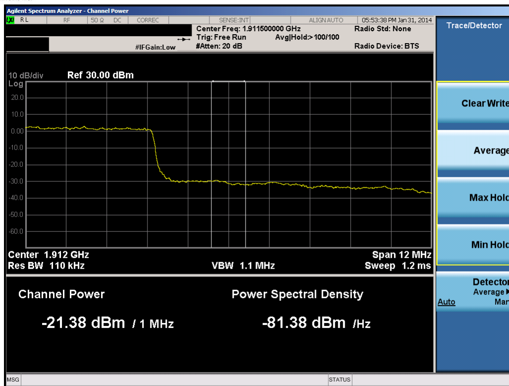
Plot 10-68. Upper Extended Band Edge Plot (15.0MHz QPSK – RB Size 75)
