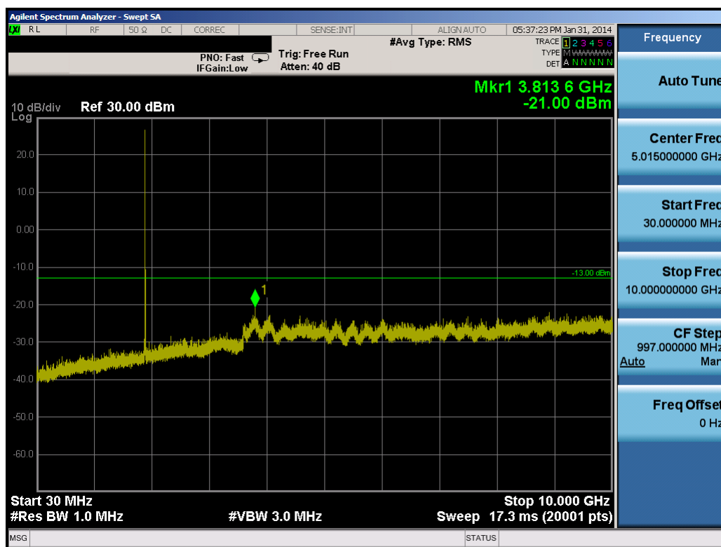
Plot 10-37. Conducted Spurious Plot (5.0MHz QPSK – RB Size 1, RB Offset 0 – High Channel)
