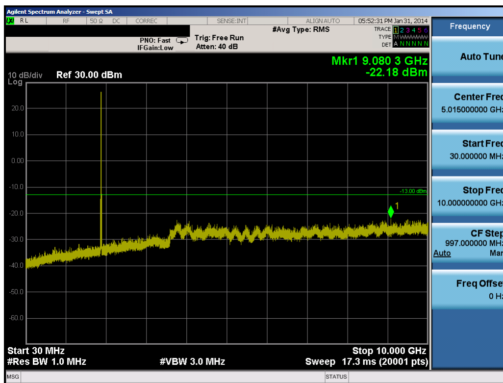
Plot 10-65. Conducted Spurious Plot (15.0MHz QPSK – RB Size 1, RB Offset 0 – High Channel)
