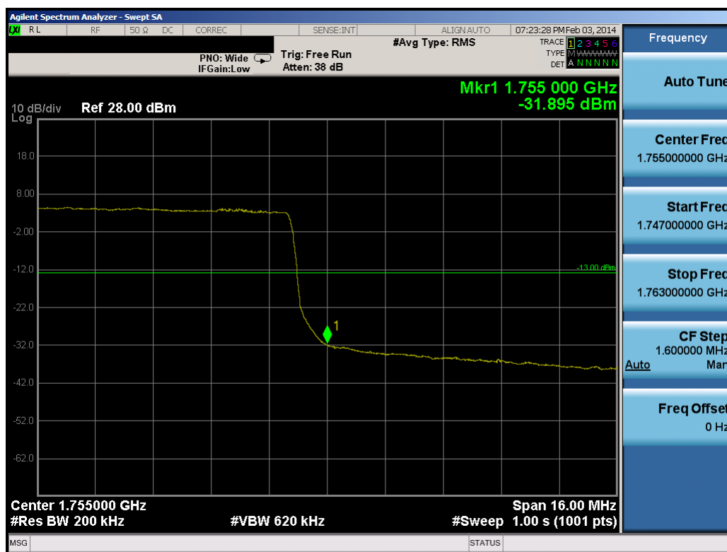
Plot 9-81. Upper Band Edge Plot (20.0MHz QPSK – RB Size 100)
