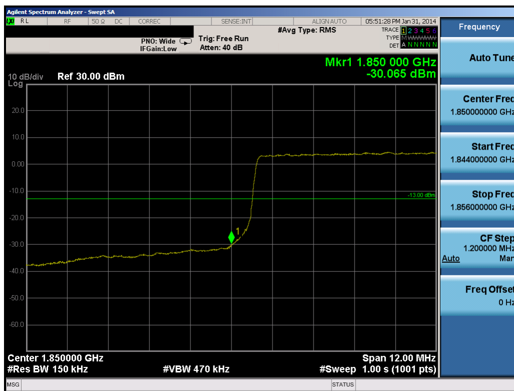
Plot 10-57. Lower Band Edge Plot (15.0MHz QPSK – RB Size 75)
