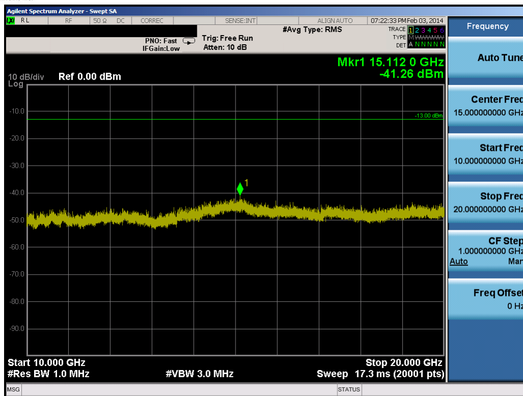
Plot 9-80. Conducted Spurious Plot (20.0MHz QPSK – RB Size 1, RB Offset 0 – High Channel)
