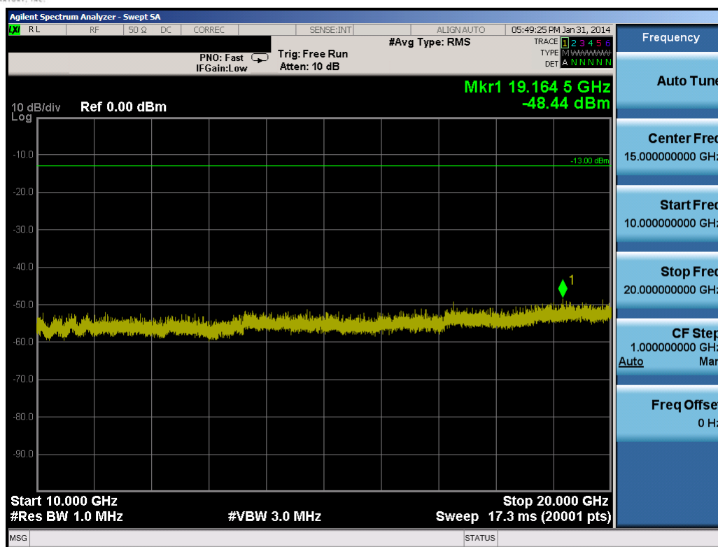
Plot 10-64. Conducted Spurious Plot (15.0MHz QPSK – RB Size 1, RB Offset 0 – Mid Channel)
