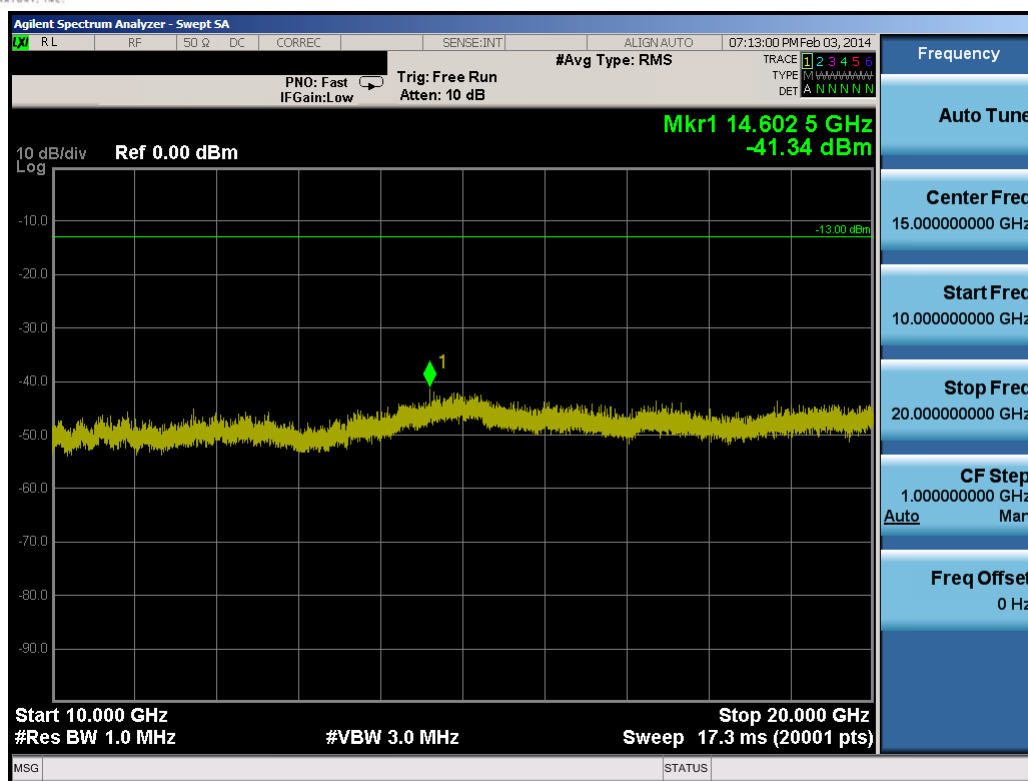
Plot 9-62. Conducted Spurious Plot (15.0MHz QPSK – RB Size 1, RB Offset 0 – Low Channel)
