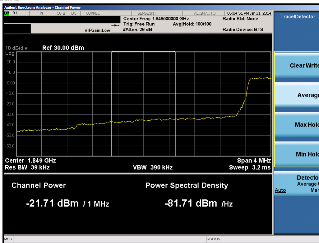
Plot 10-16. Lower Extended Band Edge Plot (3.0MHz QPSK – RB Size 15)
