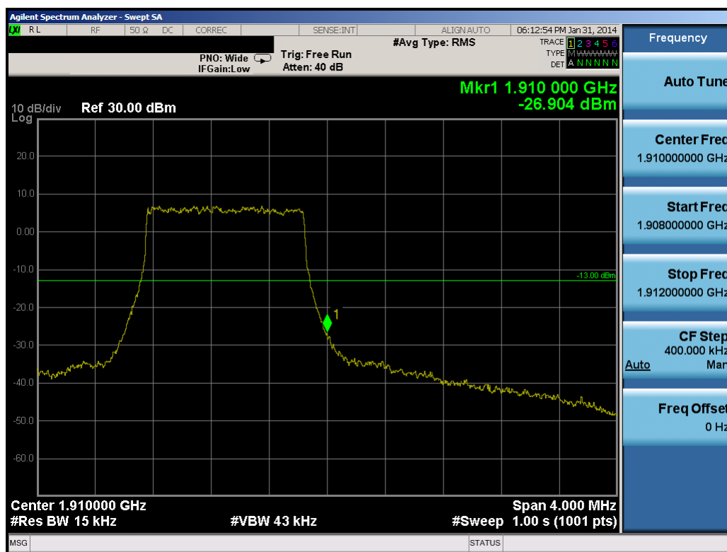
Plot 10-11. Upper Band Edge Plot (1.4MHz QPSK – RB Size 6)
