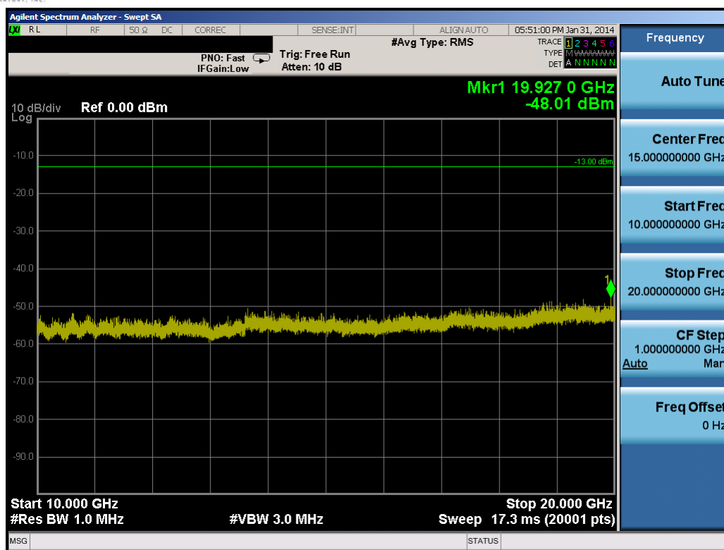
Plot 10-62. Conducted Spurious Plot (15.0MHz QPSK – RB Size 1, RB Offset 0 – Low Channel)
