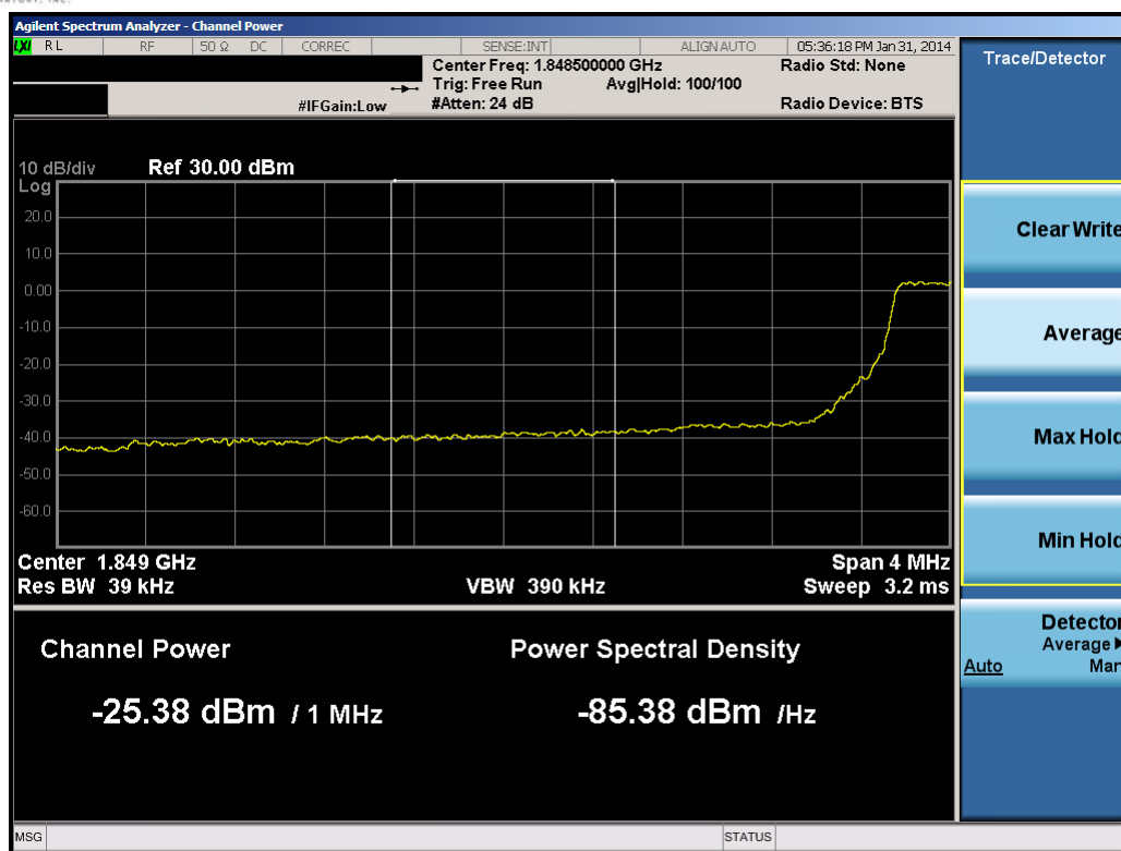
Plot 10-30. Lower Extended Band Edge Plot (5.0MHz QPSK – RB Size 25)
