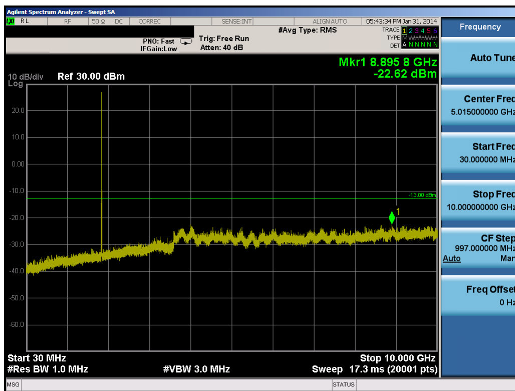
Plot 10-47. Conducted Spurious Plot (10.0MHz QPSK – RB Size 1, RB Offset 0– Low Channel)
