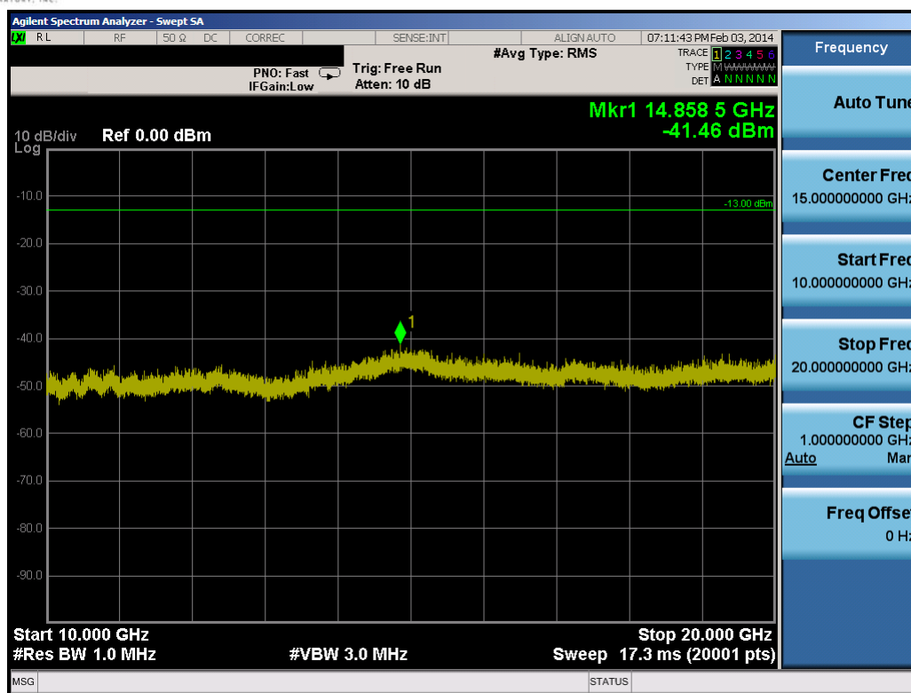
Plot 9-64. Conducted Spurious Plot (15.0MHz QPSK – RB Size 1, RB Offset 0 – Mid Channel)
