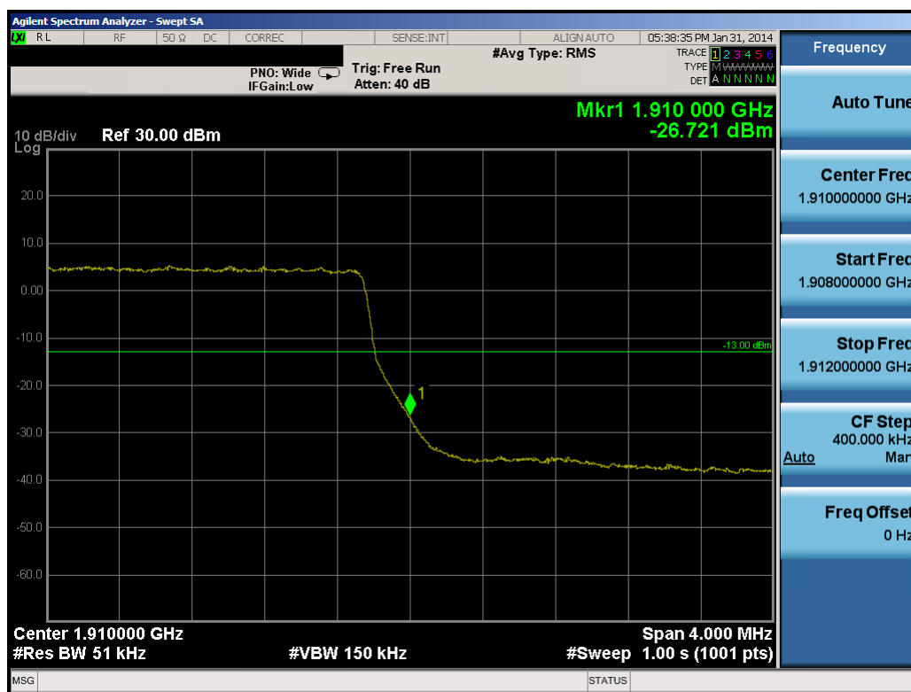
Plot 10-39. Upper Band Edge Plot (5.0MHz QPSK – RB Size 25)
