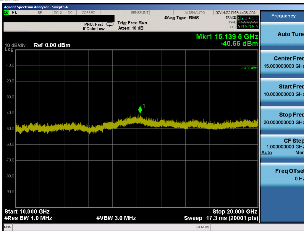
Plot 9-66. Conducted Spurious Plot (15.0MHz QPSK – RB Size 1, RB Offset 0 – High Channel)
