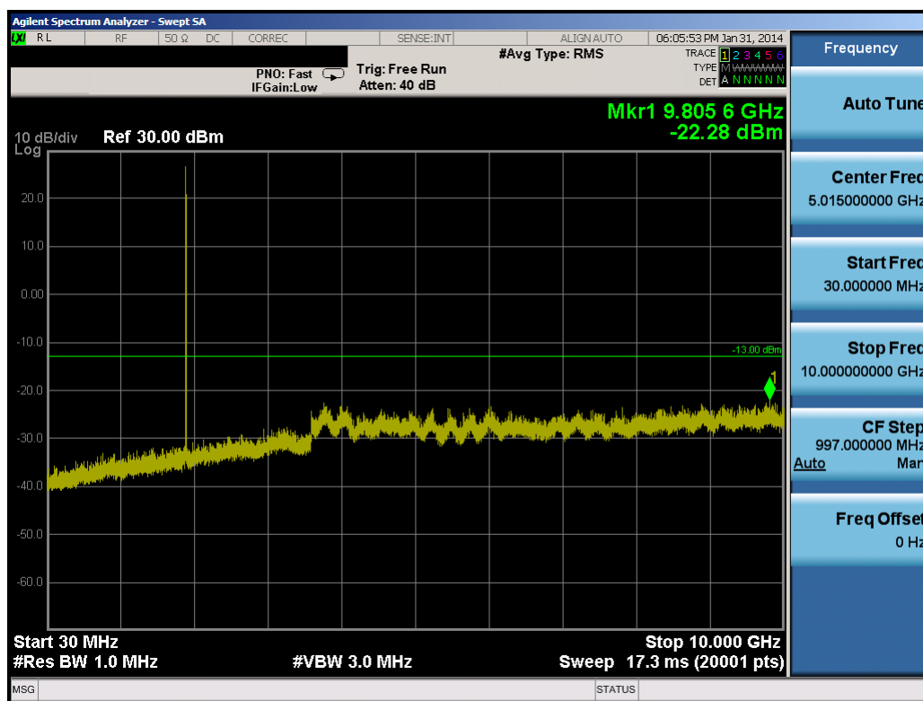
Plot 10-23. Conducted Spurious Plot (3.0MHz QPSK – RB Size 1, RB Offset 0 – High Channel)
