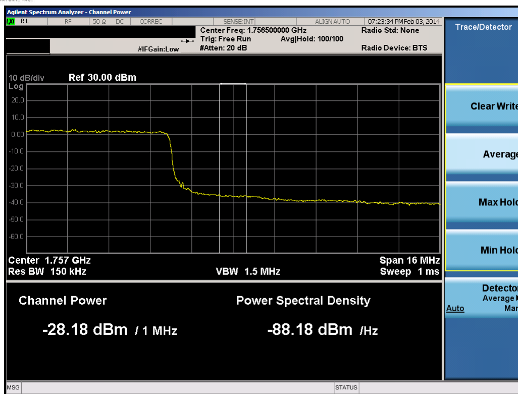
Plot 9-82. Upper Extended Band Edge Plot (20.0MHz QPSK – RB Size 100)
