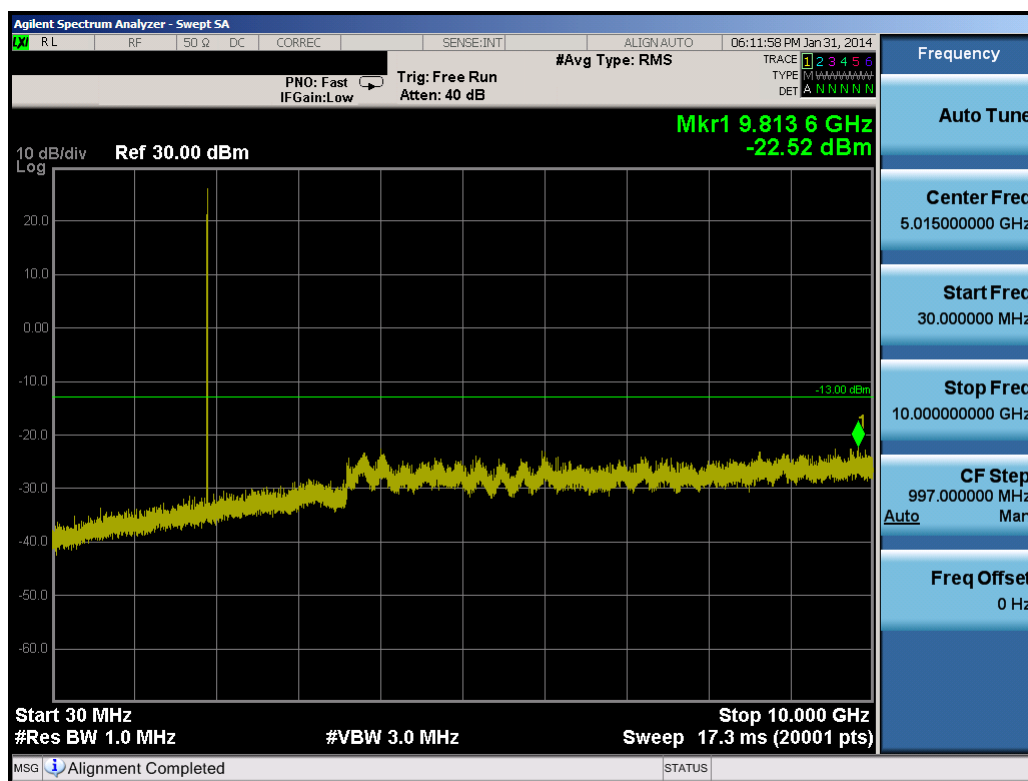
Plot 10-9. Conducted Spurious Plot (1.4MHz QPSK – RB Size 1, RB Offset 0 – High Channel)
