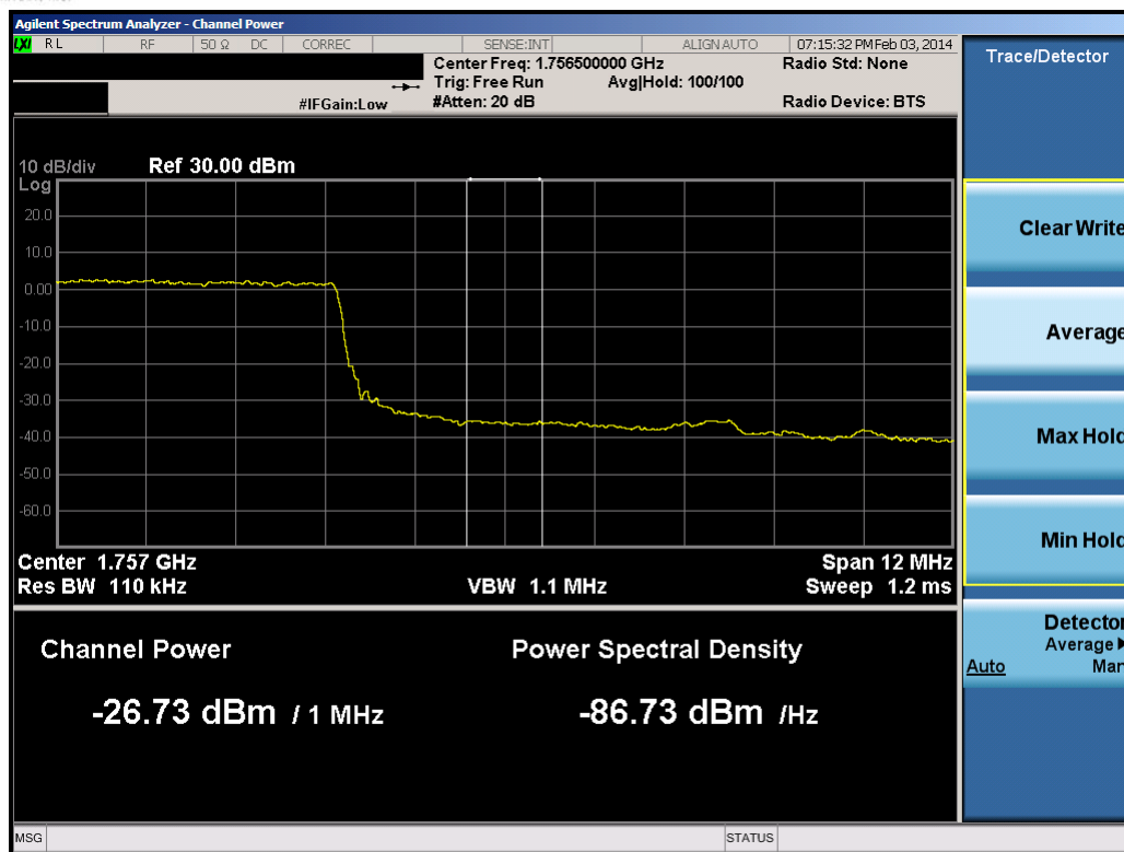
Plot 9-68. Upper Extended Band Edge Plot (15.0MHz QPSK – RB Size 75)
