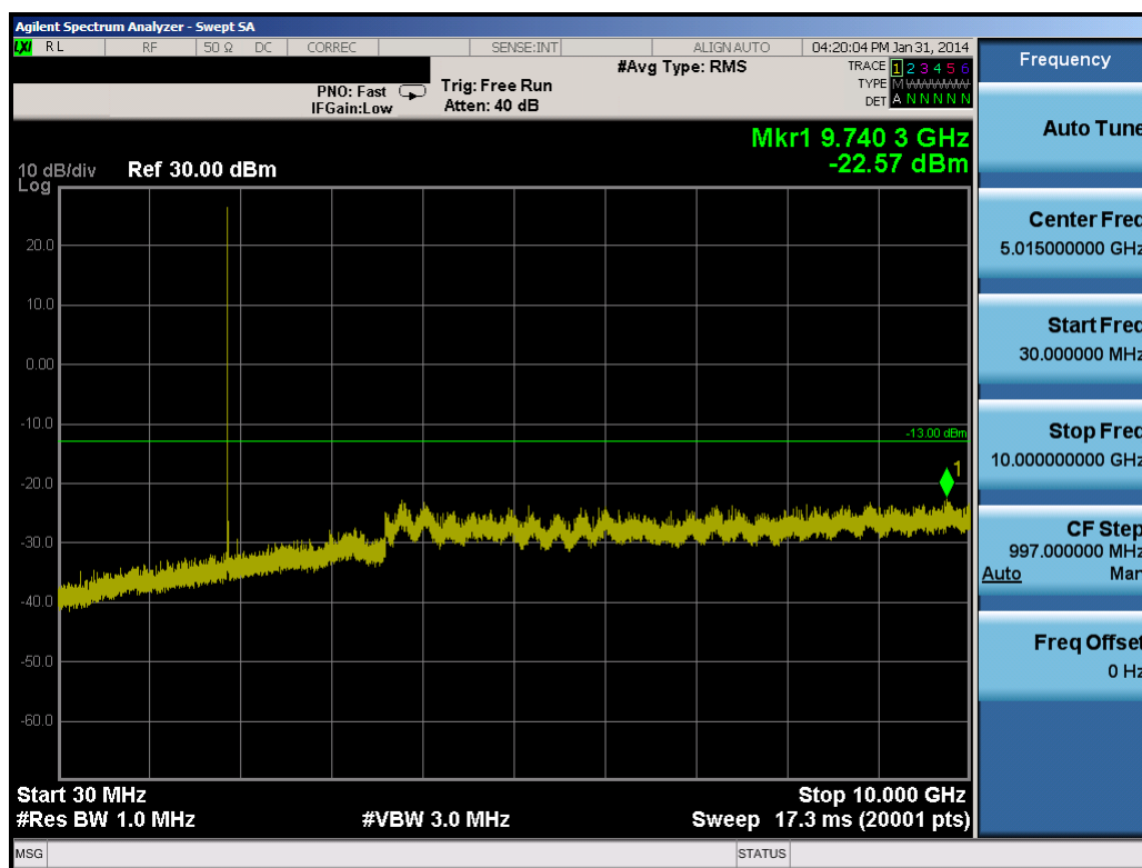
Plot 10-35. Conducted Spurious Plot (5.0MHz QPSK – RB Size 1, RB Offset 0 – Mid Channel)
