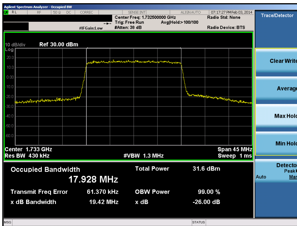
Plot 9-73. Occupied Bandwidth Plot (20.0MHz QPSK – RB Size 100)
