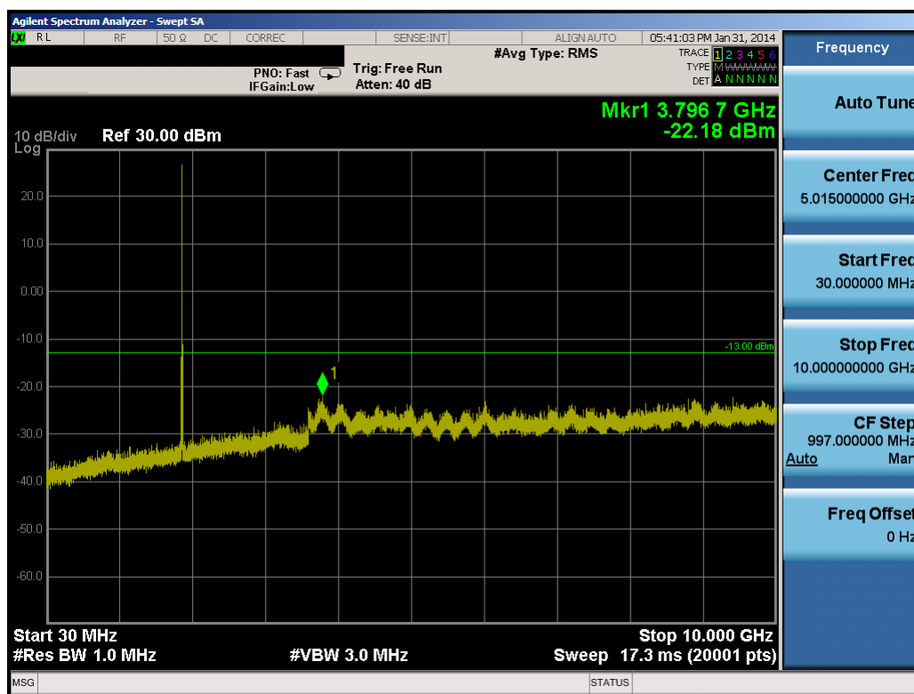
Plot 10-49. Conducted Spurious Plot (10.0MHz QPSK – RB Size 1, RB Offset 0 – Mid Channel)
