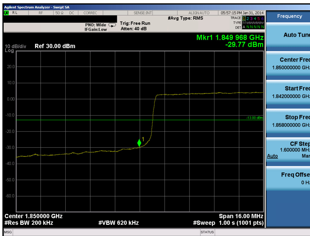
Plot 10-71. Lower Band Edge Plot (20.0MHz QPSK – RB Size 100)
