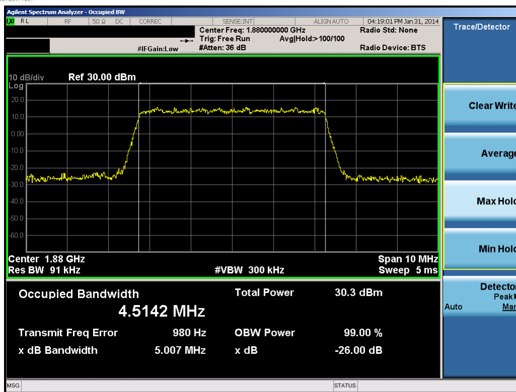
Plot 10-32. Occupied Bandwidth Plot (5.0MHz 16-QAM – RB Size 25)
