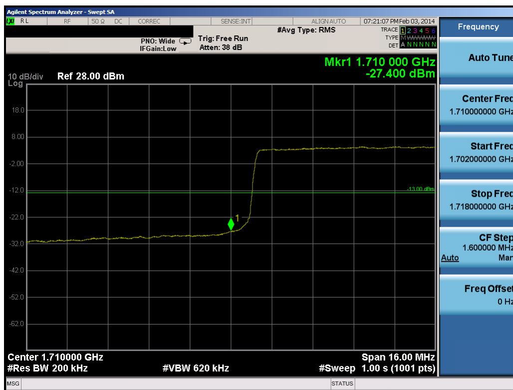
Plot 9-71. Lower Band Edge Plot (20.0MHz QPSK – RB Size 100)
