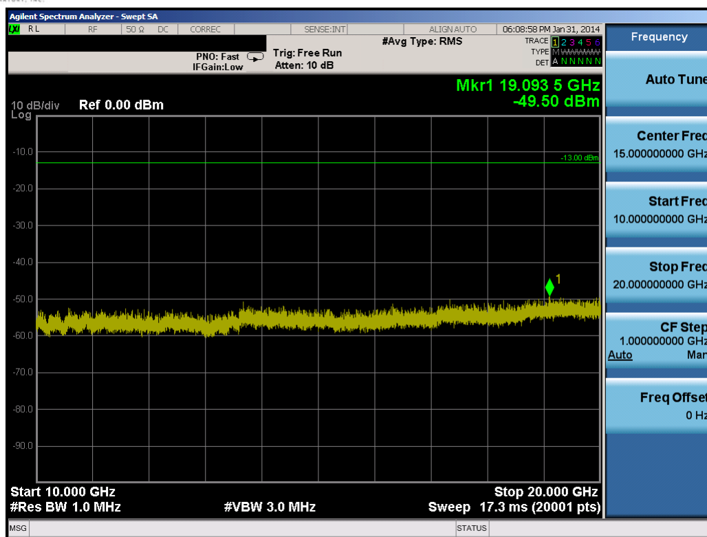
Plot 10-8. Conducted Spurious Plot (1.4MHz QPSK – RB Size 1, RB Offset 0 – Mid Channel)
