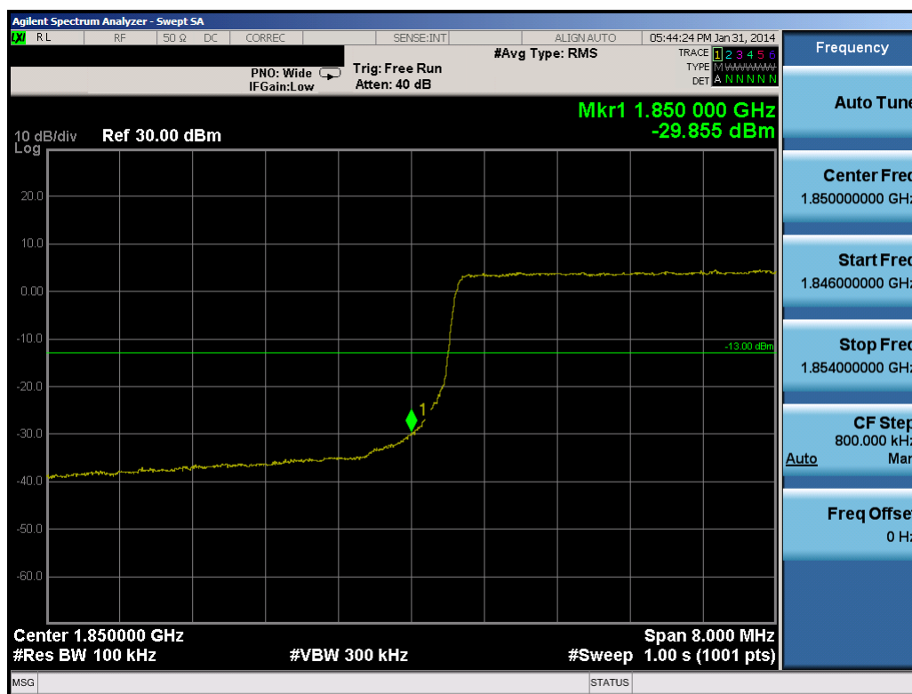
Plot 10-43. Lower Band Edge Plot (10.0MHz QPSK – RB Size 50)
