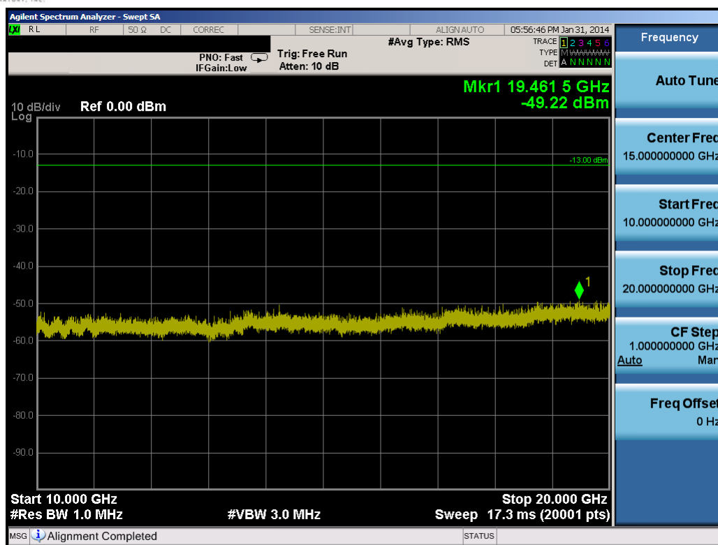
Plot 10-76. Conducted Spurious Plot (20.0MHz QPSK – RB Size 1, RB Offset 0 – Low Channel)
