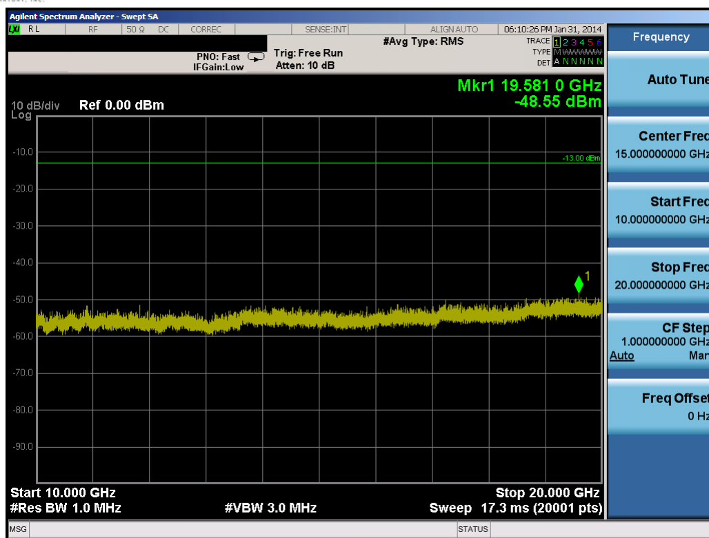
Plot 10-6. Conducted Spurious Plot (1.4MHz QPSK – RB Size 1, RB Offset 0 – Low Channel)
