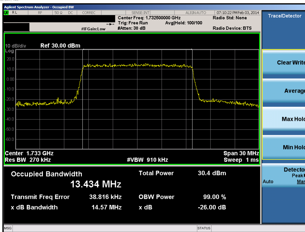
Plot 9-60. Occupied Bandwidth Plot (15.0MHz 16-QAM – RB Size 75)
