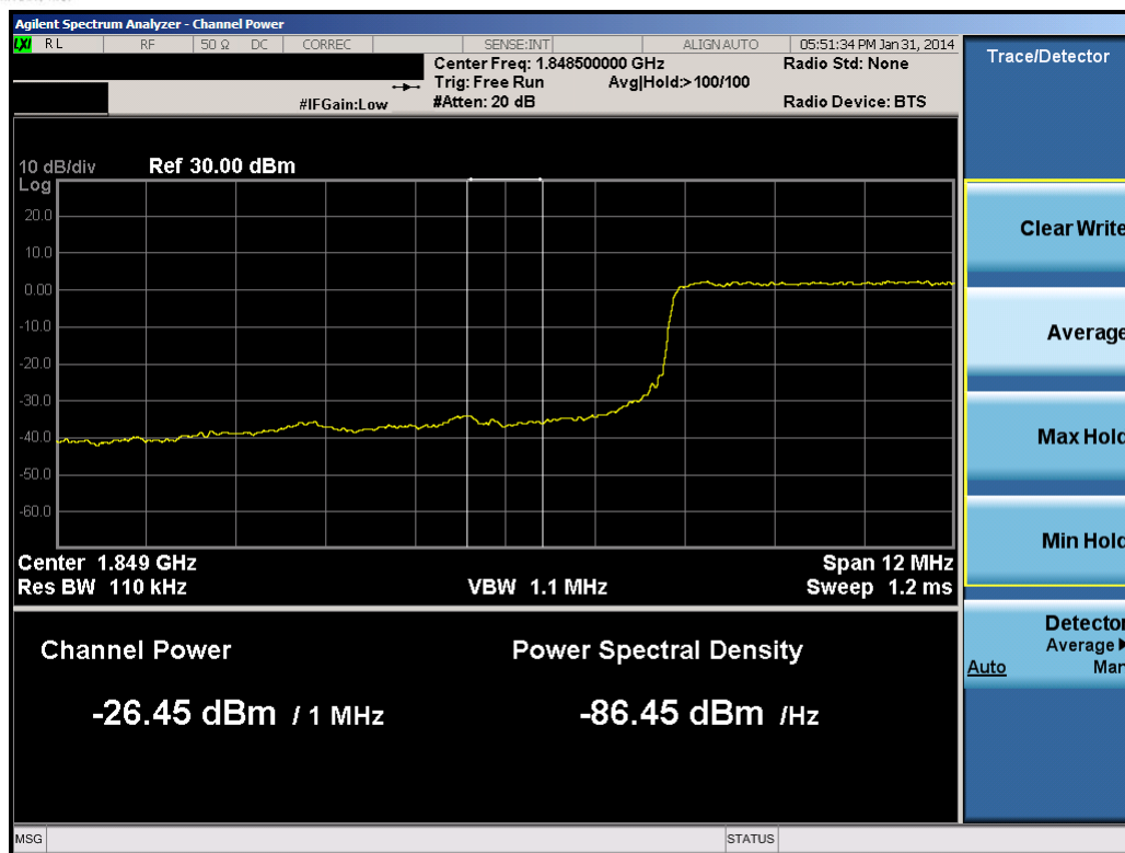
Plot 10-58. Lower Extended Band Edge Plot (15.0MHz QPSK – RB Size 75)
