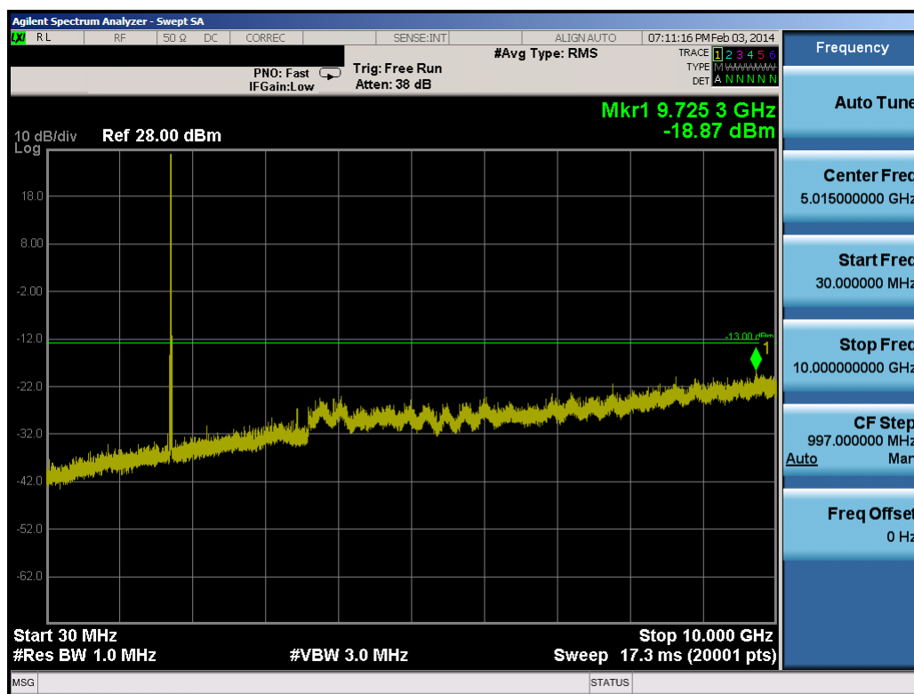
Plot 9-63. Conducted Spurious Plot (15.0MHz QPSK – RB Size 1, RB Offset 0 – Mid Channel)
