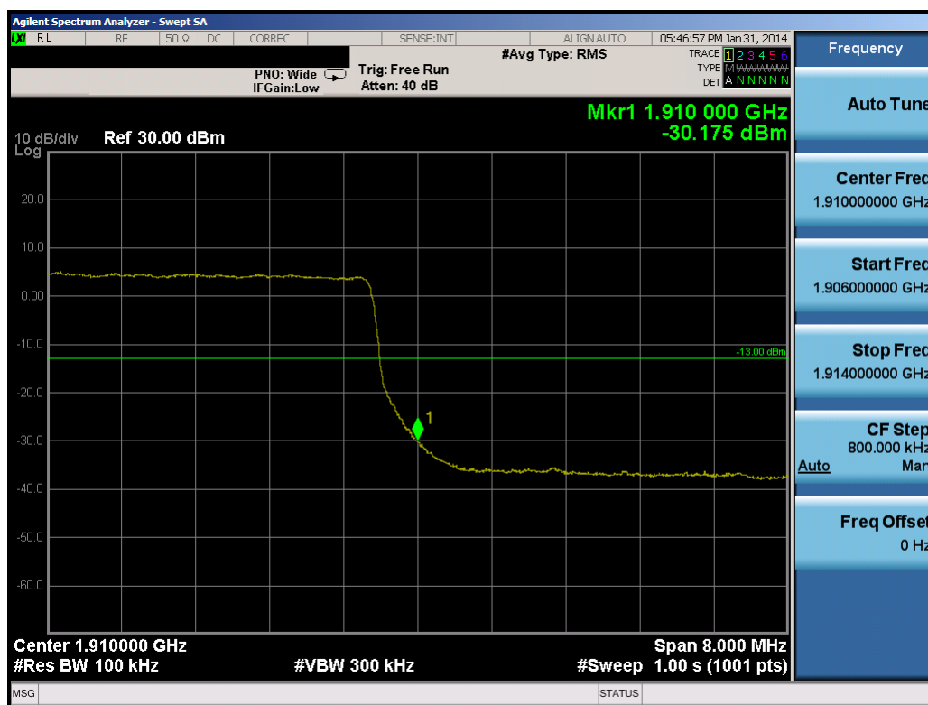
Plot 10-53. Upper Band Edge Plot (10.0MHz QPSK – RB Size 50)
