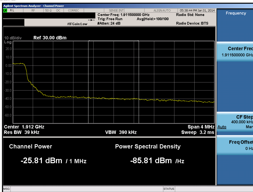
Plot 10-40. Upper Extended Band Edge Plot (5.0MHz QPSK – RB Size 25)
