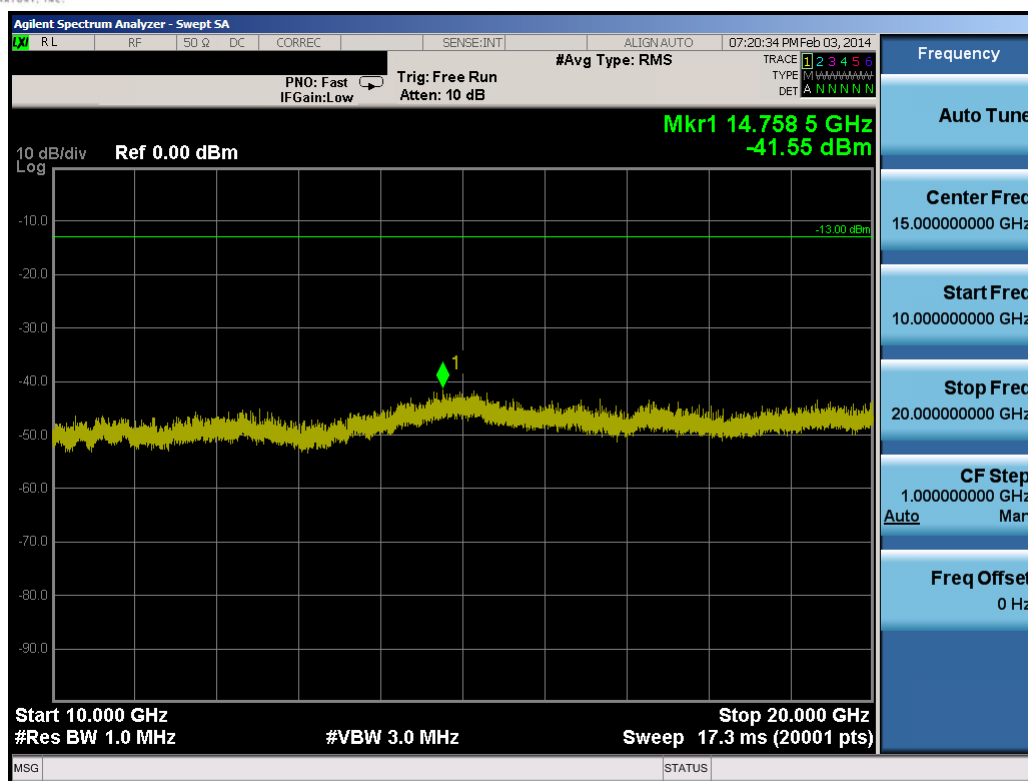
Plot 9-76. Conducted Spurious Plot (20.0MHz QPSK – RB Size 1, RB Offset 0 – Low Channel)
