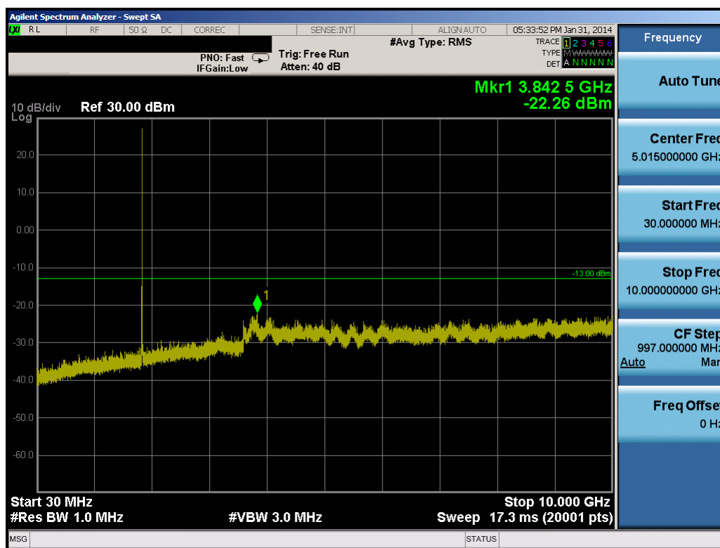
Plot 10-33. Conducted Spurious Plot (5.0MHz QPSK – RB Size 1, RB Offset 0 – Low Channel)
