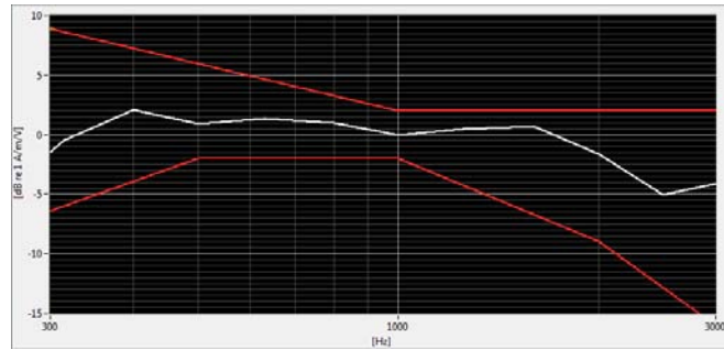
Figure 7-1 Axial Frequency Response
